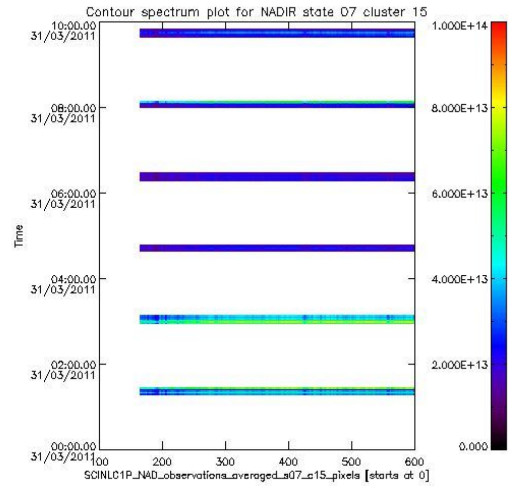
sciamachy_i1b_source_packet_report_SCIA_7_04_U_20110331_4.PNG
