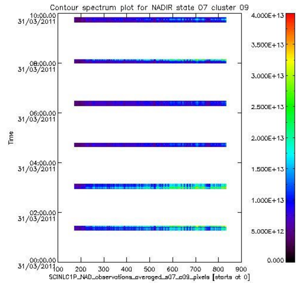
sciamachy_i1b_source_packet_report_SCIA_7_04_U_20110331_2.PNG
