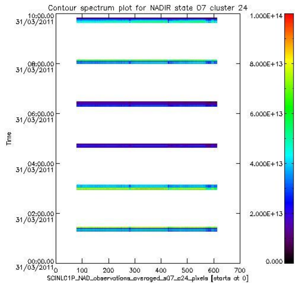
sciamachy_i1b_source_packet_report_SCIA_7_04_U_20110331_6.PNG
