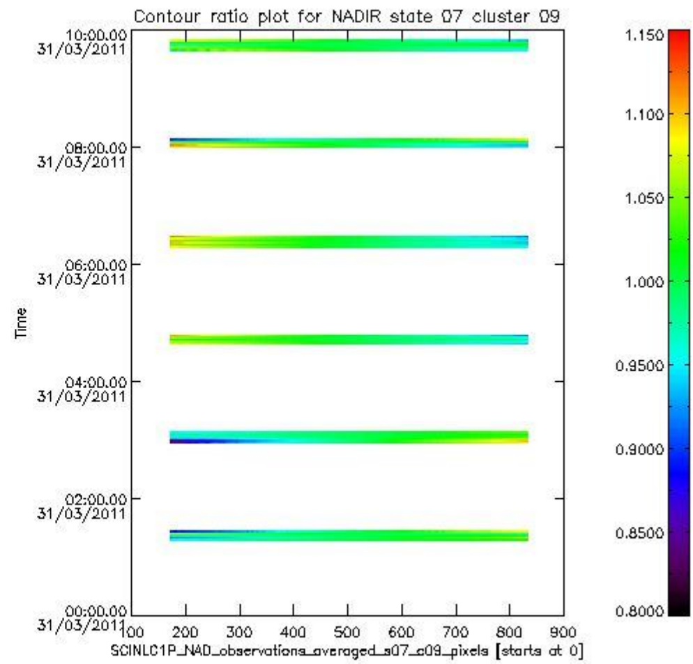
sciamachy_i1b_source_packet_report_SCIA_7_04_U_20110331_3.PNG
