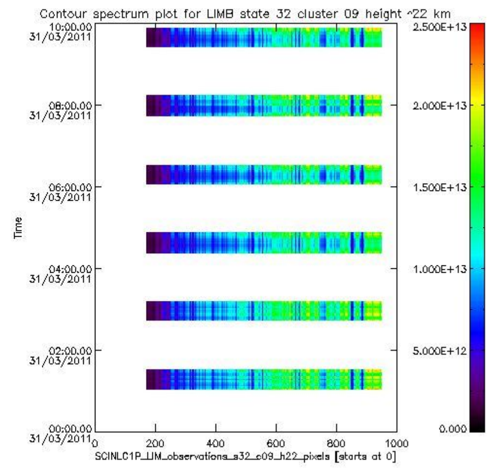
sciamachy_i1b_source_packet_report_SCIA_7_04_U_20110331_12.PNG
