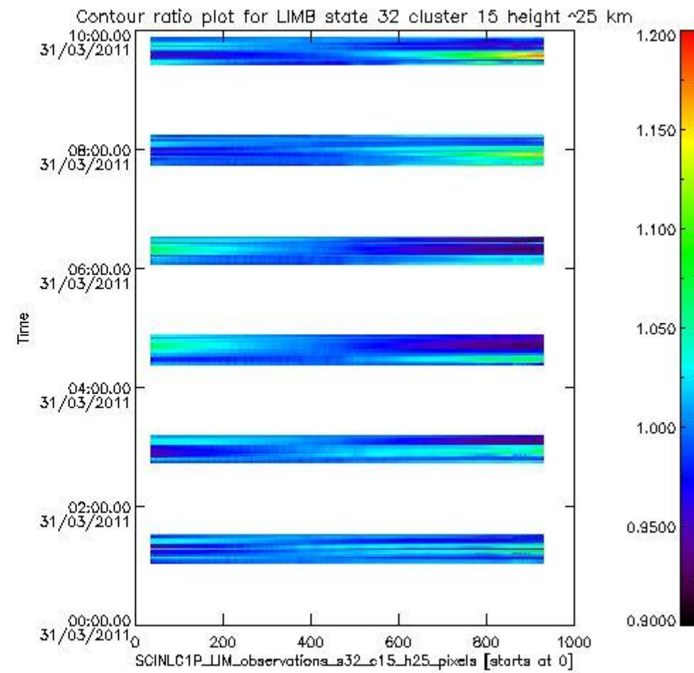
sciamachy_11b_source_packet_report_SCIA_7_04_U_20110331_19.PNG
