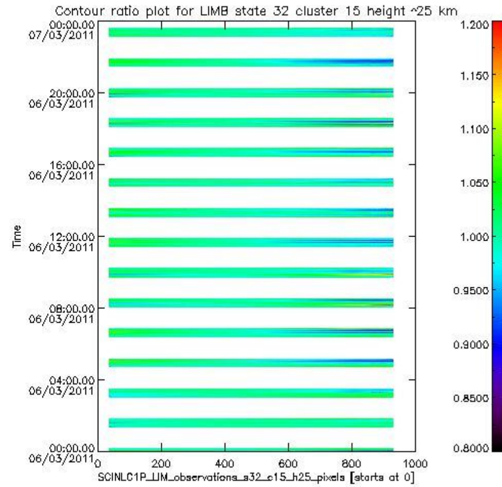
sciamachy_11b_source_packet_report_SCIA_7_04_U_20110306_19.PNG
