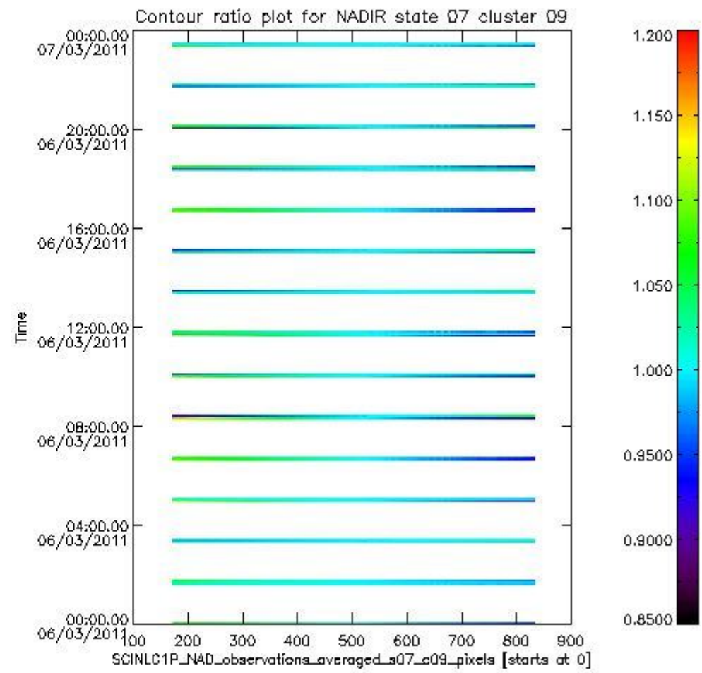
sciamachy_i1b_source_packet_report_SCIA_7_04_U_20110306_3.PNG
