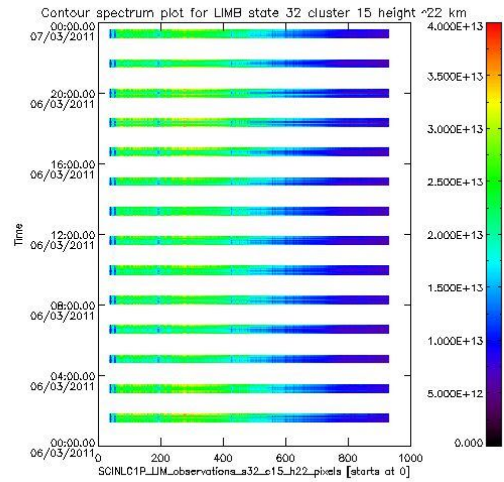
sciamachy_i1b_source_packet_report_SCIA_7_04_U_20110306_16.PNG
