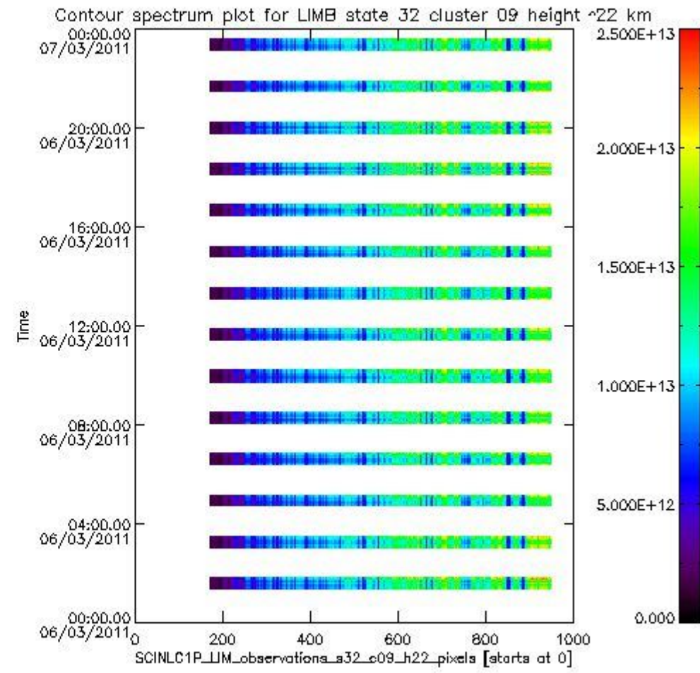
sciamachy_i1b_source_packet_report_SCIA_7_04_U_20110306_12.PNG
