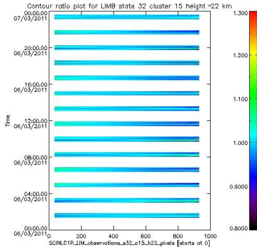
sciamachy_11b_source_packet_report_SCIA_7_04_U_20110306_17.PNG
