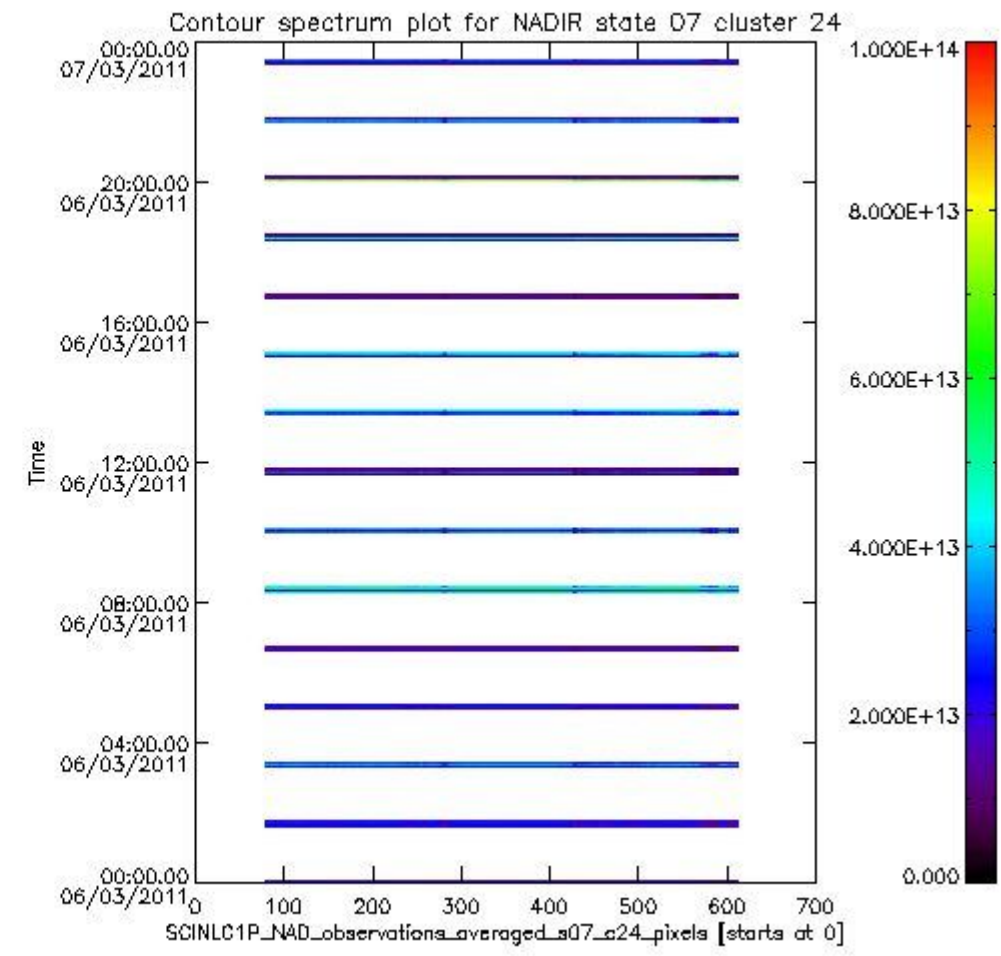
sciamachy_i1b_source_packet_report_SCIA_7_04_U_20110306_6.PNG
