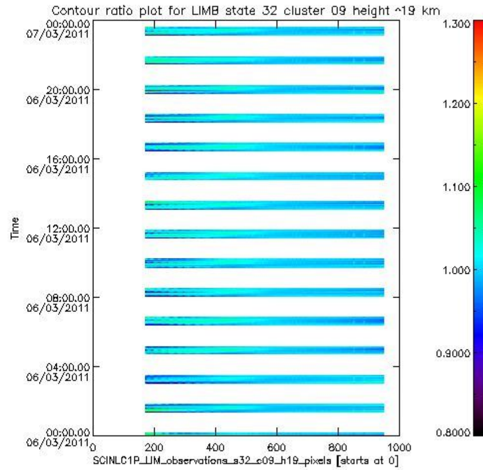
sciamachy_i1b_source_packet_report_SCIA_7_04_U_20110306_11.PNG
