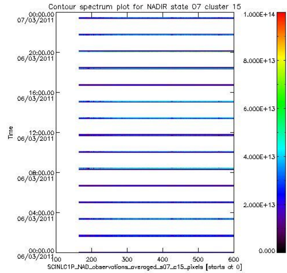
sciamachy_i1b_source_packet_report_SCIA_7_04_U_20110306_4.PNG
