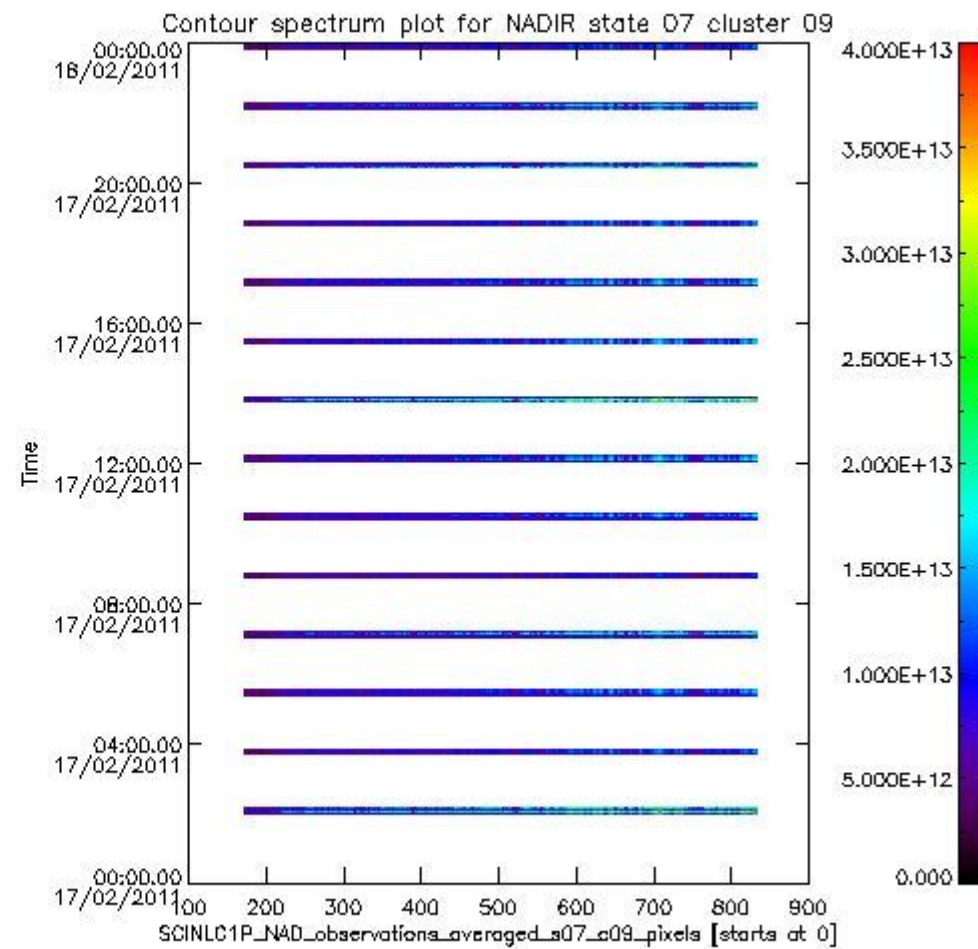
sciamachy_i1b_source_packet_report_SCIA_7_04_U_20110217_2.PNG
