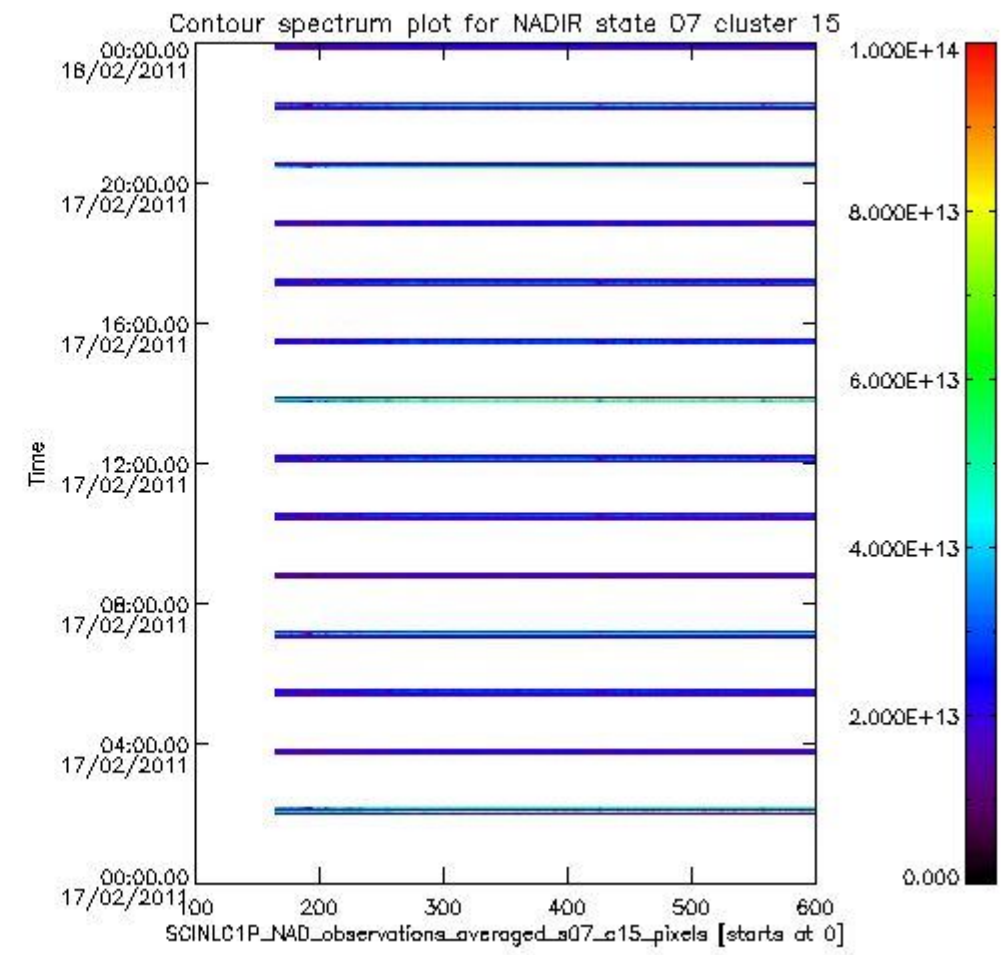
sciamachy_i1b_source_packet_report_SCIA_7_04_U_20110217_4.PNG
