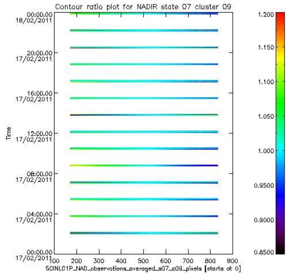
sciamachy_i1b_source_packet_report_SCIA_7_04_U_20110217_3.PNG
