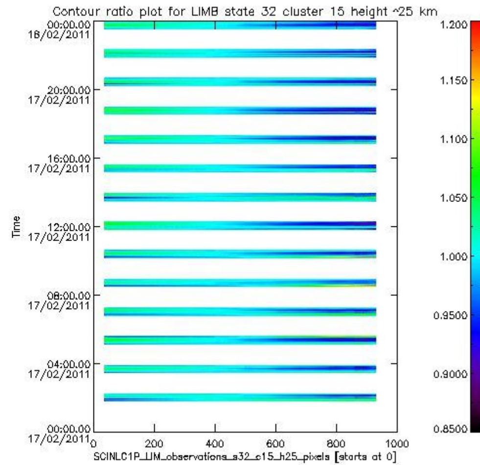
sciamachy_11b_source_packet_report_SCIA_7_04_U_20110217_19.PNG
