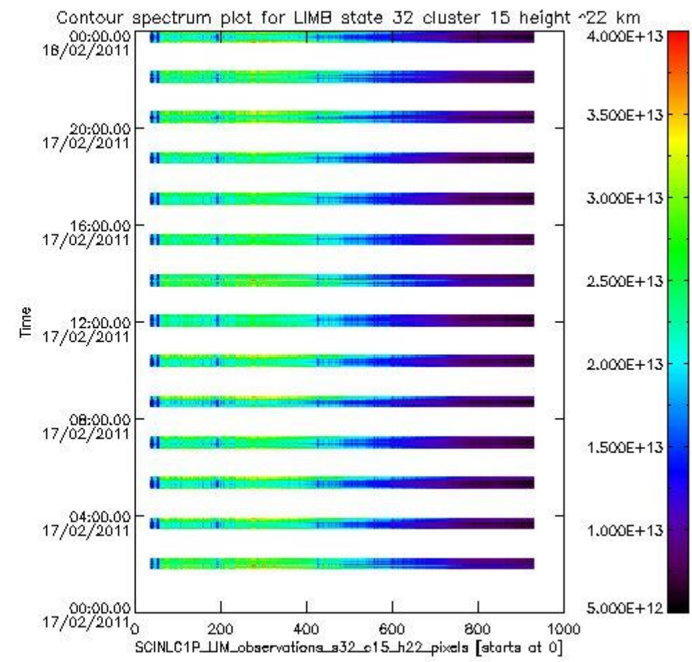
sciamachy_i1b_source_packet_report_SCIA_7_04_U_20110217_16.PNG
