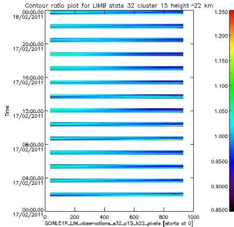
sciamachy_11b_source_packet_report_SCIA_7_04_U_20110217_17.PNG
