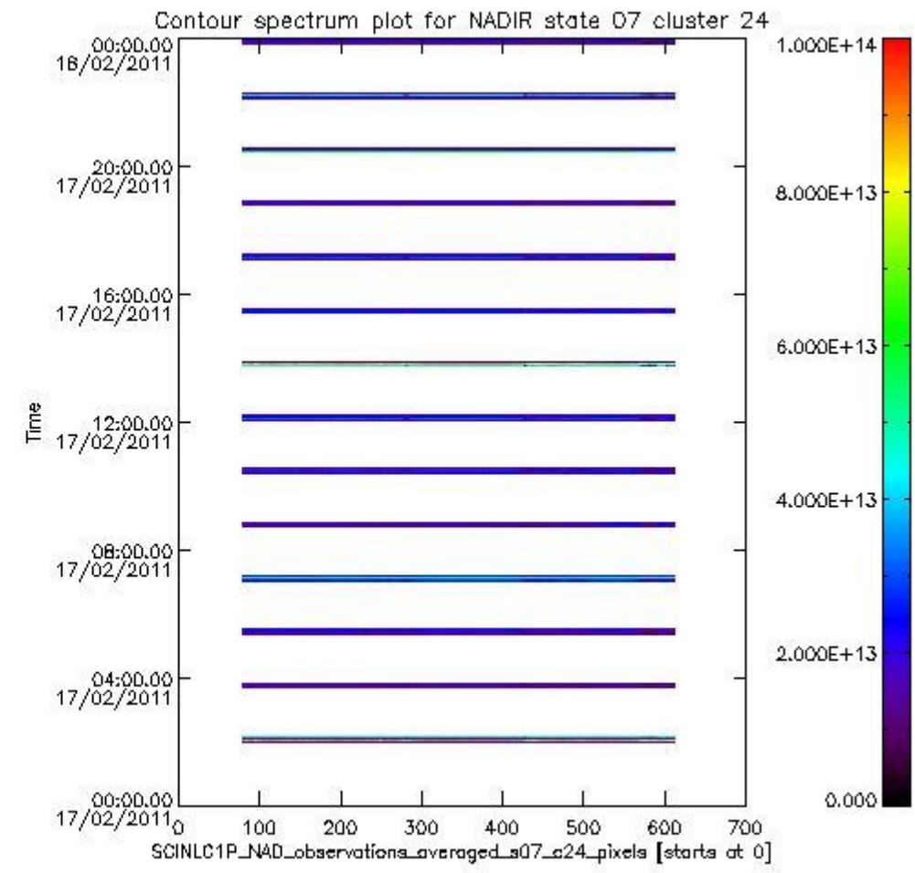
sciamachy_i1b_source_packet_report_SCIA_7_04_U_20110217_6.PNG
