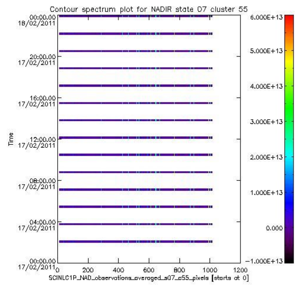
sciamachy_i1b_source_packet_report_SCIA_7_04_U_20110217_8.PNG
