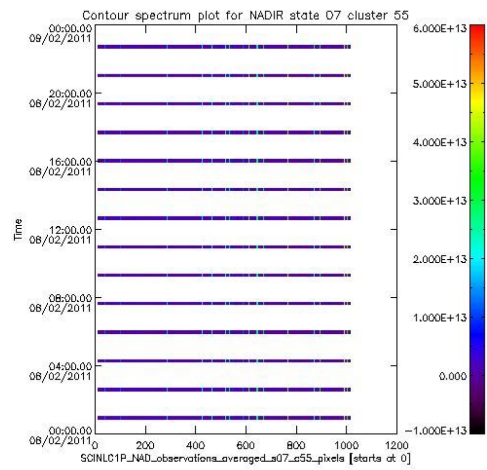
sciamachy_i1b_source_packet_report_SCIA_7_04_U_20110208_8.PNG
