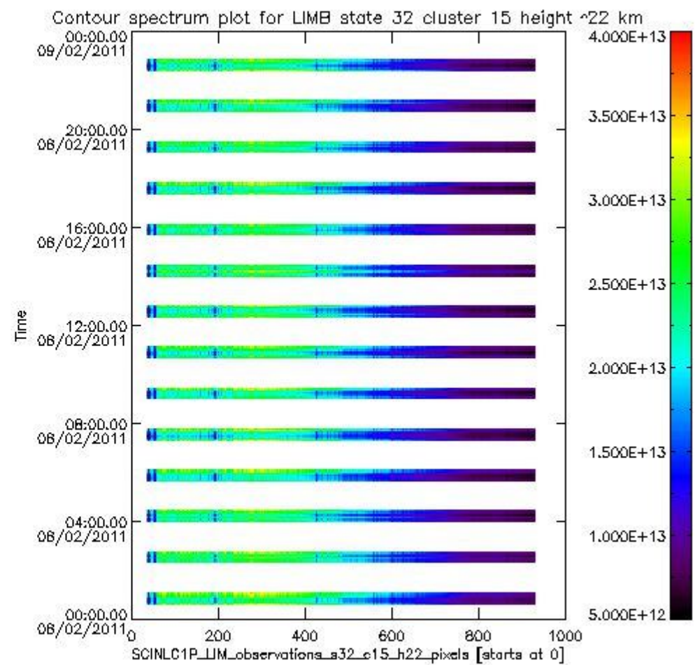
sciamachy_i1b_source_packet_report_SCIA_7_04_U_20110208_16.PNG
