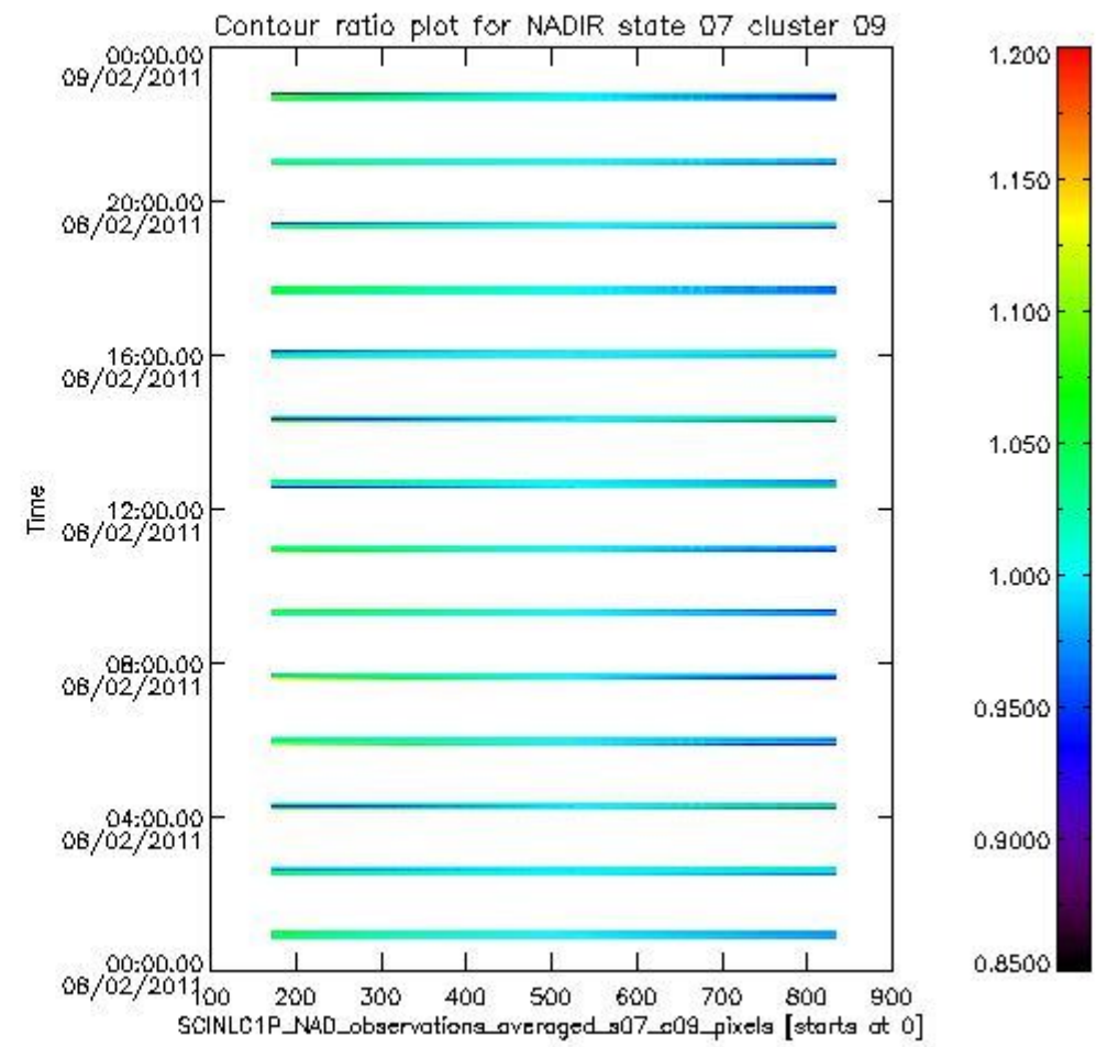
sciamachy_i1b_source_packet_report_SCIA_7_04_U_20110208_3.PNG
