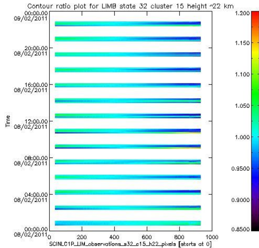
sciamachy_11b_source_packet_report_SCIA_7_04_U_20110208_17.PNG
