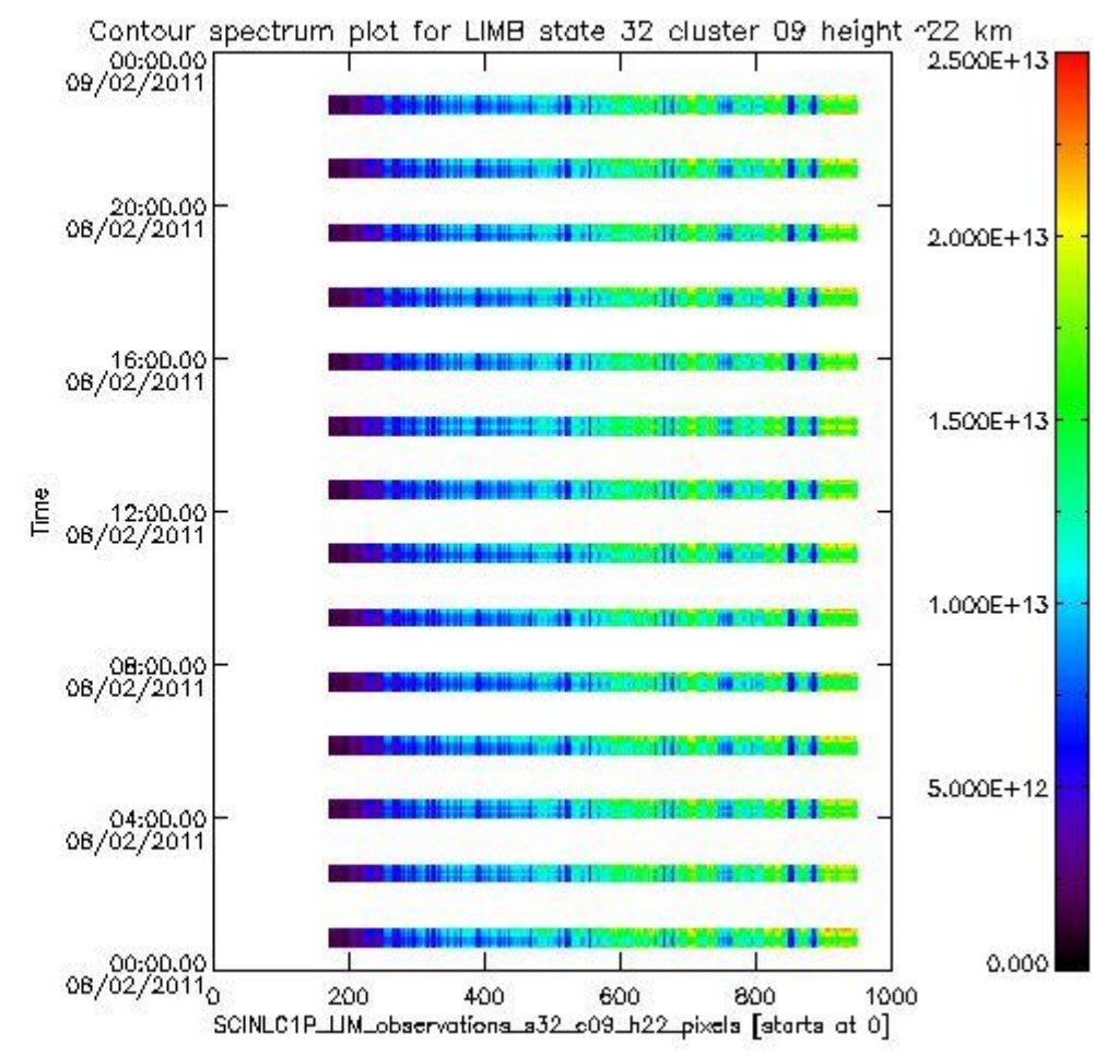
sciamachy_i1b_source_packet_report_SCIA_7_04_U_20110208_12.PNG
