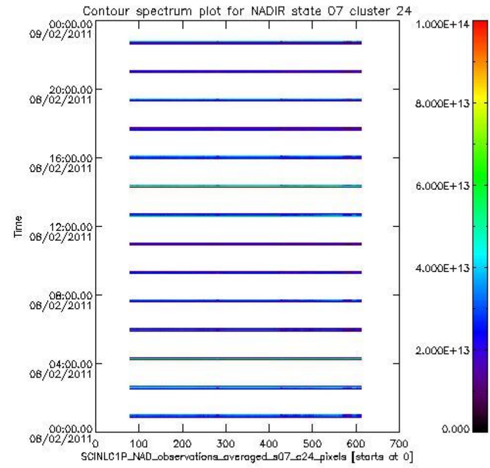
sciamachy_i1b_source_packet_report_SCIA_7_04_U_20110208_6.PNG
