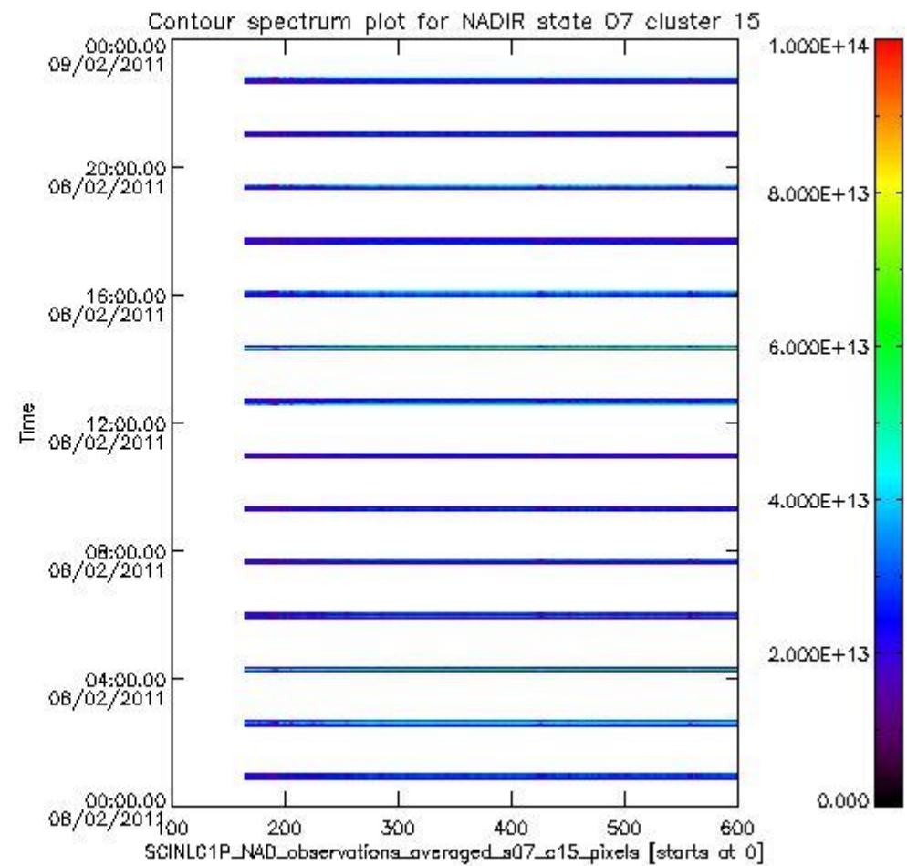
sciamachy_i1b_source_packet_report_SCIA_7_04_U_20110208_4.PNG
