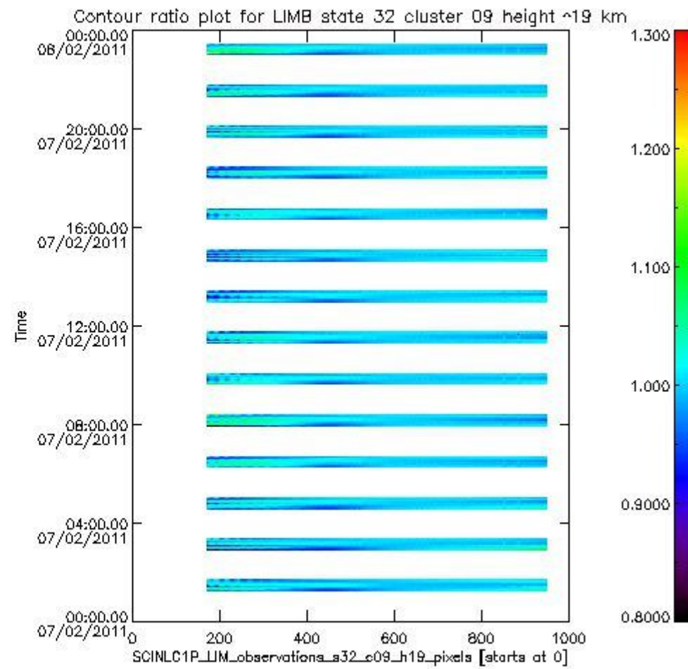
sciamachy_i1b_source_packet_report_SCIA_7_04_U_20110207_11.PNG
