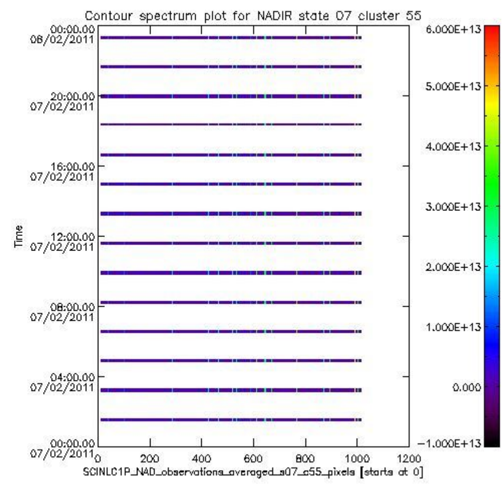
sciamachy_l1b_source_packet_report_SCIA_7_04_U_20110207_8.PNG
