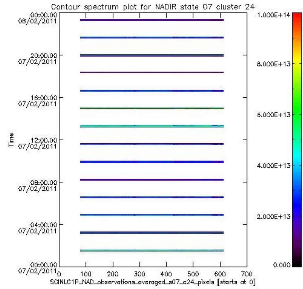
sciamachy_i1b_source_packet_report_SCIA_7_04_U_20110207_6.PNG
