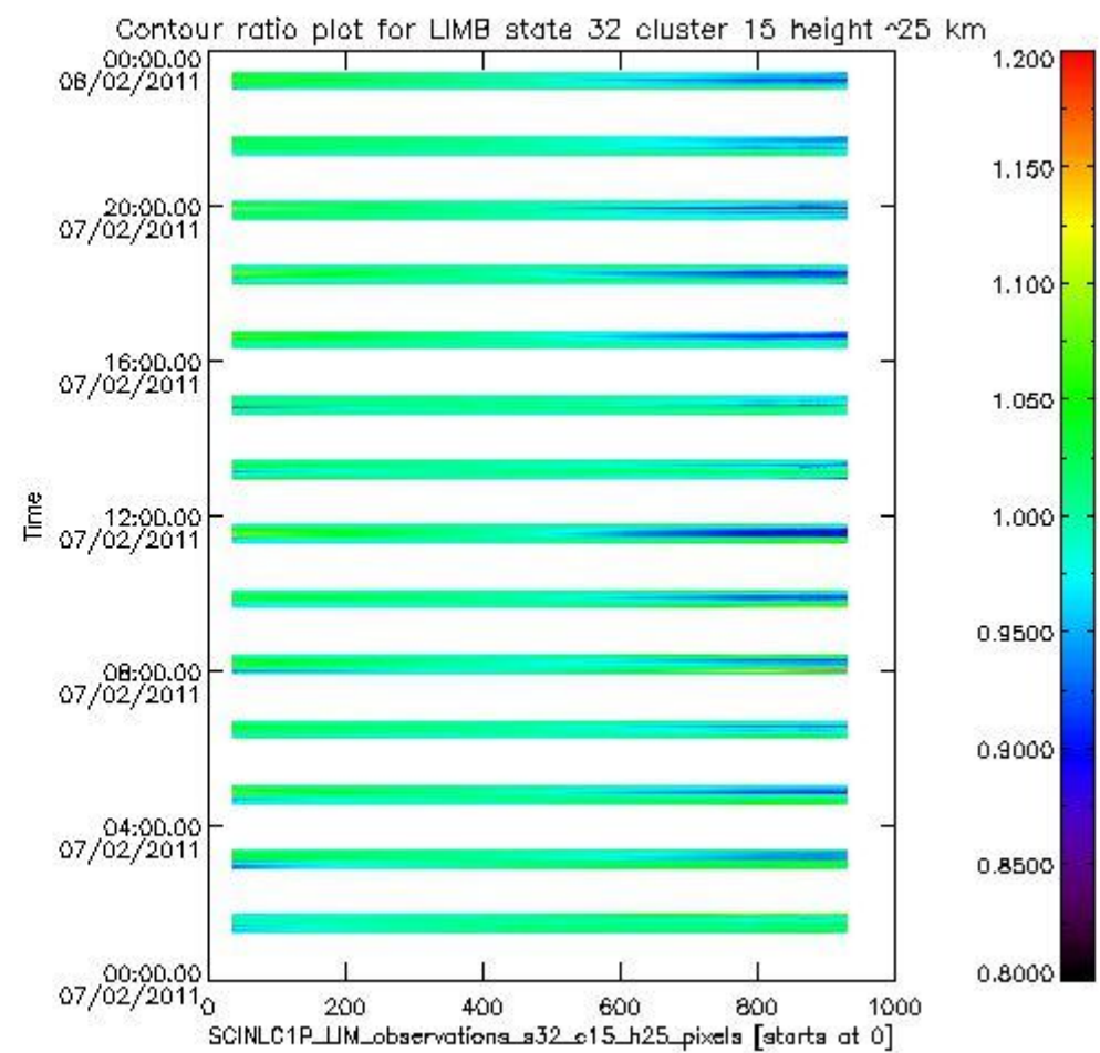
sciamachy_11b_source_packet_report_SCIA_7_04_U_20110207_19.PNG
