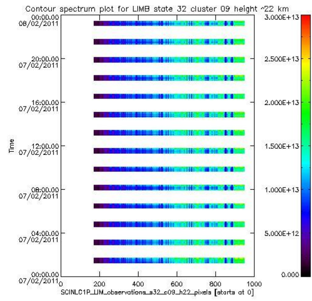
sciamachy_i1b_source_packet_report_SCIA_7_04_U_20110207_12.PNG
