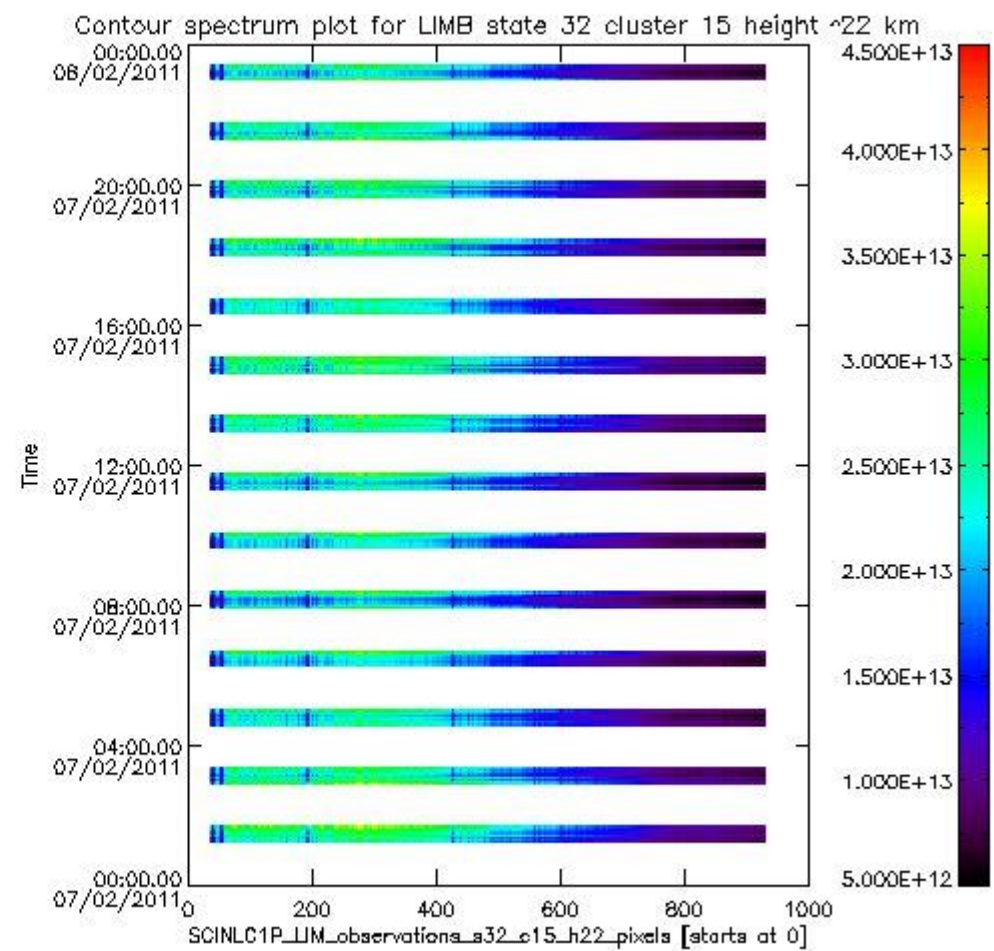
sciamachy_i1b_source_packet_report_SCIA_7_04_U_20110207_16.PNG
