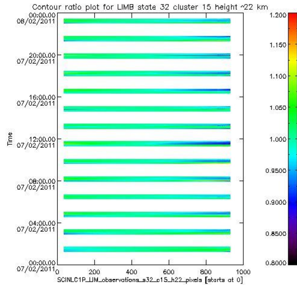
sciamachy_11b_source_packet_report_SCIA_7_04_U_20110207_17.PNG
