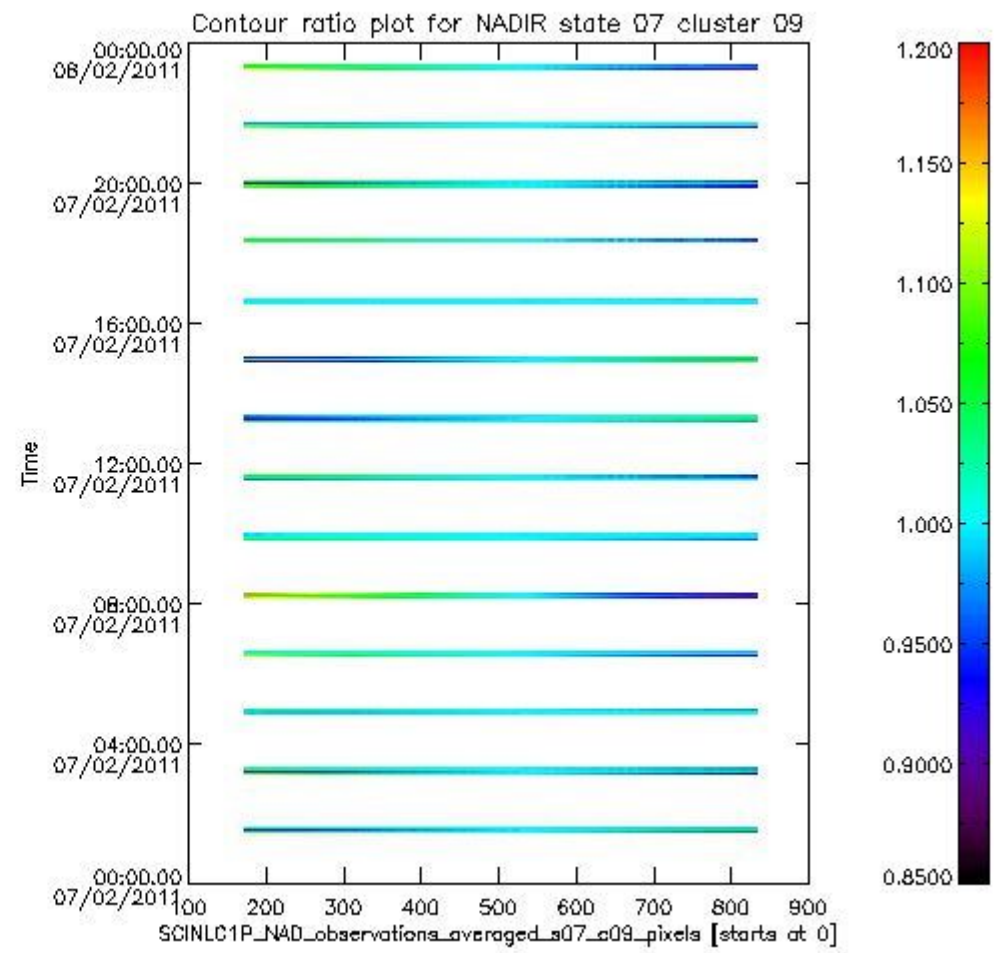
sciamachy_i1b_source_packet_report_SCIA_7_04_U_20110207_3.PNG
