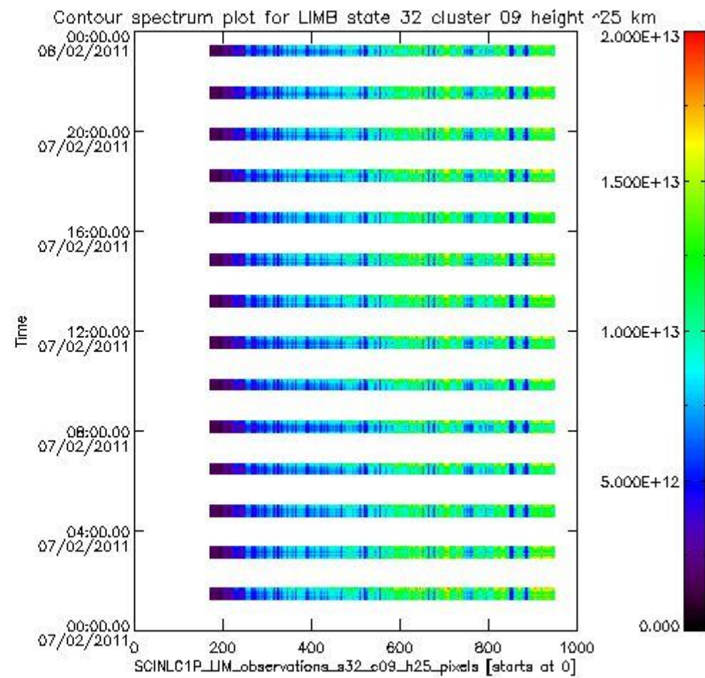
sciamachy_i1b_source_packet_report_SCIA_7_04_U_20110207_14.PNG
