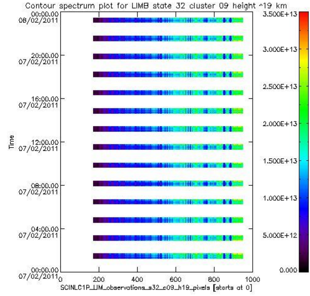
sciamachy_i1b_source_packet_report_SCIA_7_04_U_20110207_10.PNG
