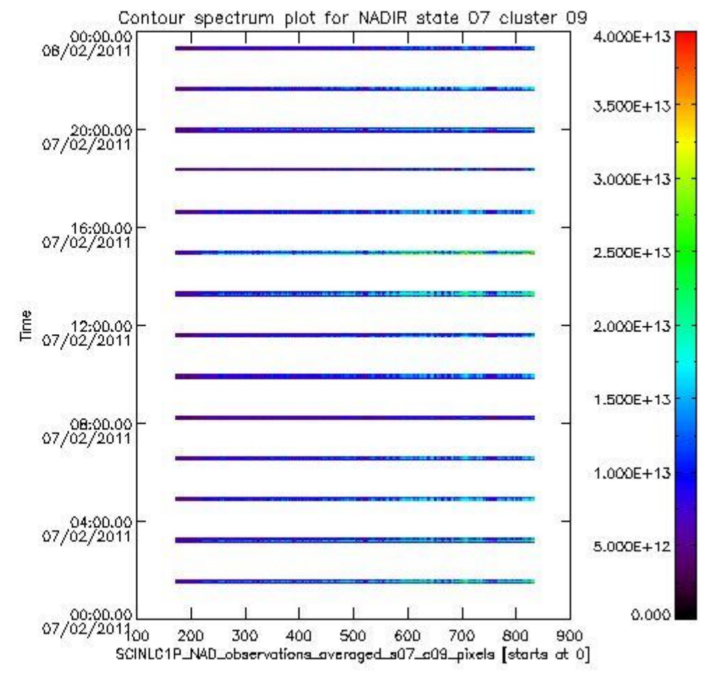
sciamachy_i1b_source_packet_report_SCIA_7_04_U_20110207_2.PNG
