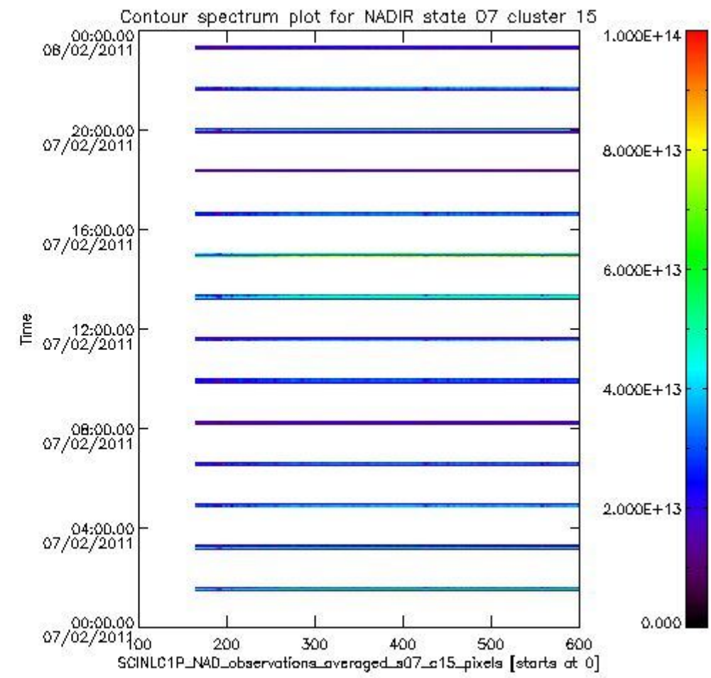
sciamachy_i1b_source_packet_report_SCIA_7_04_U_20110207_4.PNG
