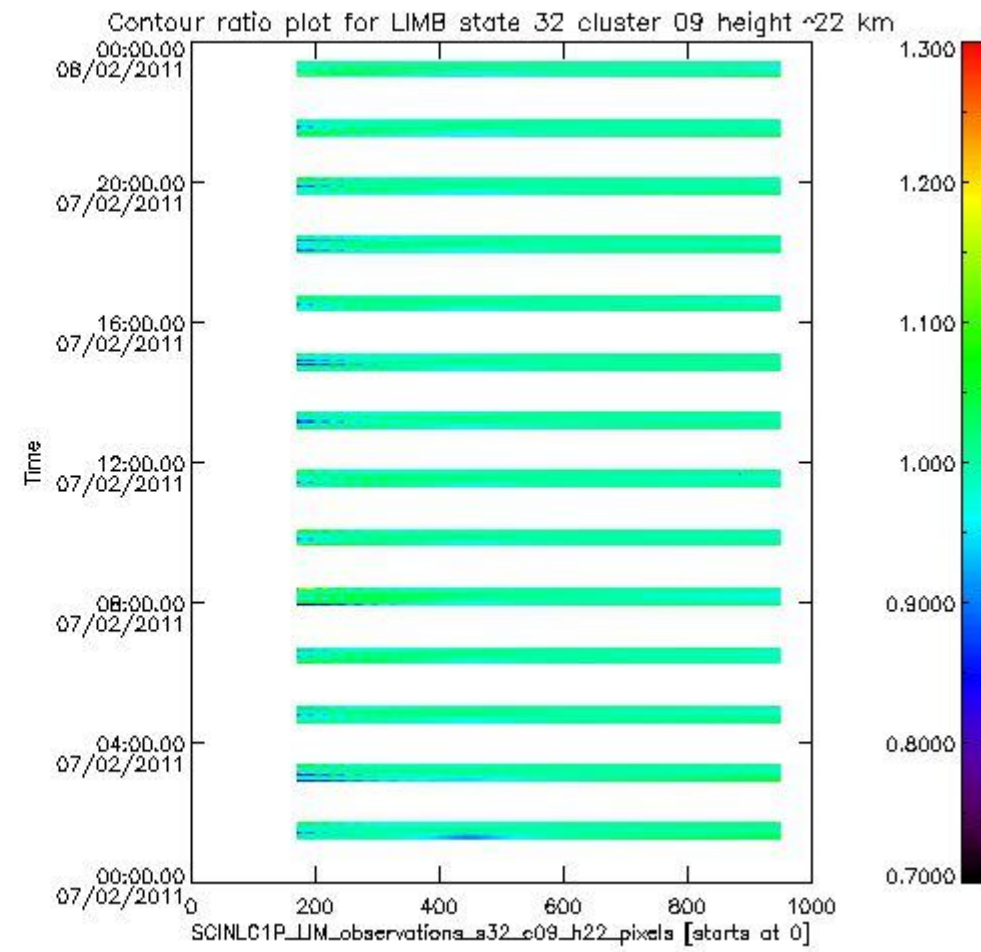
sciamachy_l1b_source_packet_report_SCIA_7_04_U_20110207_13.PNG
