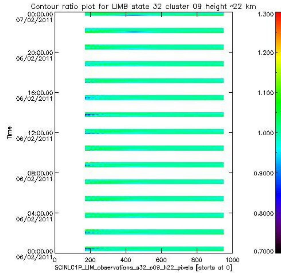
sciamachy_l1b_source_packet_report_SCIA_7_04_U_20110206_13.PNG
