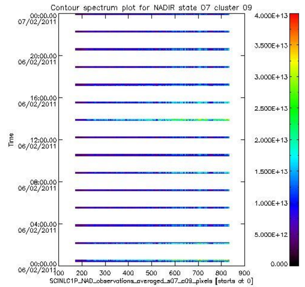
sciamachy_i1b_source_packet_report_SCIA_7_04_U_20110206_2.PNG
