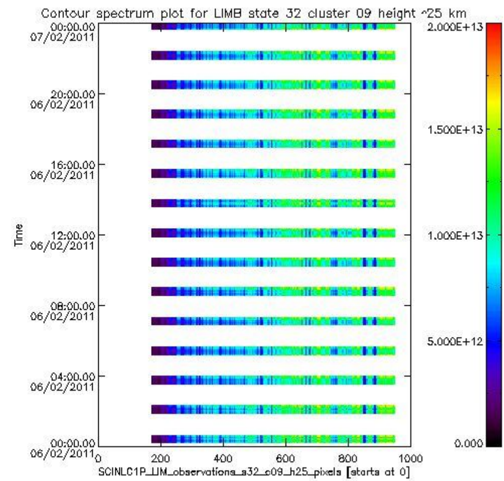
sciamachy_l1b_source_packet_report_SCIA_7_04_U_20110206_14.PNG
