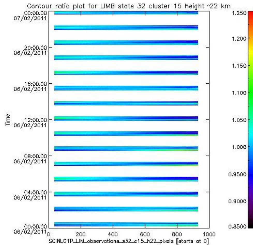
sciamachy_11b_source_packet_report_SCIA_7_04_U_20110206_17.PNG
