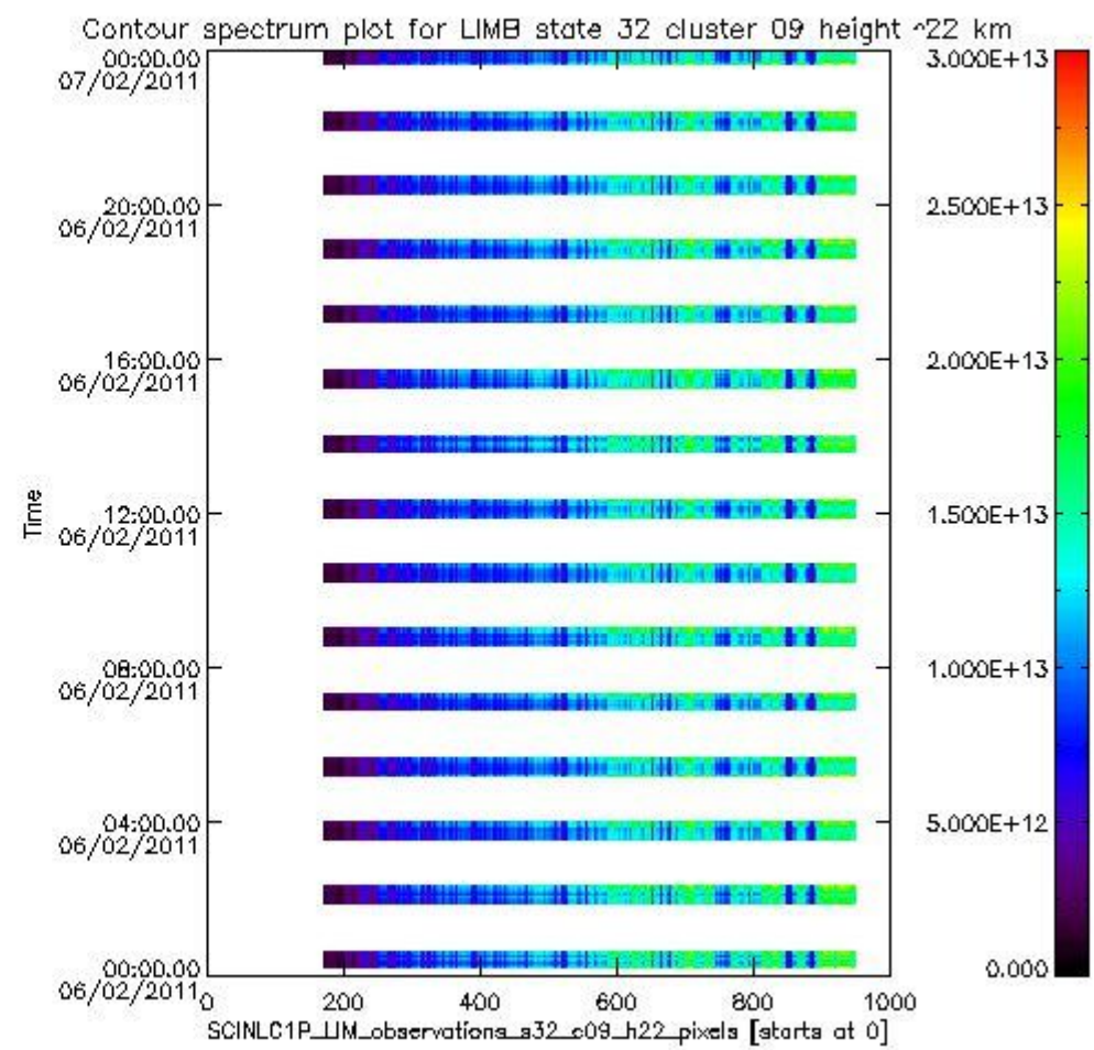
sciamachy_i1b_source_packet_report_SCIA_7_04_U_20110206_12.PNG
