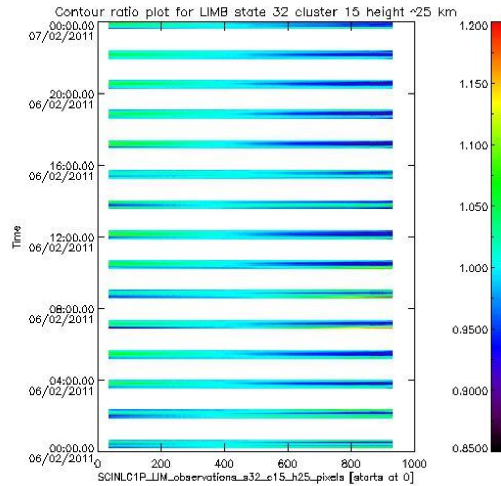
sciamachy_11b_source_packet_report_SCIA_7_04_U_20110206_19.PNG
