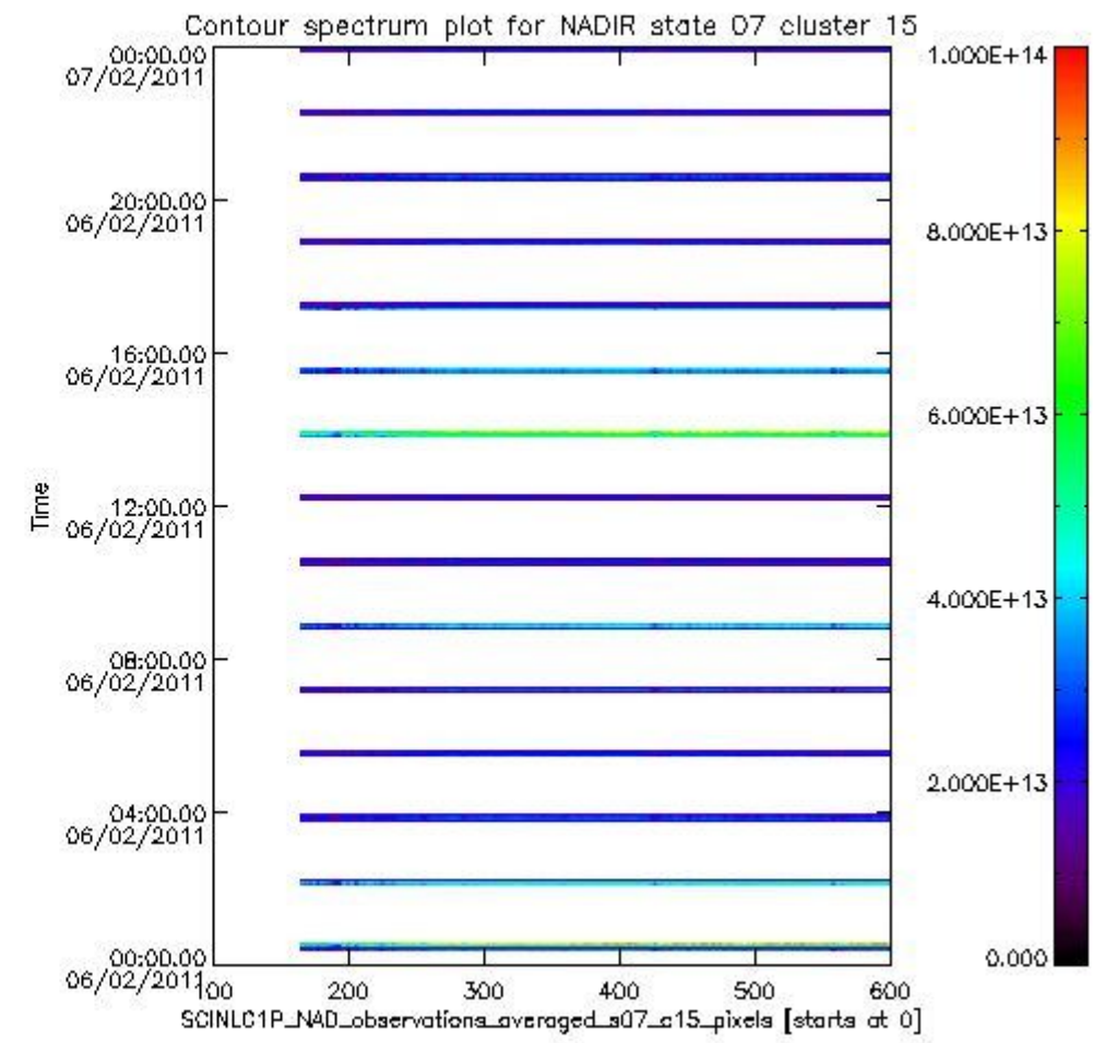
sciamachy_i1b_source_packet_report_SCIA_7_04_U_20110206_4.PNG
