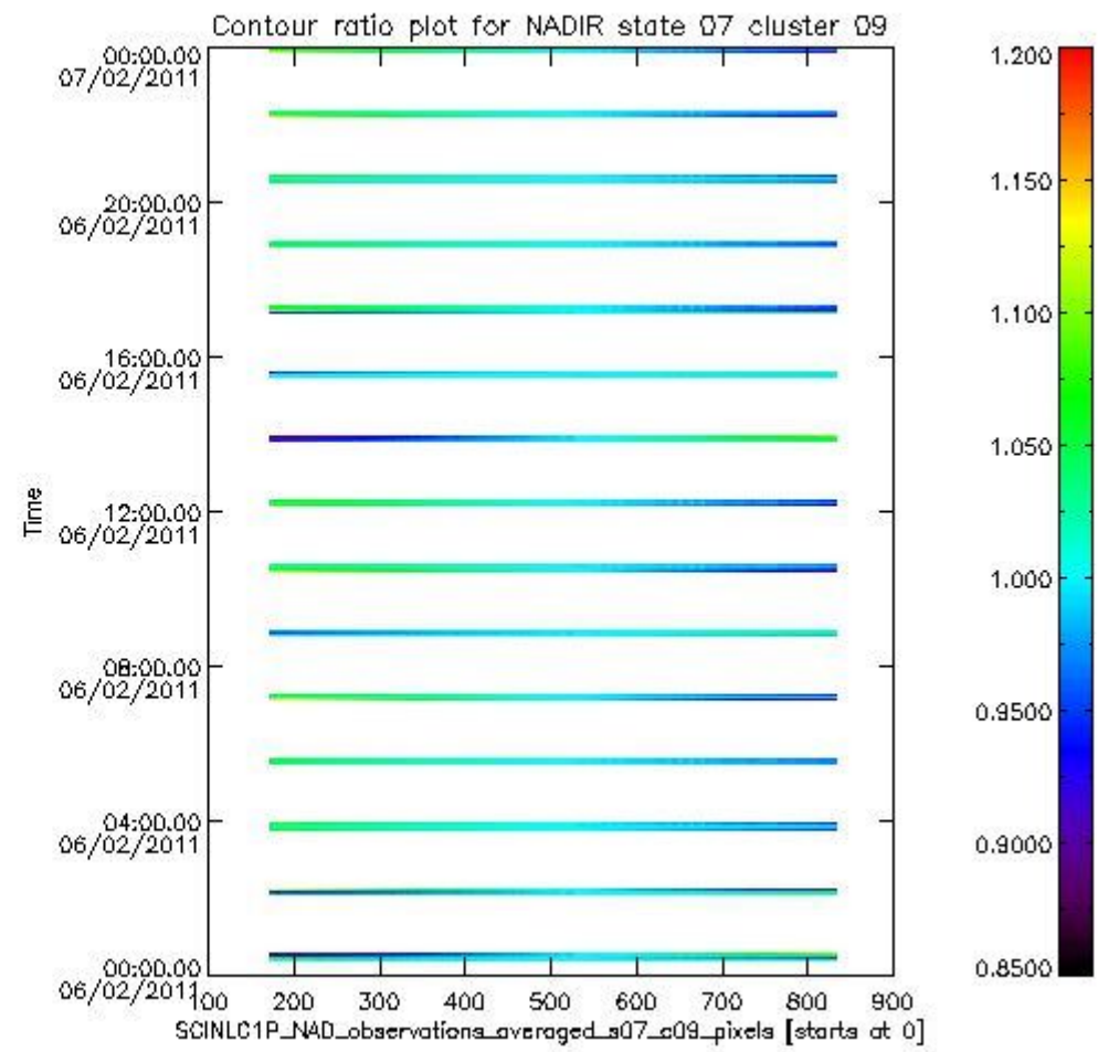
sciamachy_i1b_source_packet_report_SCIA_7_04_U_20110206_3.PNG
