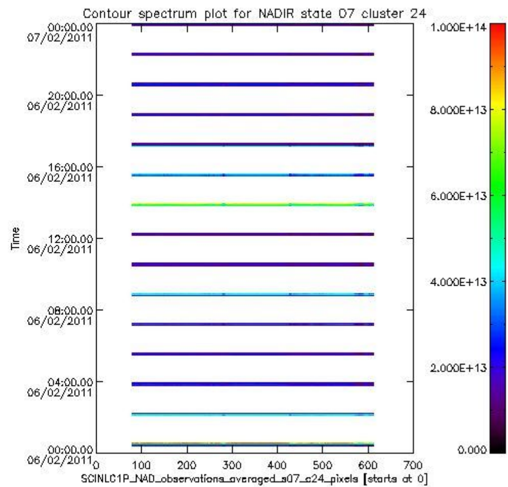
sciamachy_i1b_source_packet_report_SCIA_7_04_U_20110206_6.PNG
