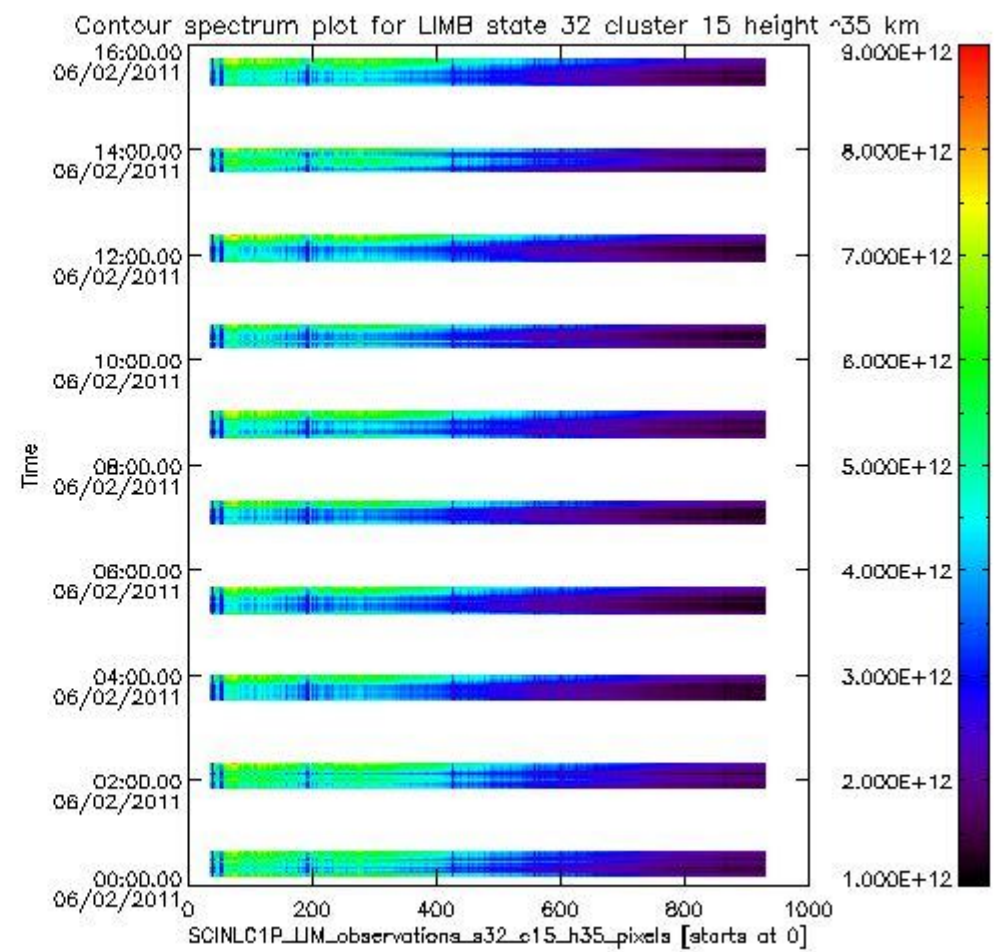
sciamachy_11b_source_packet_report_SCIA_7_04_U_20110206_20.PNG
