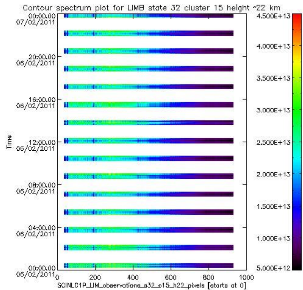
sciamachy_i1b_source_packet_report_SCIA_7_04_U_20110206_16.PNG
