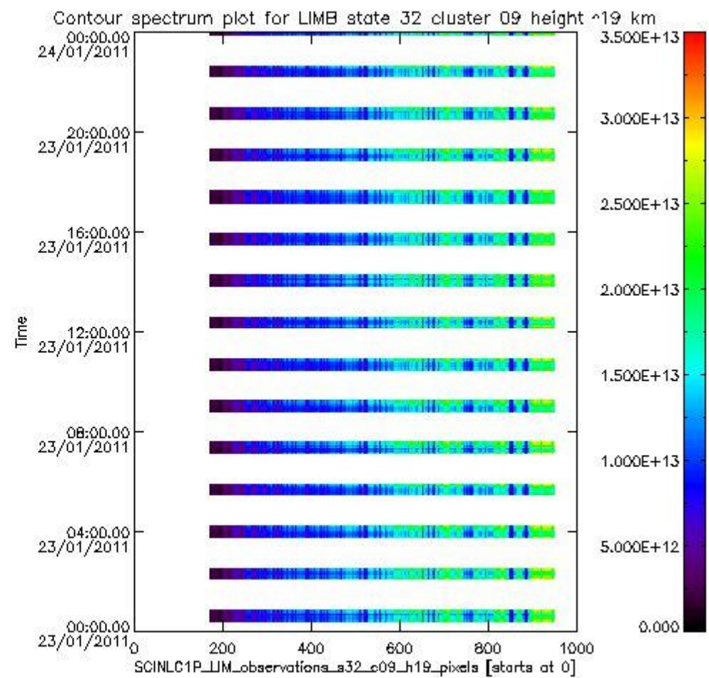
sciamachy_i1b_source_packet_report_SCIA_7_04_U_20110123_10.PNG
