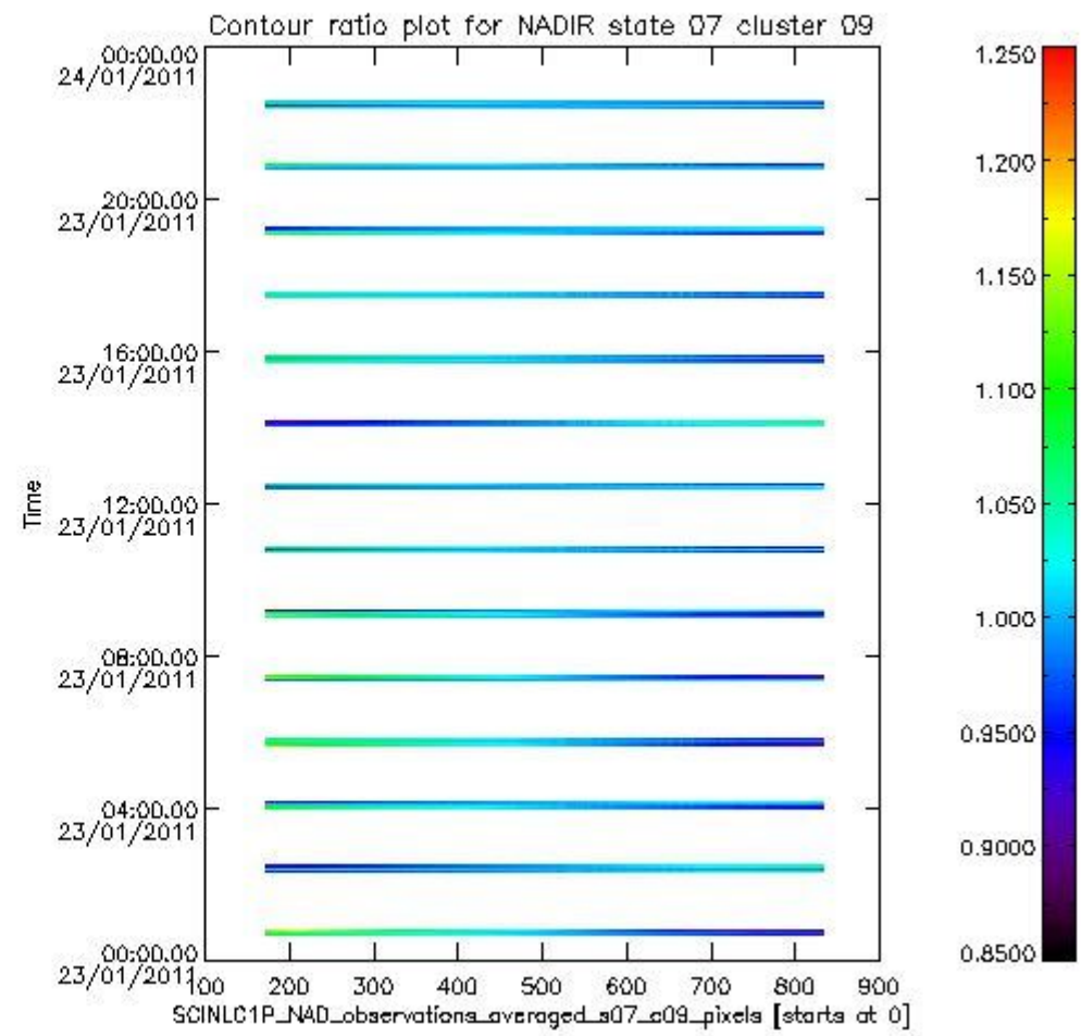
sciamachy_i1b_source_packet_report_SCIA_7_04_U_20110123_3.PNG
