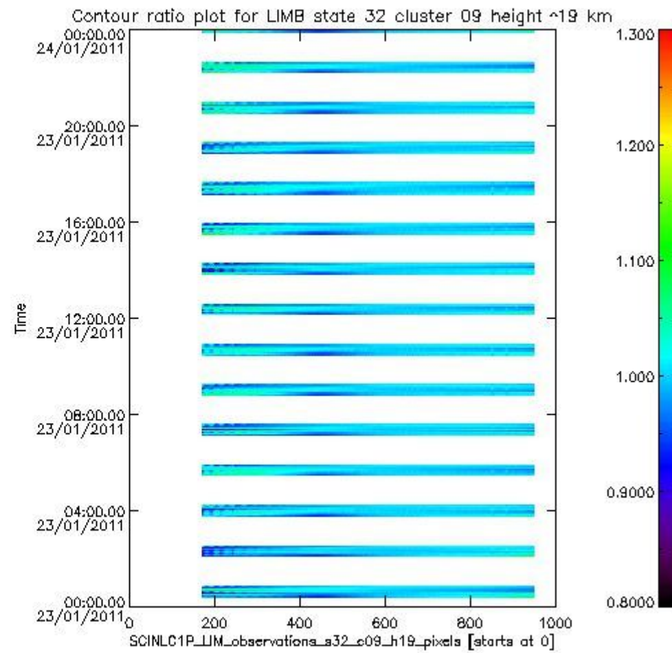
sciamachy_i1b_source_packet_report_SCIA_7_04_U_20110123_11.PNG
