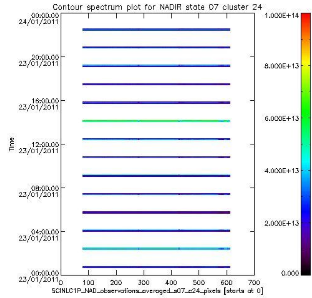
sciamachy_i1b_source_packet_report_SCIA_7_04_U_20110123_6.PNG
