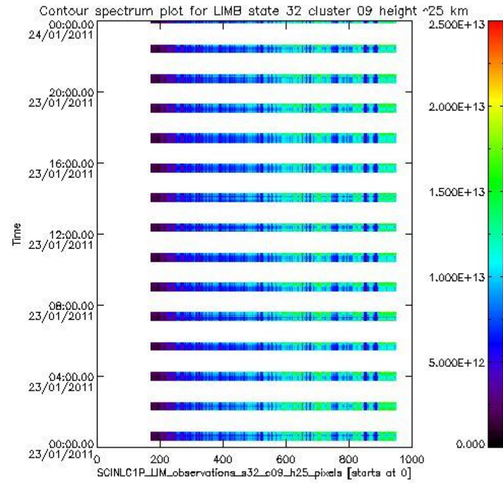
sciamachy_i1b_source_packet_report_SCIA_7_04_U_20110123_14.PNG
