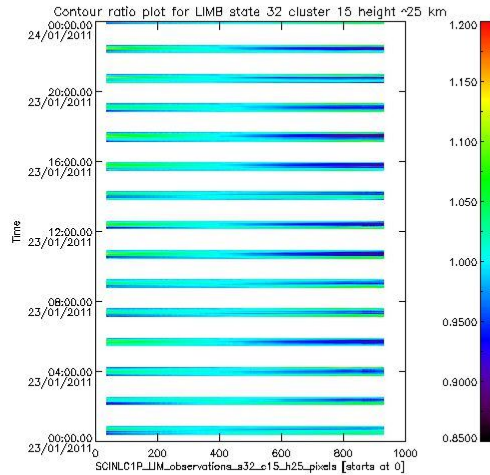
sciamachy_11b_source_packet_report_SCIA_7_04_U_20110123_19.PNG
