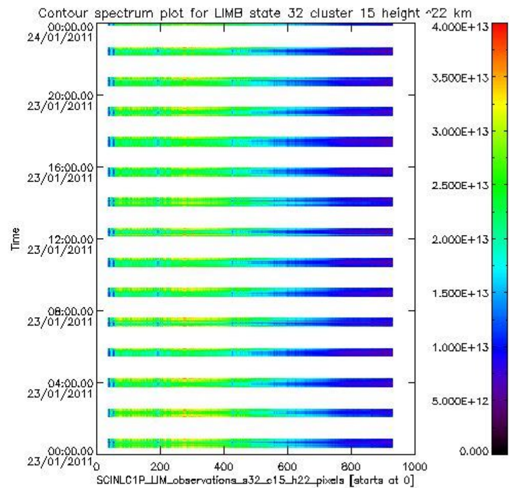
sciamachy_i1b_source_packet_report_SCIA_7_04_U_20110123_16.PNG
