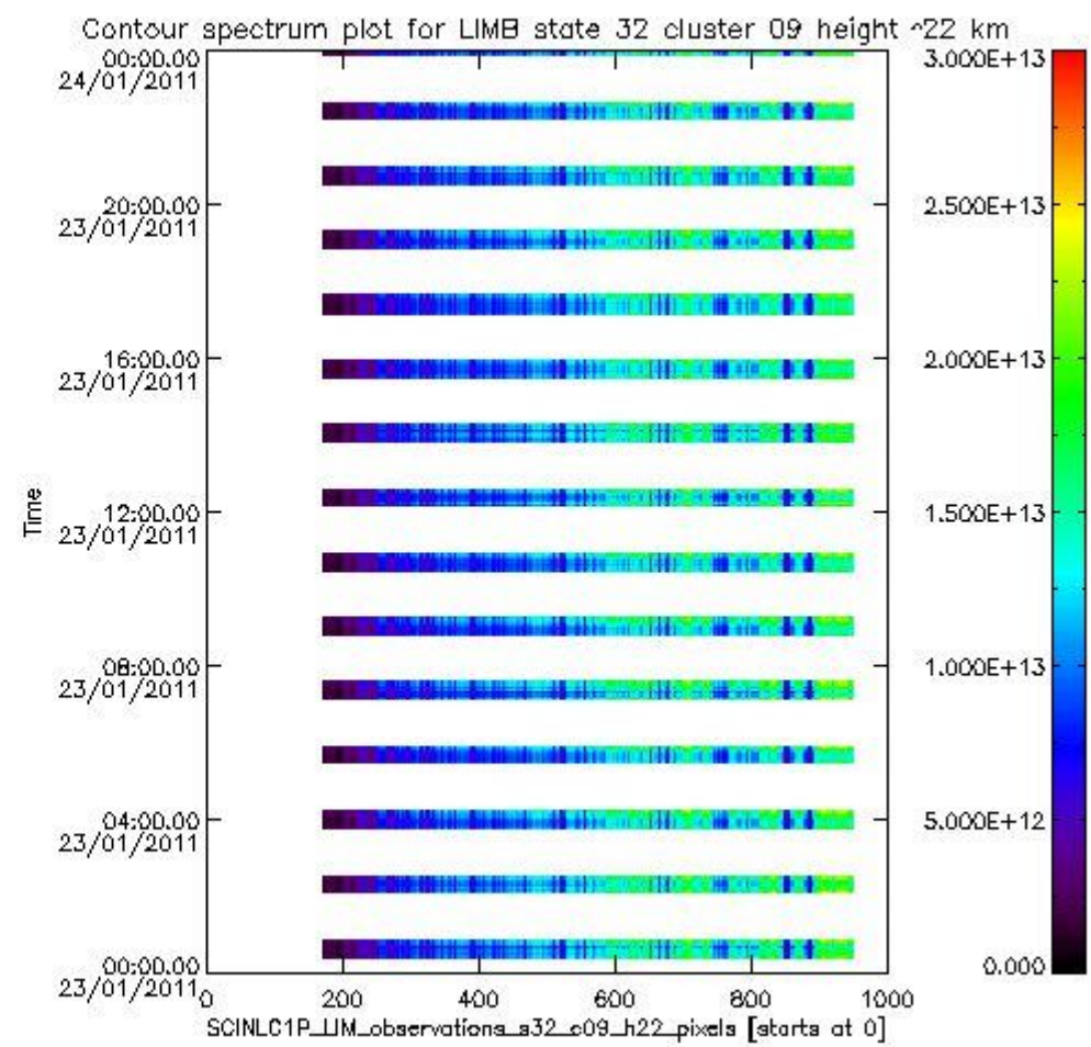
sciamachy_i1b_source_packet_report_SCIA_7_04_U_20110123_12.PNG
