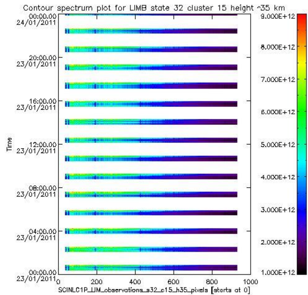
sciamachy_11b_source_packet_report_SCIA_7_04_U_20110123_20.PNG
