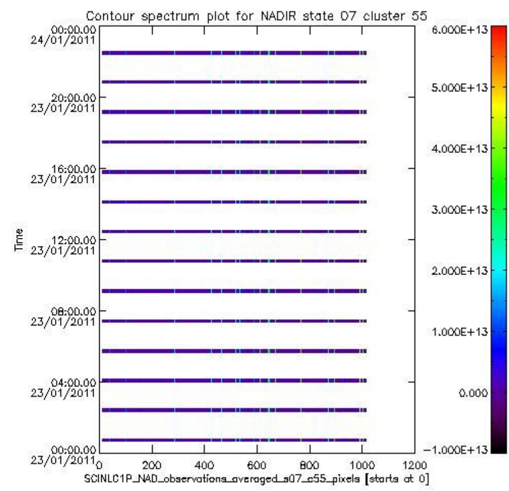
sciamachy_i1b_source_packet_report_SCIA_7_04_U_20110123_8.PNG
