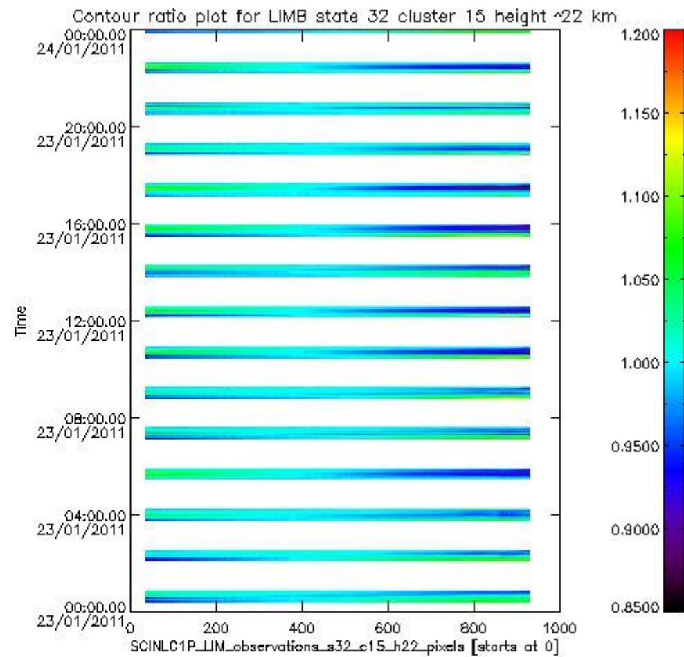
sciamachy_11b_source_packet_report_SCIA_7_04_U_20110123_17.PNG
