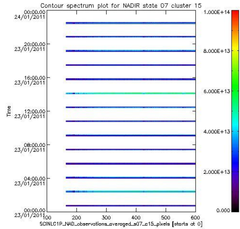
sciamachy_i1b_source_packet_report_SCIA_7_04_U_20110123_4.PNG
