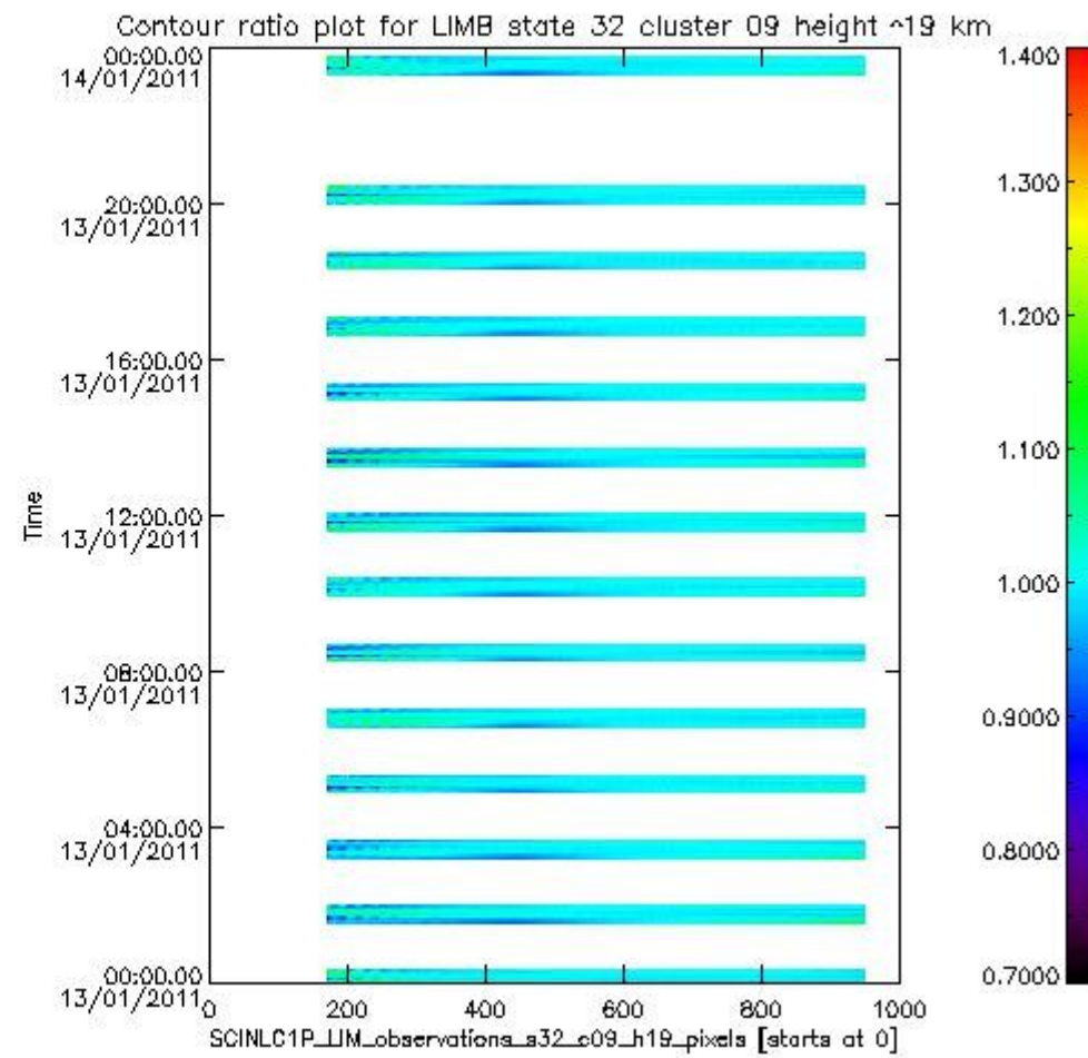
sciamachy_i1b_source_packet_report_SCIA_7_04_U_20110113_11.PNG
