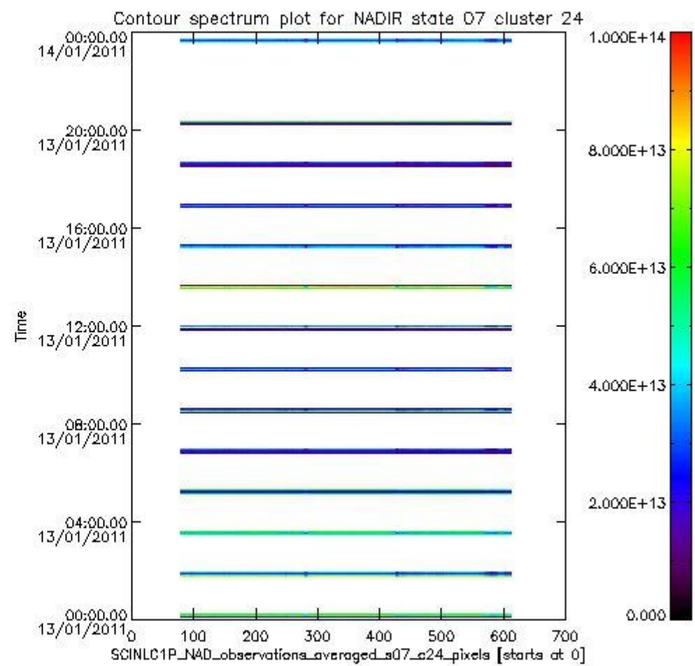
sciamachy_i1b_source_packet_report_SCIA_7_04_U_20110113_6.PNG
