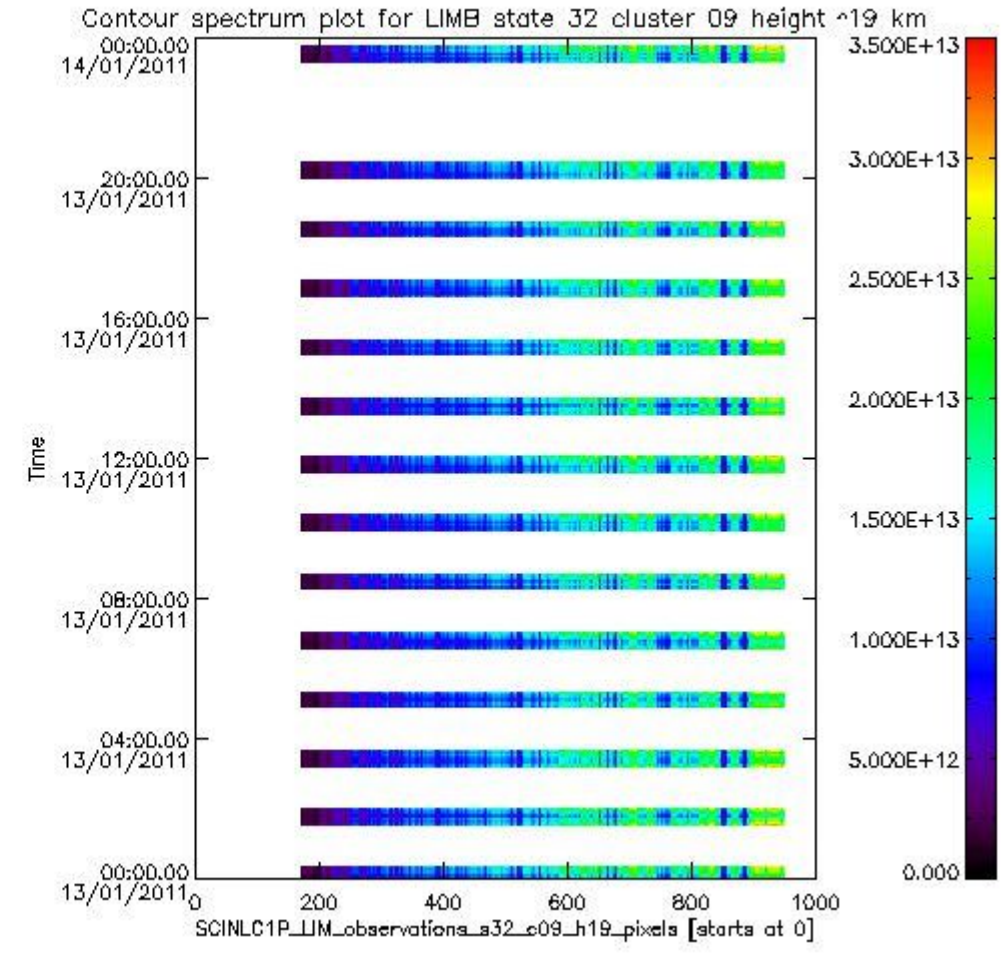
sciamachy_i1b_source_packet_report_SCIA_7_04_U_20110113_10.PNG
