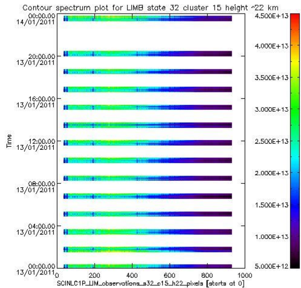
sciamachy_i1b_source_packet_report_SCIA_7_04_U_20110113_16.PNG
