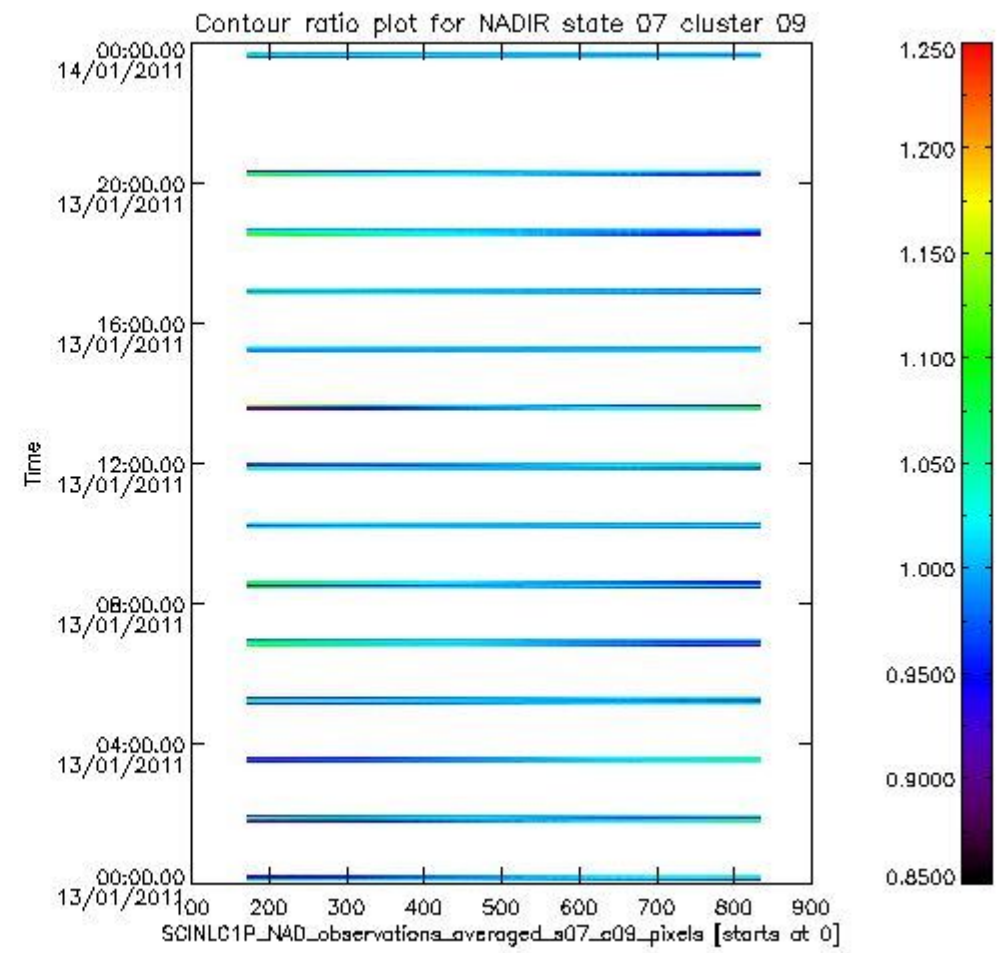
sciamachy_i1b_source_packet_report_SCIA_7_04_U_20110113_3.PNG
