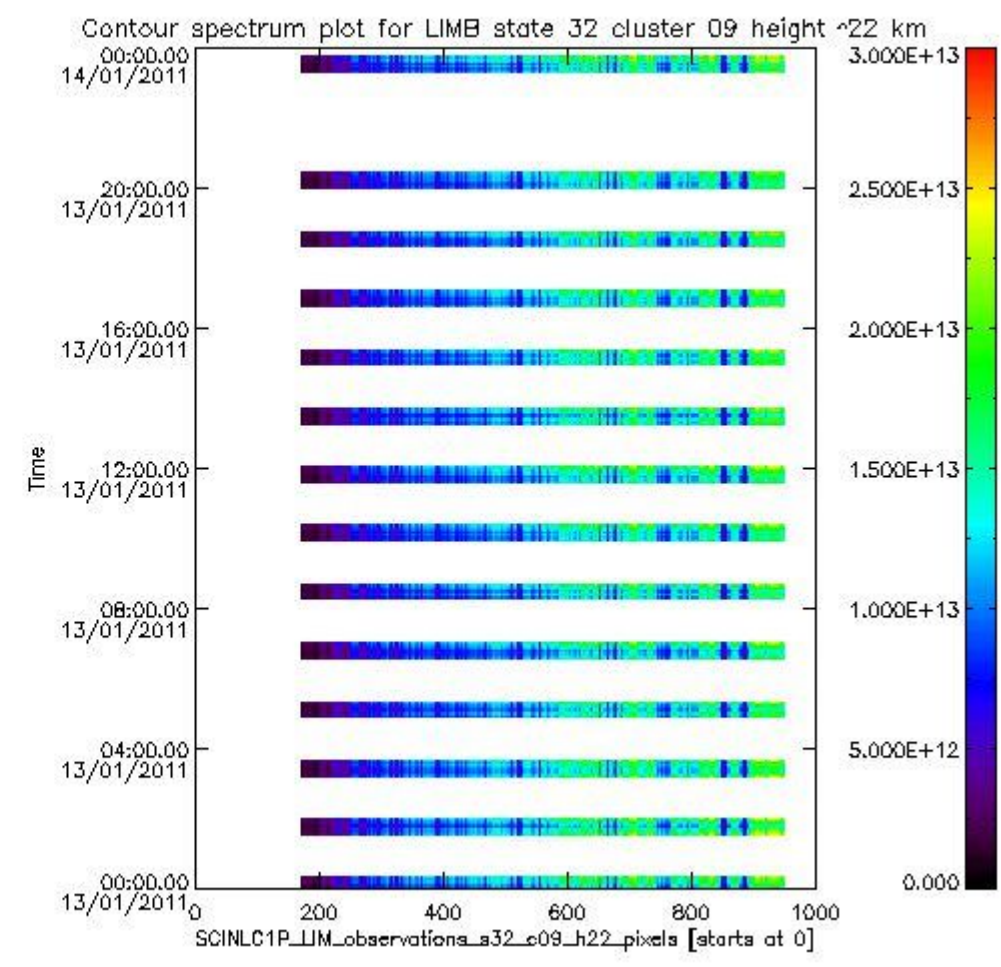
sciamachy_i1b_source_packet_report_SCIA_7_04_U_20110113_12.PNG
