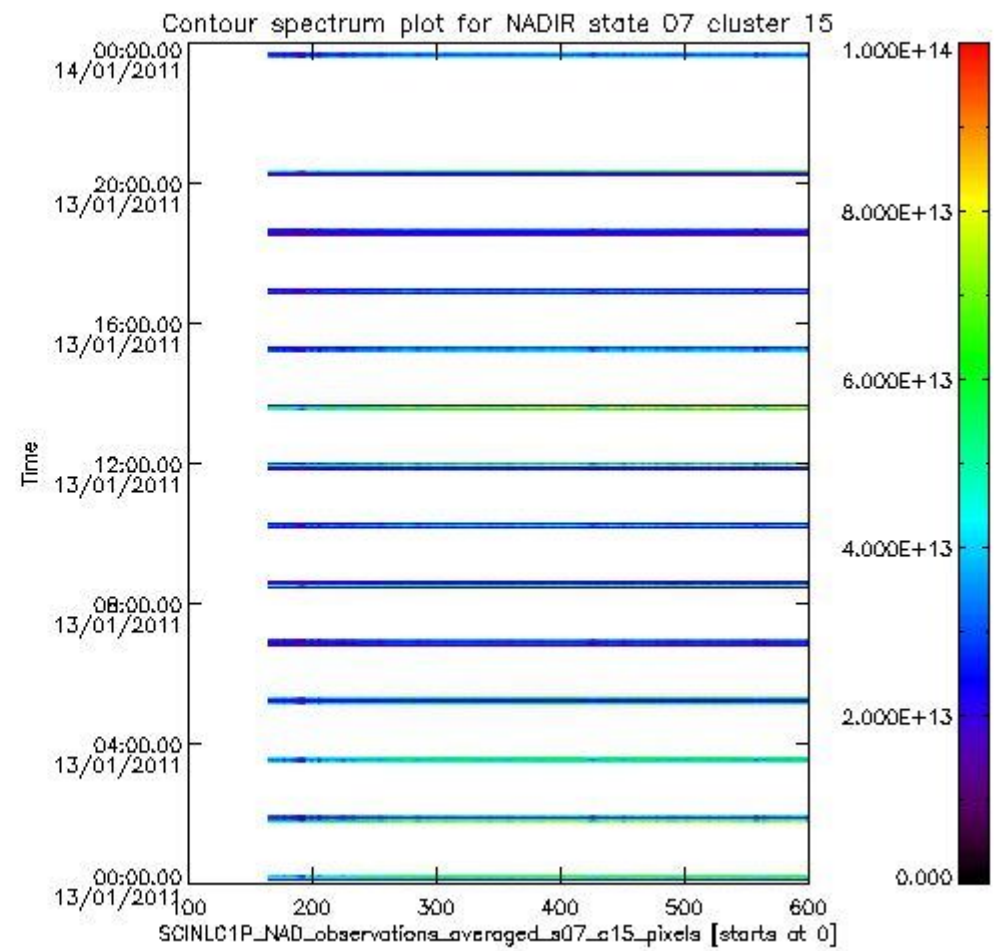
sciamachy_i1b_source_packet_report_SCIA_7_04_U_20110113_4.PNG
