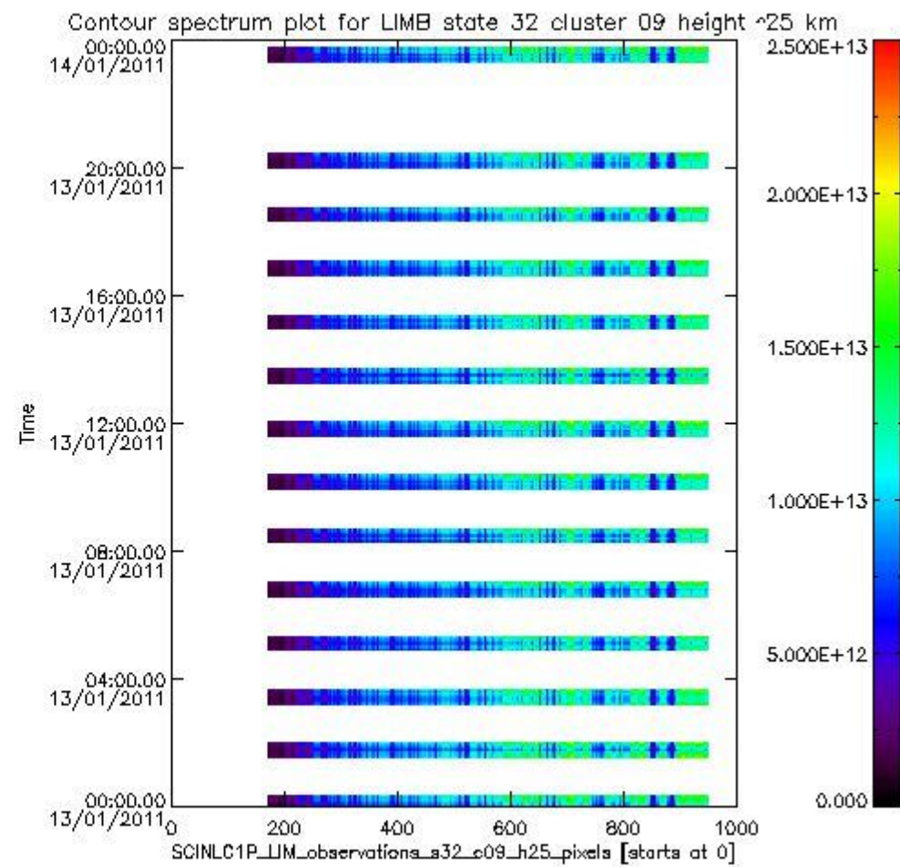
sciamachy_i1b_source_packet_report_SCIA_7_04_U_20110113_14.PNG
