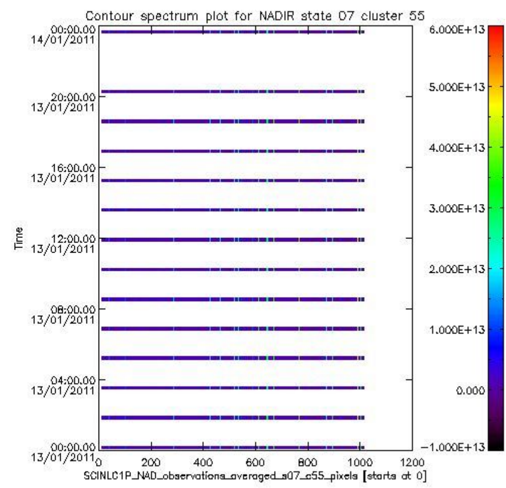
sciamachy_i1b_source_packet_report_SCIA_7_04_U_20110113_8.PNG
