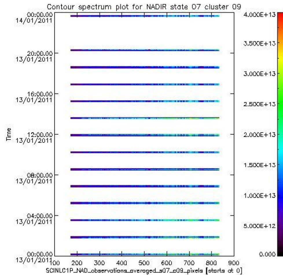
sciamachy_i1b_source_packet_report_SCIA_7_04_U_20110113_2.PNG
