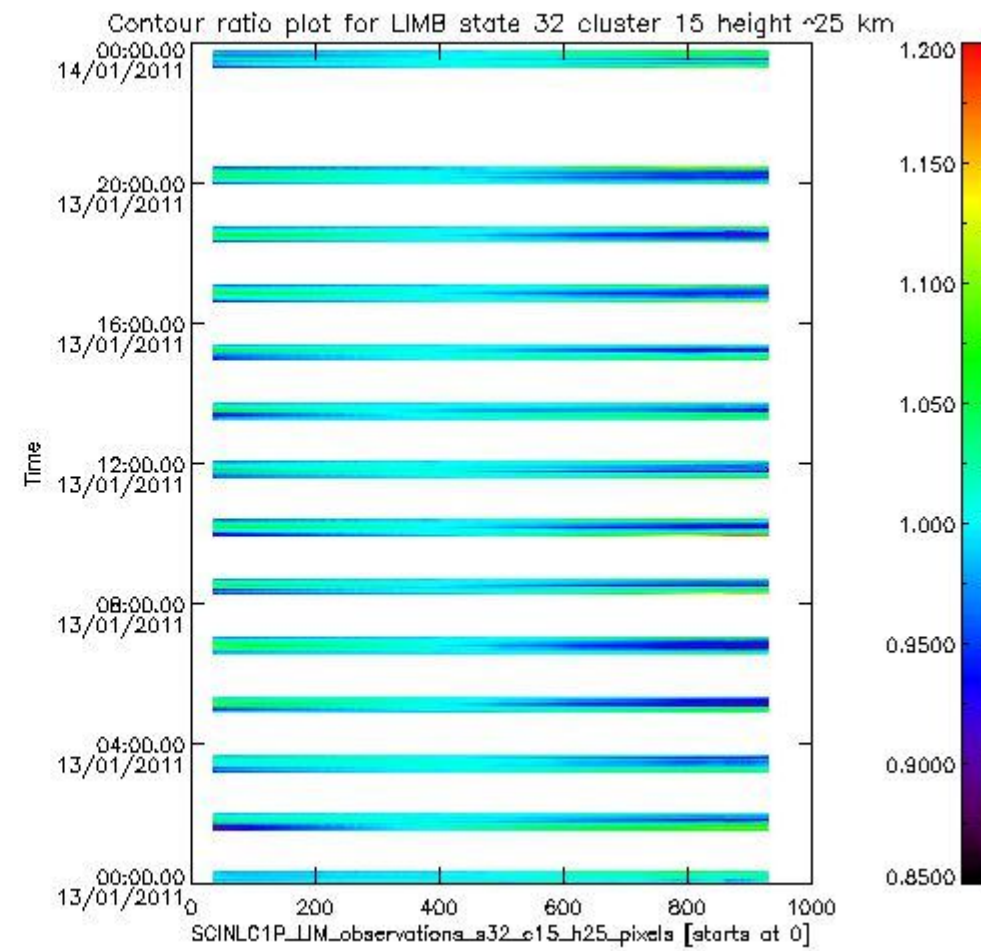
sciamachy_11b_source_packet_report_SCIA_7_04_U_20110113_19.PNG
