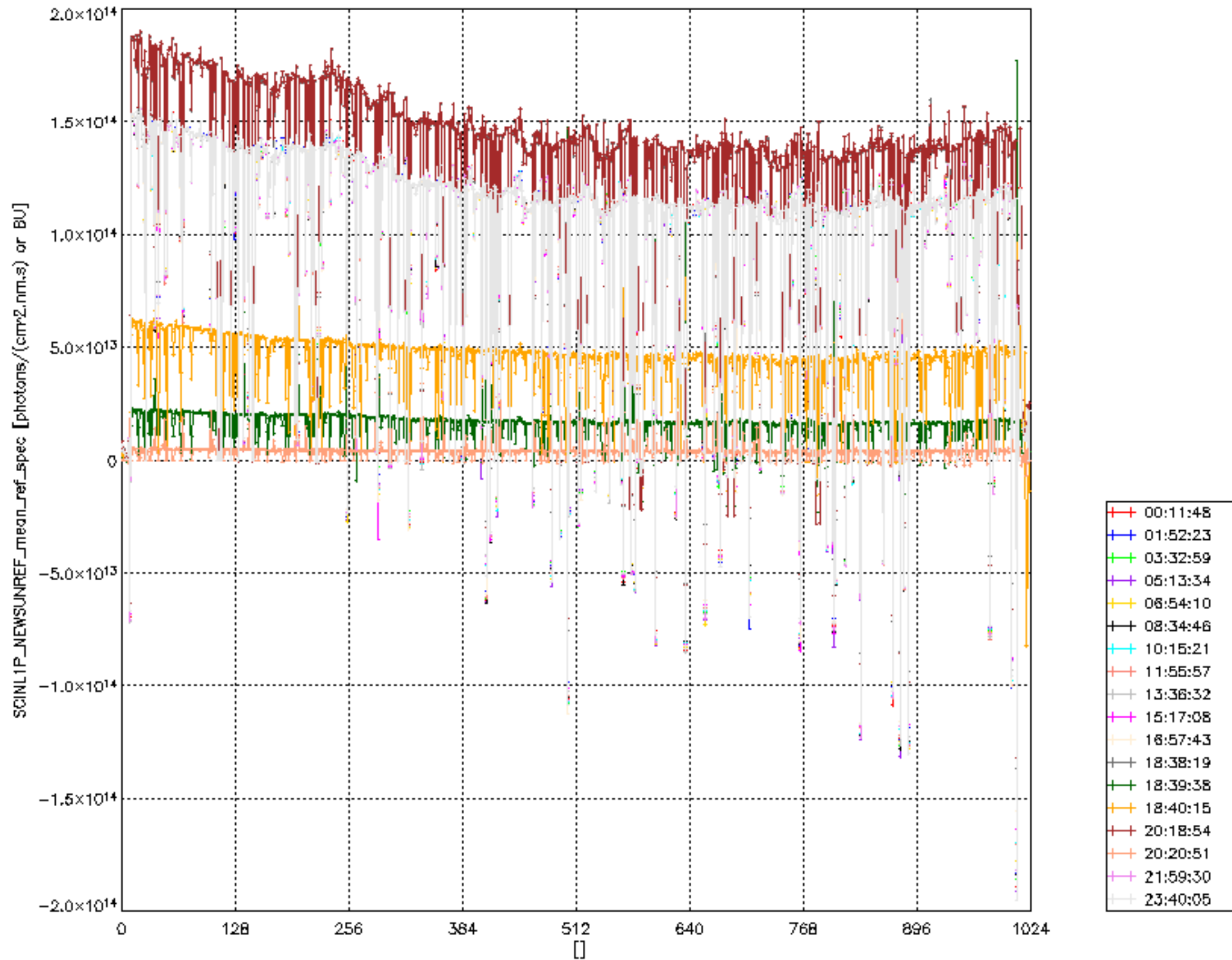
Plot of SCINL1P_NEWSUNREF_mean_ref_spec for detector B on 15APR2008 The colours indicate the time in hours since 15APR2008 00:00:00
