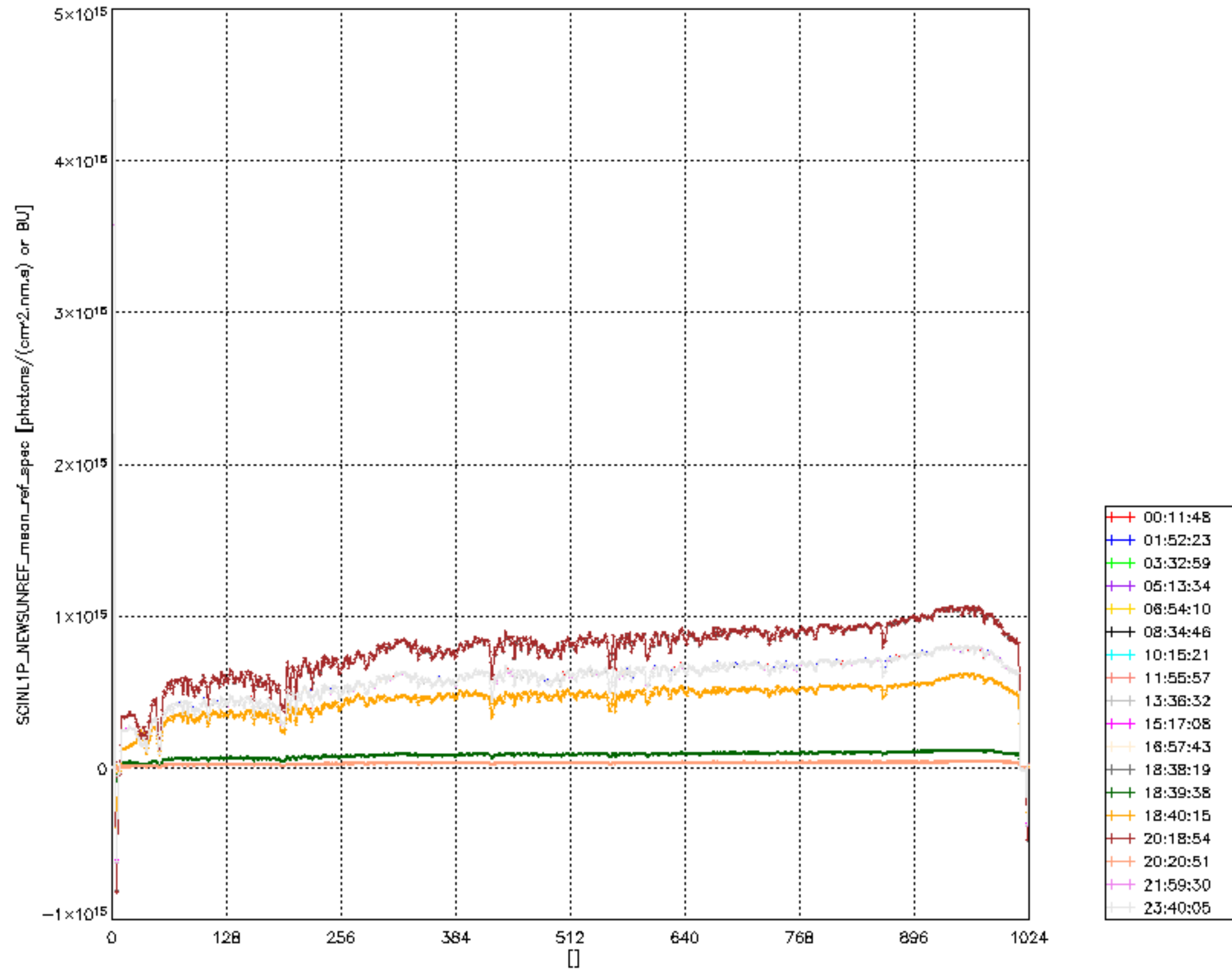
Plot of SCINL1P_NEWSUNREF_mean_ref_spec for detector 3 on 15APR2008 The colours indicate the time in hours since 15APR2008 00:00:00
