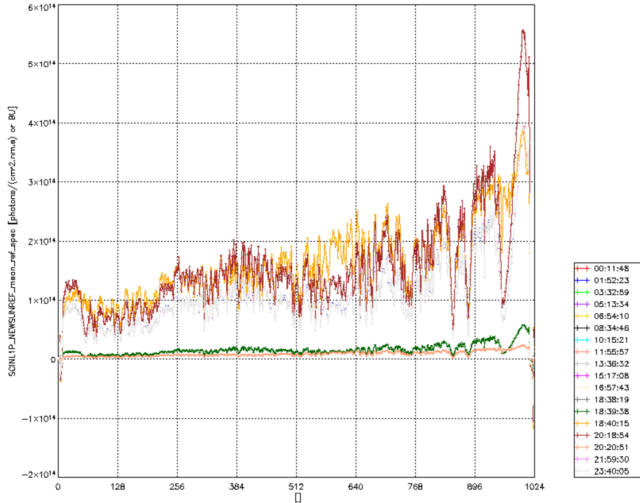
Plot of SCINL1P_NEWSUNREF_mean_ref_spec for detector 2 on 15APR2008 The colours indicate the time in hours since 15APR2008 00:00:00
