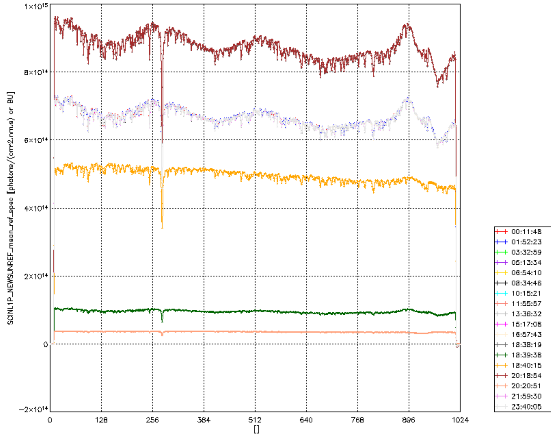
Plot of SCINL1P_NEWSUNREF_mean_ref_spec for detector 4 on 15APR2008 The colours indicate the time in hours since 15APR2008 00:00:00
