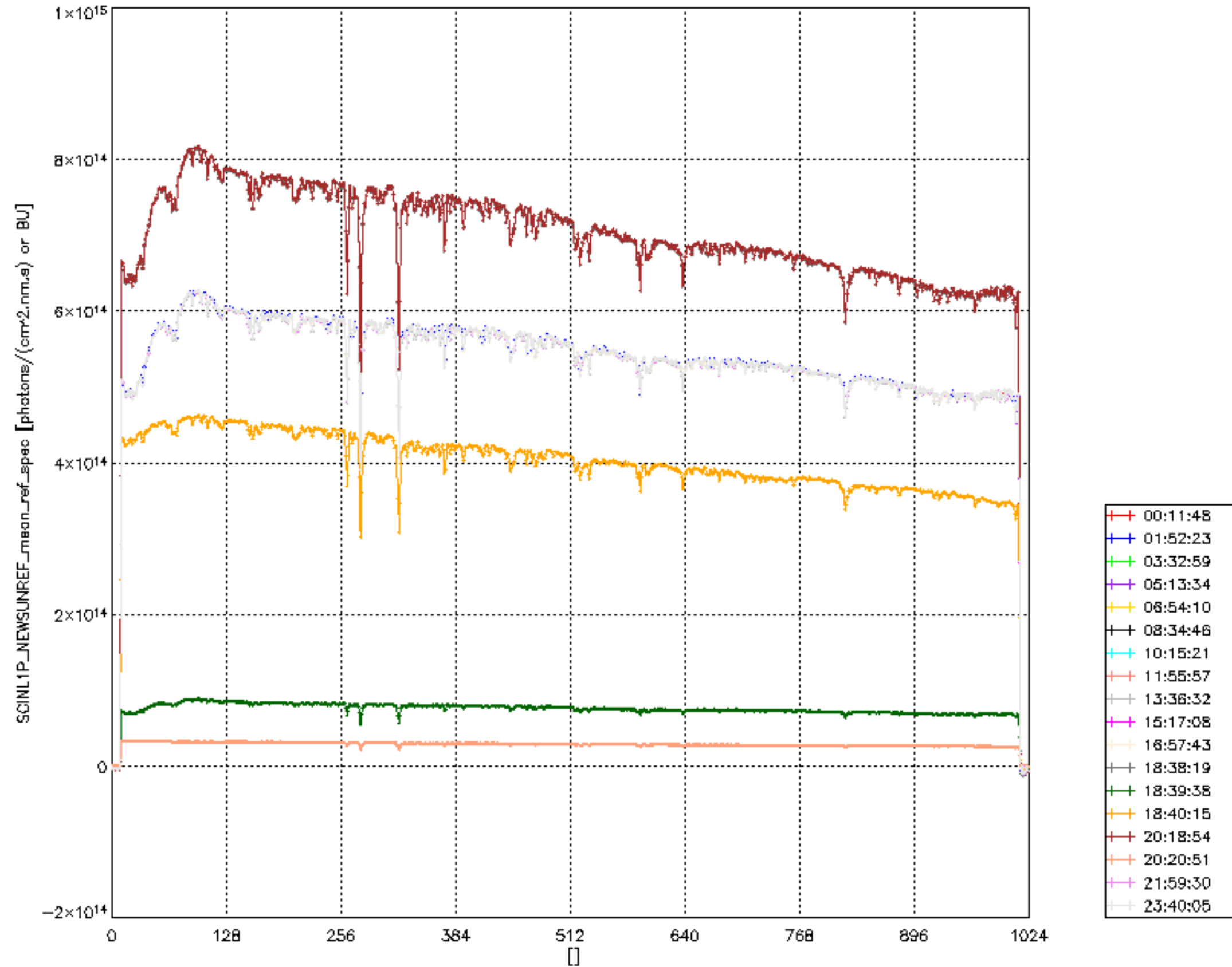
Plot of SCINL1P_NEWSUNREF_mean_ref_spec for detector 5 on 15APR2008 The colours indicate the time in hours since 15APR2008 00:00:00
