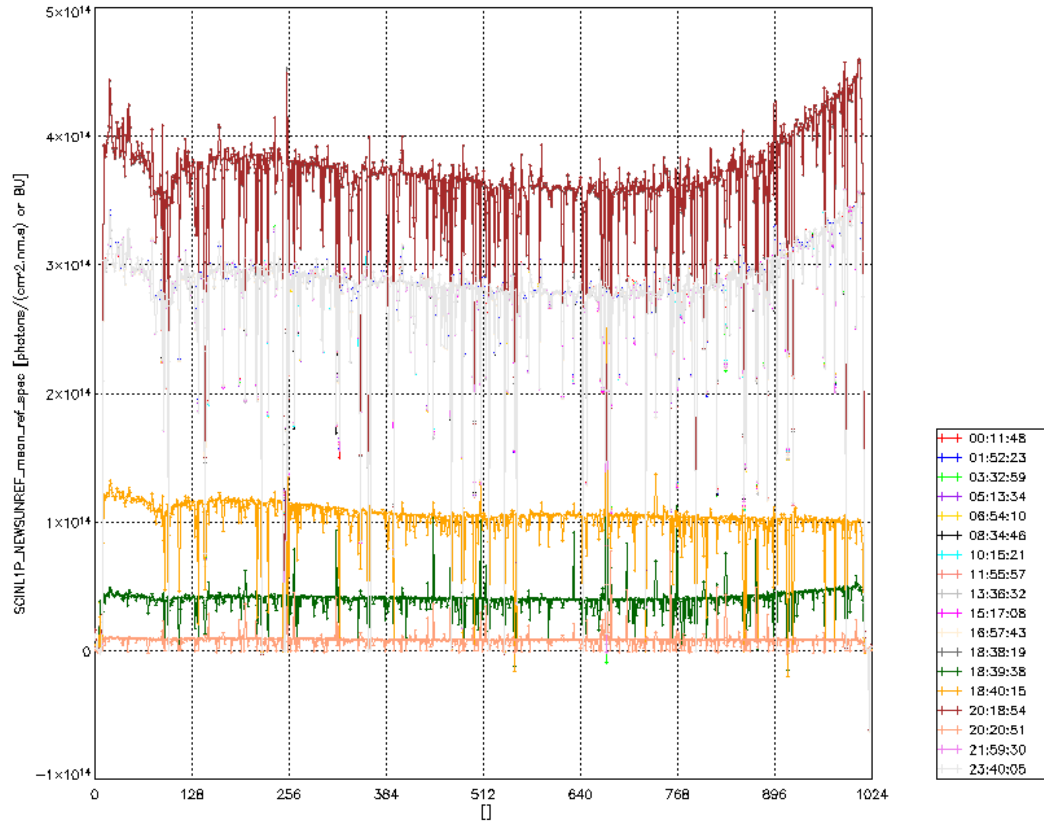
Plot of SCINL1P_NEWSUNREF_mean_ref_spec for detector 7 on 15APR2008 The colours indicate the time in hours since 15APR2008 00:00:00
