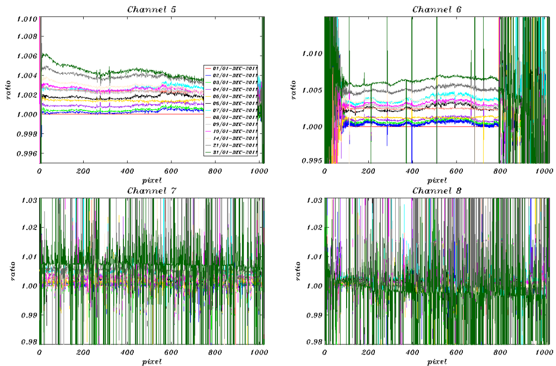
Figure 6.5: SMR ratios per detector channel 5-8 (changes during December 2011).
