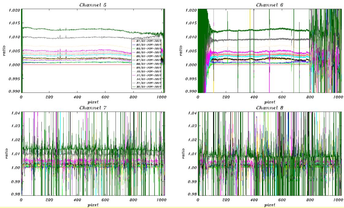
Figure 6.3: SMR ratios per detector channel 5-8 (changes during November 2011).
