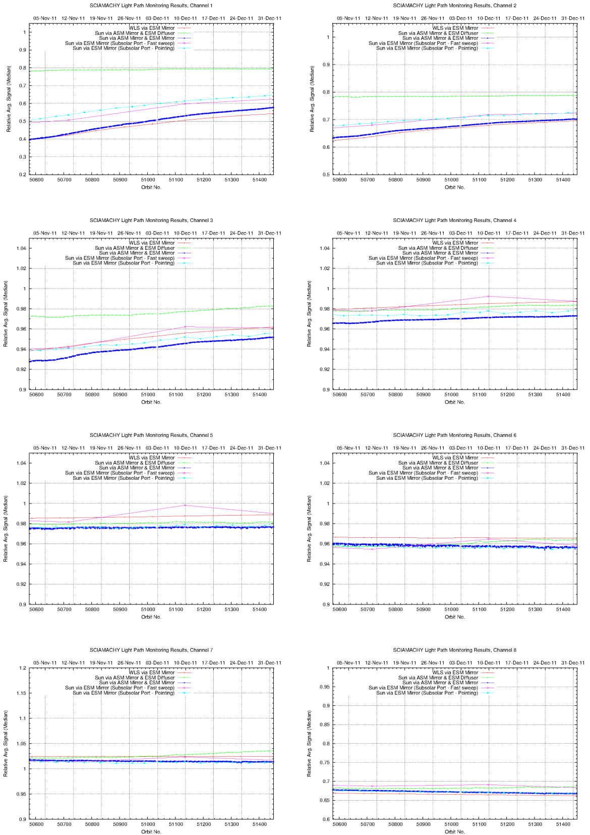
Figure 3.7: Light path monitoring results November to December 2011 (medians).
