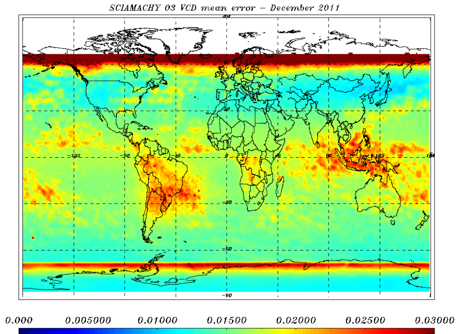
Figure 8.8: O 3 VCD error for 01- 31 December 2011 - monthly average.
