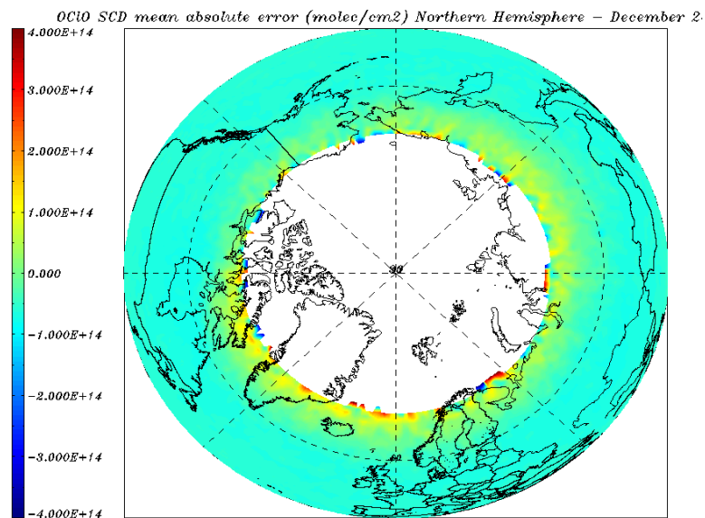
Figure 8.30: OCIO SCD error (molec/cm 2 ) for 01 – 31 December 2011- monthly average over the Northern Hemisphere.
