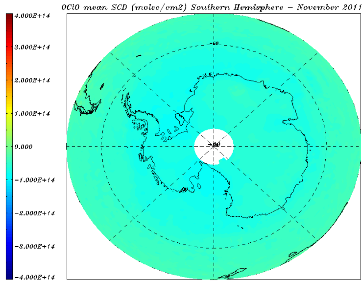
Figure 8.27: OCIO SCD (molec/cm 2 ) for 01 – 30 November 2011 – monthly average over the Southern Hemisphere.
