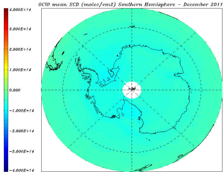
Figure 8.31: OCIO SCD (molec/cm 2 ) for 01 – 31 December 2011 – monthly average over the Southern Hemisphere.
