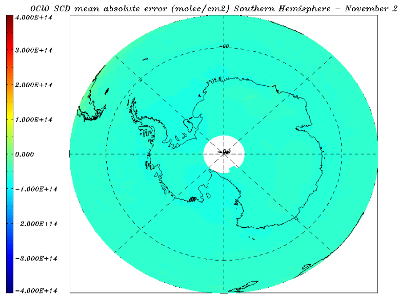
Figure 8.28: OCIO SCD error (molec/cm 2 ) for 01 – 30 November 2011- monthly average over the Southern Hemisphere.
