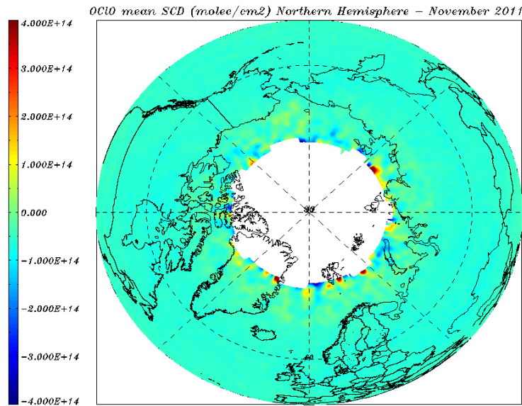
Figure 8.25: OCIO SCD (molec/cm 2 ) for 01 – 30 November 2011 – monthly average over the Northern Hemisphere.
