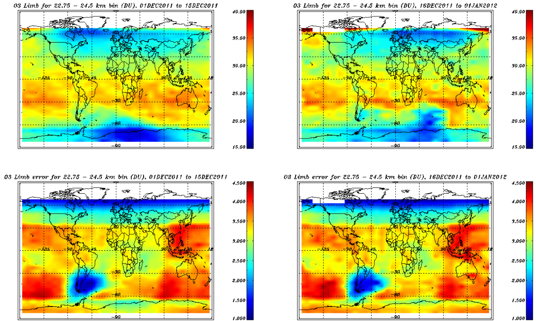
Figure 8.35: Limb Ozone profiles binned over 22.75 – 24.5 km, December 2011.
