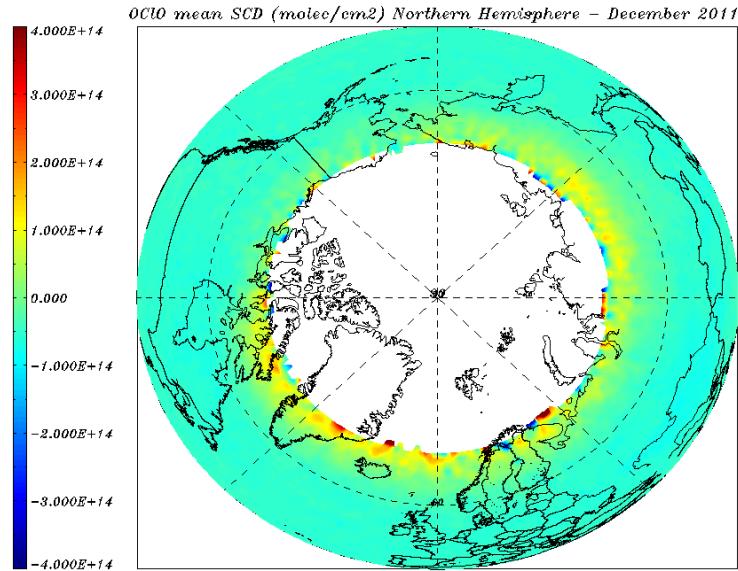
Figure 8.29: OCIO SCD (molec/cm 2 ) for 01 – 31 December 2011 – monthly average over the Northern Hemisphere.
