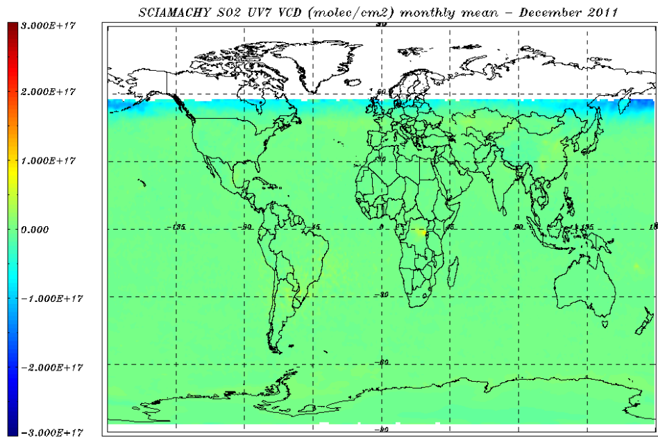
Figure 8.23: SO 2 VCD (molec/cm 2 ) world map for 01 – 31 December 2011 – monthly average.
