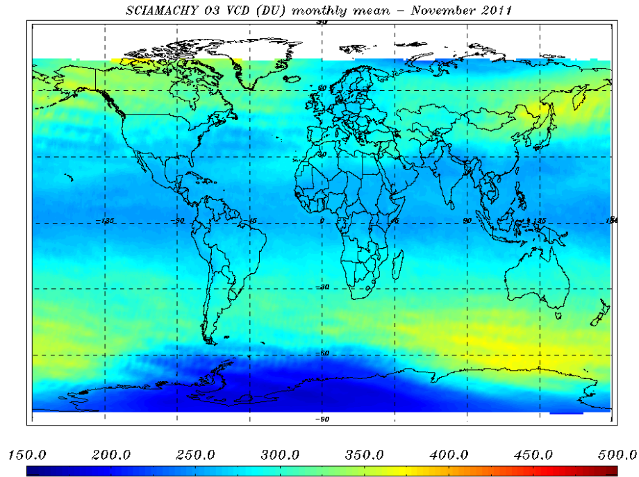
Figure 8.5: O 3 VCD (DU) world map for 01 - 30 November 2011 – monthly average.
