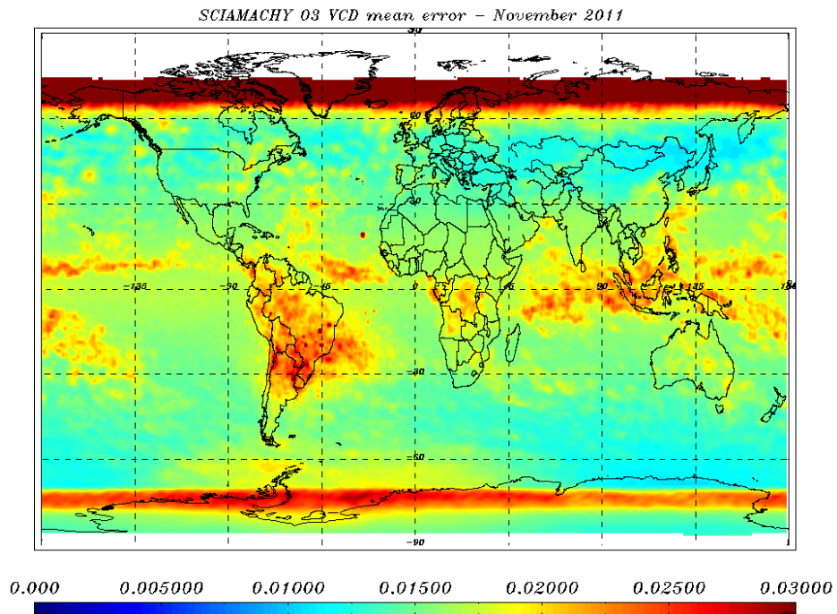
Figure 8.6: O 3 VCD error for 01 - 30 November 2011 - monthly average.
