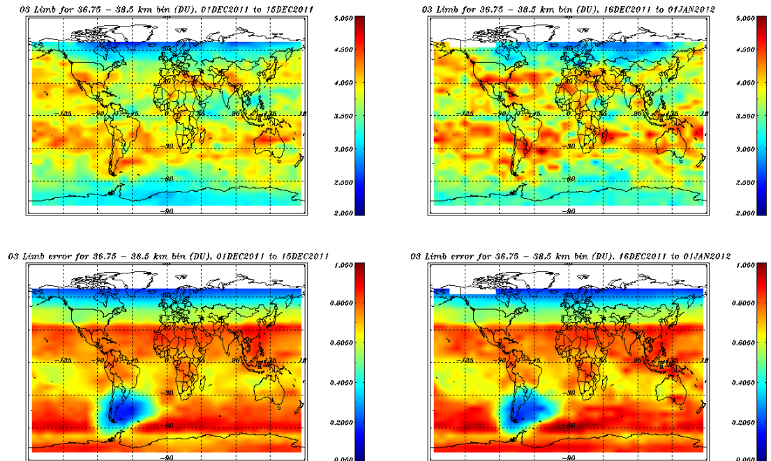
Figure 8.36: Limb Ozone profiles binned over 36.75 – 38.5 km, December 2011.
