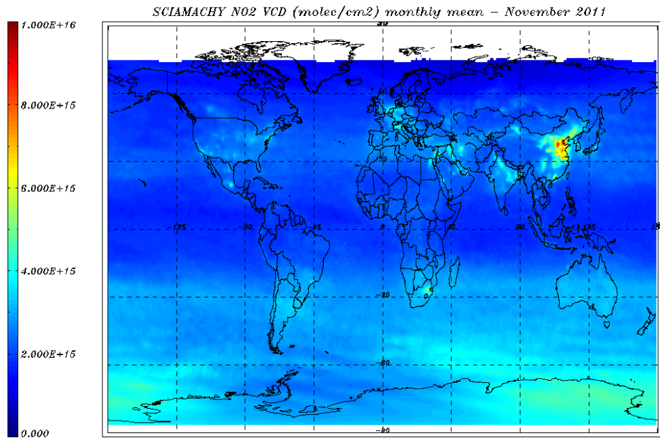
Figure 8.1: NO 2 VCD (molec/cm 2 ) world map for 01 - 30 November 2011 – monthly average.
