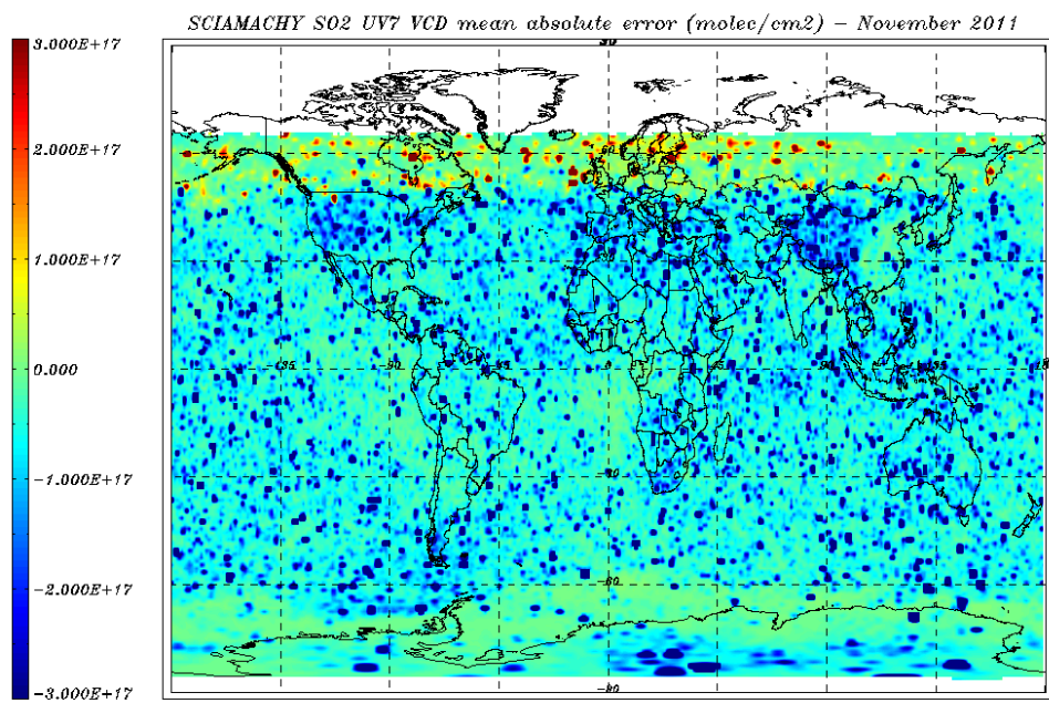
Figure 8.22: SO 2 VCD error (molec/cm 2 ) for 01 – 30 November 2011 – monthly average.
