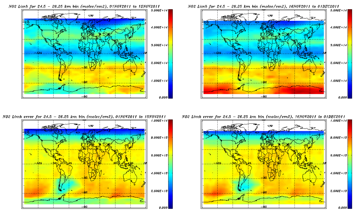
Figure 8.37: Limb NO 2 profiles binned over 24.5 – 26.25 km, November 2011.
