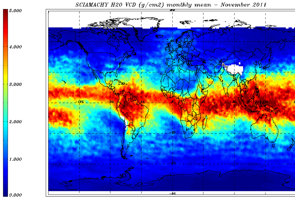
Figure 8.9: H 2 O VCD (g/cm 2 ) world map for 01 - 30 November 2011 – monthly average.
