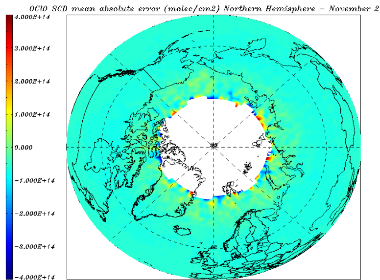
Figure 8.26: OCIO SCD error (molec/cm 2 ) for 01 – 30 November 2011- monthly average over the Northern Hemisphere.
