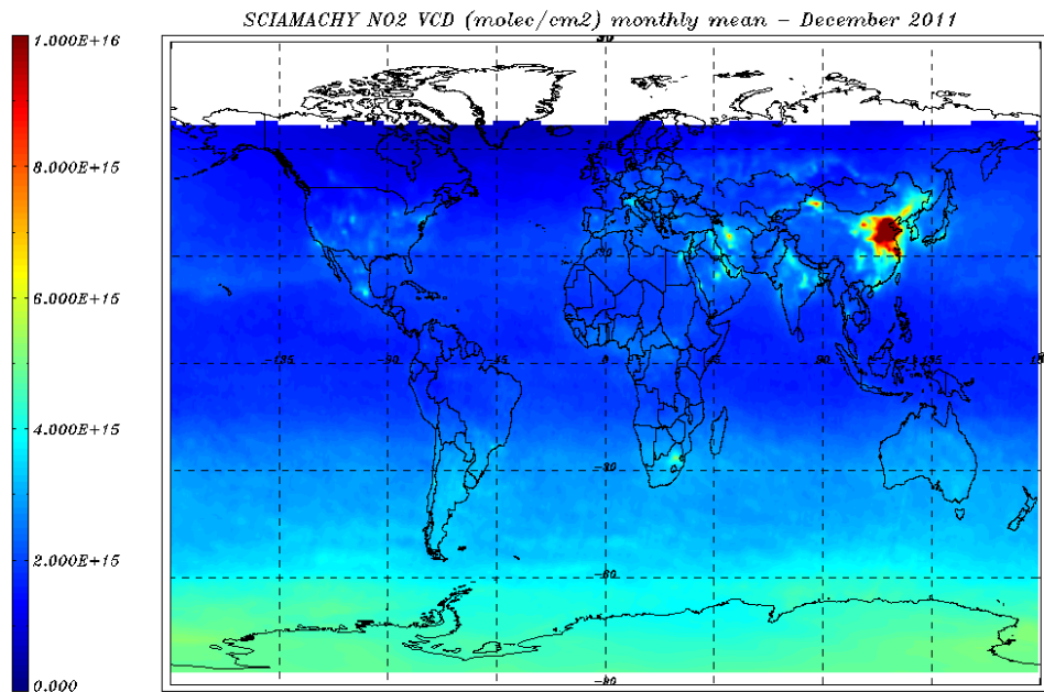
Figure 8.3: NO 2 VCD (molec/cm 2 ) world map for 01 – 31 December 2011 – monthly average.
