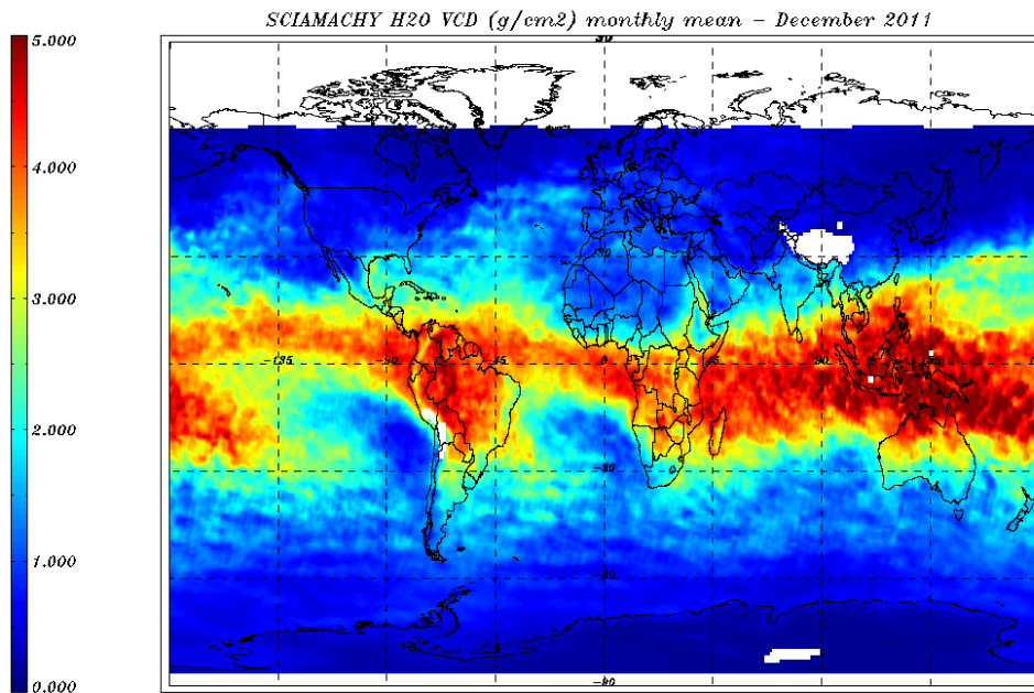
Figure 8.11: H 2 O VCD (g/cm 2 ) world map for 01 – 31 December 2011 – monthly average.
