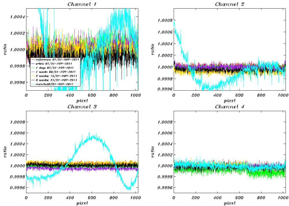
Figure 6.8: Dark current ratios (constant part) channels 1-4 during November 2011.
