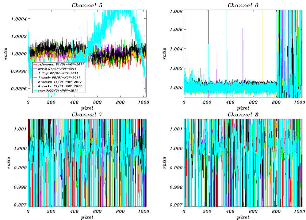
Figure 6.9: Dark current ratios (constant part) channels 5-8 during November 2011.
