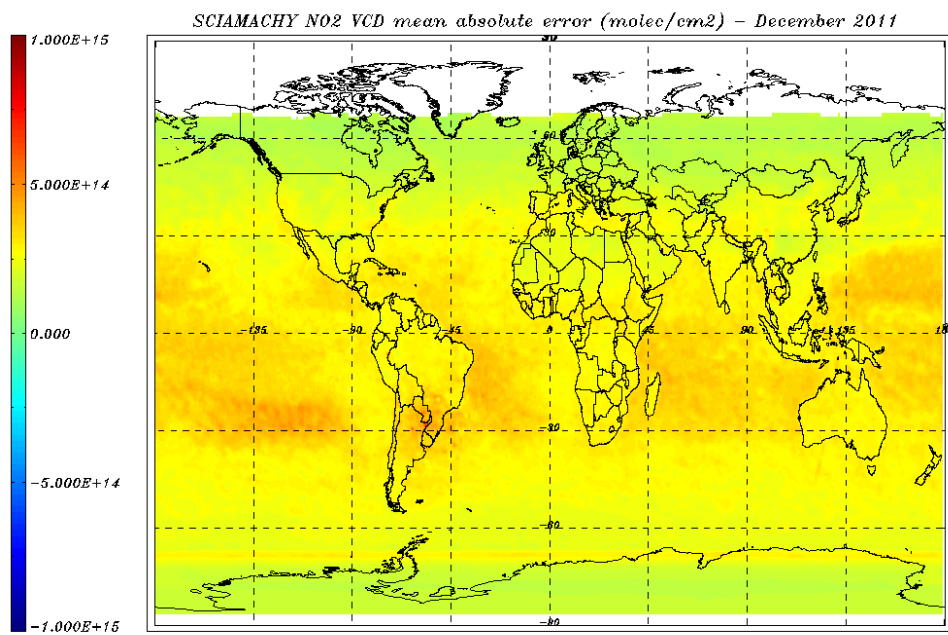
Figure 8.4: NO 2 VCD error (molec/cm 2 ) for 01 – 31 December 2011- monthly average.
