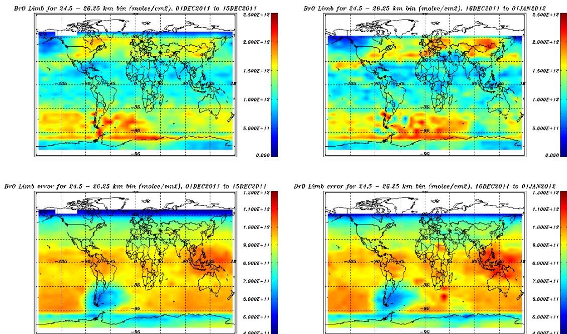
Figure 8.40: Limb BrO profiles binned over 24.5 – 26.25 km, December 2011.
