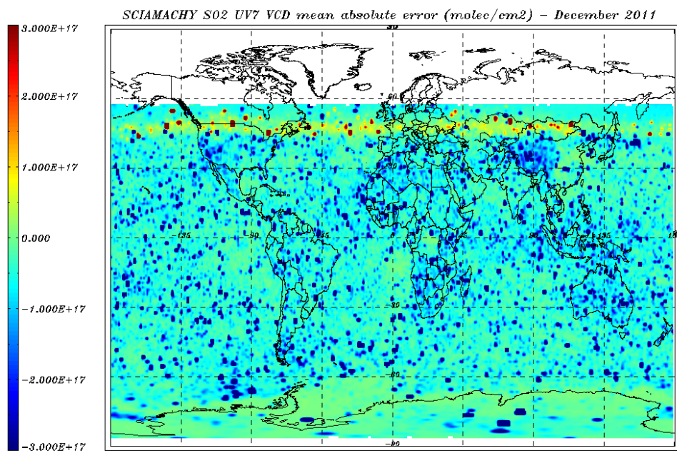
Figure 8.24: SO 2 VCD error (molec/cm 2 ) for 01 – 31 December 2011 – monthly average.
