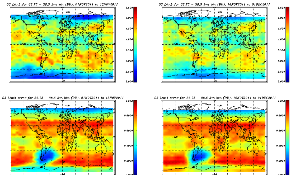
Figure 8.34: Limb Ozone profiles, binned over 36.75 – 38.5 km, November 2011.
