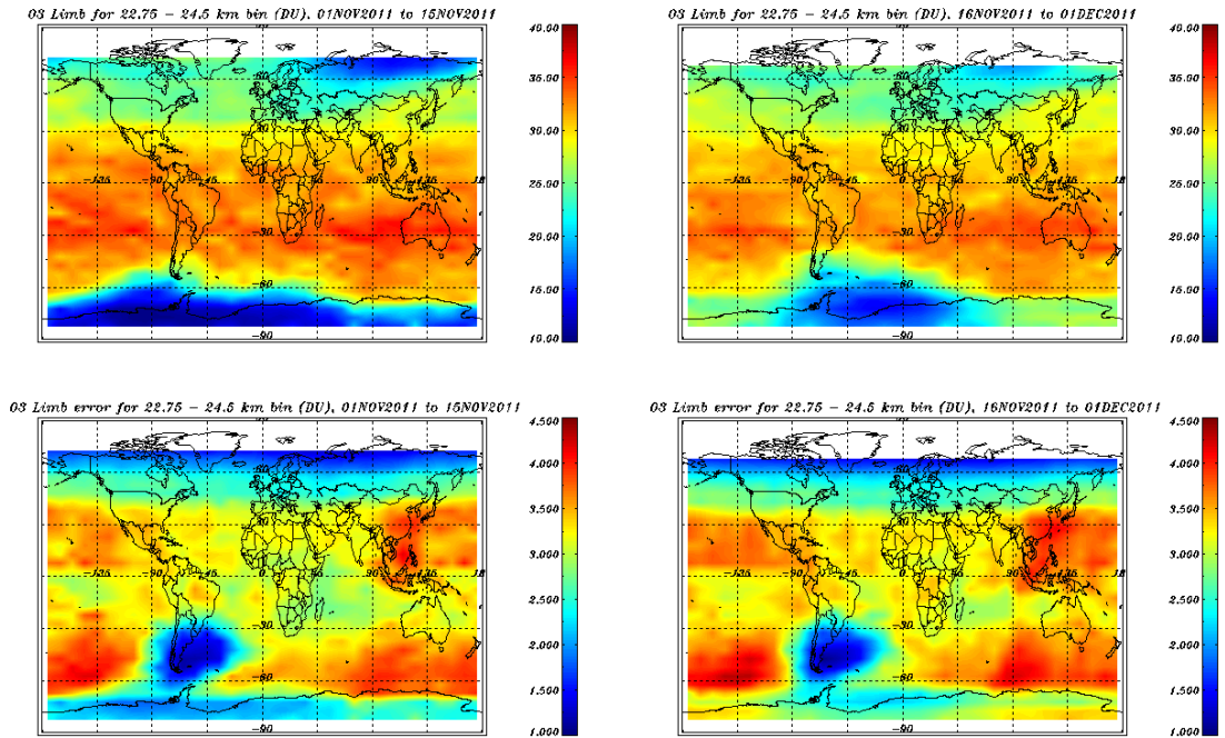
Figure 8.33: Limb Ozone profiles, binned over 22.75 – 24.5 km, November 2011.
