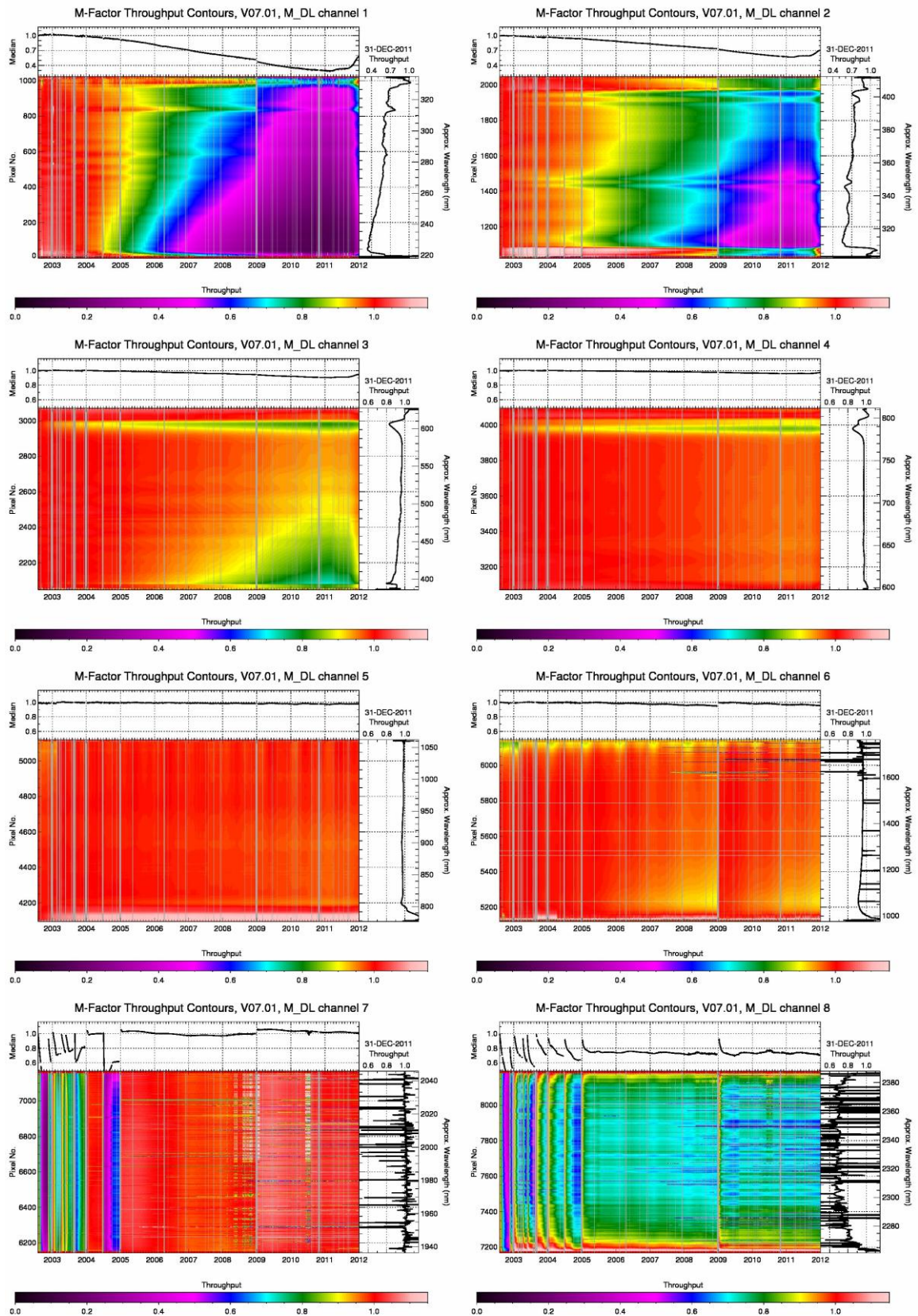
Figure 4.2: Degradation derived from m-factors August 2002 to December 2011 (limb light path).
