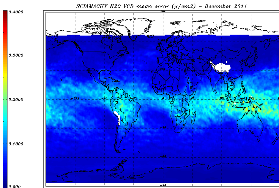
Figure 8.12: H 2 O VCD (g/cm 2 ) error for 01 – 31 December 2011- monthly average.
