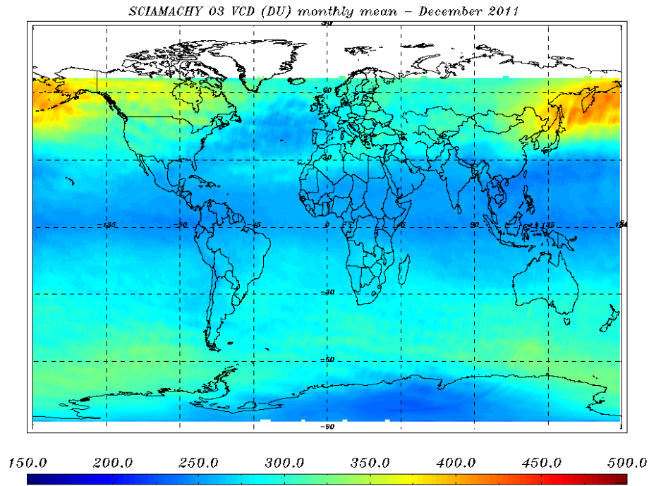
Figure 8.7: O 3 VCD (DU) world map for 01 - 31 December 2011 – monthly average.
