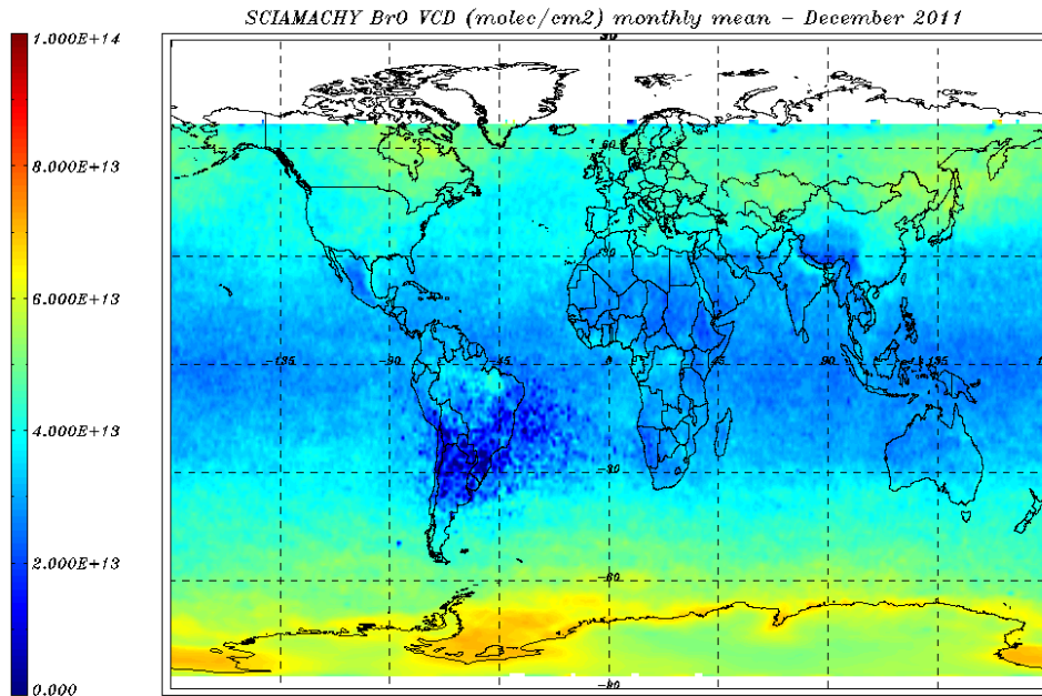
Figure 8.15: BrO VCD (molec/cm 2 ) world map for 01 – 31 December 2011 – monthly average.
