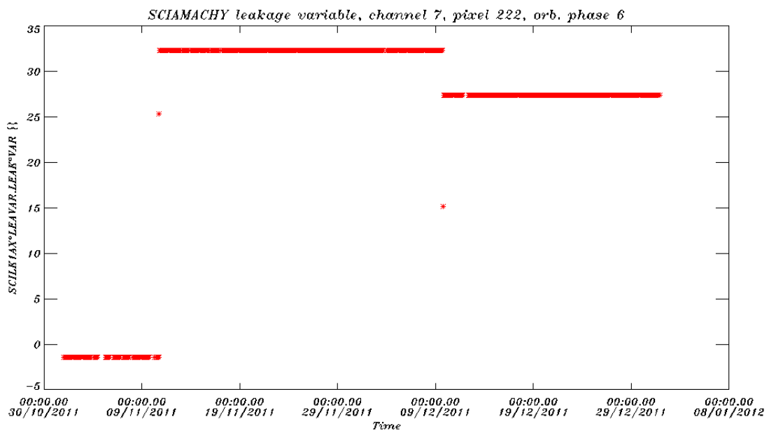
Figure 6.12: Leakage variable part from 01 November 2011 to 31 December 2011, for channel 7, orbit phase 6, pixel 222.
