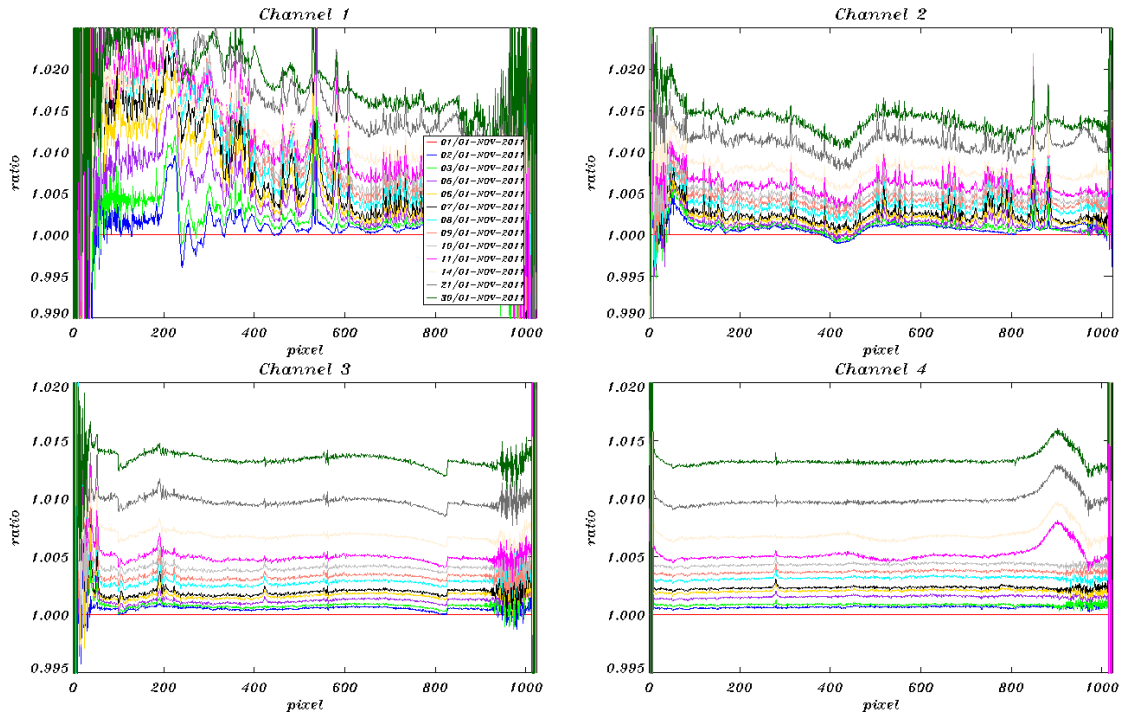
Figure 6.2: SMR ratios per detector channel 1-4 (changes during November 2011).
