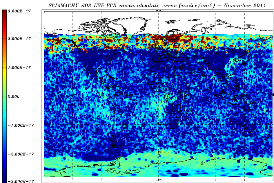
Figure 8.18: SO 2 VCD error (molec/cm 2 ) for 01 –30 November 2011- monthly average.
