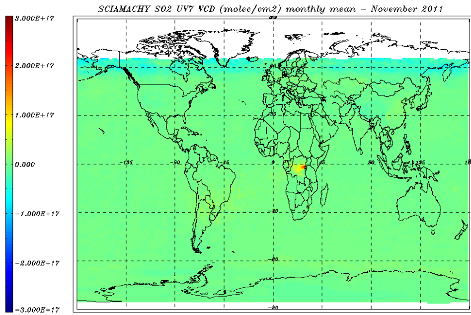
Figure 8.21: SO 2 VCD (molec/cm 2 ) world map for 01 –30 November 2011 – monthly average.
