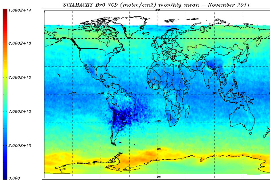
Figure 8.13: BrO VCD (molec/cm 2 ) world map for 01 – 30 November 2011 – monthly average.
