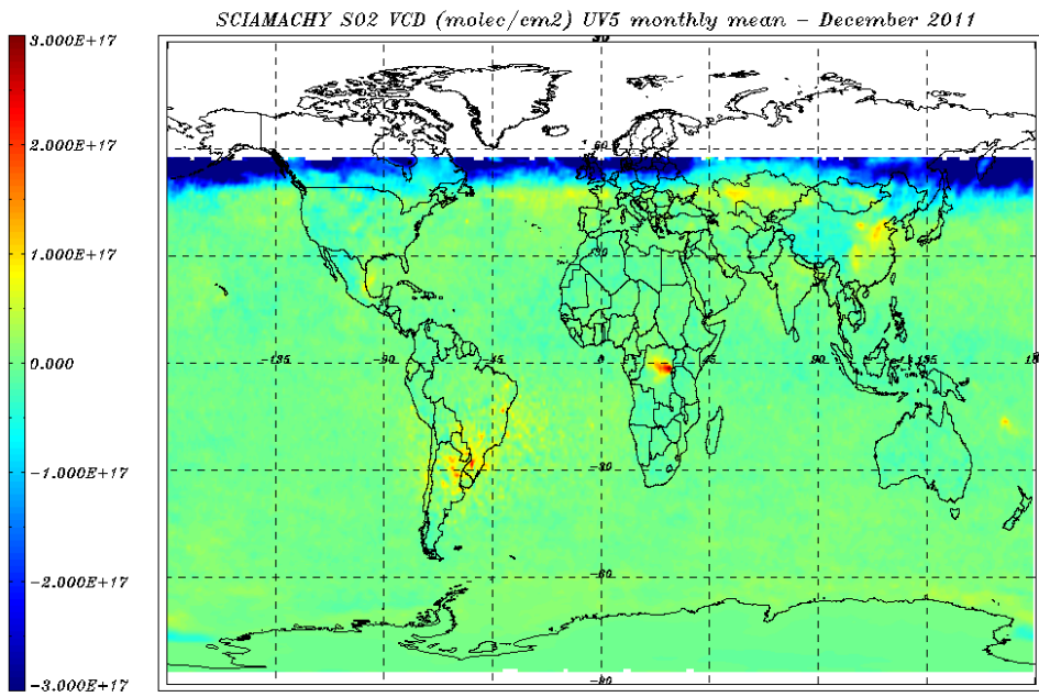
Figure 8.19: SO 2 VCD (molec/cm 2 ) world map for 01 – 31 December 2011 – monthly average.
