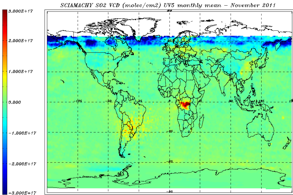
Figure 8.17: SO 2 VCD (molec/cm 2 ) world map for 01 –30 November 2011 – monthly average.
