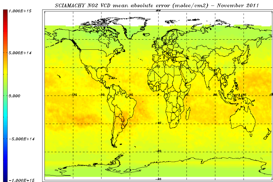
Figure 8.2: NO 2 VCD error (molec/cm 2 ) for 01 - 30 November 2011 - monthly average.
