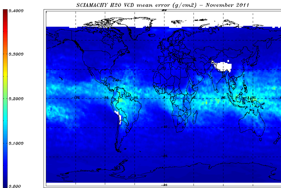
Figure 8.10: H 2 O VCD (g/cm 2 ) error for 01 - 30 November 2011 - monthly average.
