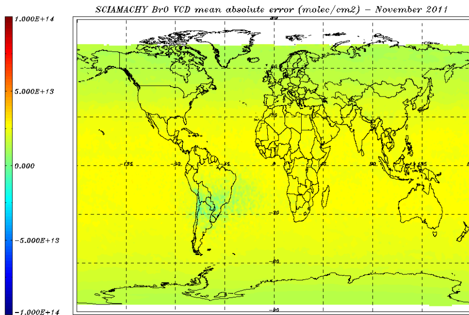
Figure 8.14: BrO VCD error (molec/cm 2 ) for 01 – 30 November 2011- monthly average.
