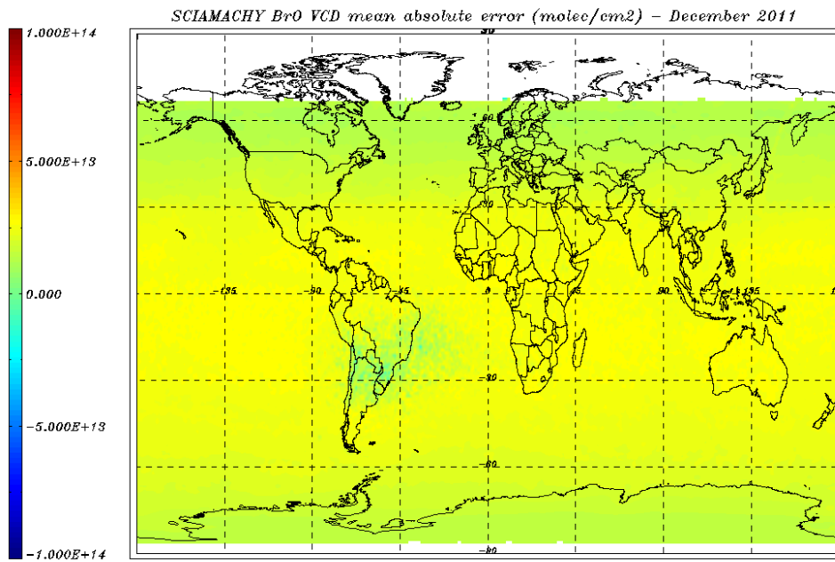
Figure 8.16: BrO VCD error (molec/cm 2 ) for 01 – 31 December 2011- monthly average.
