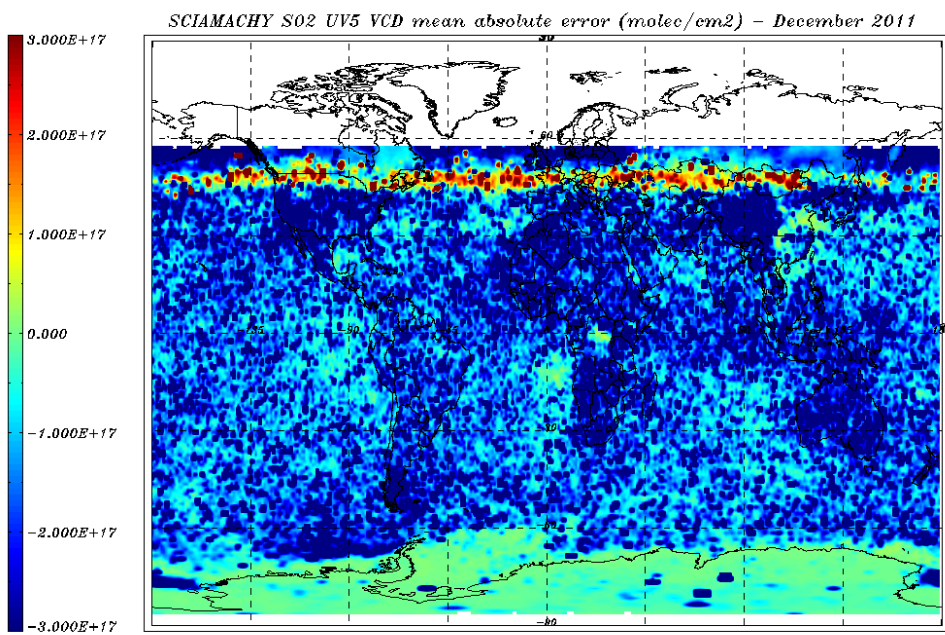
Figure 8.20: SO 2 VCD error (molec/cm 2 ) for 01 – 31 December 2011- monthly average.
