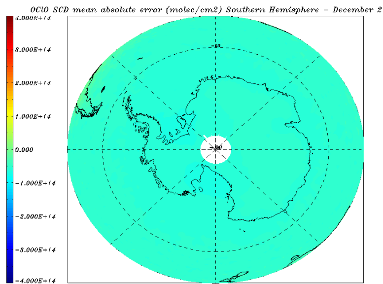
Figure 8.32: OCIO SCD error (molec/cm 2 ) for 01 – 31 December 2011- monthly average over the Southern Hemisphere.
