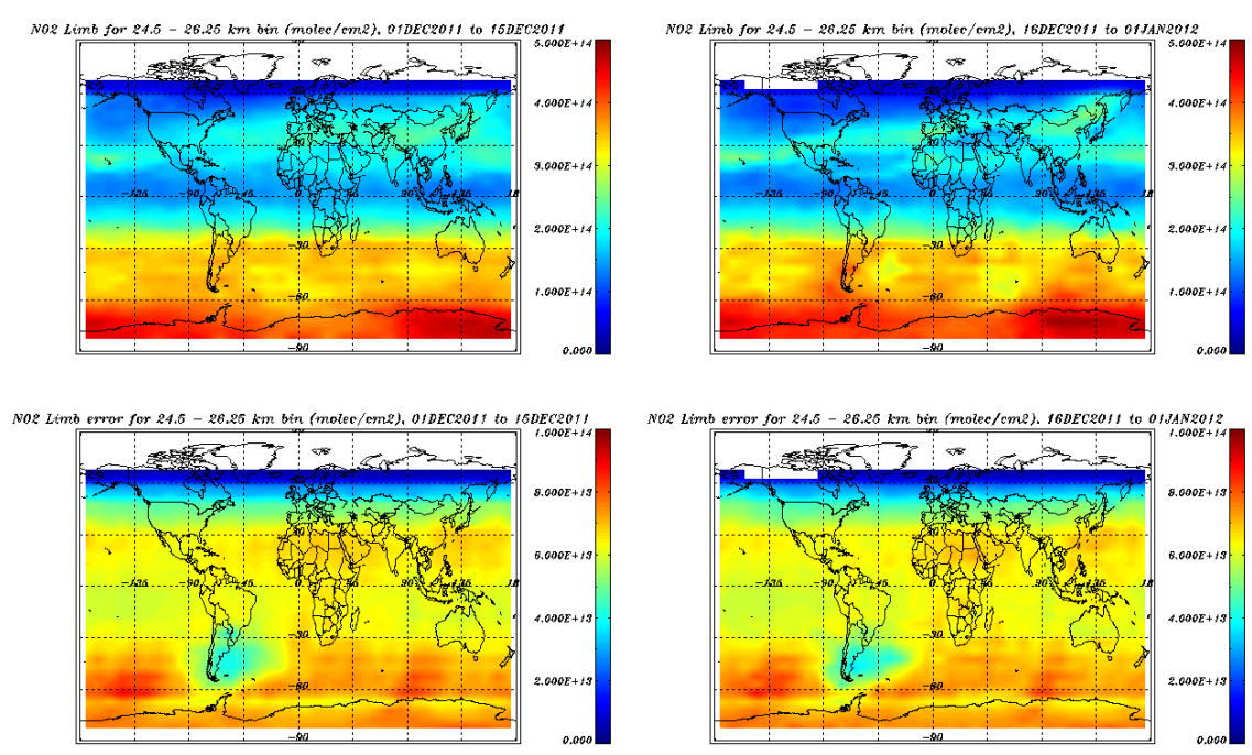
Figure 8.38: Limb NO 2 profiles binned over 24.5 – 26.25 km, December 2011.
