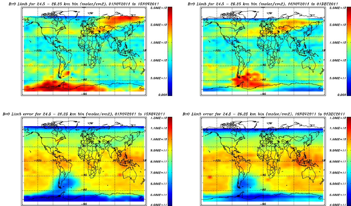
Figure 8.39: Limb BrO profiles binned over 24.5 – 26.25 km, November 2011.
