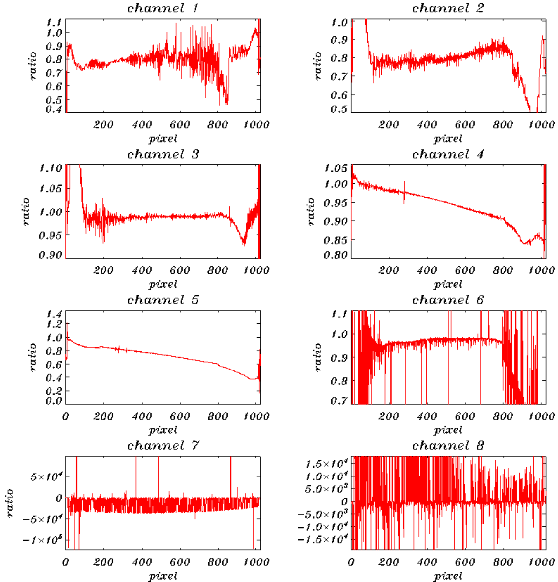
Figure 6.7: SMR ratios per detector channel on Long Term Trend 31/12/2011 divided by 31/12/2003.
