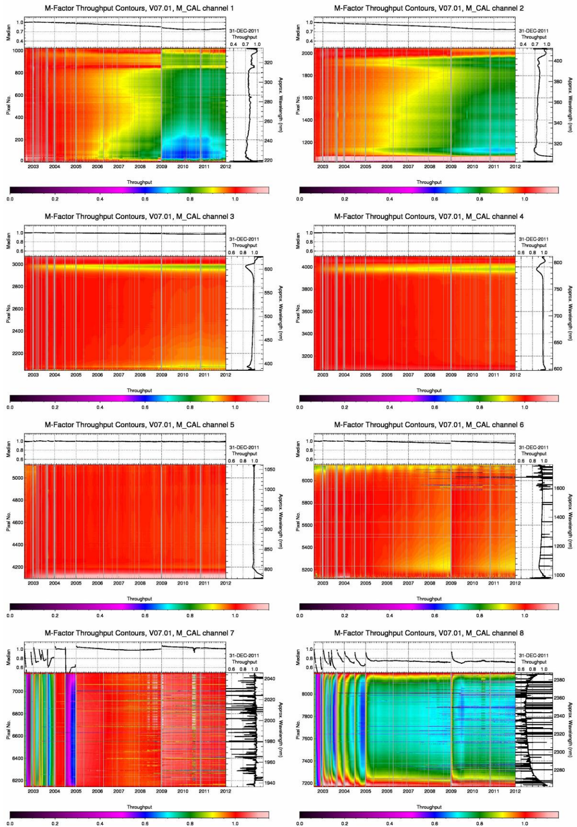
Figure 4.3: Degradation derived from m-factors August 2002 to December 2011 (calibr. light path).
