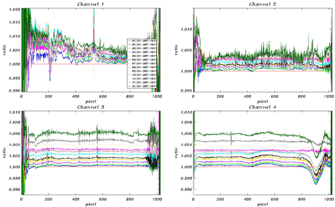
Figure 6.4: SMR ratios per detector channel 1-4 (changes during December 2011).
