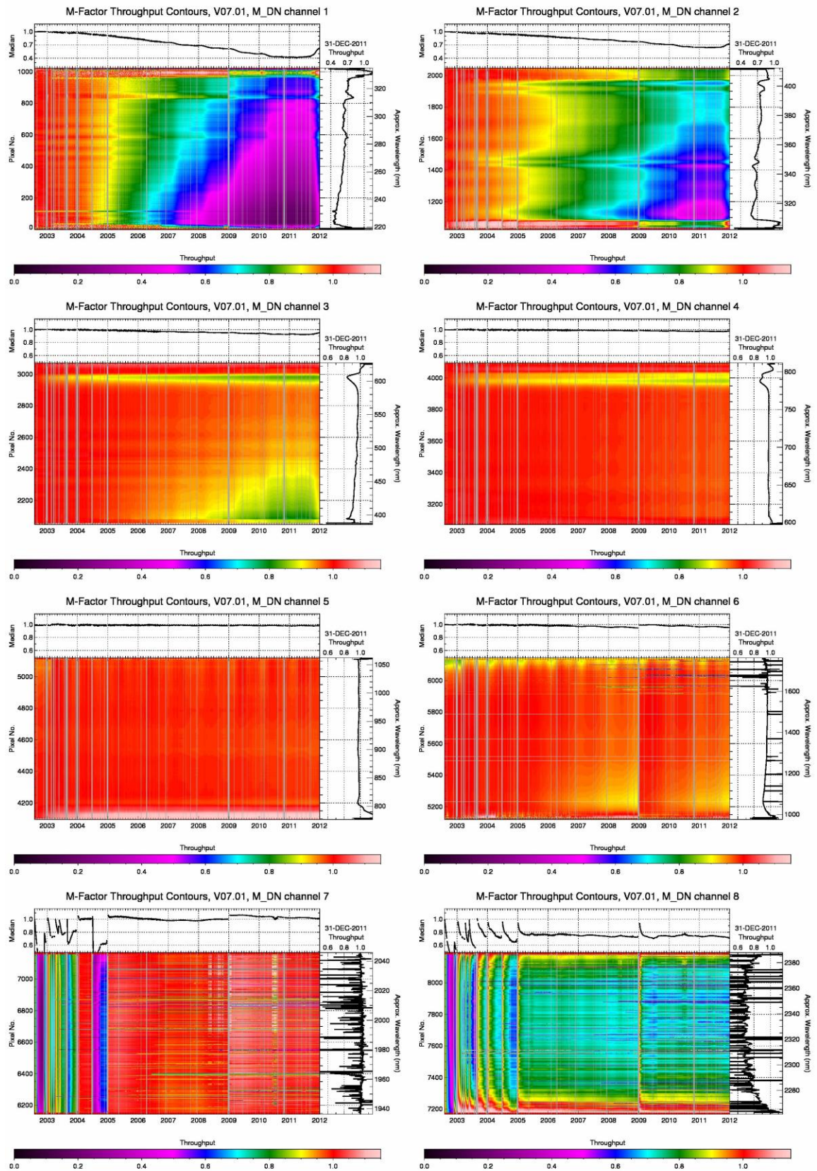
Figure 4.1: Degradation derived from m-factors August 2002 to December 2011 (nadir light path).
