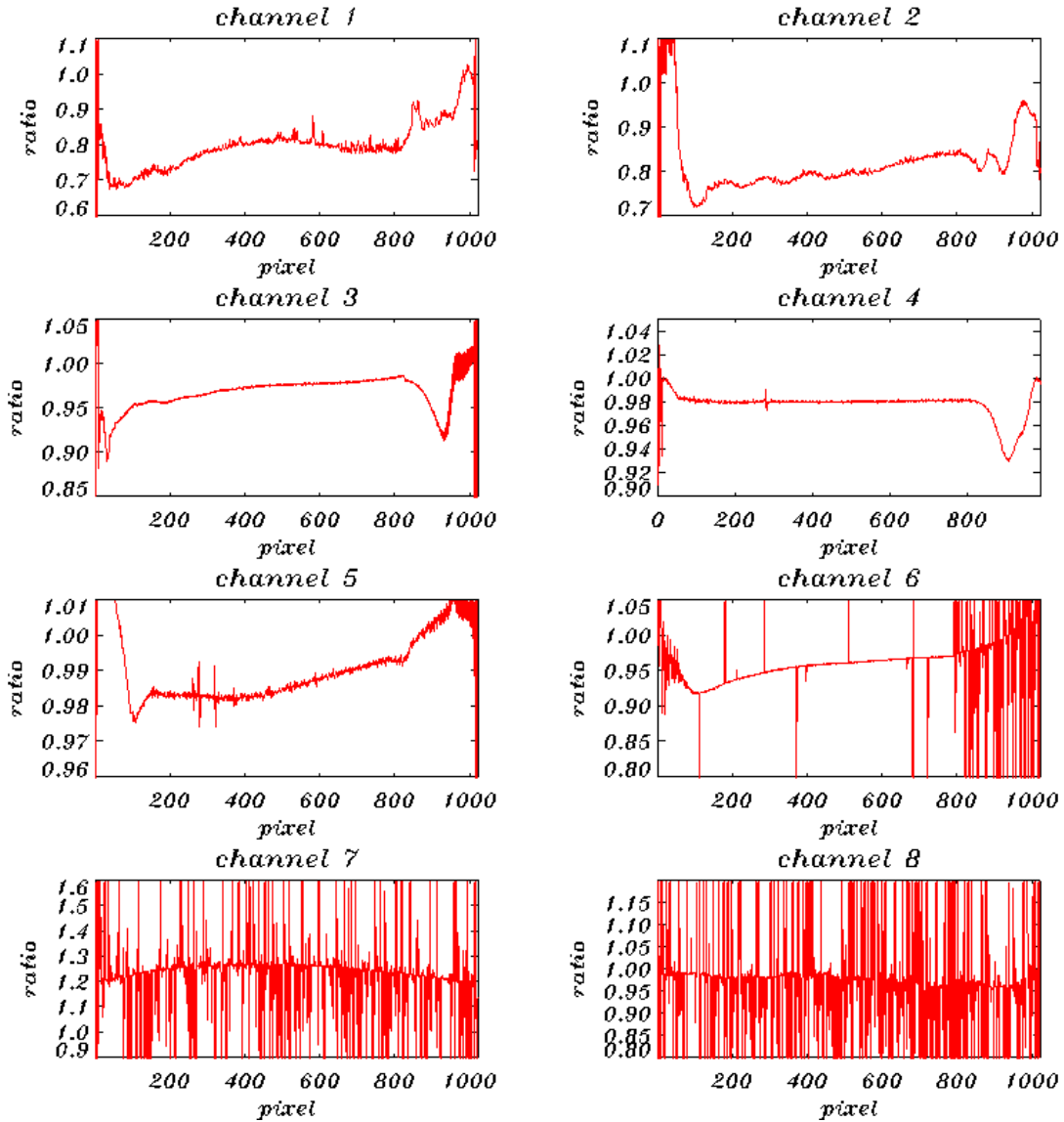
Figure 6.6: SMR ratios per detector channel on Long Term Trend 30/11/2011 divided by 30/11/2003.
