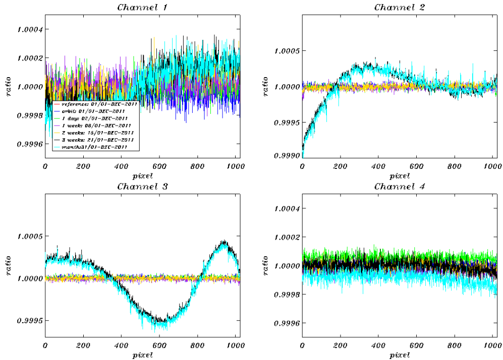
Figure 6.10: Dark current ratios (constant part) channels 1-4 during December 2011. Reference spectrum used: Orbit 51012, 01 December 2011.
