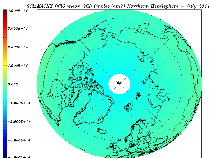
Figure 8.25: OClO SCD (molec/cm 2 ) for 01 – 31 July 2011 – monthly average over the Northern Hemisphere.
