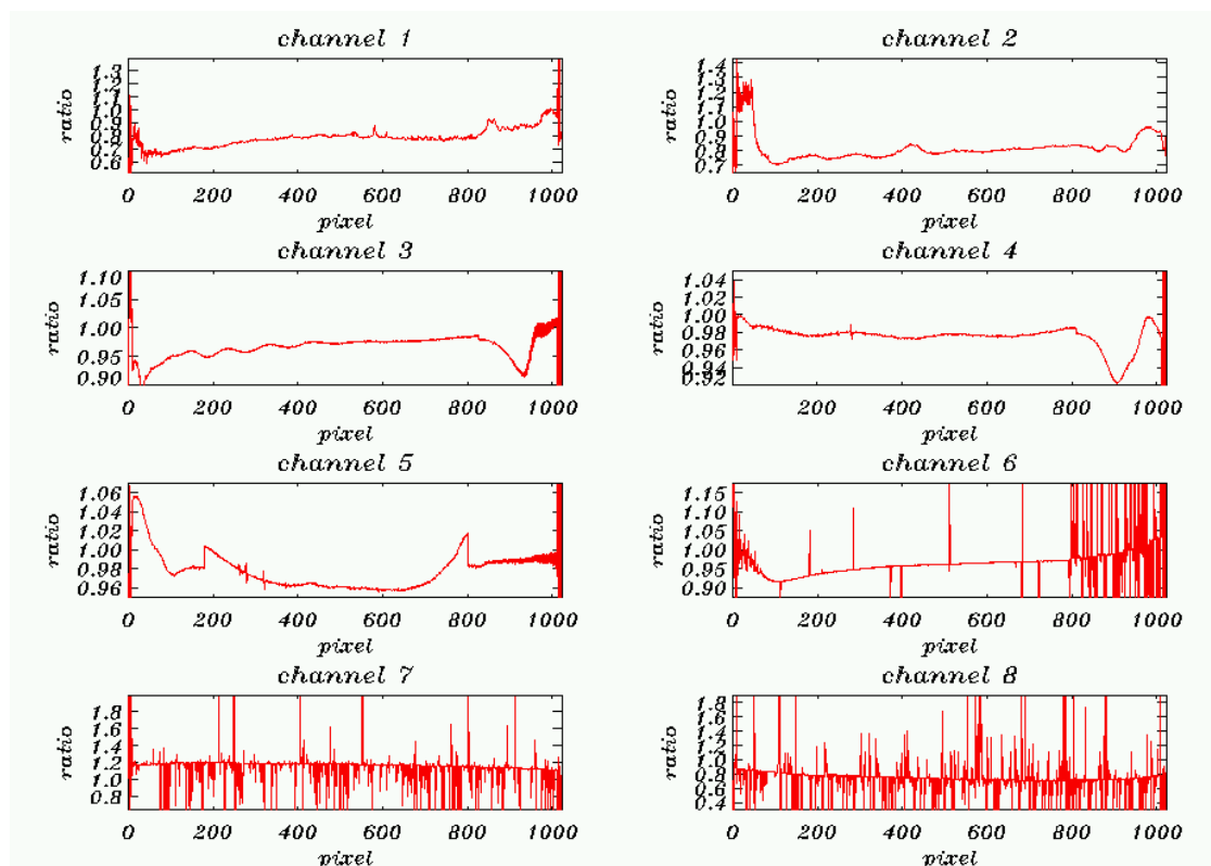
Figure 6.6: SMR ratios per detector channel on Long Term Trend 31/08/2011 divided by 31/08/2003.
