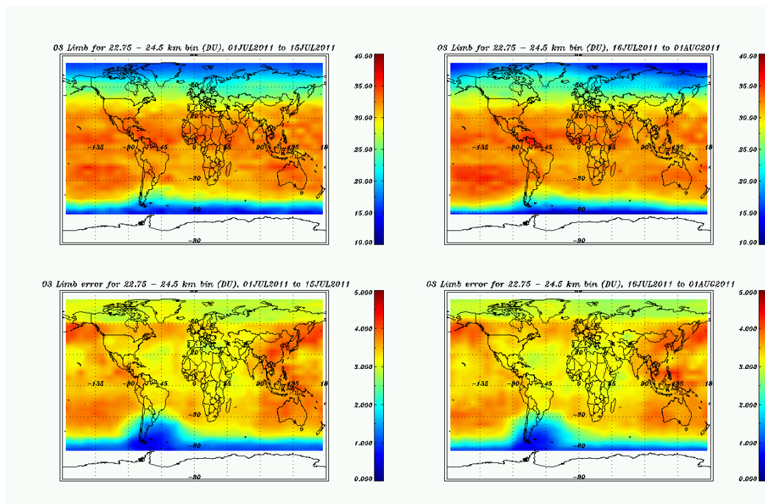
Figure 8.33: Limb Ozone profiles, binned over 22.75 – 24.5 km, July 2011.
