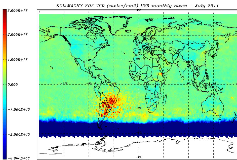
Figure 8.17: \text{SO}_2 VCD (molec/cm 2 ) world map for 01 –31 July 2011 – monthly average.
