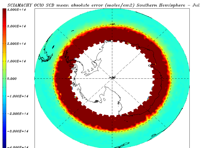
Figure 8.28: OCIO SCD error (molec/cm 2 ) for 01 – 31 July 2011- monthly average over the Southern Hemisphere.
