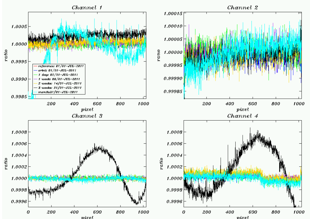
Figure 6.7: Dark current ratios (constant part) channels 1-4 during July 2011.
