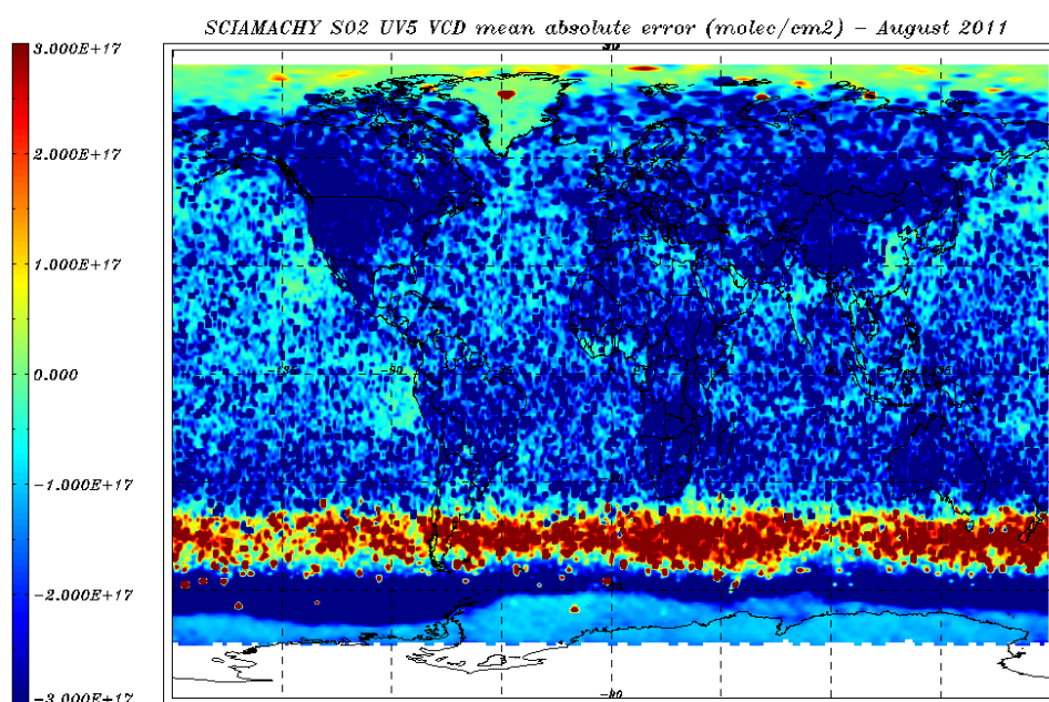
Figure 8.20: \text{SO}_2 VCD error (molec/cm 2 ) for 01 – 31 August 2011- monthly average.
