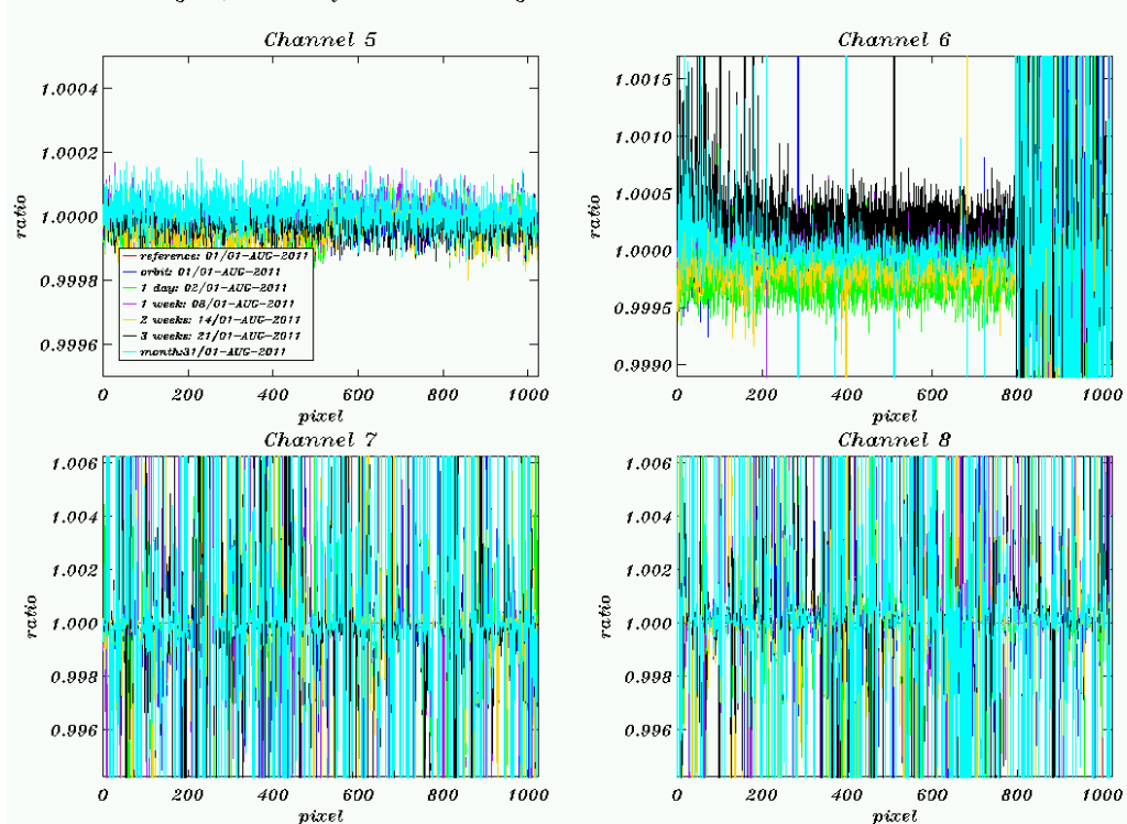
Figure 6.10: Dark current ratios (constant part) channels 5-8 during August 2011.
