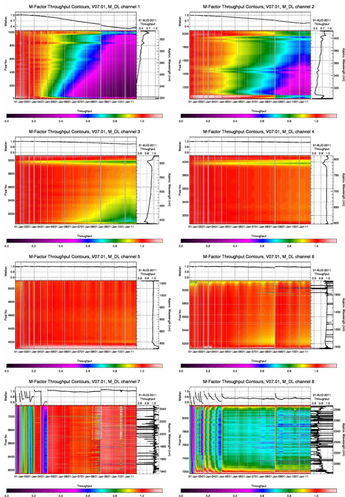
Figure 4.2: Degradation derived from m-factors August 2002 to August 2011 (limb light path).
