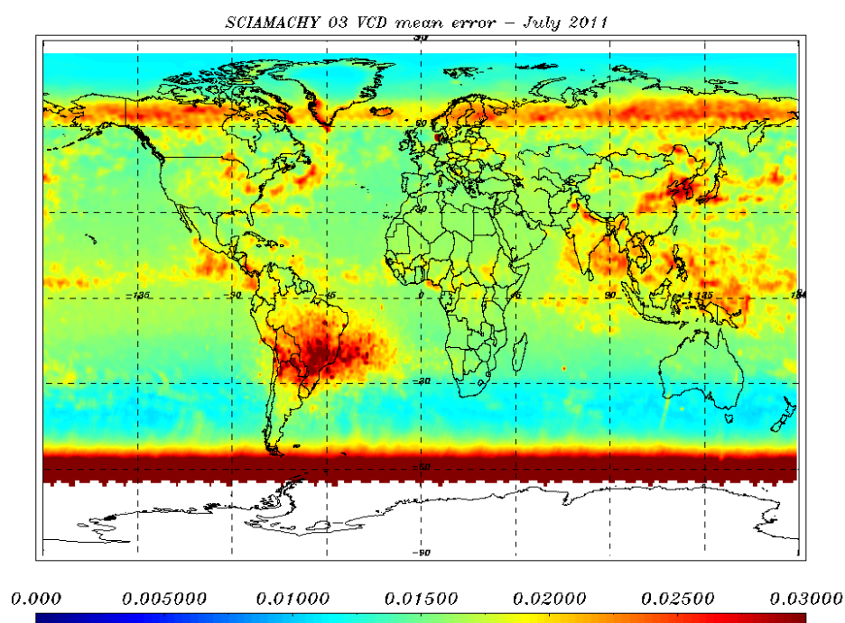
Figure 8.6: O_3 VCD error for 01 - 31 July 2011 - monthly average.
