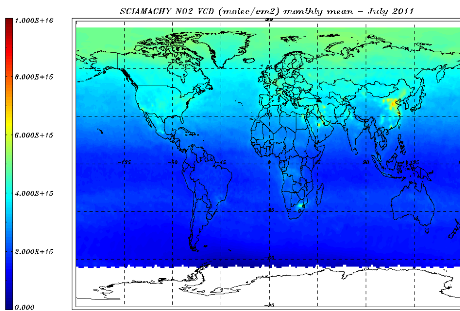
Figure 8.1: \text{NO}_2 VCD (molec/cm 2 ) world map for 01 - 31 July 2011 – monthly average.
