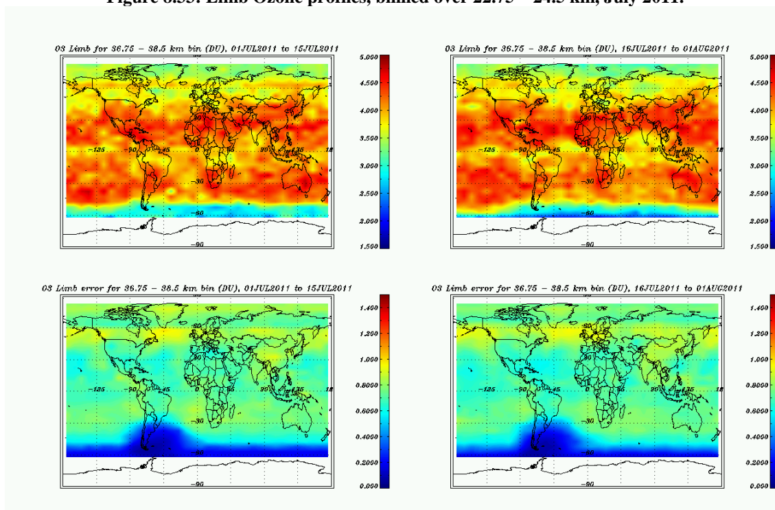
Figure 8.34: Limb Ozone profiles, binned over 36.75 – 38.5 km, July 2011.
