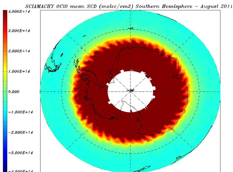
Figure 8.31: OCIO SCD (molec/cm 2 ) for 01 – 31 August 2011 – monthly average over the Southern Hemisphere.
