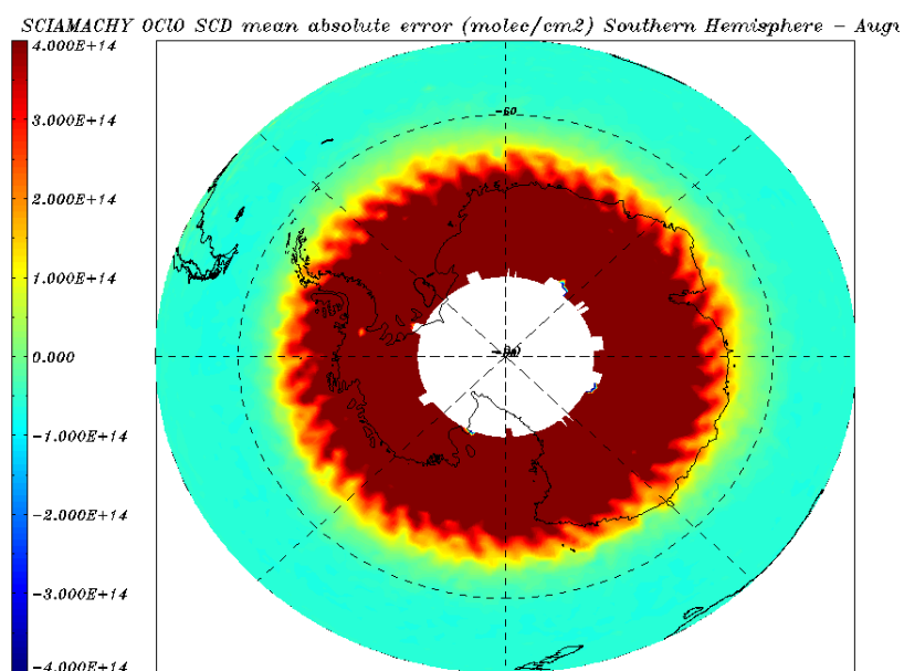
Figure 8.32: OCIO SCD error (molec/cm 2 ) for 01 – 31 August 2011- monthly average over the Southern Hemisphere.
