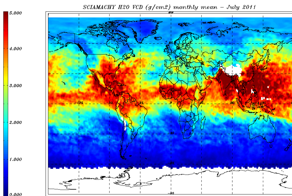
Figure 8.9: H_2O VCD ( g/cm^2 ) world map for 01 - 31 July 2011 – monthly average.
