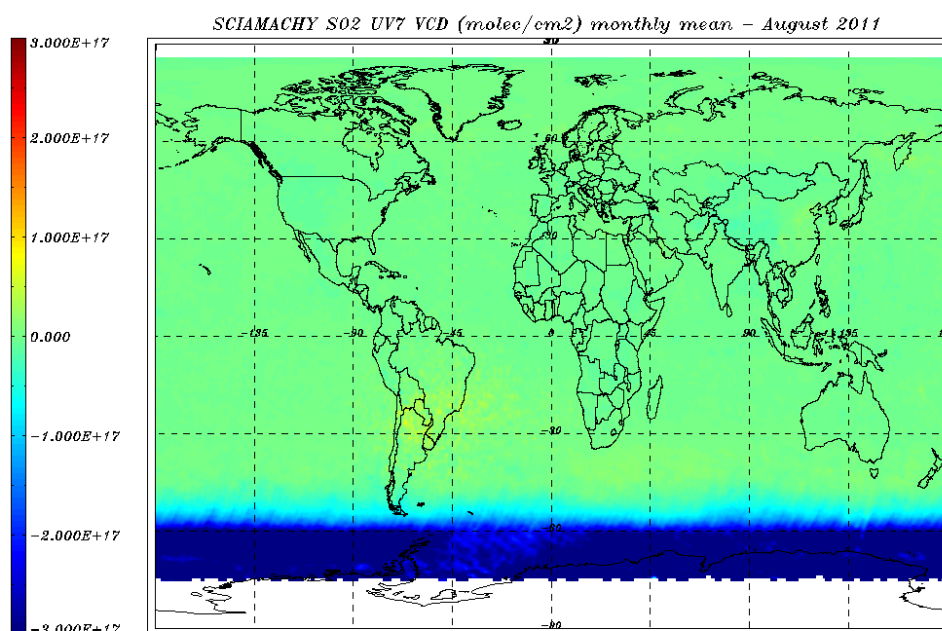
Figure 8.23: \text{SO}_2 VCD (molec/cm 2 ) world map for 01 – 31 August 2011 – monthly average.
