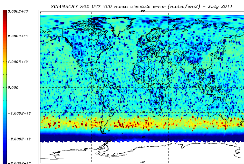
Figure 8.22: \text{SO}_2 VCD error (molec/cm 2 ) for 01 – 31 July 2011 – monthly average.
