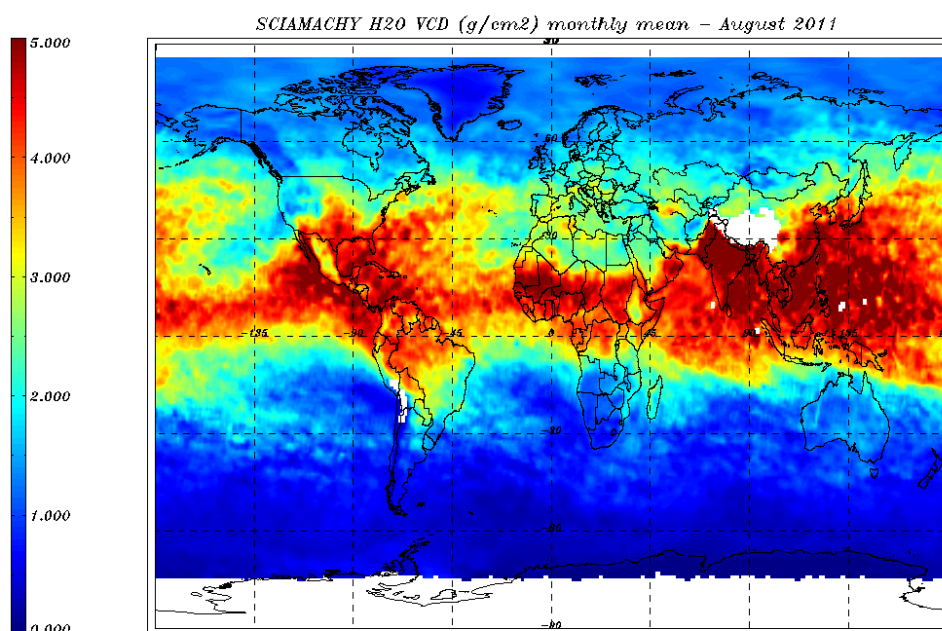
Figure 8.11: H_2O VCD ( g/cm^2 ) world map for 01 – 31 August 2011 – monthly average.
