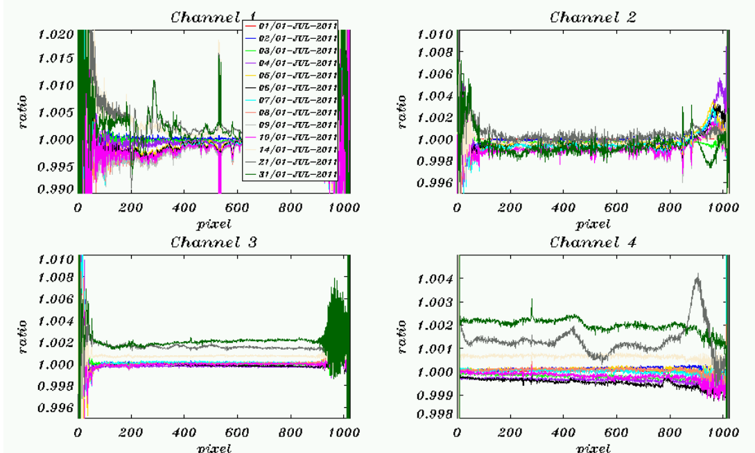
Figure 6.1: SMR ratios per detector channel 1-4 (changes during July 2011).
