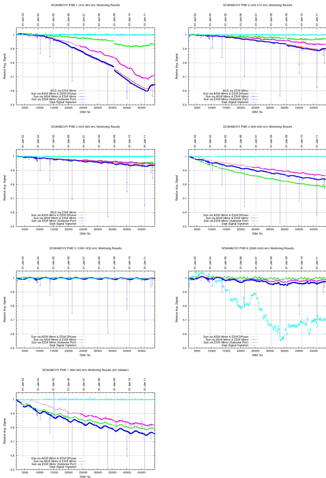
Figure 3.8: PMD monitoring results August 2002 to August 2011.
