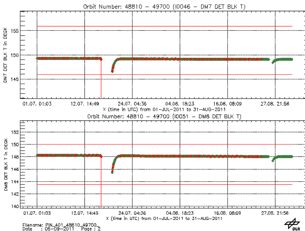
Figure 3.2: Detector temperatures.
