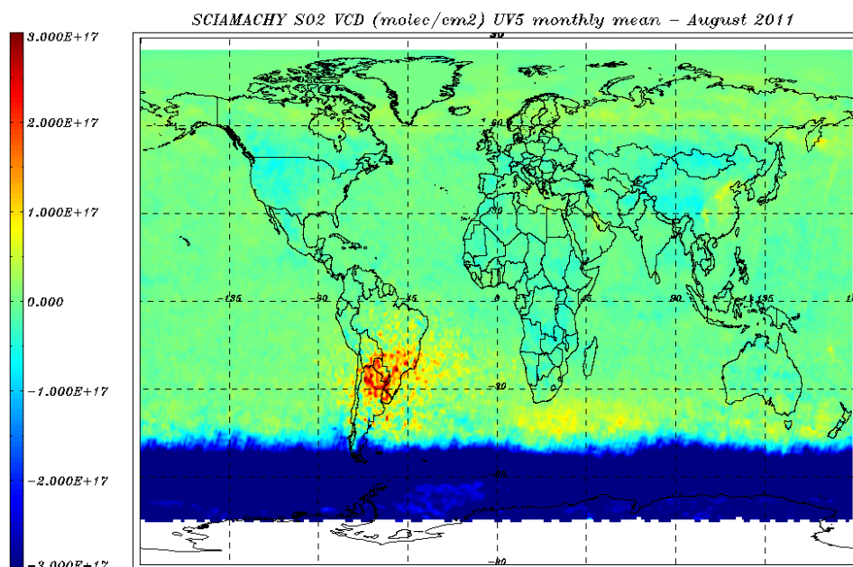
Figure 8.19: \text{SO}_2 VCD (molec/cm 2 ) world map for 01 – 31 August 2011 – monthly average.
