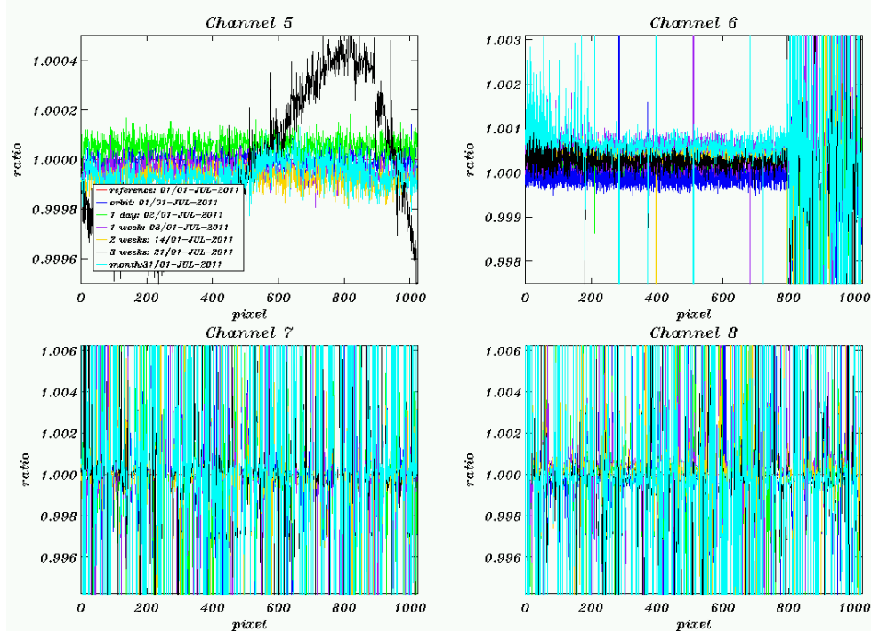
Figure 6.8: Dark current ratios (constant part) channels 5-8 during July 2011.
