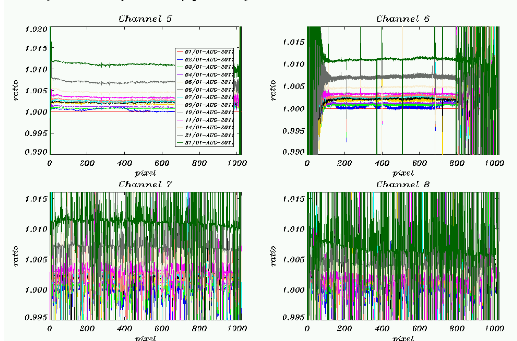
Figure 6.4: SMR ratios per detector channel 5-8 (changes during August 2011).
