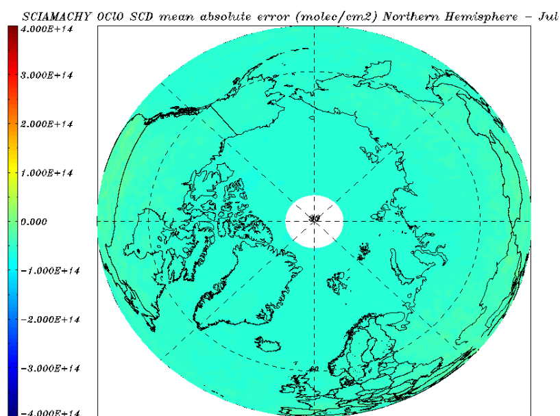
Figure 8.26: OClO SCD error (molec/cm 2 ) for 01 – 31 July 2011- monthly average over the Northern Hemisphere.
