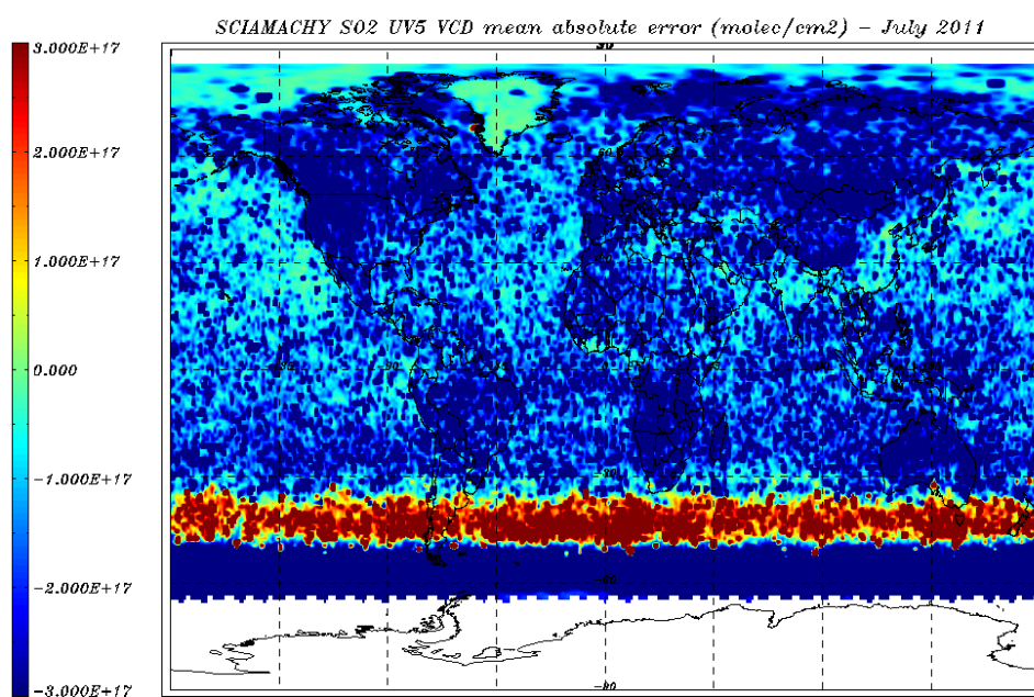
Figure 8.18: \text{SO}_2 VCD error (molec/cm 2 ) for 01 –31 July 2011- monthly average.
