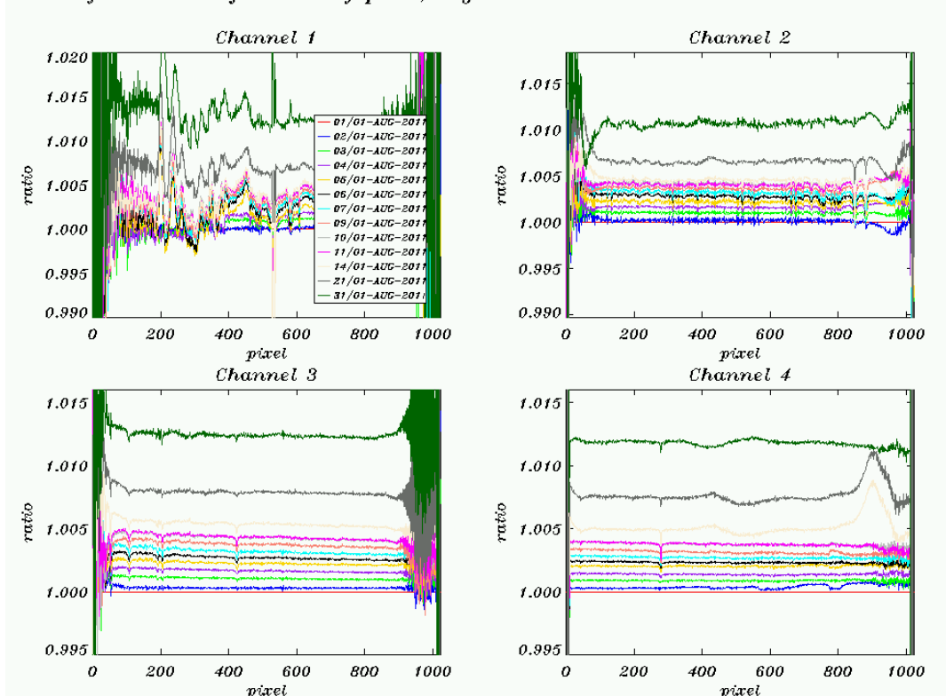
Figure 6.3: SMR ratios per detector channel 1-4 (changes during August 2011).
