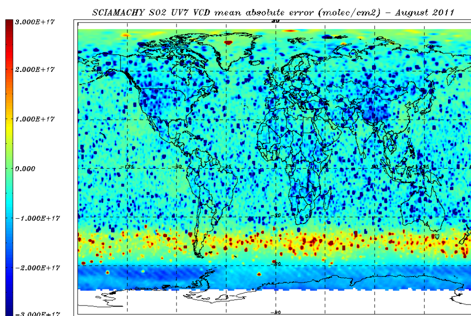
Figure 8.24: \text{SO}_2 VCD error (molec/cm 2 ) for 01 – 31 August 2011 – monthly average.
