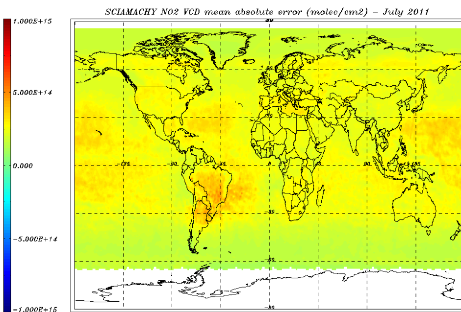
Figure 8.2: \text{NO}_2 VCD error (molec/cm 2 ) for 01 - 31 July 2011 - monthly average.
