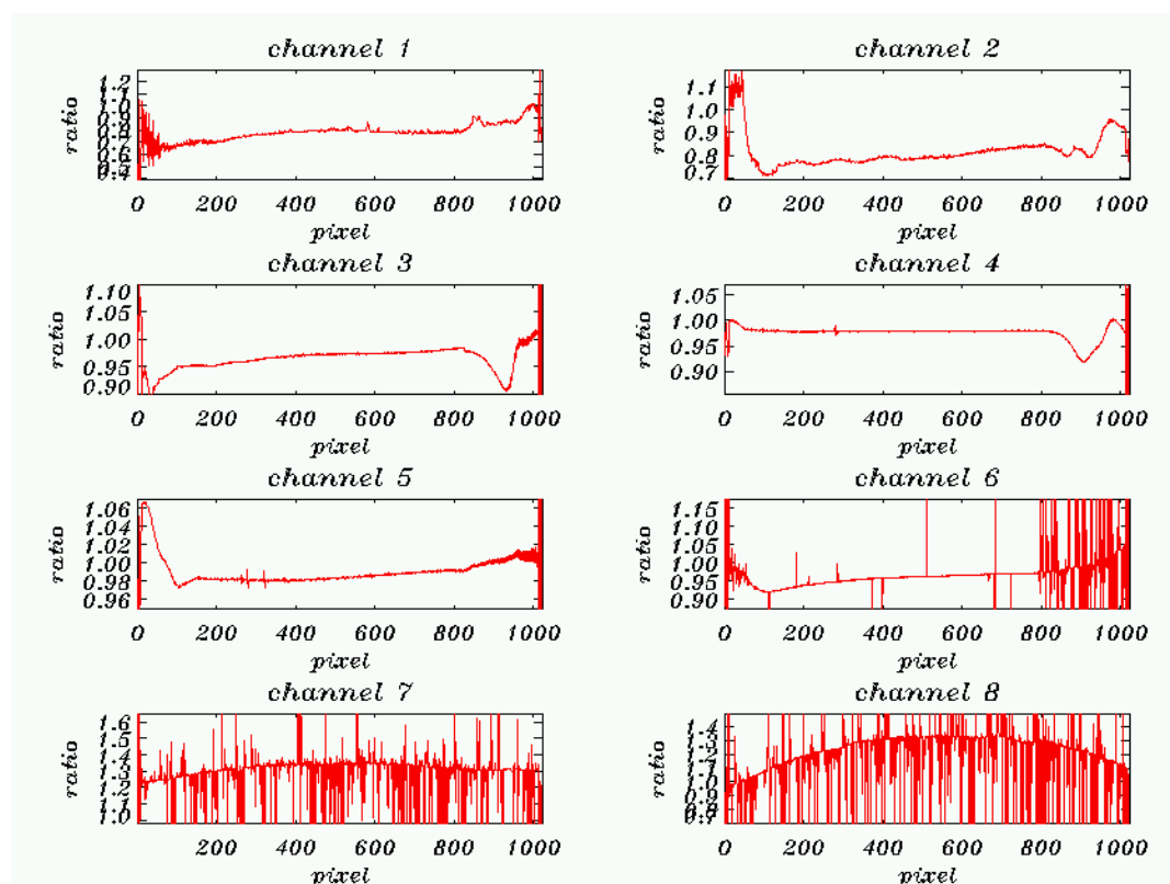
Figure 6.5: SMR ratios per detector channel on Long Term Trend 31/07/2011 divided by 31/07/2003.
