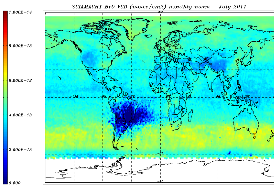
Figure 8.13: BrO VCD (molec/cm 2 ) world map for 01 – 31 July 2011 – monthly average.
