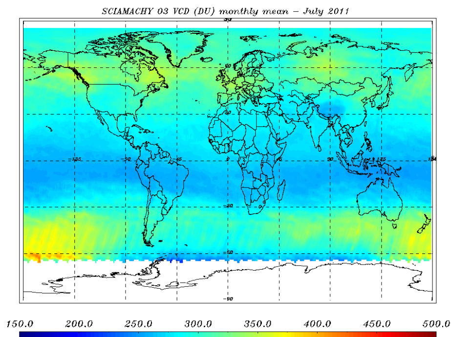
Figure 8.5: O_3 VCD (DU) world map for 01 - 31 July 2011 – monthly average.
