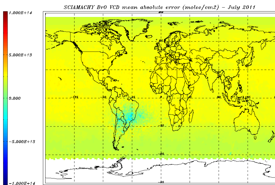
Figure 8.14: BrO VCD error (molec/cm 2 ) for 01 – 31 July 2011- monthly average.
