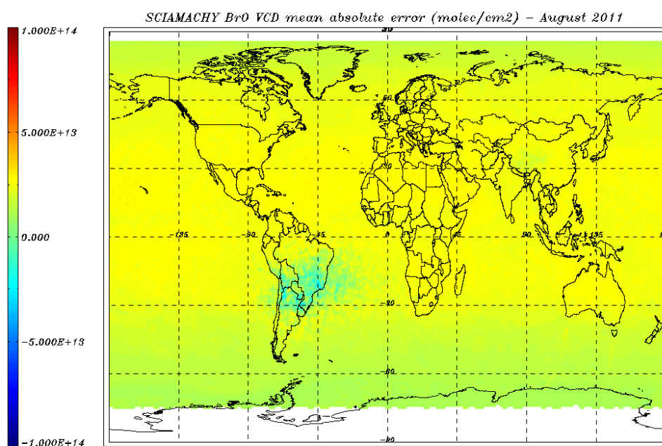
Figure 8.16: BrO VCD error (molec/cm 2 ) for 01 – 31 August 2011- monthly average.
