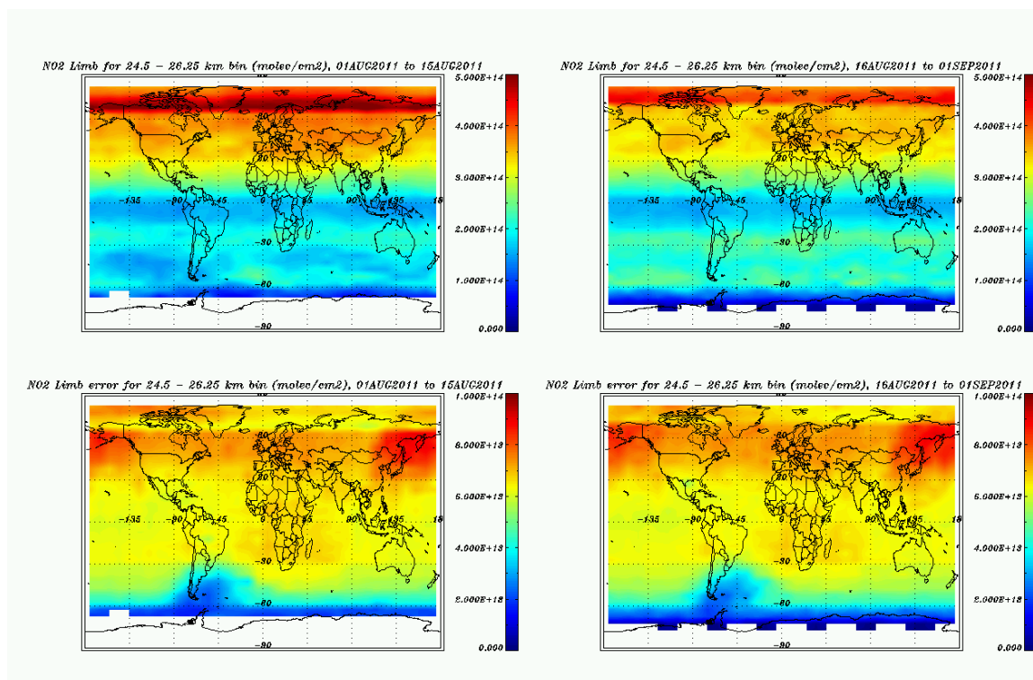
Figure 8.38: Limb NO 2 profiles binned over 24.5 – 26.25 km, August 2011.
