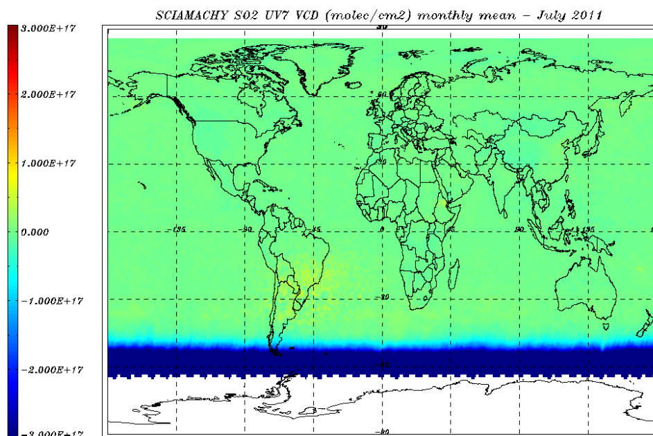
Figure 8.21: \text{SO}_2 VCD (molec/cm 2 ) world map for 01 – 31 July 2011 – monthly average.
