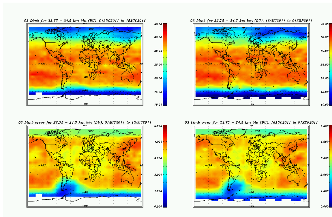
Figure 8.35: Limb Ozone profiles binned over 22.75 – 24.5 km, August 2011.
