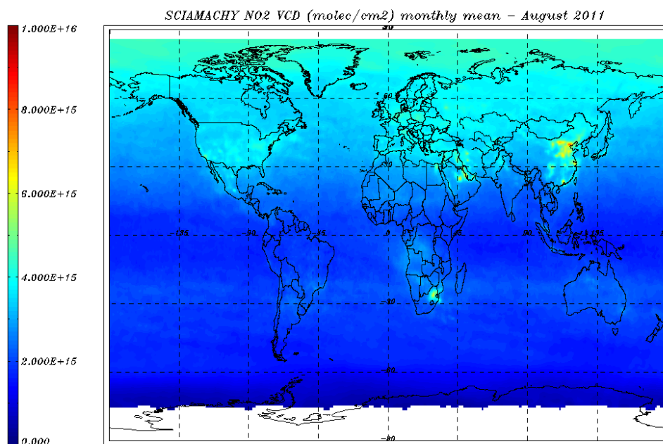
Figure 8.3: NO 2 VCD (molec/cm 2 ) world map for 01 – 31 August 2011 – monthly average.
