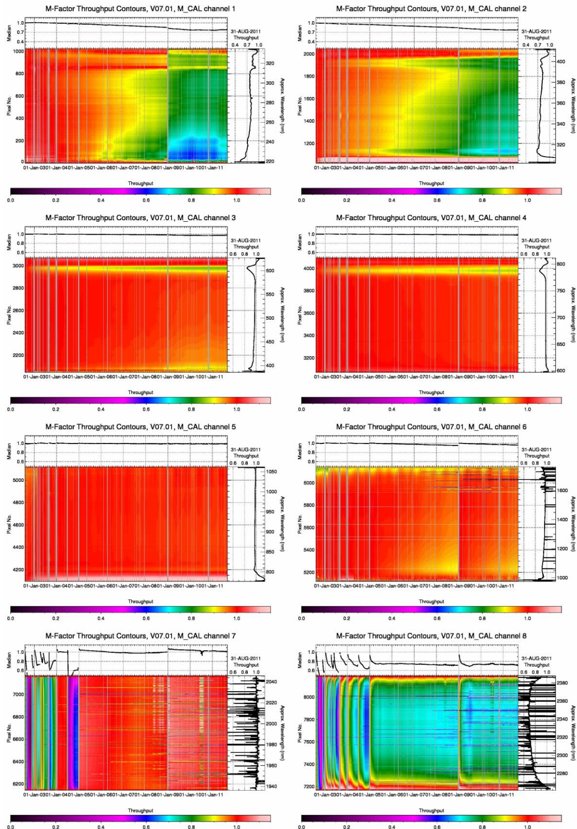
Figure 4.3: Degradation derived from m-factors August 2002 to August 2011 (calibr. light path).
