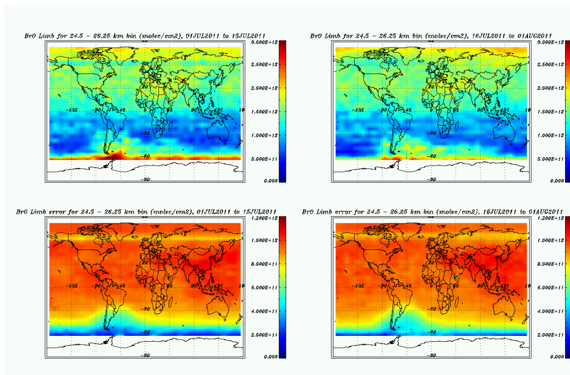
Figure 8.39: Limb BrO profiles binned over 24.5 – 26.25 km, July 2011.
