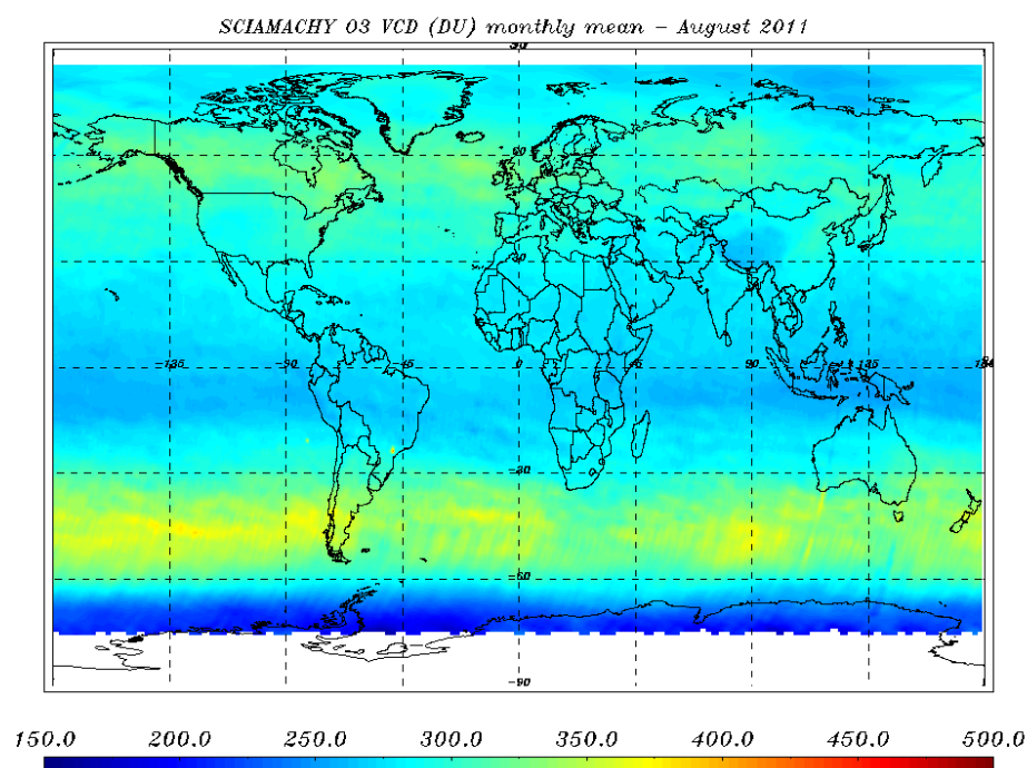
Figure 8.7: O 3 VCD (DU) world map for 01 - 31 August 2011 – monthly average.
