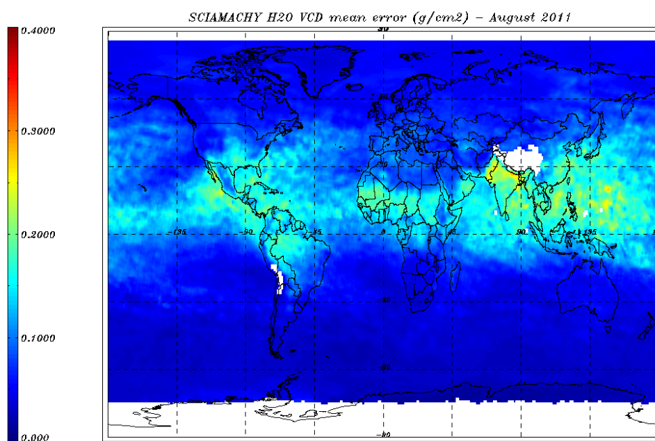
Figure 8.12: H_2O VCD ( g/cm^2 ) error for 01 – 31 August 2011- monthly average.
