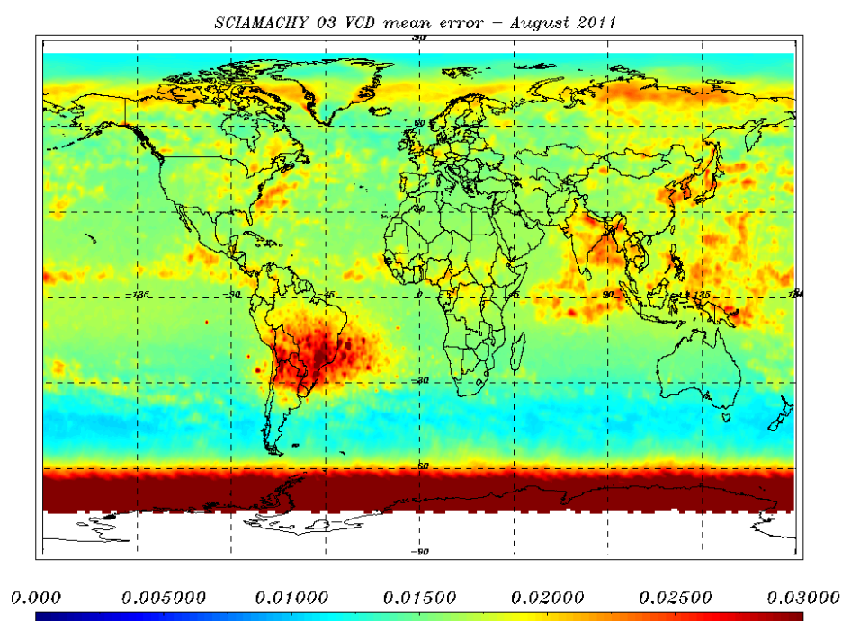
Figure 8.8: O 3 VCD error for 01- 31 August 2011 - monthly average.
