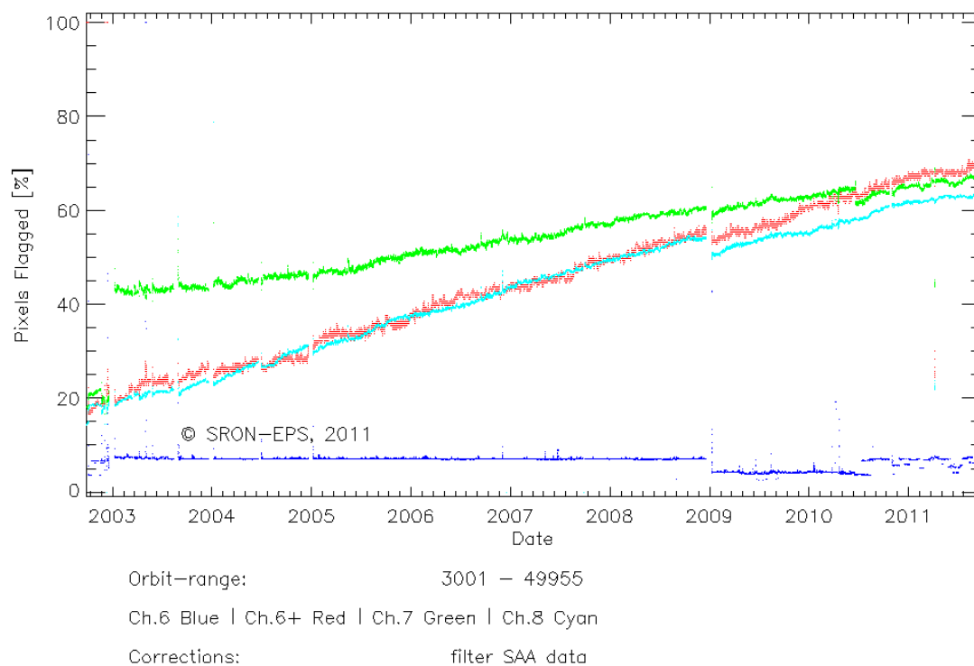
Figure 6.12: Number/Fraction of pixels that is flagged as bad by the SDMF smoothmask for channels 6 (blue), 6+ (red), 7 (green) and 8 (cyan). Orbits during SODAP or decontaminations have been removed. Note the temporary decrease in the number of bad pixels after the last decontamination, for channel 8 about 6%, a few percent more than after the previous decontaminations.
