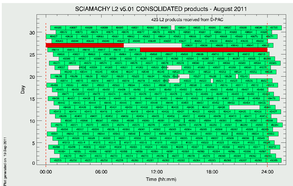
Figure 5.2: SCIAMACHY Level 2 off-line data production at D-PAC for August 2011.
