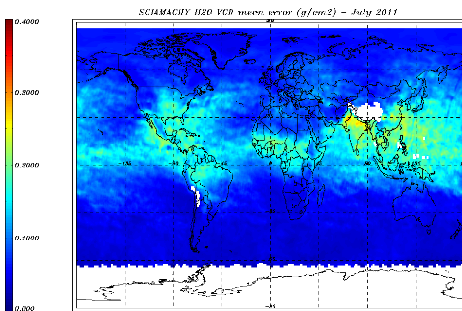
Figure 8.10: H_2O VCD ( g/cm^2 ) error for 01 - 31 July 2011 - monthly average.
