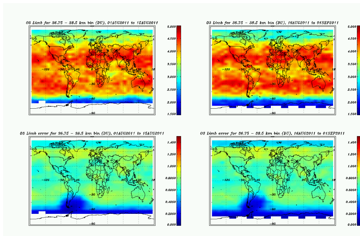
Figure 8.36: Limb Ozone profiles binned over 36.75 – 38.5 km, August 2011.
