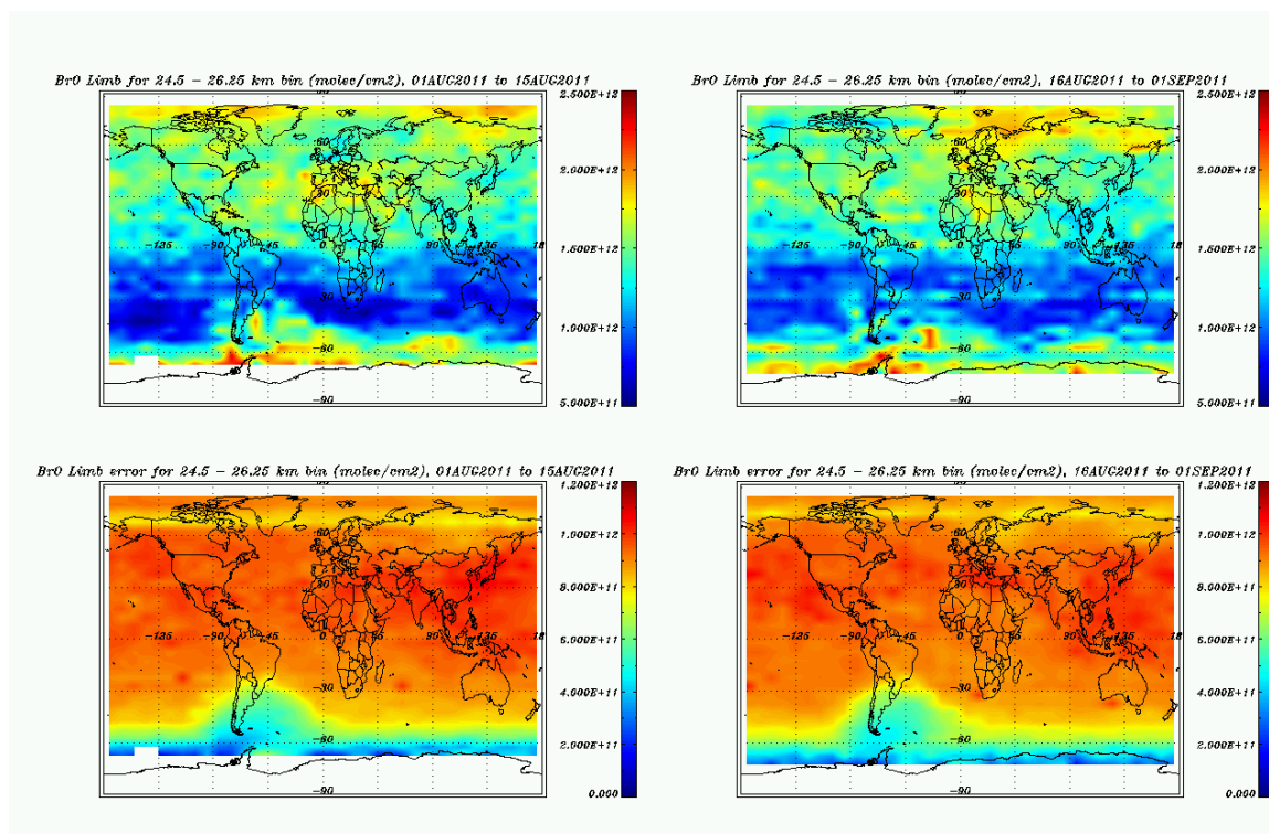
Figure 8.40: Limb BrO profiles binned over 24.5 – 26.25 km, August 2011.
