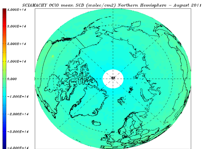
Figure 8.29: OCIO SCD (molec/cm 2 ) for 01 – 31 August 2011 – monthly average over the Northern Hemisphere.
