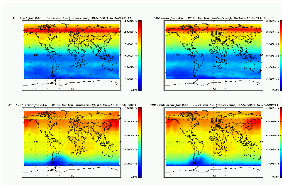
Figure 8.37: Limb NO 2 profiles binned over 24.5 – 26.25 km, July 2011.
