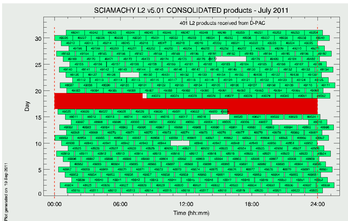
Figure 5.1: SCIAMACHY Level 2 off-line data production at D-PAC for July 2011.
