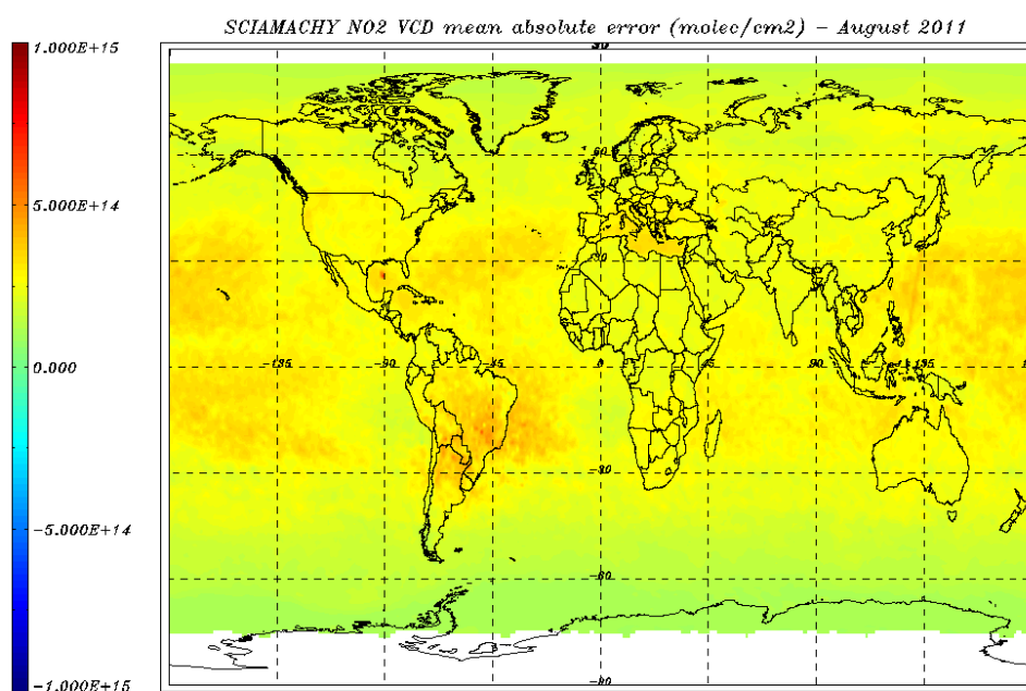
Figure 8.4: NO 2 VCD error (molec/cm 2 ) for 01 – 31 August 2011- monthly average.
