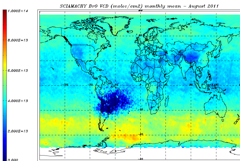
Figure 8.15: BrO VCD (molec/cm 2 ) world map for 01 – 31 August 2011 – monthly average.
