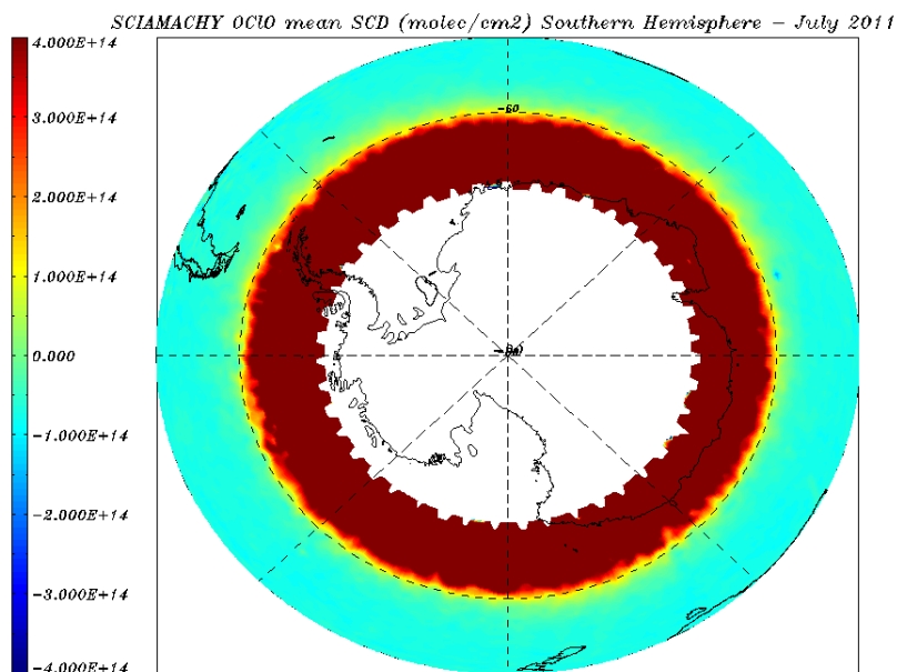
Figure 8.27: OCIO SCD (molec/cm 2 ) for 01 – 31 July 2011 – monthly average over the Southern Hemisphere.
