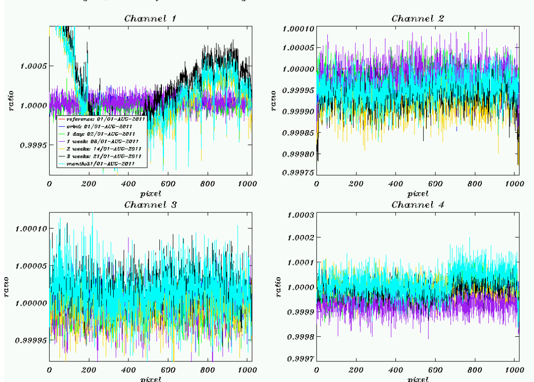
Figure 6.9: Dark current ratios (constant part) channels 1-4 during August 2011.
