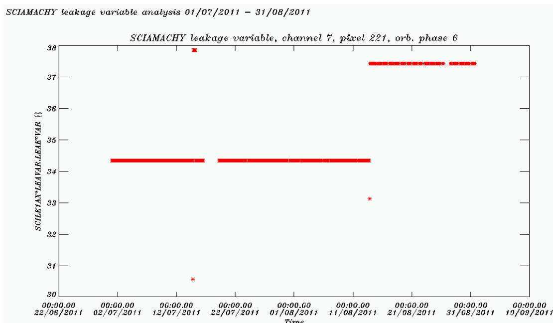
Figure 6.11: Leakage variable part from 01 July 2011 to 31 August 2011, for channel 7, orbit phase 6, pixel 222.
