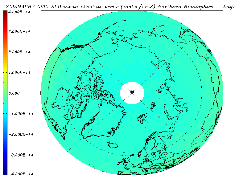
Figure 8.30: OCIO SCD error (molec/cm 2 ) for 01 – 31 August 2011- monthly average over the Northern Hemisphere.
