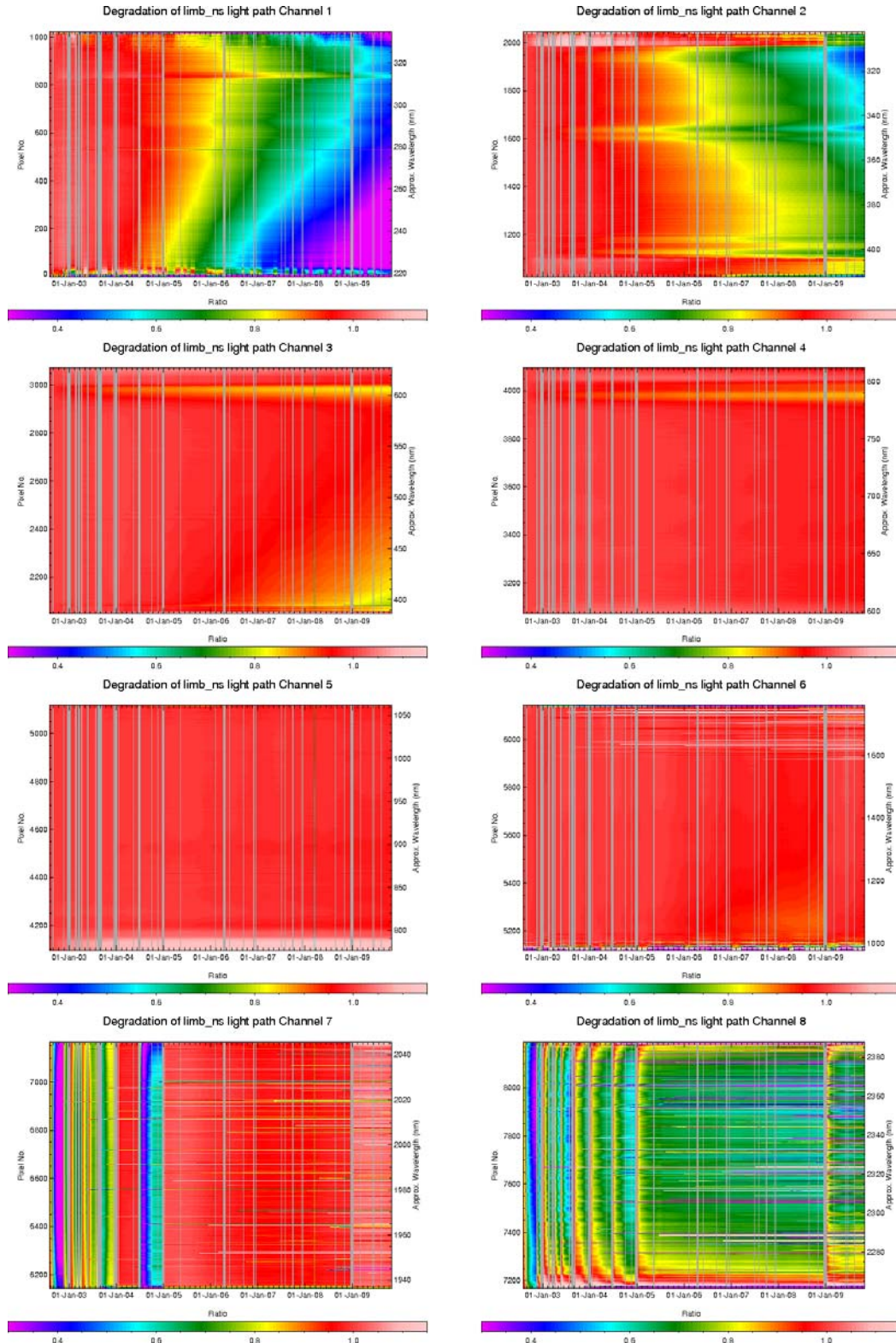
Fig. 3.9: Spectral light path monitoring results August 2002 to October 2009 (limb light path).
