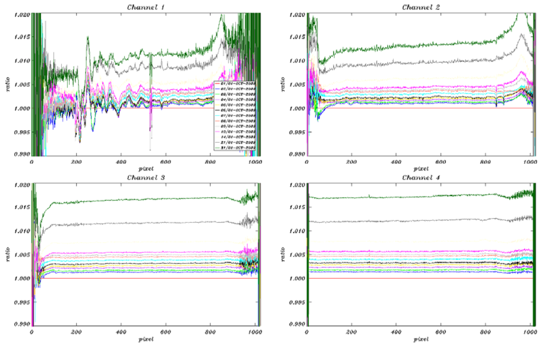
Fig. 5-4: SMR ratios per detector channel 1-4 (changes during October 2009).
