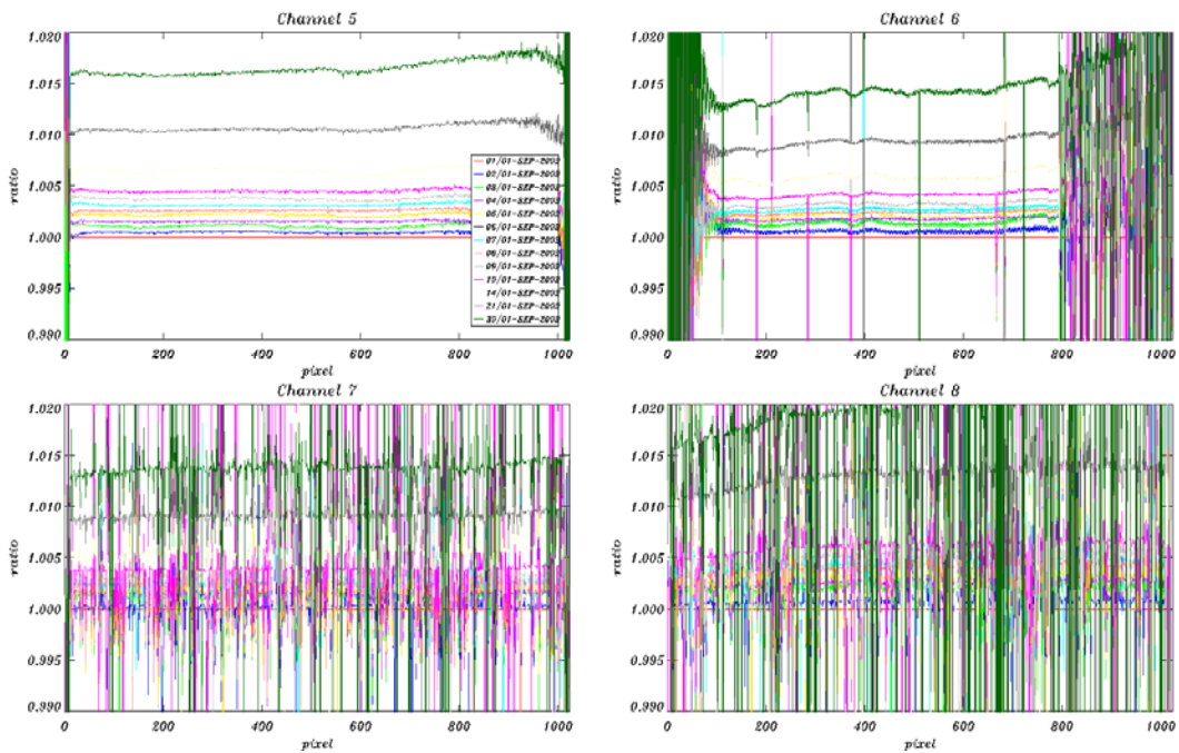
Fig. 5-3: SMR ratios per detector channel 5-8 (changes during September 2009).
