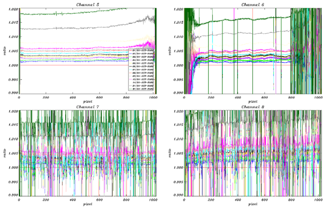
Fig. 5-5: SMR ratios per detector channel 5-8 (changes during October 2009).
