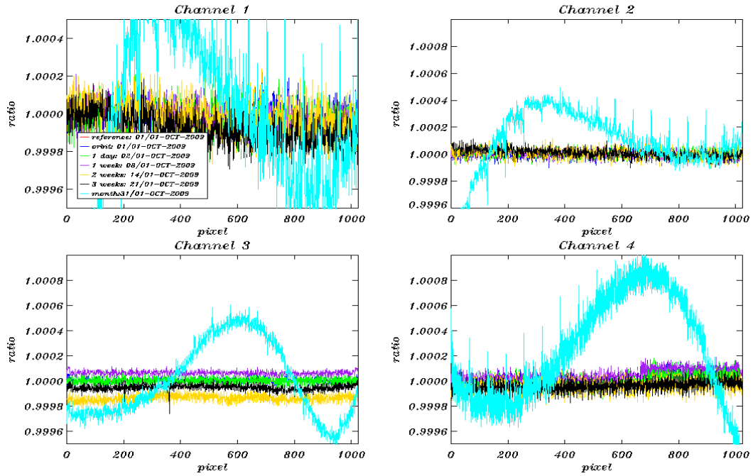
Fig. 5-10: Dark current ratios (constant part) channel 1-4 during October 2009. Reference Spectrum used: Orbit 39669, 01-October-2009
