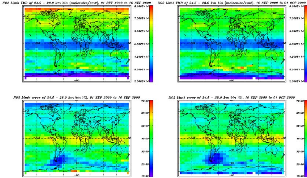
Figure 7-13 Limb NO 2 profiles binned over 24.5 – 28 km, September 2009.
