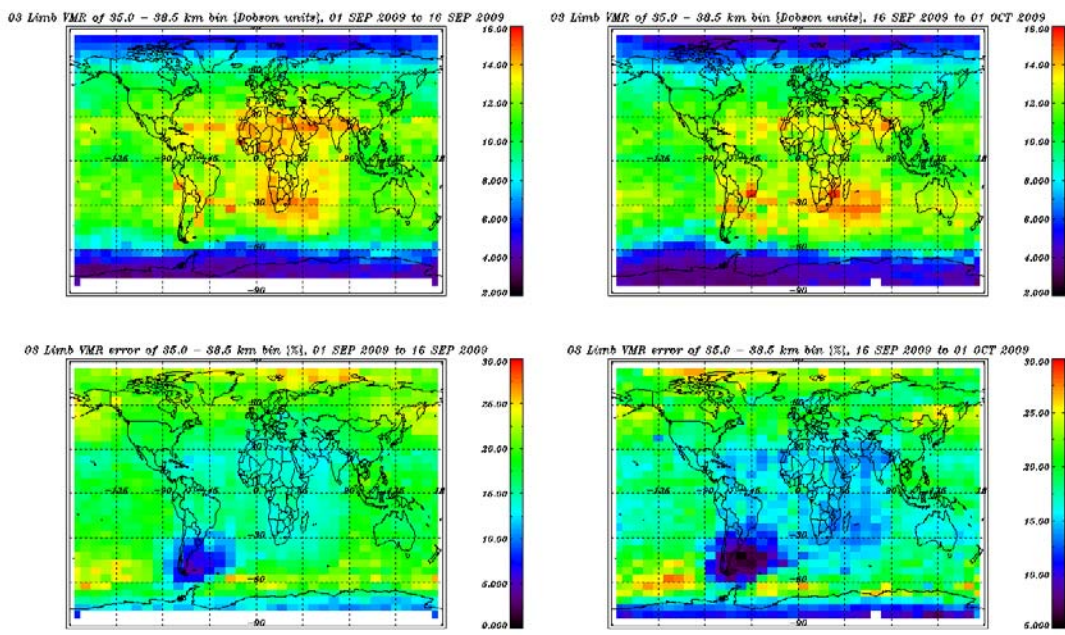
Figure 7-10 Limb Ozone profiles, binned over 35.0 – 38.5 km, September 2009.
