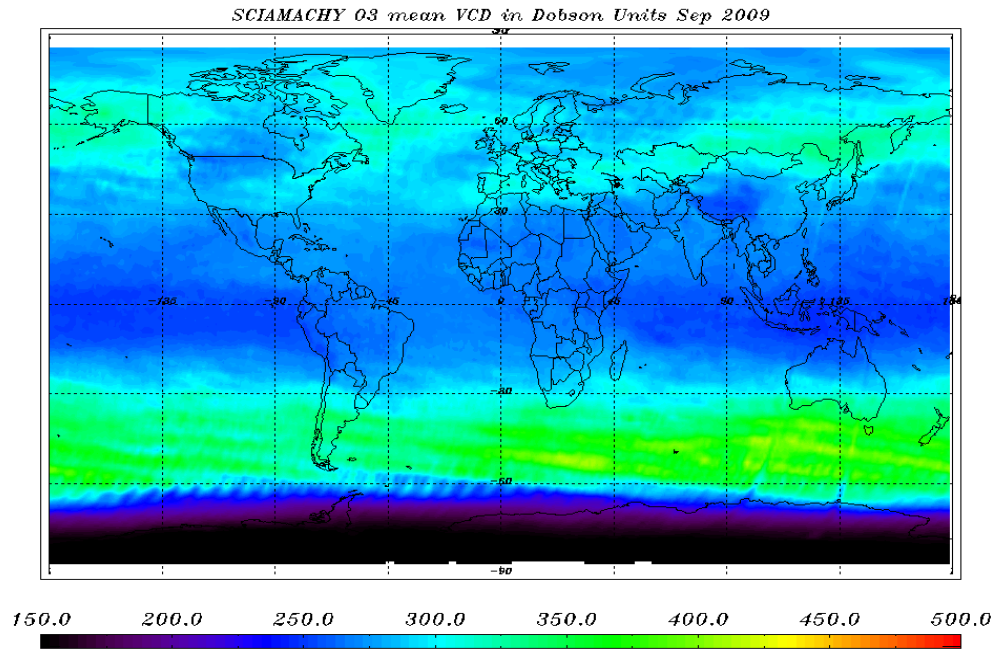
Figure 7-5: O 3 VCD world map for 01 - 30 September 2009 – monthly average.
