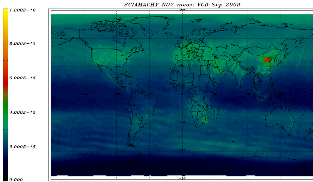
Figure 7-1: NO 2 VCD world map for 01 - 30 September 2009 – monthly average.
