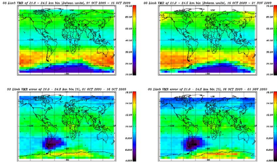
Figure 7-11: Limb Ozone profiles binned over 21.0 – 24.5 km, October 2009.
