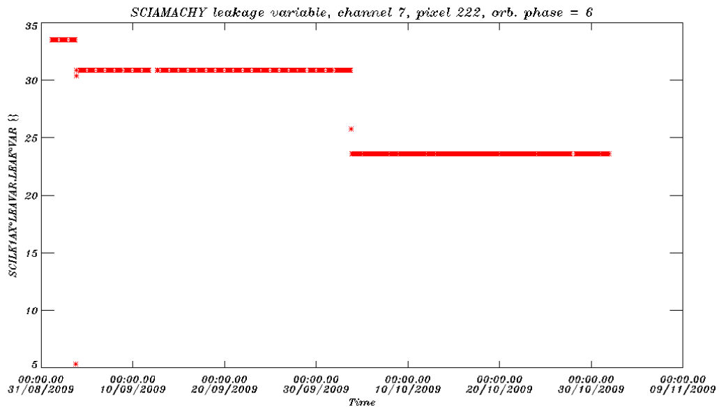
Figure 5-12: Leakage VARIABLE, SCI_LK1_AX, 01 September – 31 October 2009, channel 7, orbit phase 6, pixel 222.
