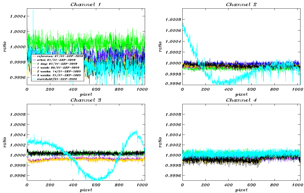
Fig. 5-8: Dark current ratios (constant part) channel 1-4 during September 2009. Reference Spectrum used: Orbit 39239, 01-September-2009.
