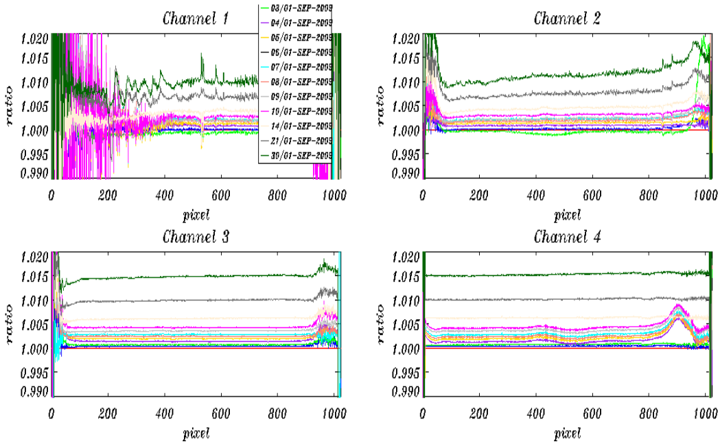
Fig. 5-2: SMR ratios per detector channel 1-4 (changes during September 2009).
