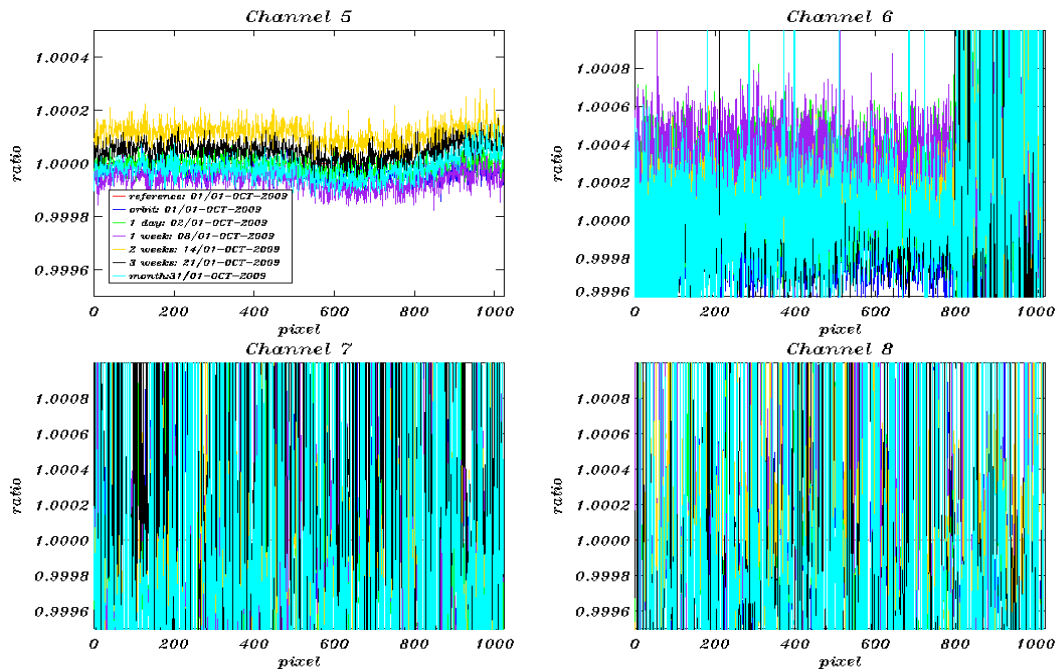
Fig. 5-11: Dark current ratios (constant part) channel 5-8 during October 2009. Reference Spectrum used: Orbit 39669, 01-October-2009.
