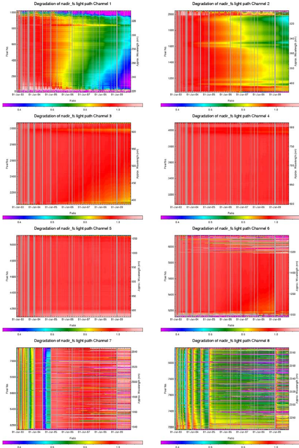
Fig. 3.8: Spectral light path monitoring results August 2002 to October 2009 (nadir light path).
