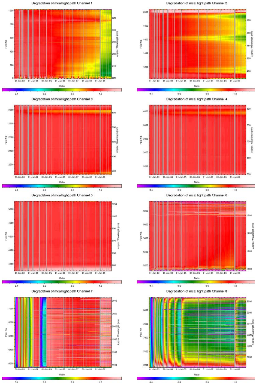
Fig. 3.10: Spectral light path monitoring results August 2002 to October 2009 (calibration light path).
