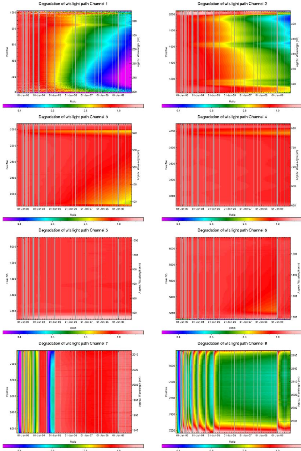
Fig. 3.11: Spectral light path monitoring results August 2002 to October 2009 (WLS light path).
