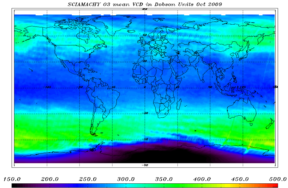
Figure 7-7: O 3 VCD world map for 01 - 31 October 2009 – monthly average.
