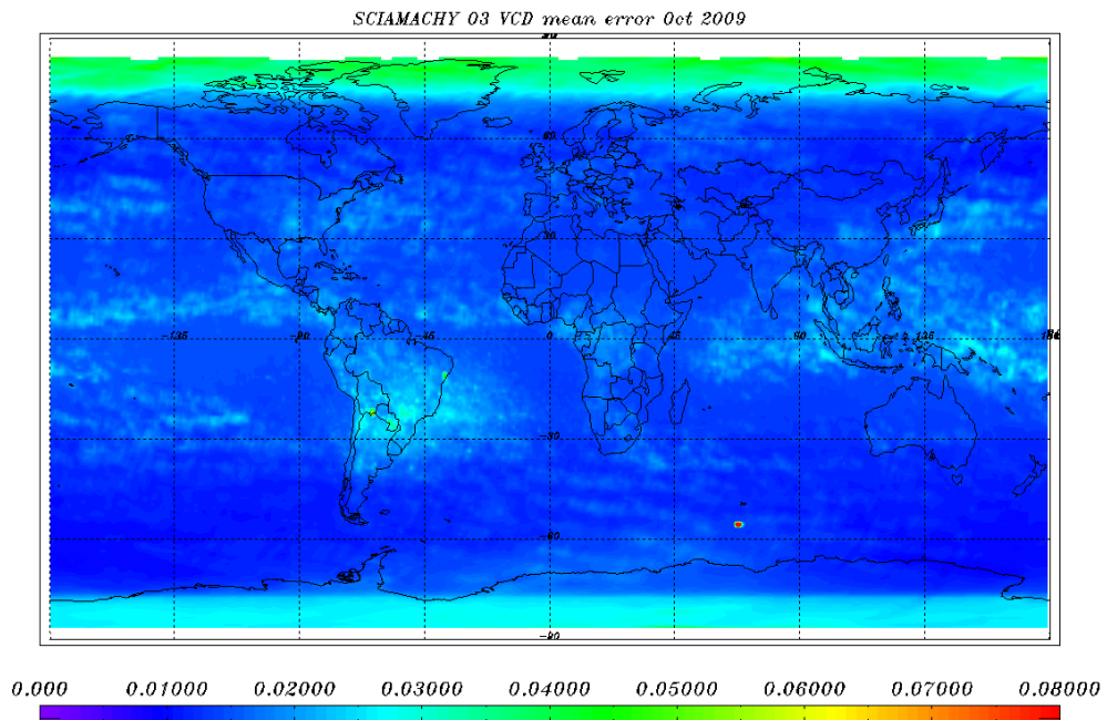
Figure 7-8: O 3 VCD error for 01- 31 October 2009 - monthly average.
