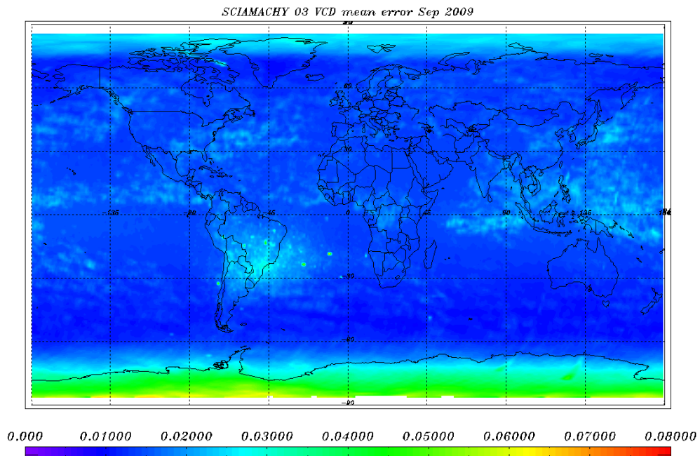
Figure 7-6: O 3 VCD error for 01 - 30 September 2009 - monthly average.
