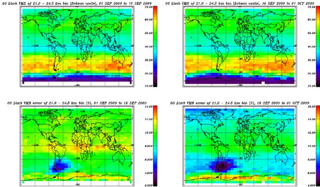
Figure 7-9 Limb Ozone profiles, binned over 21.0 – 24.5 km, September 2009.
