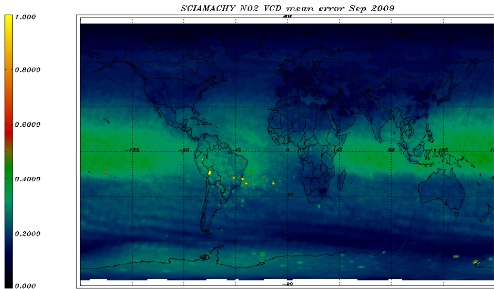
Figure 7-2: NO 2 VCD error for 01 - 30 September 2009 - monthly average.
