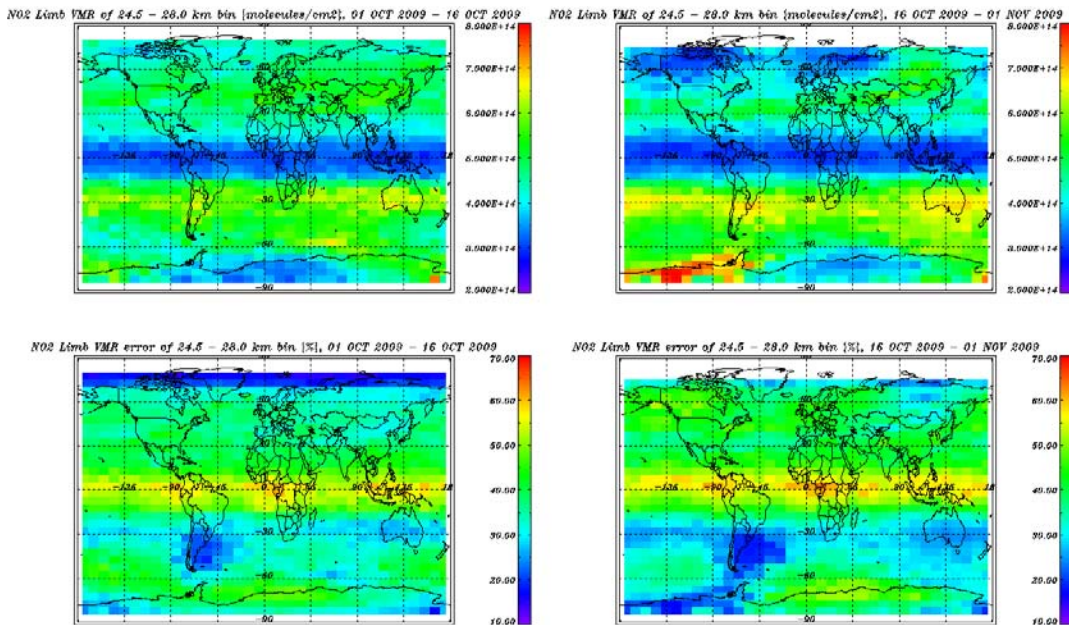
Figure 7-14 Limb NO 2 profiles binned over 24.5 – 28 km, October 2009.
