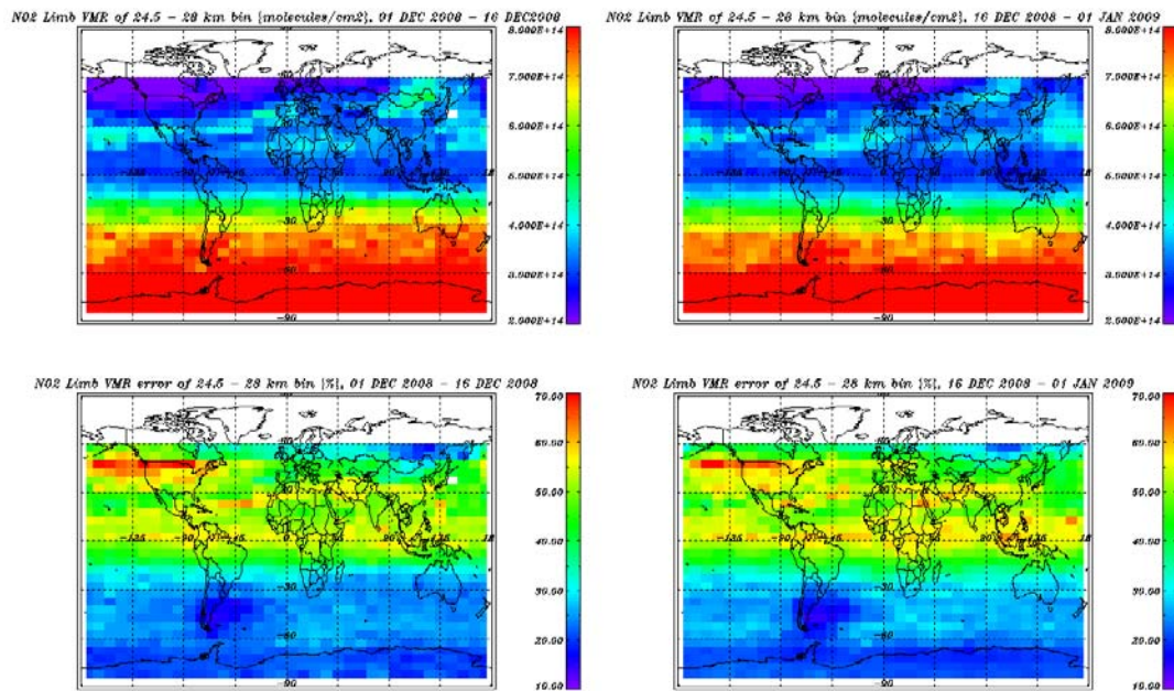
Figure 7-14 Limb NO 2 profiles binned over 24.5 - 28 km, December 2008
