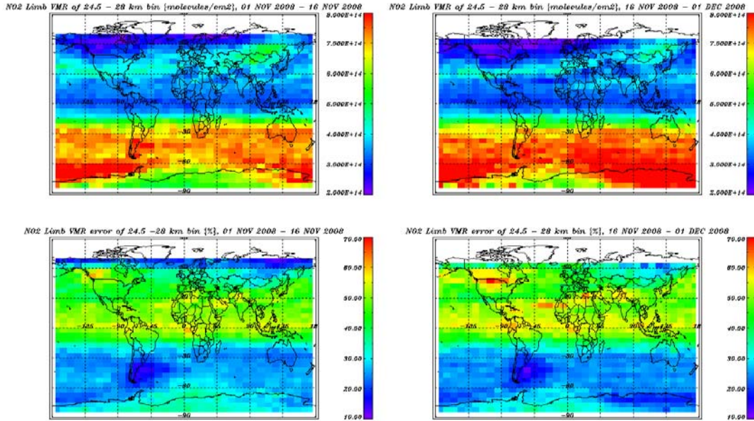
Figure 7-13 Limb NO 2 profiles binned over 24.5 - 28 km, November 2008
