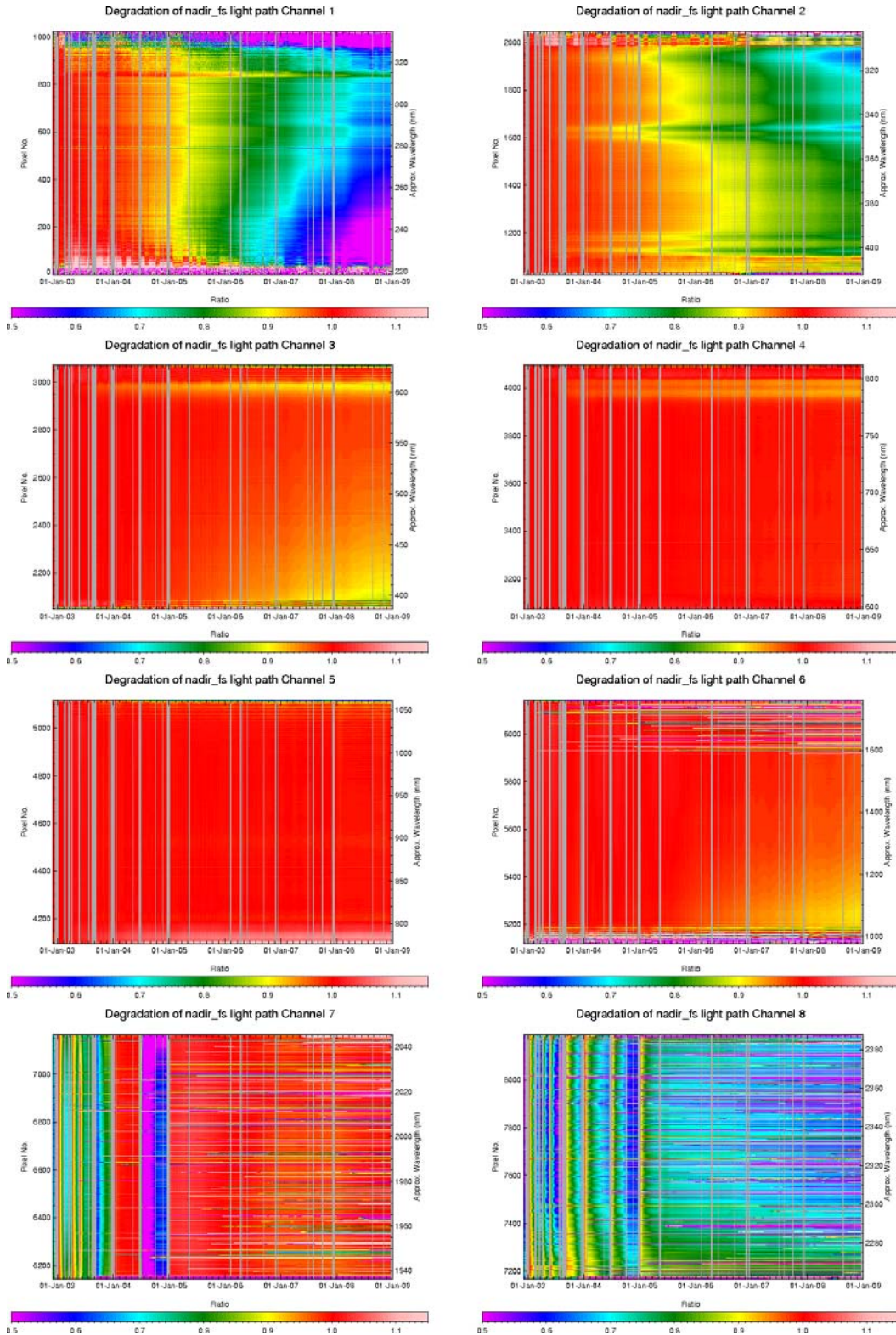
Fig. 3.8: Spectral light path monitoring results August 2002 to December 2008 (nadir light path)
