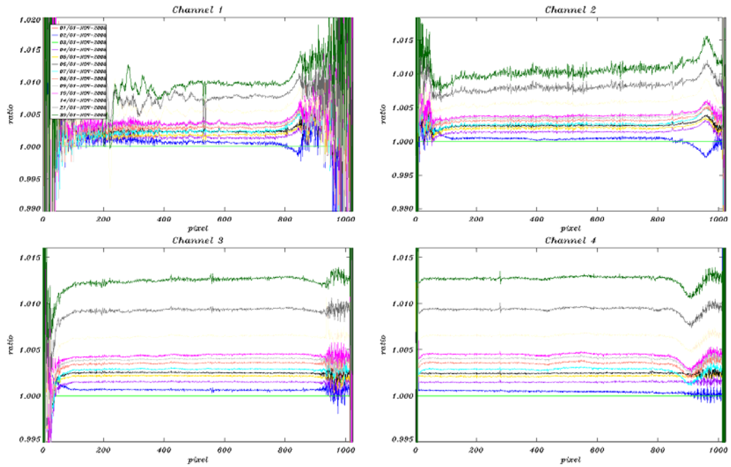
Fig. 5-2: SMR ratios per detector channel 1-4 (changes during November 2008)
