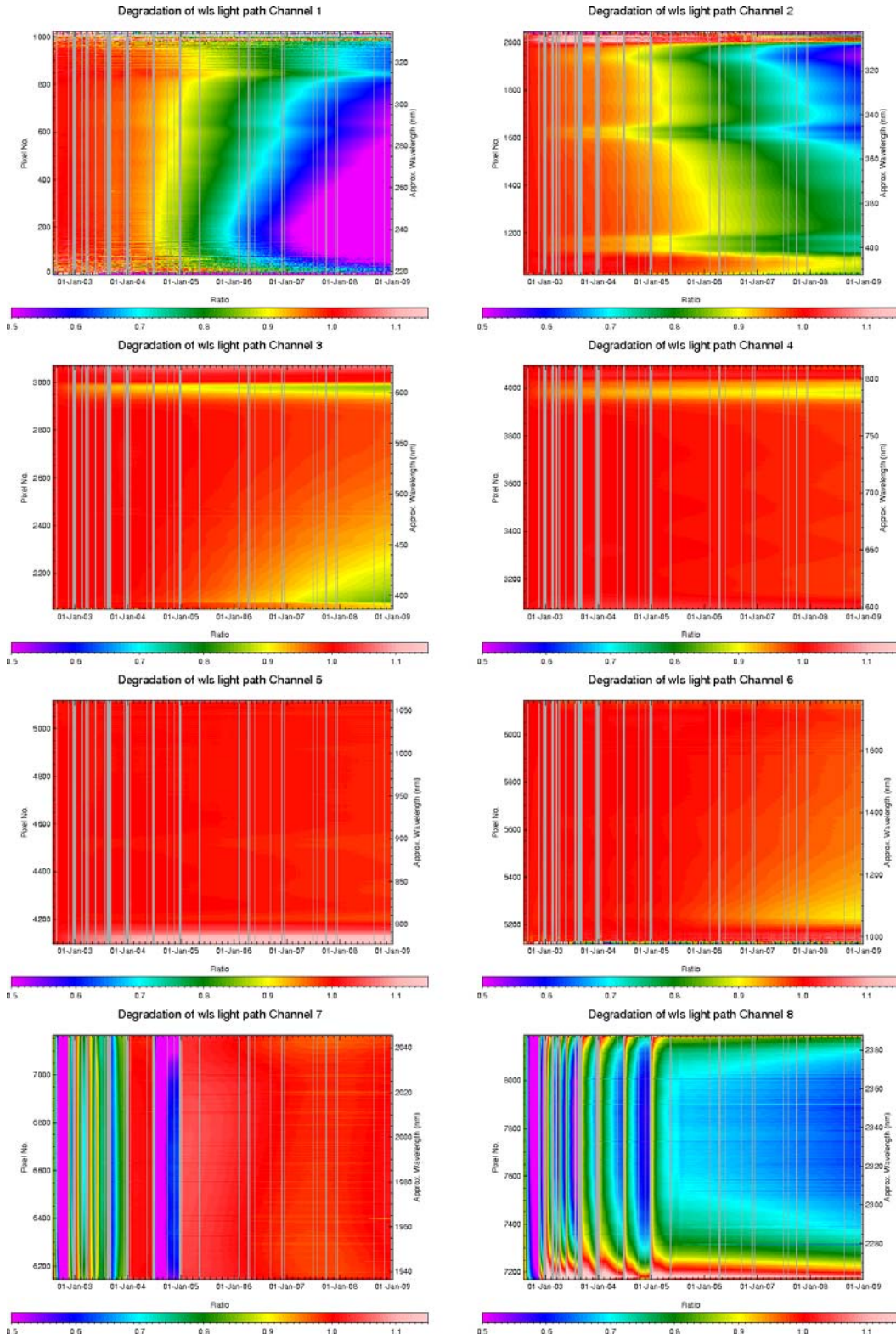
Fig. 3.11: Spectral light path monitoring results August 2002 to December 2008 (WLS light path)
