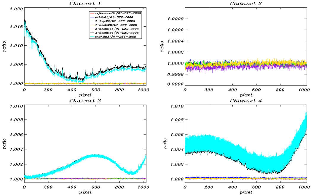
Fig. 5-10: dark current ratios (constant part) channel 1-4 during December 2008, Reference Spectrum used: Orbit 35316, 01-December 2008
