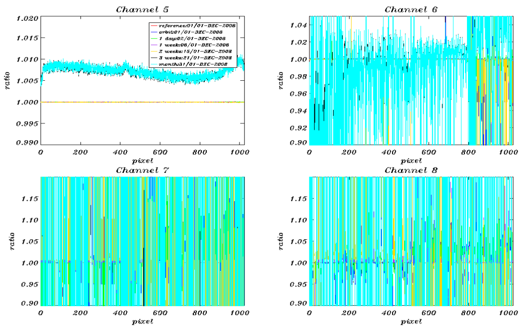
Fig. 5-11: dark current ratios (constant part) channel 5-8 during December 2008, Reference Spectrum used: Orbit 35316, 01-December-2008
