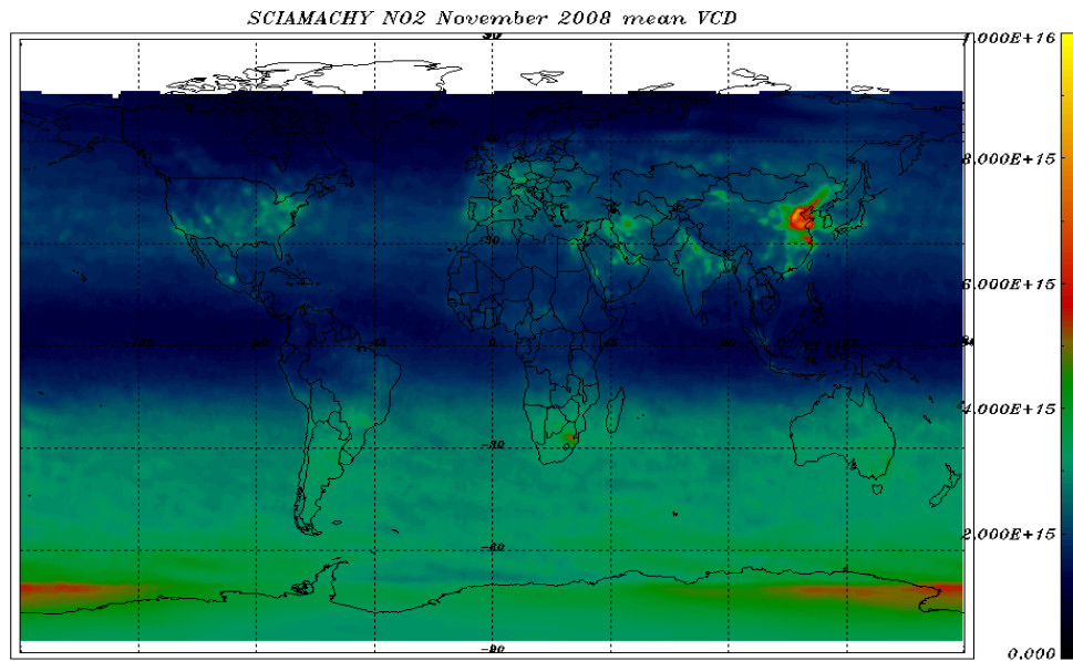
Figure 7-1: NO 2 VCD world map 01 - 30 November 2008 – monthly average
