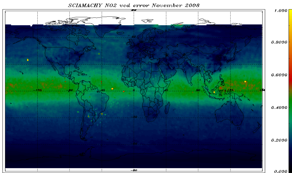
Figure 7-2: NO 2 VCD error 01-30 November 2008
