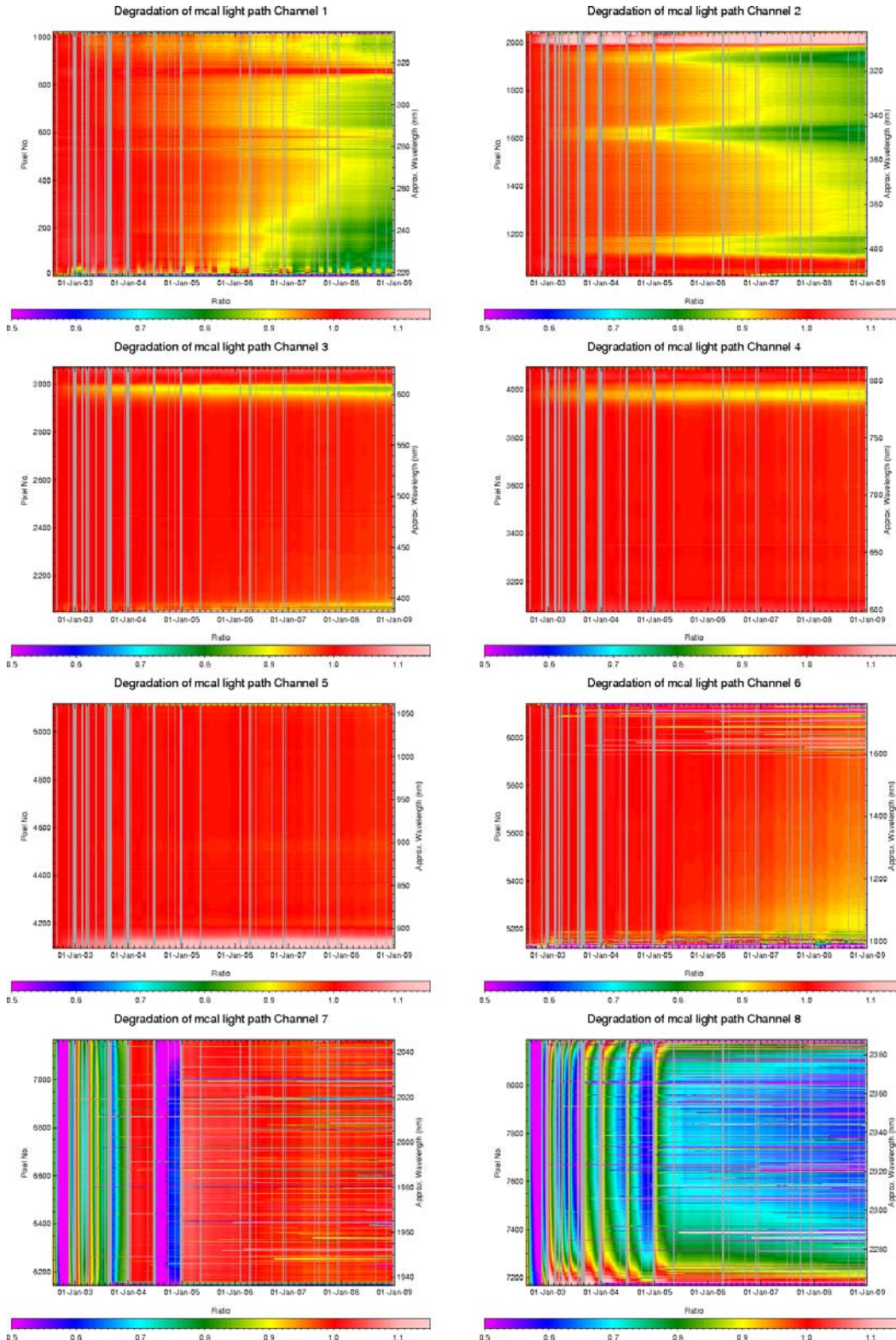
Fig. 3.10: Spectral light path monitoring results August 2002 to December 2008 (calibration light path)
