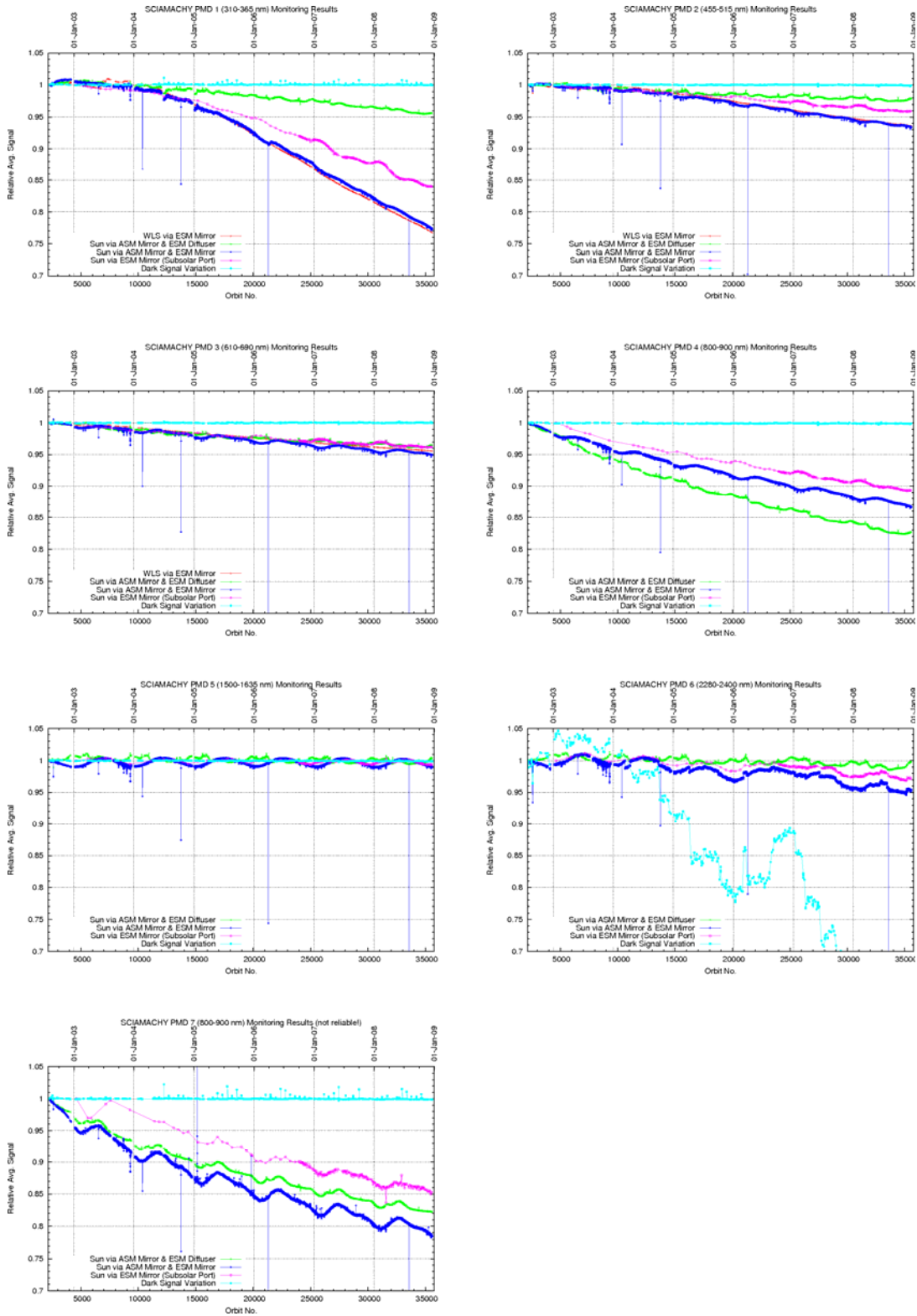
Fig. 3.12: PMD monitoring results August 2002 to December 2008
