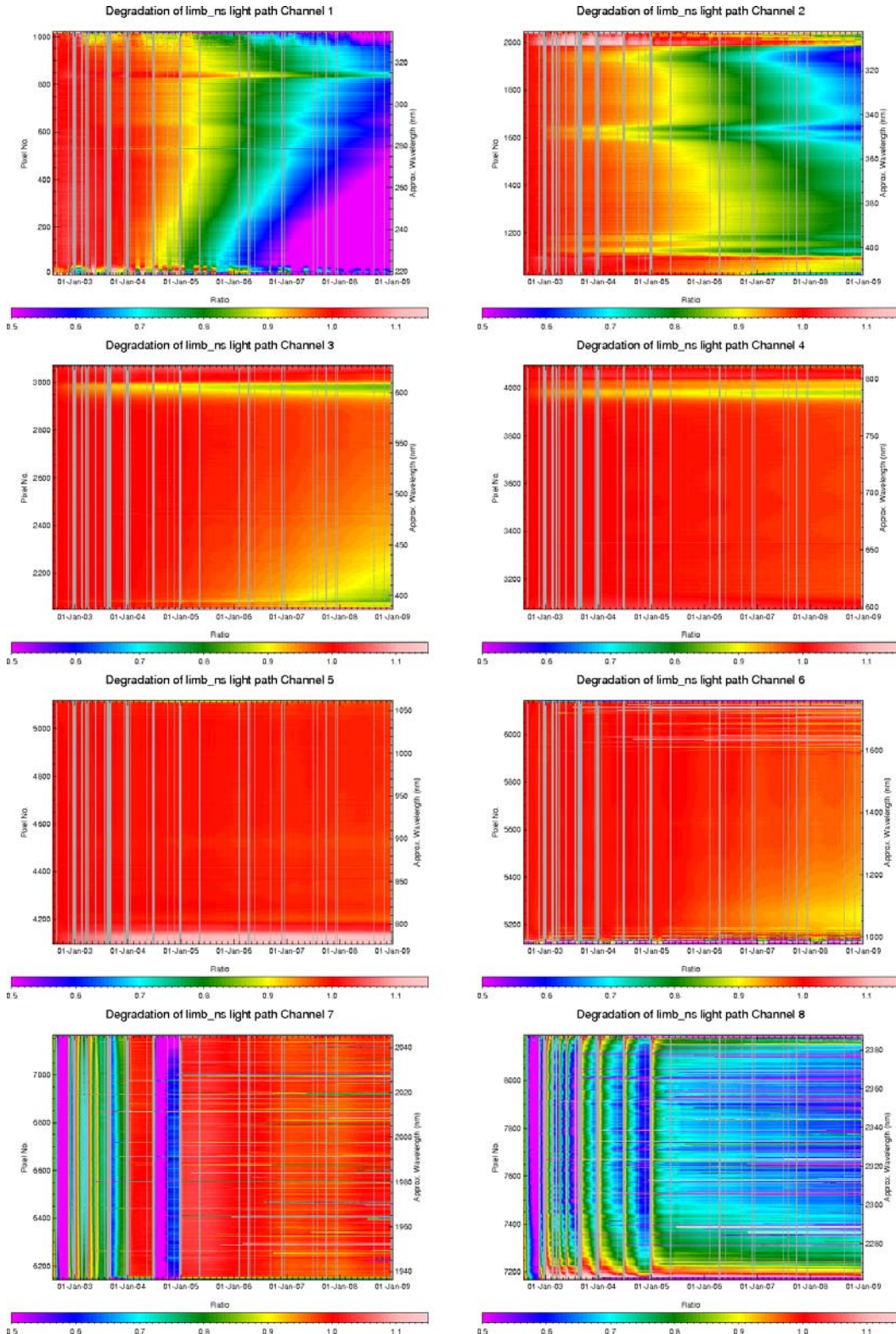
Fig. 3.9: Spectral light path monitoring results August 2002 to December 2008 (limb light path)
