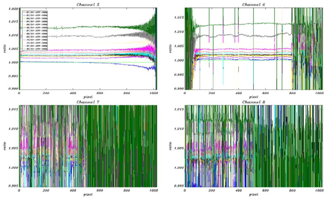
Fig. 5-3: SMR ratios per detector channel 5-8 (changes during November 2008)
