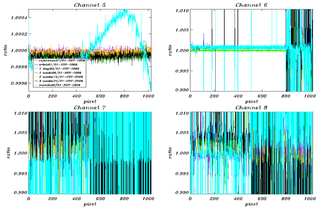
Fig. 5-9: dark current ratios (constant part) channel 5-8 during November 2008, Reference Spectrum used: Orbit 34887, 01-November-2008
