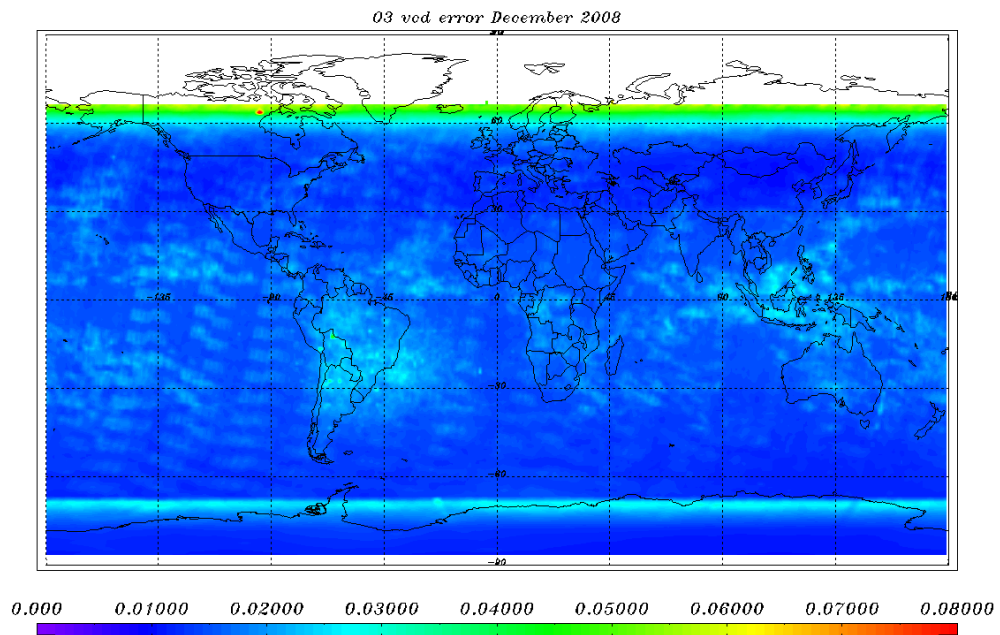
Figure 7-8: O 3 VCD error 01-31 December 2008
