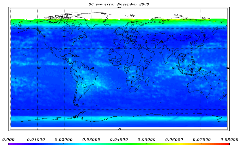
Figure 7-6: O 3 VCD error 01-30 November 2008
