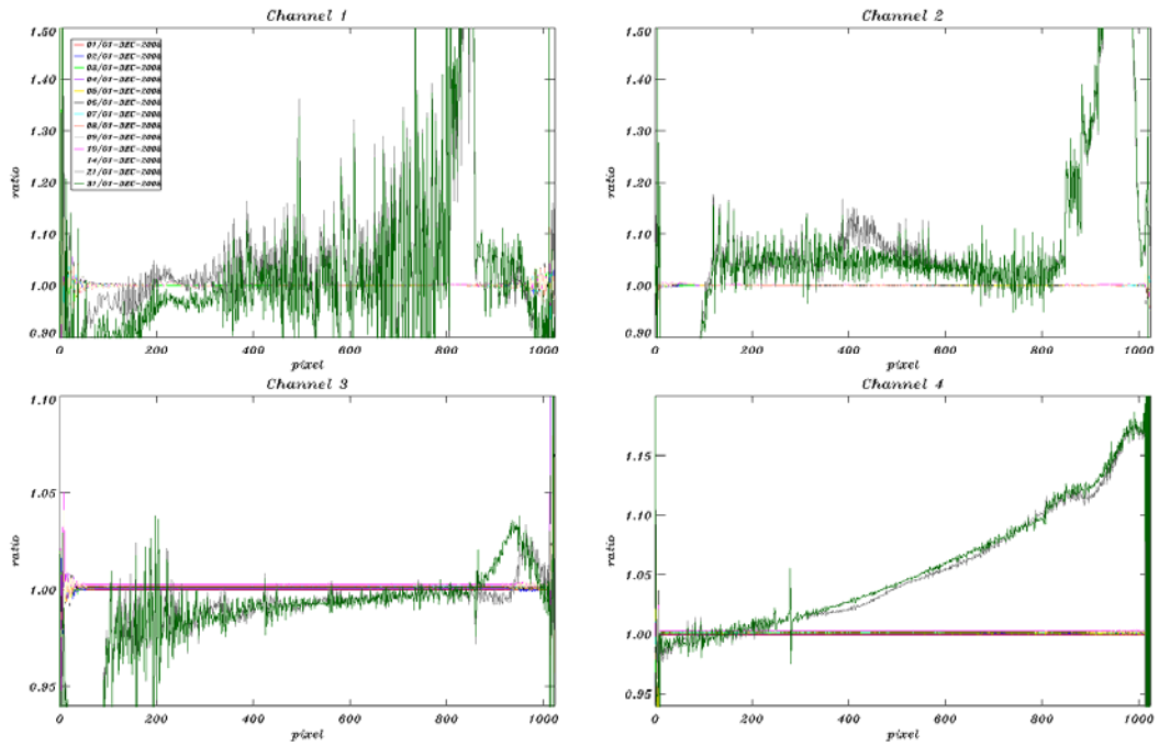
Fig. 5-4: SMR ratios per detector channel 1-4 (changes during December 2008)
