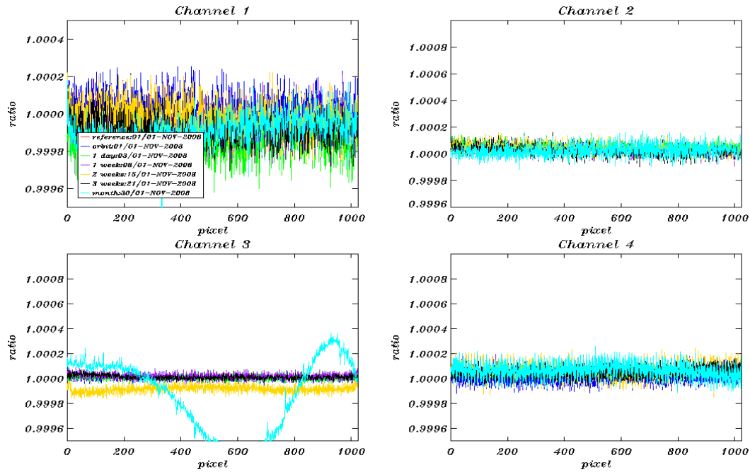
Fig. 5-8: dark current ratios (constant part) channel 1-4 during November 2008, Reference Spectrum used: Orbit 34887, 01-November-2008
