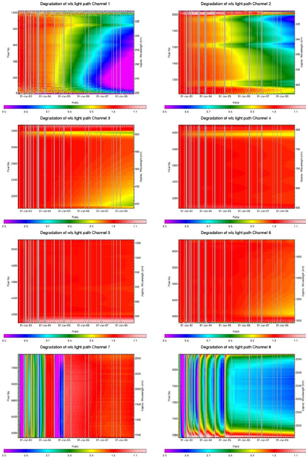
Fig. 3.11: Spectral light path monitoring results August 2002 to August 2008 (WLS light path)
