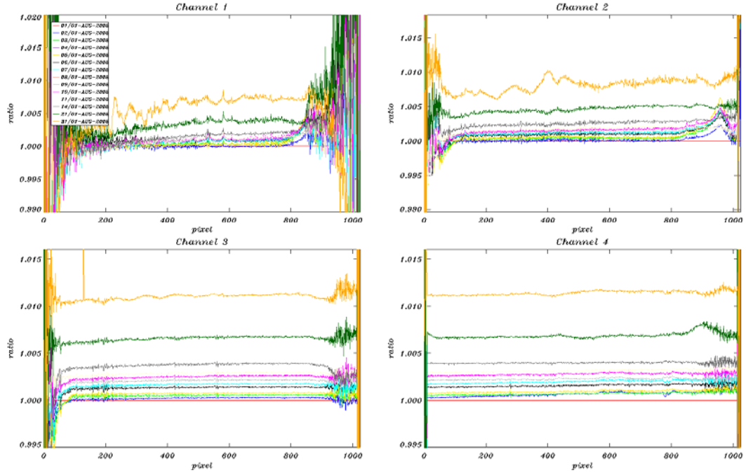
Fig. 5-4: SMR ratios per detector channel 1-4 (changes during August 2008)
