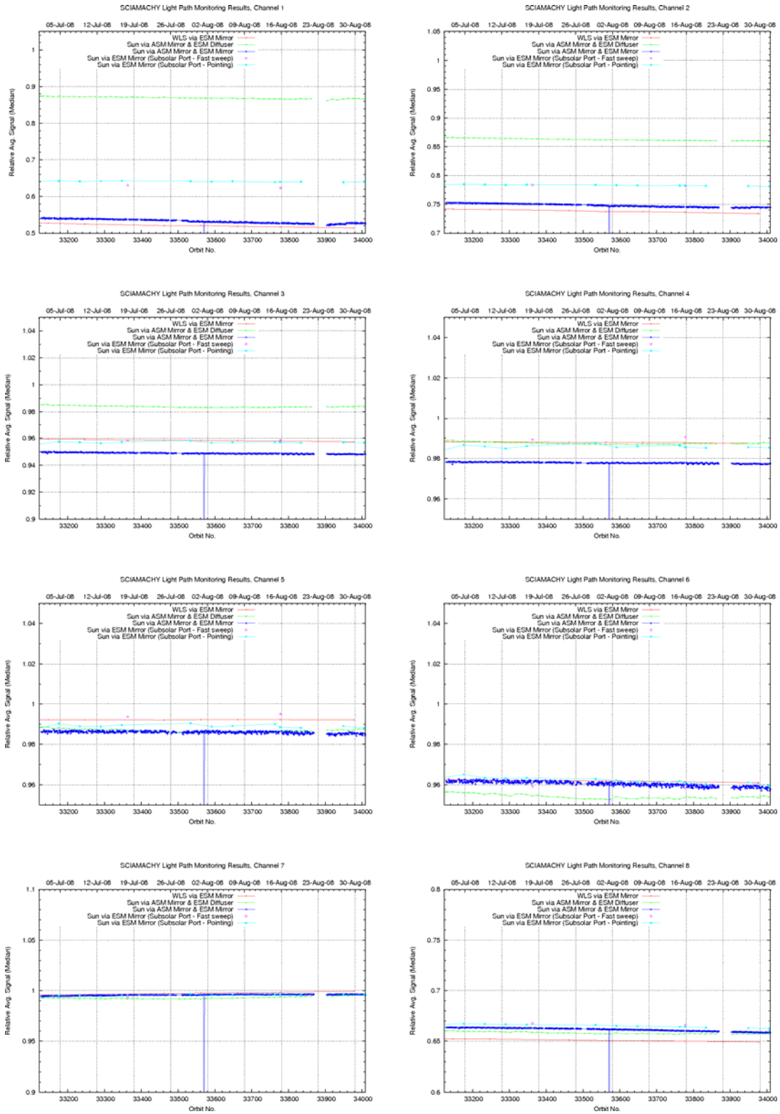
Fig. 3.7: Light path monitoring results July to August 2008 (medians).
