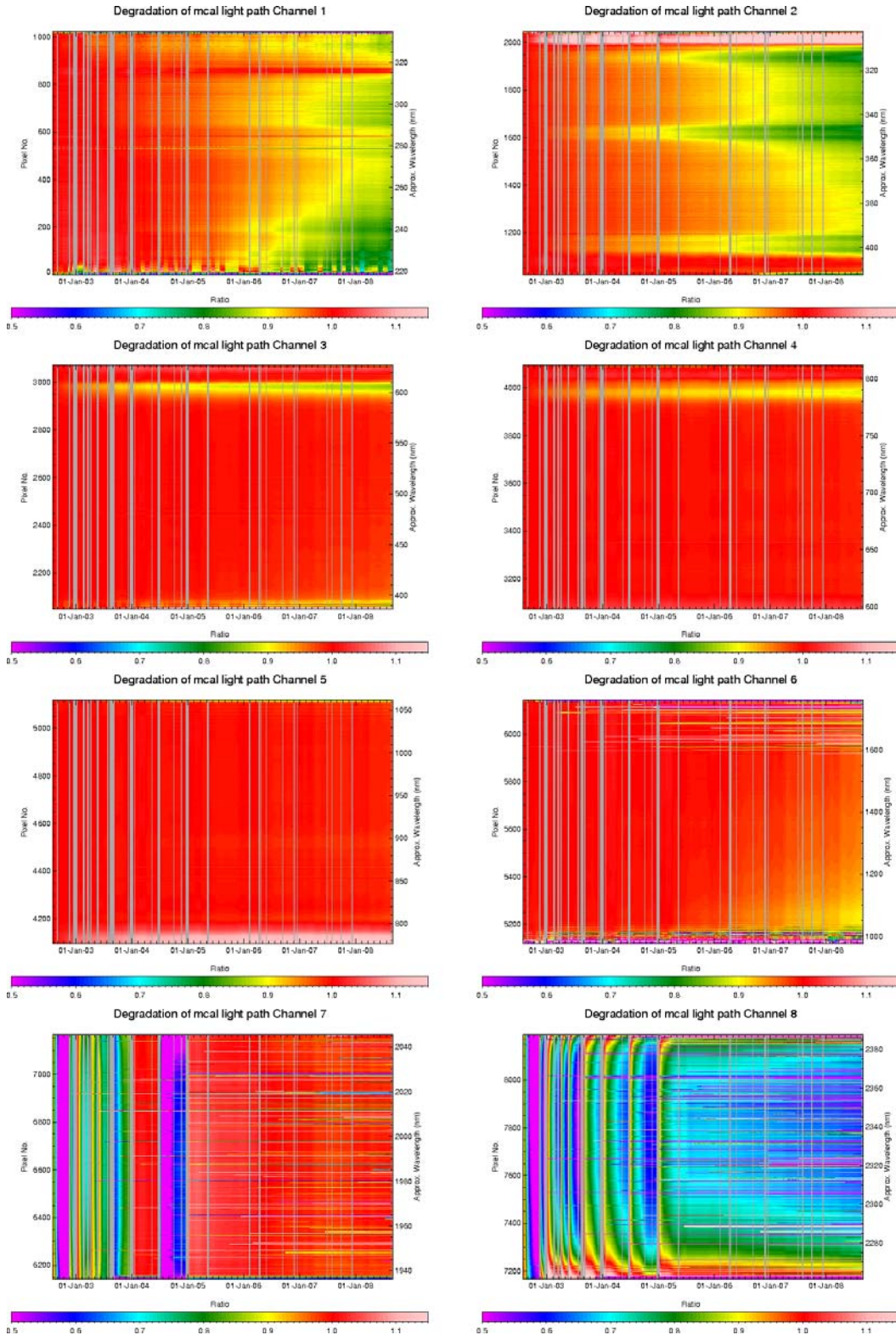
Fig. 3.10: Spectral light path monitoring results August 2002 to August 2008 (calibration light path)
