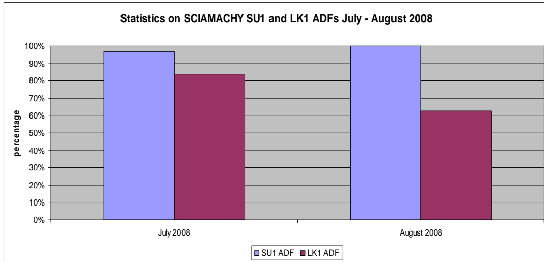
Fig. 5-1: Statistics on SU1 and LK1 processing
