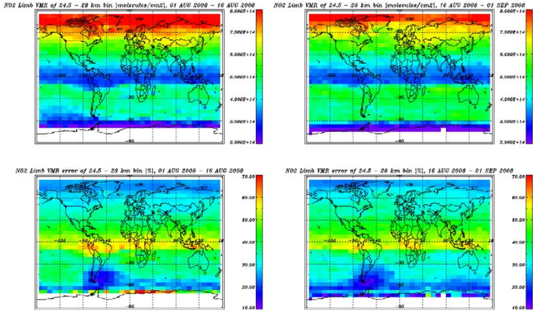
Figure 7-14 Limb NO 2 profiles binned over 24.5 - 28 km, August 2008
