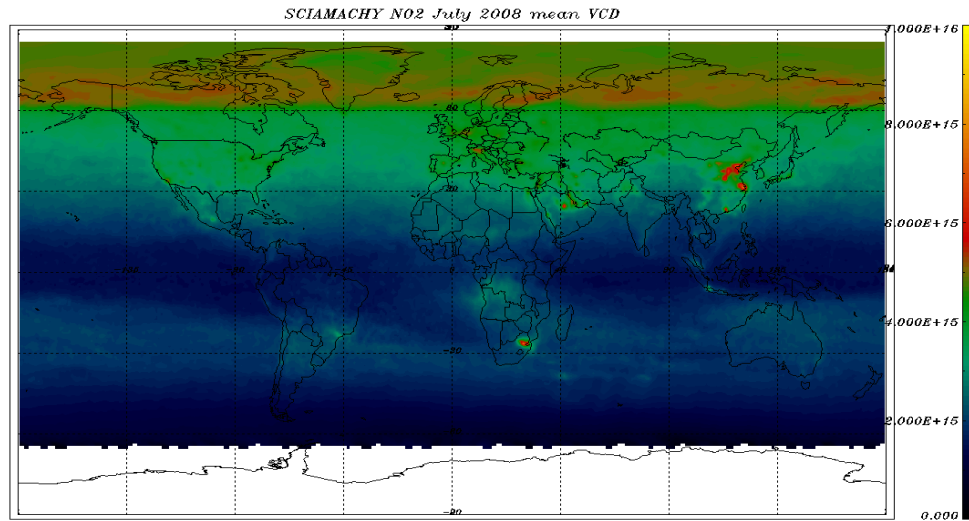
Figure 7-1: NO2 VCD world map 01 - 31 July 2008 – monthly average
