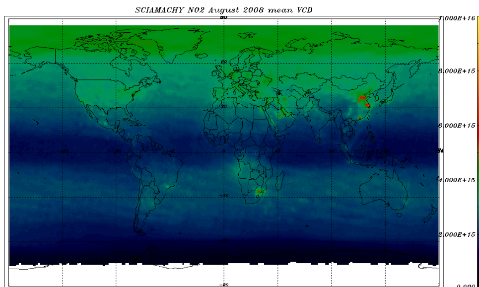
Figure 7-3: NO 2 VCD world map 01 – 31 August 2008 – monthly average
