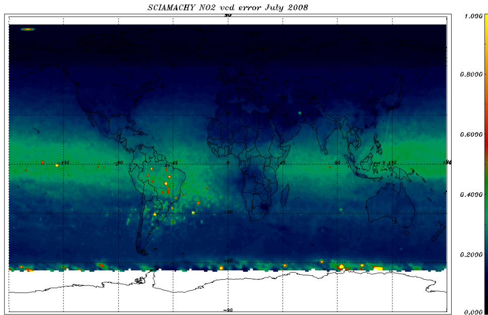
Figure 7-2: NO2 VCD error 01-31 July 2008
