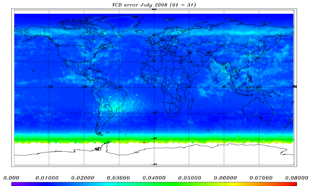
Figure 7-6: O 3 VCD error 01-31 July 2008
