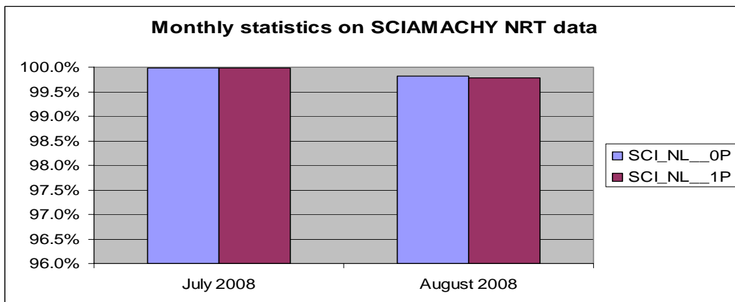
Fig. 4-1: Statistics on available unconsolidated level 0 and level 1b products
