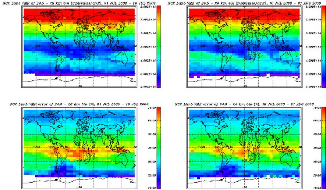
Figure 7-13 Limb NO 2 profiles binned over 24.5 - 28 km, July 2008
