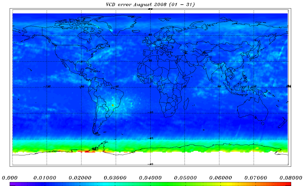
Figure 7-8: O 3 VCD error 01-31 August 2008
