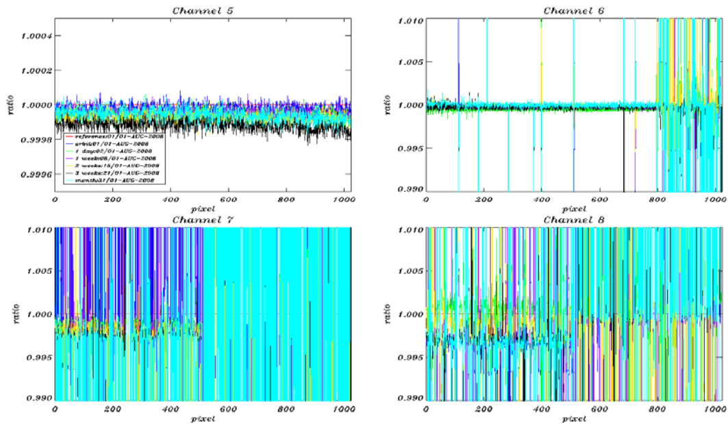
Fig. 5-11: dark current ratios (constant part) channel 5-8 during August 2008, Reference Spectrum used: Orbit 33570, 01-August-2008
