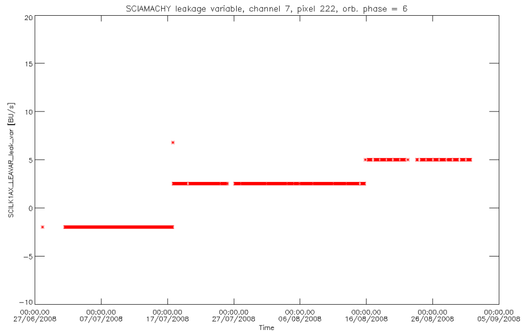
Figure 5-12: Leakage VARIABLE, SCI_LK1_AX, 01 July – 31 August 2008, channel 7, Orbit phase=6 pixel 222
