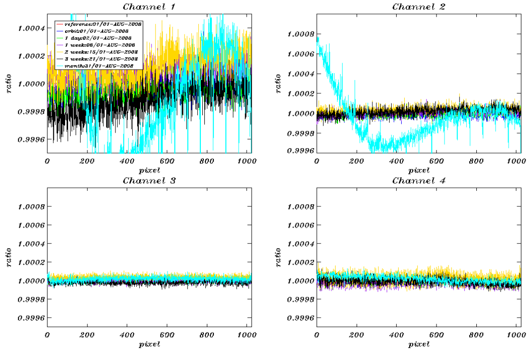
Fig. 5-10: dark current ratios (constant part) channel 1-4 during August 2008, Reference Spectrum used: Orbit 33570, 01-August 2008
