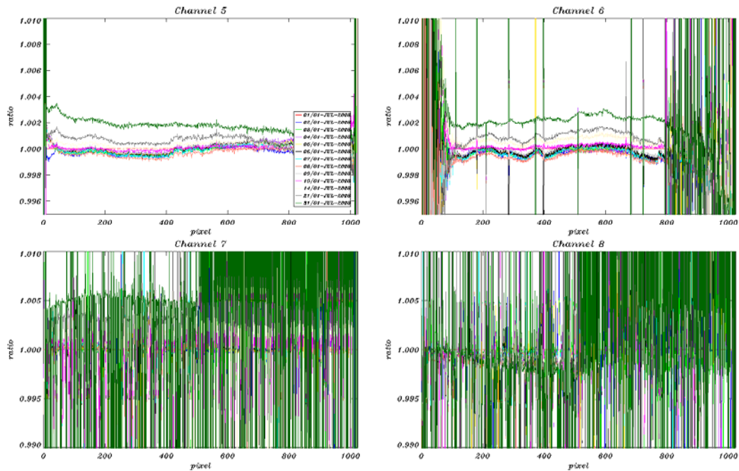
Fig. 5-3: SMR ratios per detector channel 5-8 (changes during July 2008)
