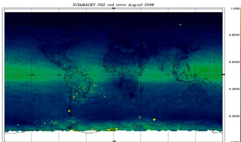
Figure 7-4: NO 2 VCD error 01 – 31 August 2008
