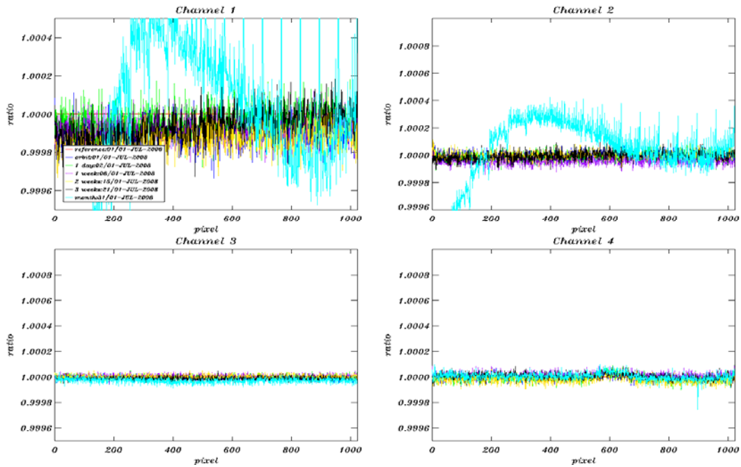
Fig. 5-8: dark current ratios (constant part) channel 1-4 during July 2008, Reference Spectrum used: Orbit 33129, 01-July-2008
