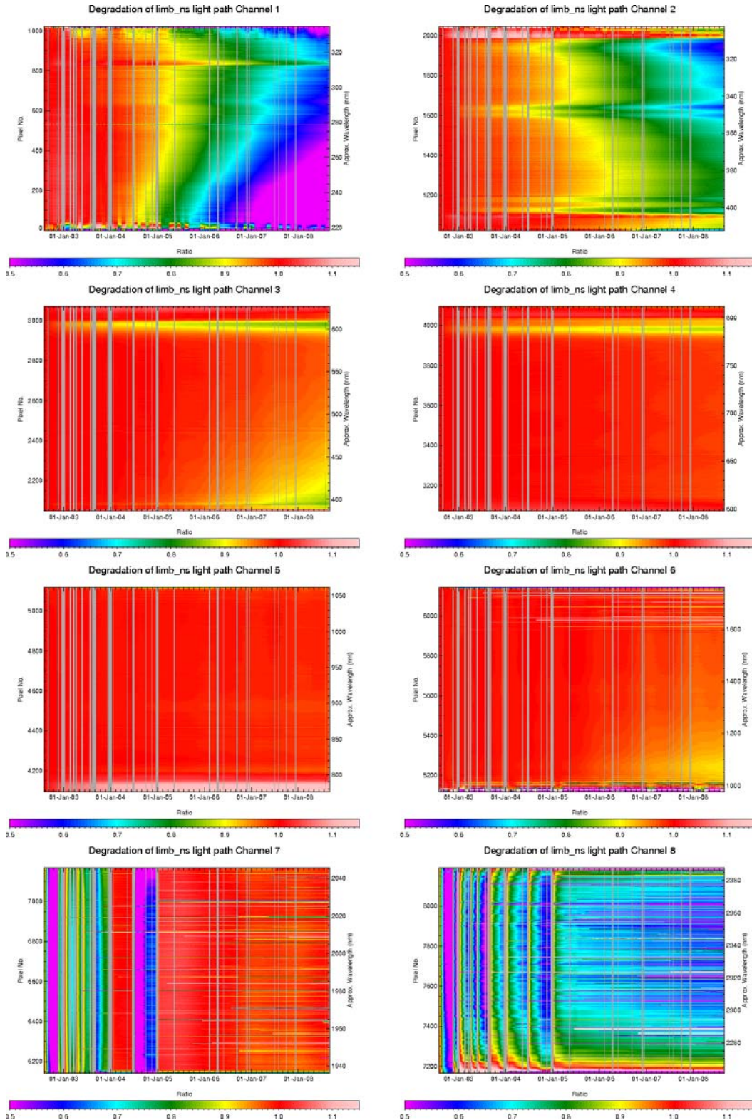
Fig. 3.9: Spectral light path monitoring results August 2002 to August 2008 (limb light path)
