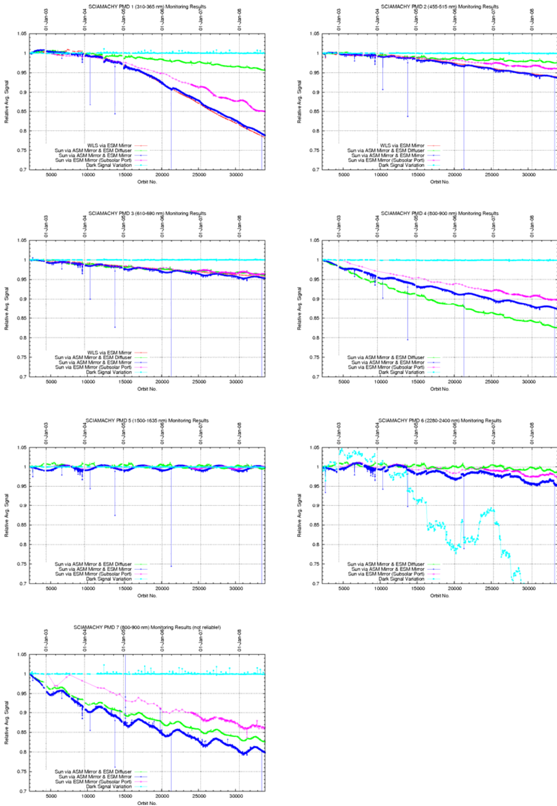
Fig. 3.12: PMD monitoring results August 2002 to August 2008
