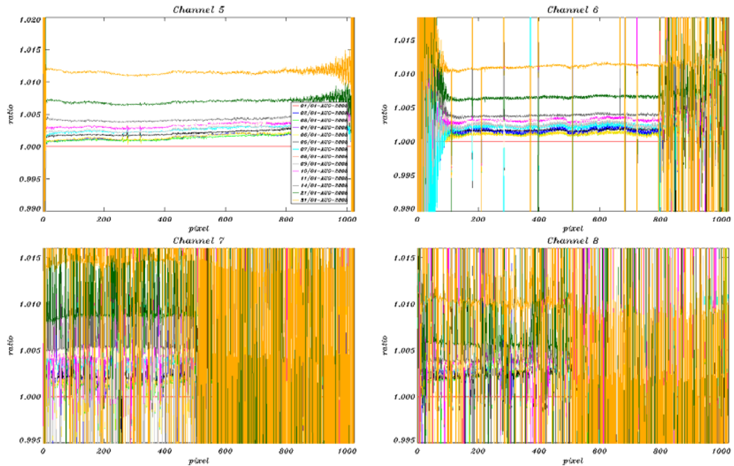
Fig. 5-5: SMR ratios per detector channel 5-8 (changes during August 2008)
