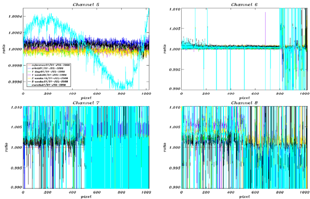
Fig. 5-9: dark current ratios (constant part) channel 5-8 during July 2008, Reference Spectrum used: Orbit 33129, 01-July-2008
