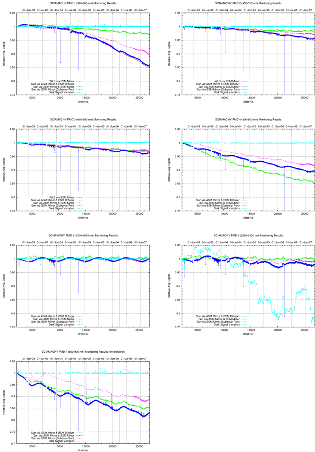
Fig. 3.12: PMD monitoring results August 2002 to April 2007
