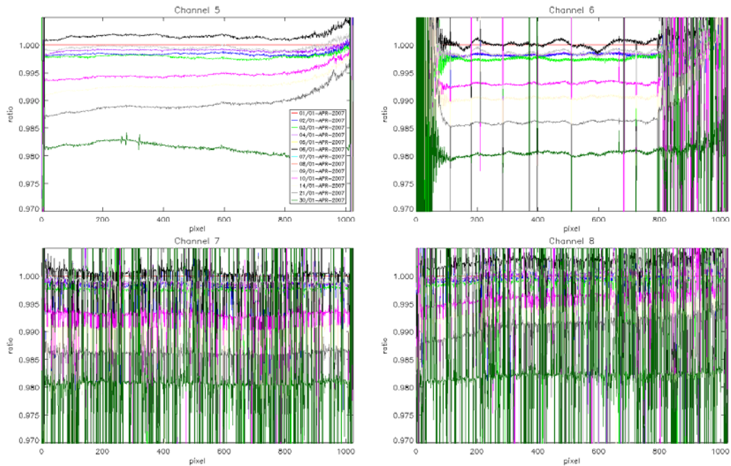
Fig. 5-5: SMR ratios per detector channel 5-8 (changes during April 2007)
