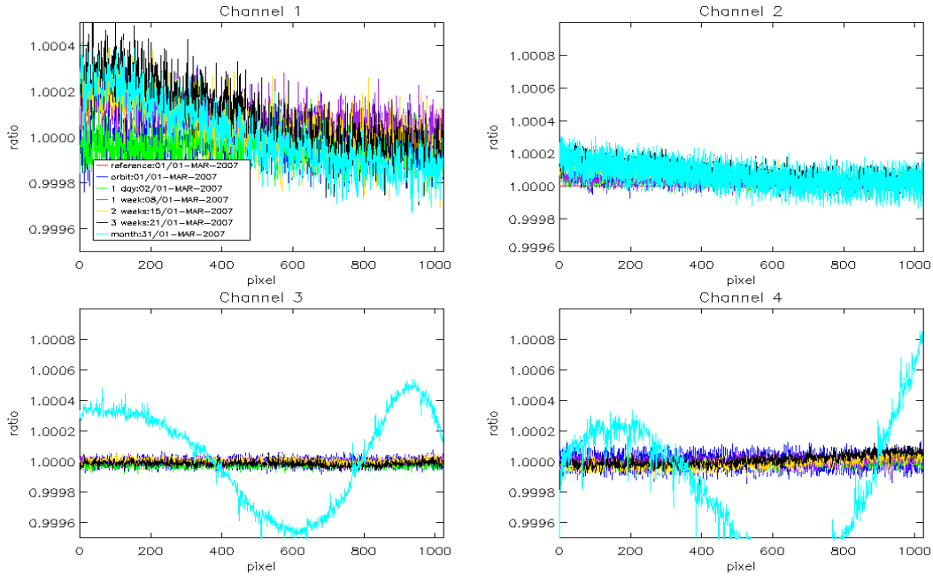
Fig. 5-8: dark current ratios (constant part) channel 1-4 during March 2007, Reference Spectrum used: Orbit 26141, 01-March-2007
