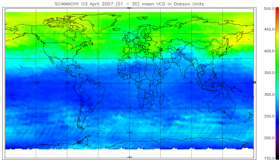
Figure 7-7: O 3 VCD world map 01-30 April 2007 – monthly average
