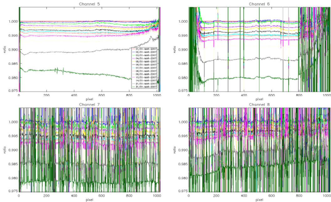
Fig. 5-3: SMR ratios per detector channel 5-8 (changes during March 2007)
