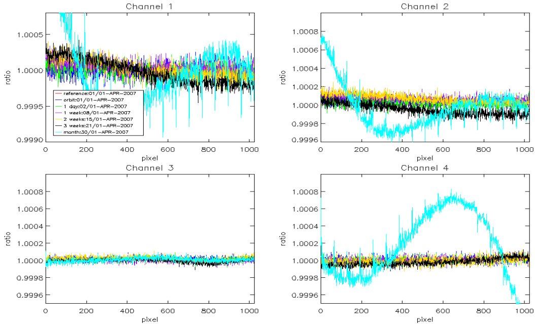
Fig. 5-10: dark current ratios (constant part) channel 1-4 during April 2007, Reference Spectrum used: Orbit 26584, 01-April 2007
