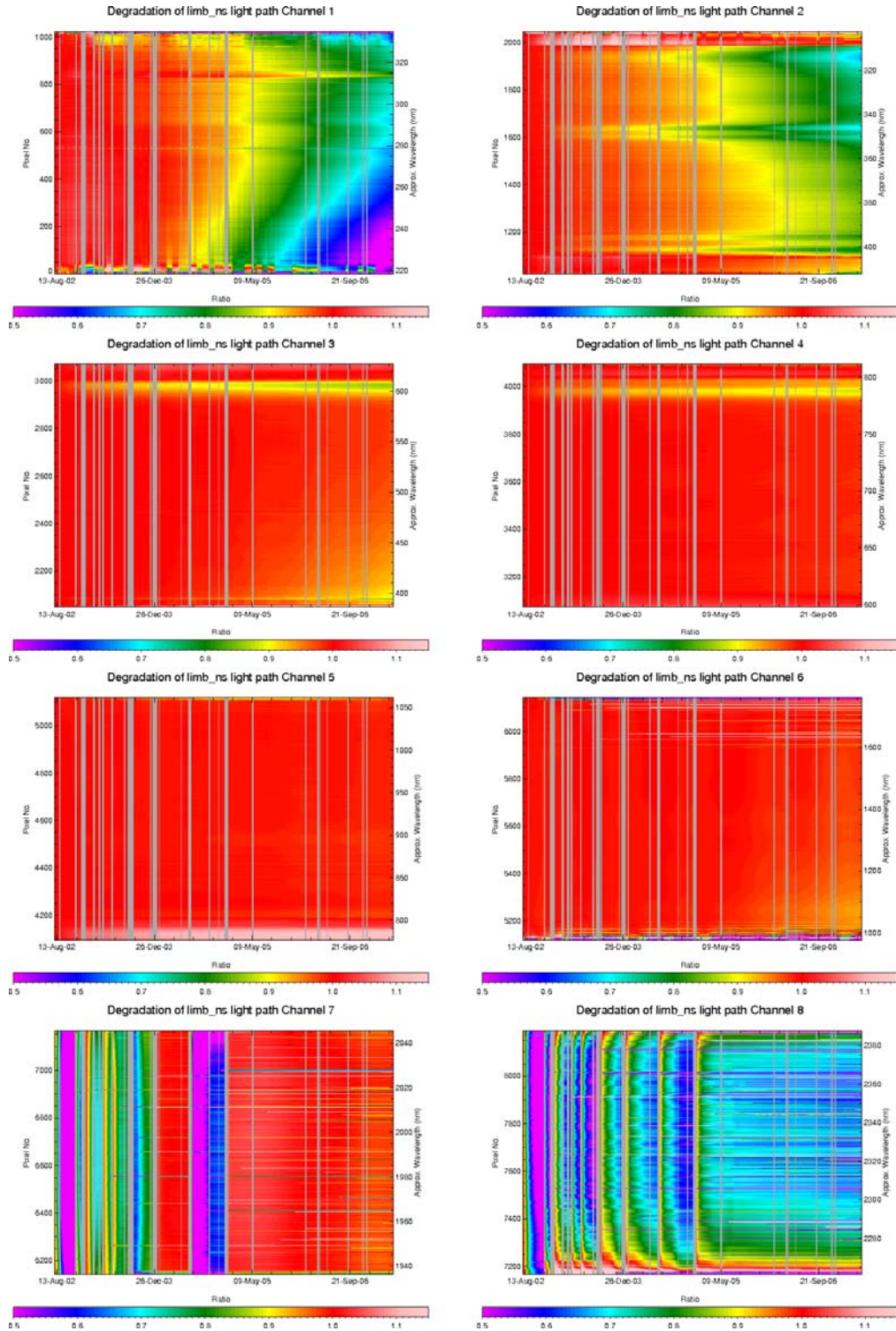
Fig. 3.9: Spectral light path monitoring results August 2002 to April 2007 (limb light path)
