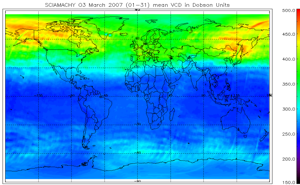
Figure 7-5: O 3 VCD world map 01-31 March 2007 – monthly average
