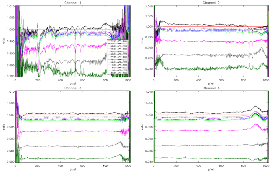
Fig. 5-4: SMR ratios per detector channel 1-4 (changes during April 2007)
