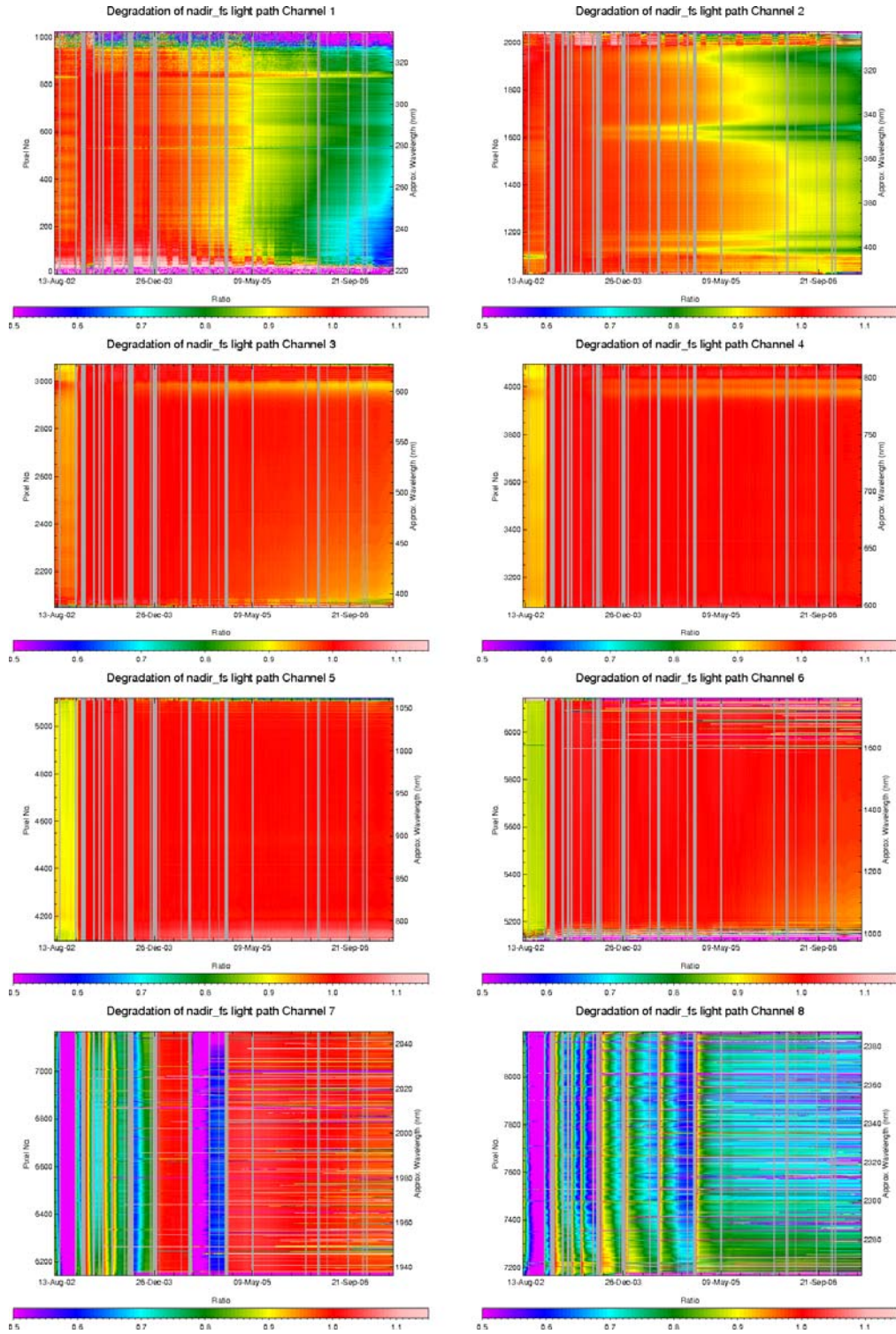
Fig. 3.8: Spectral light path monitoring results August 2002 to April 2007 (nadir light path)
