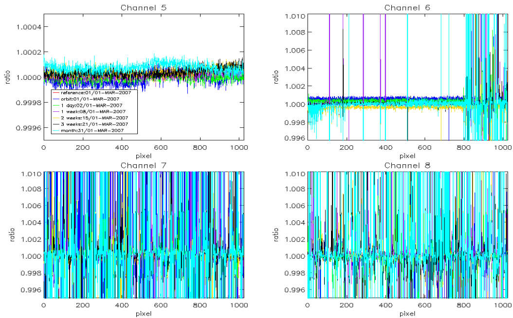
Fig. 5-9: dark current ratios (constant part) channel 5-8 during March 2007, Reference Spectrum used: Orbit 26141, 01-March-2007
