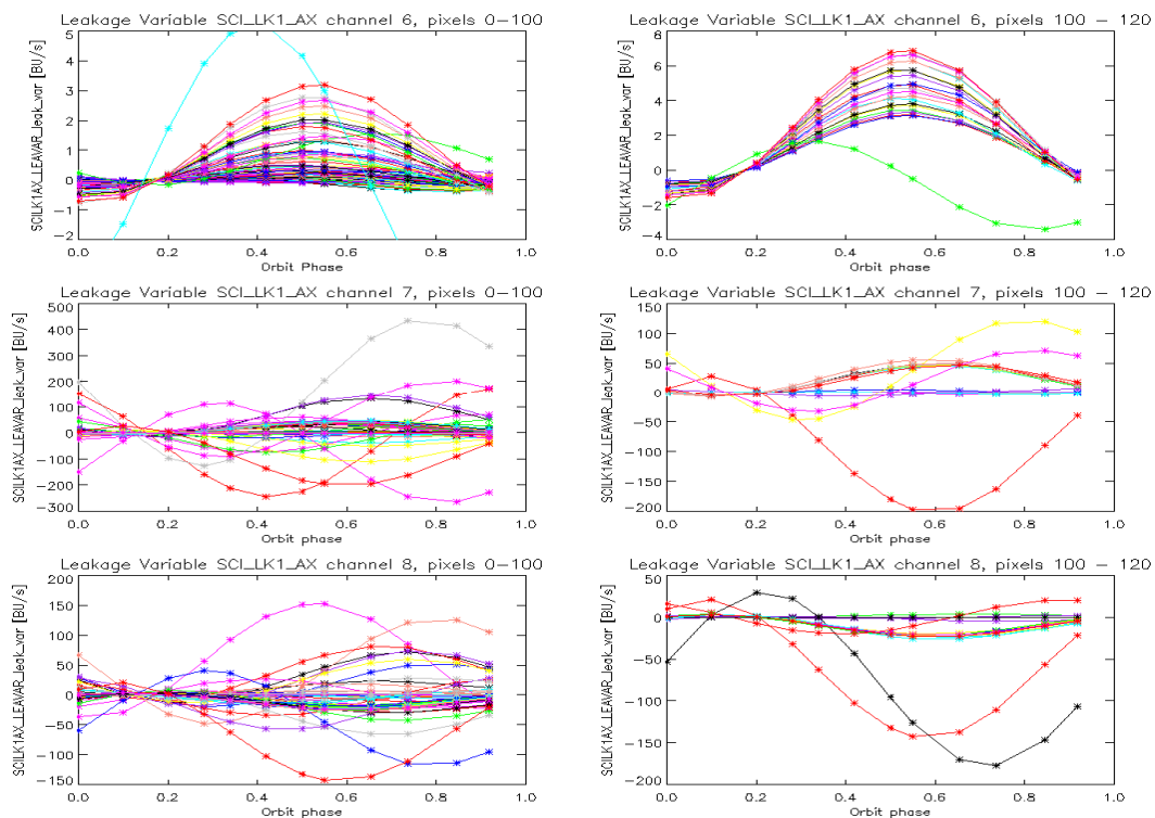
Figure 5-12: Example on leakage variation, SCI_LK1_AX 31 December 2006
