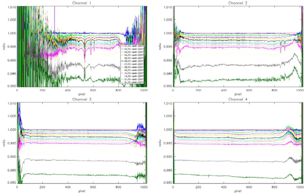
ratio of smrs as a function of pixel, March 2007
