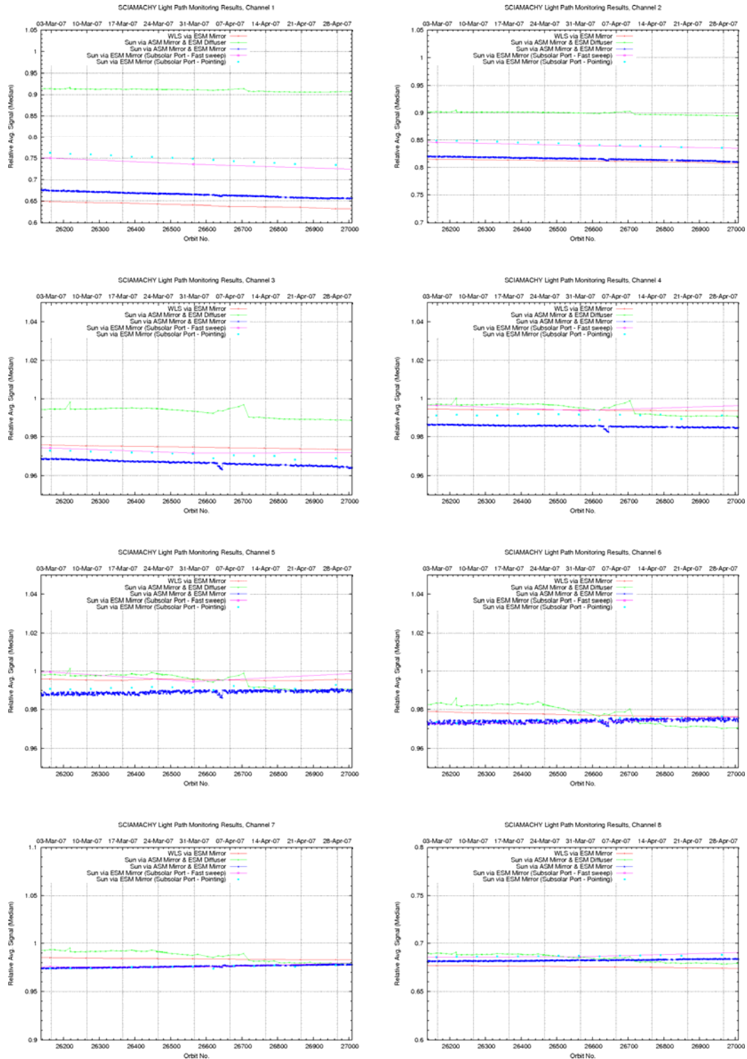
Fig. 3.7: Light path monitoring results March to April 2007 (medians).
