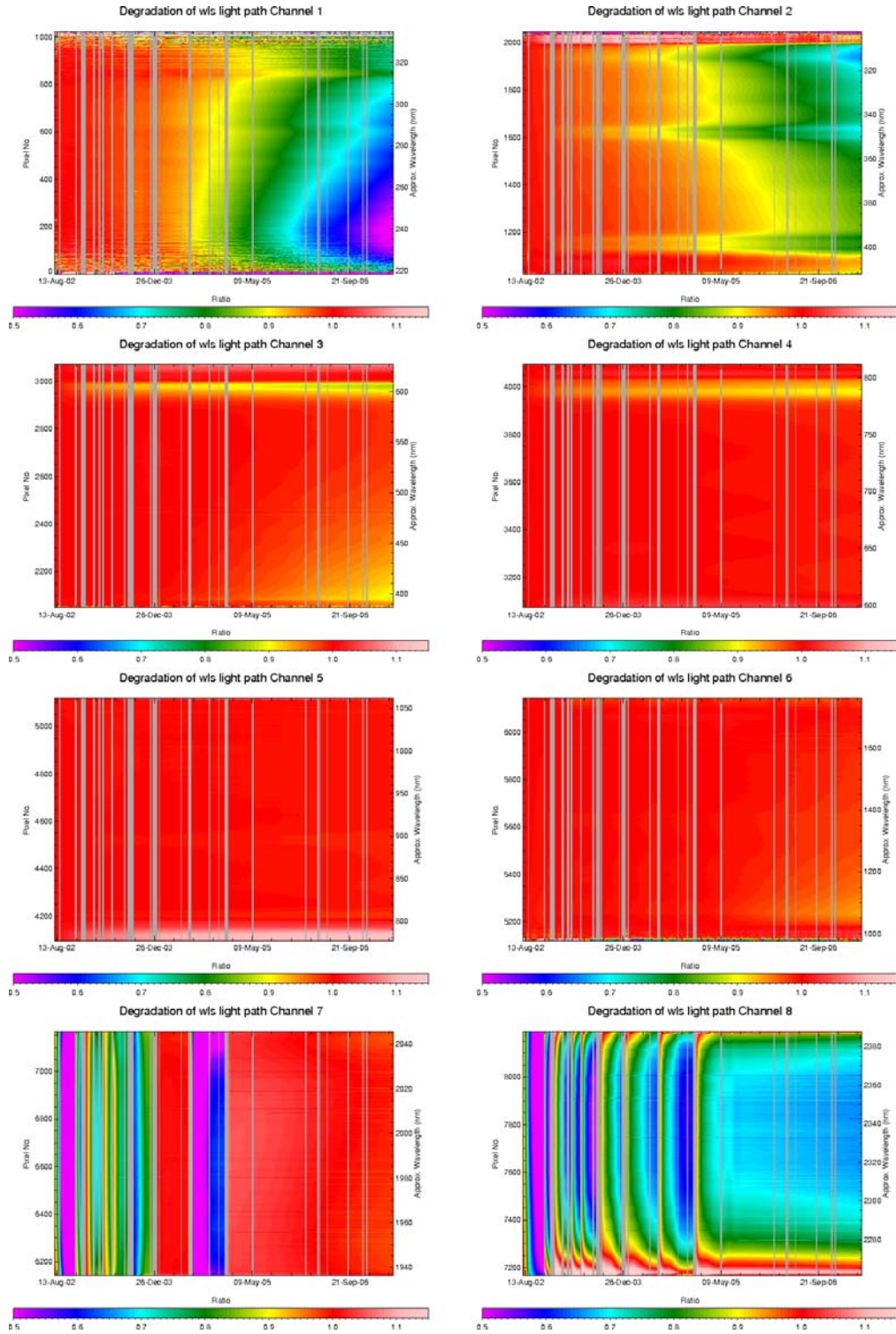
Fig. 3.11: Spectral light path monitoring results August 2002 to April 2007 (WLS light path)
