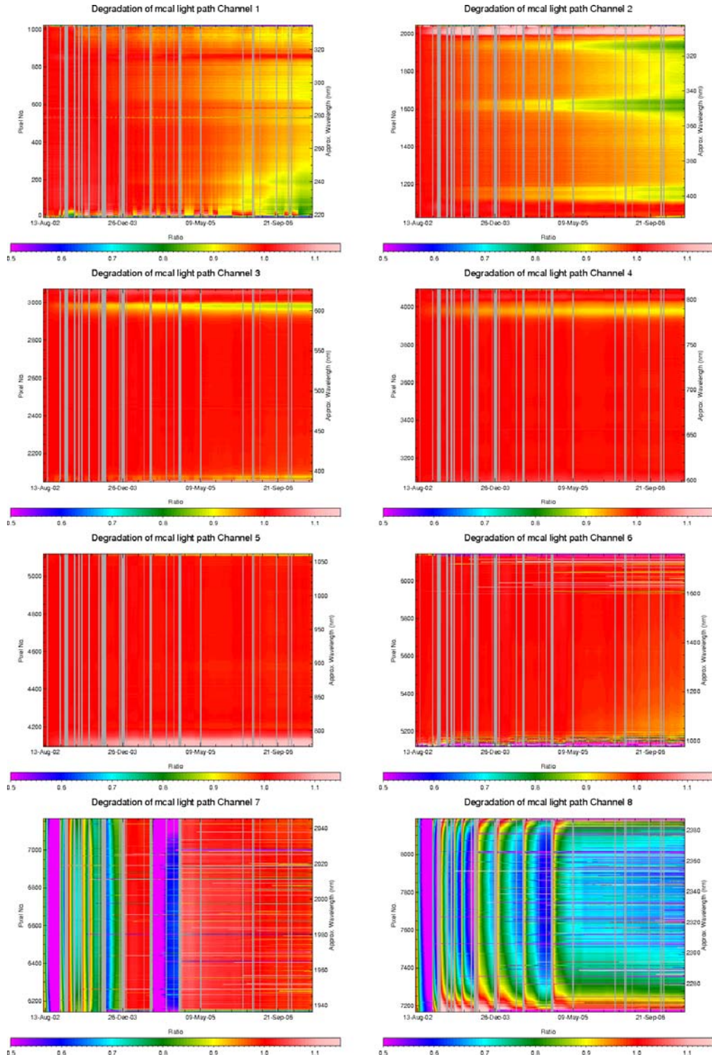
Fig. 3.10: Spectral light path monitoring results August 2002 to April 2007 (calibration light path)
