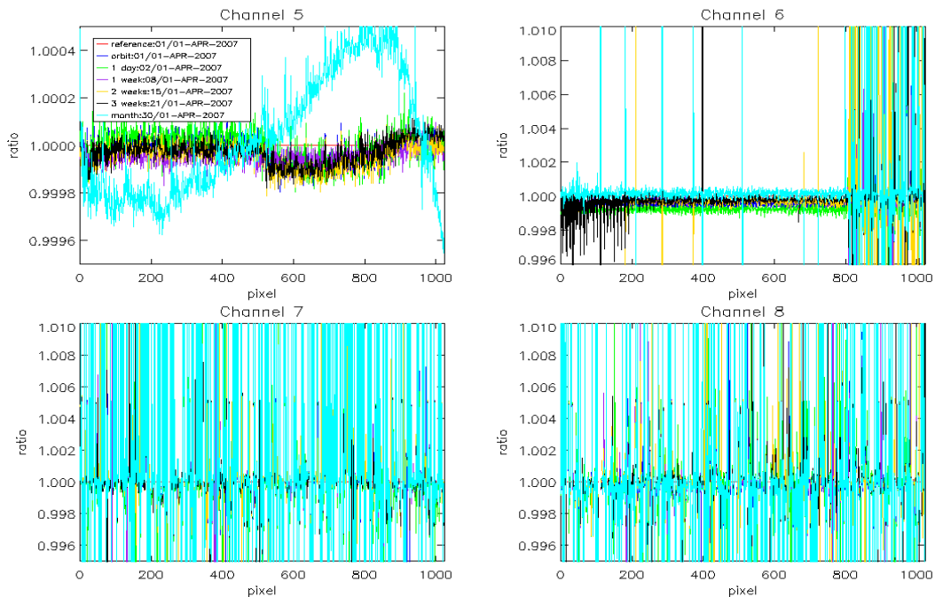
Fig. 5-11: dark current ratios (constant part) channel 5-8 during April 2007, Reference Spectrum used: Orbit 26584, 01-April-2007
