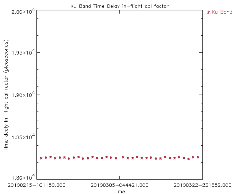
Figure 14: Ku Band in-flight time delay calibration factor for cycle 87 (averaged per day)
