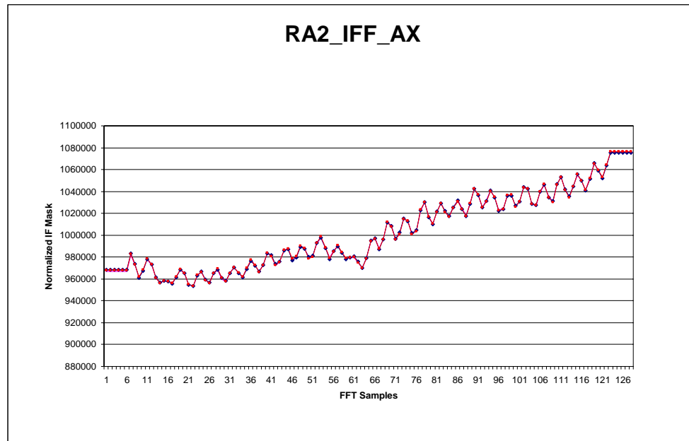
Figure 6: Previous and IF Mask updated on 4 th March 2010.
