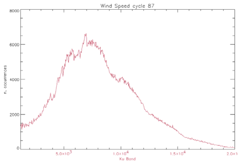
Figure 33: Histogram of Ku Wind Speed for cycle 87 (mm/sec)
