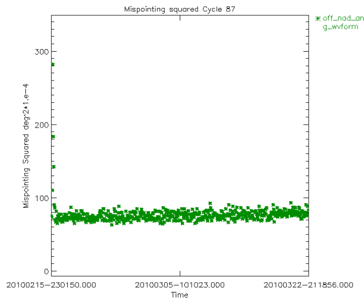
Figure 19: Smoothed mispointing squared trend for cycle 87 ( \text{deg}^2 \cdot 10^{-4} )
