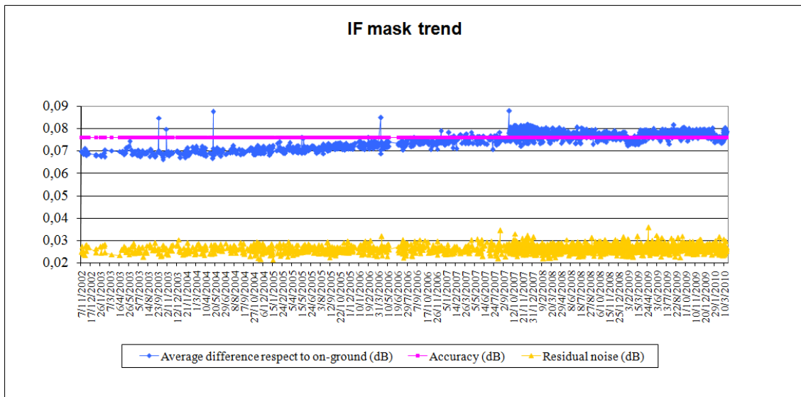
Figure 7: Evolution of the IF mask related parameters for valid IF masks retrieved up to cycle 87
