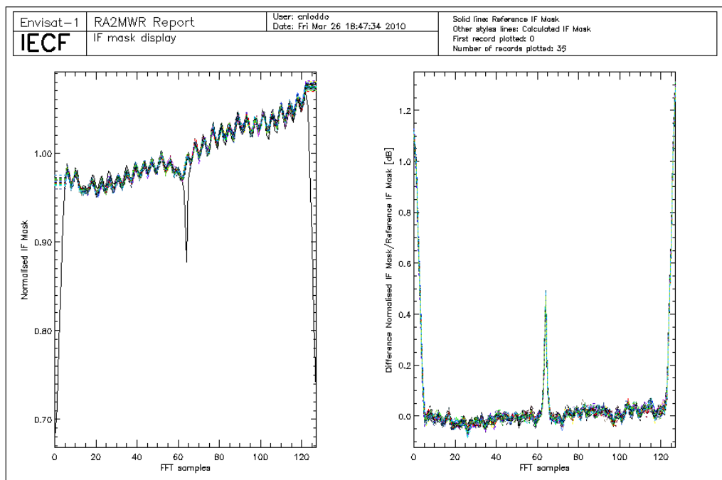
Figure 5: Valid IF masks retrieved during cycle 87 plotted together with the on-ground reference.
