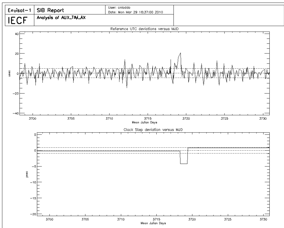
Figure 11: UTC deviations and ICU clock period for cycle 87
