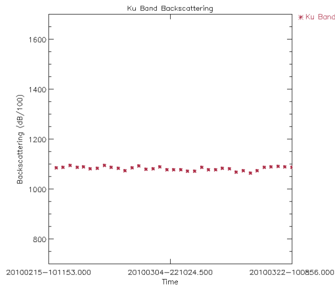
Figure 32: Ku Band Sigma_0 daily average for cycle 87 (dB/100)
