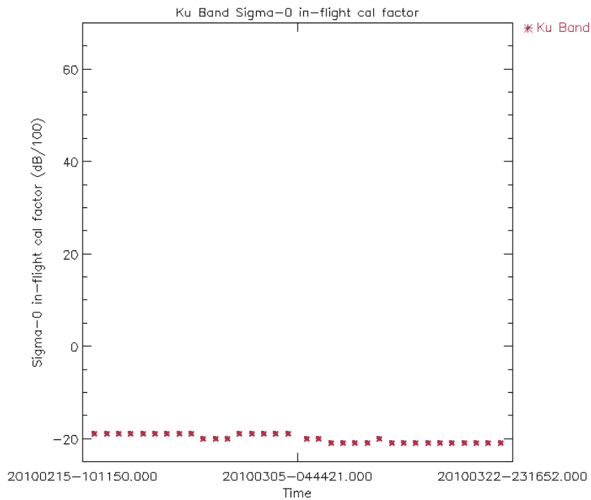
Figure 15: Ku Band in-flight Sigma0 calibration factor for cycle 87 (averaged per day)
