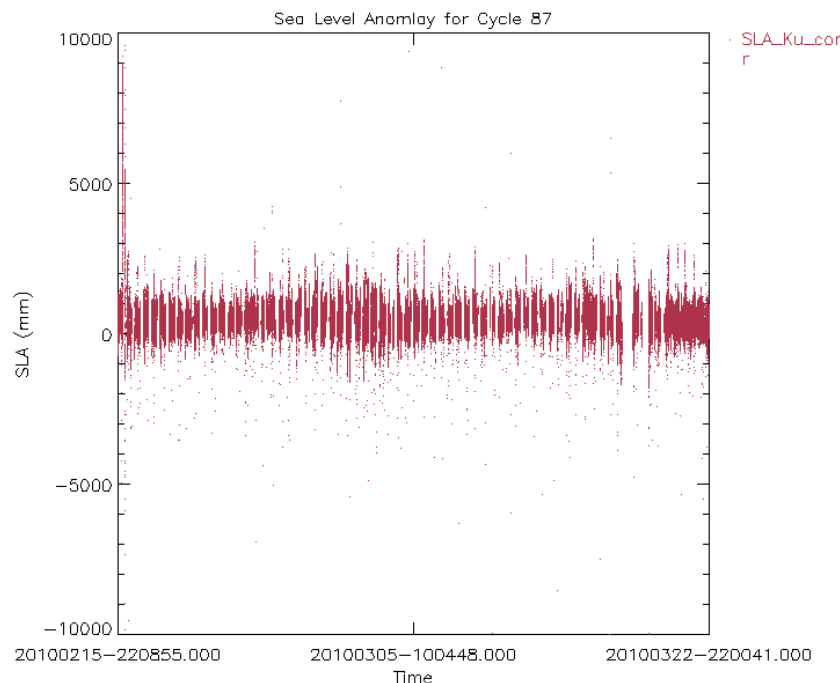
Figure 27A: Sea Level Anomalies Cycle 87 only MDSRs with valid DORIS Flag
