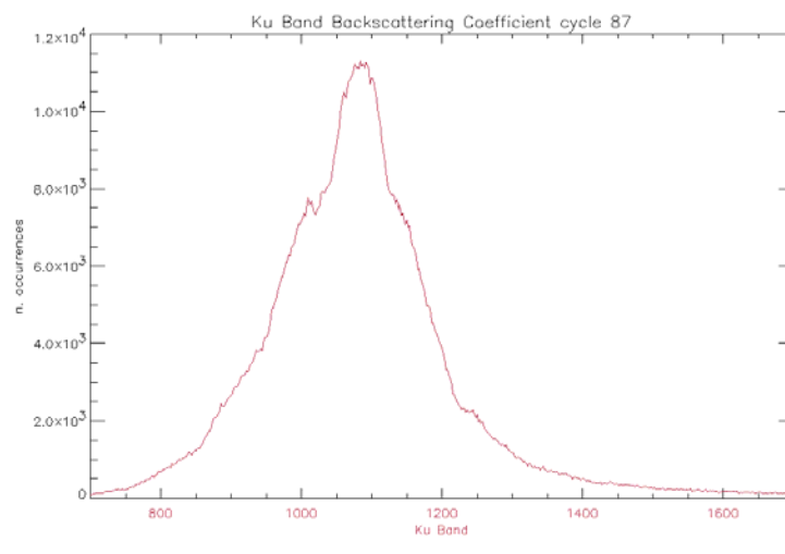
Figure 31: Histogram of Ku Band Backscattering Coefficient for cycle 87
