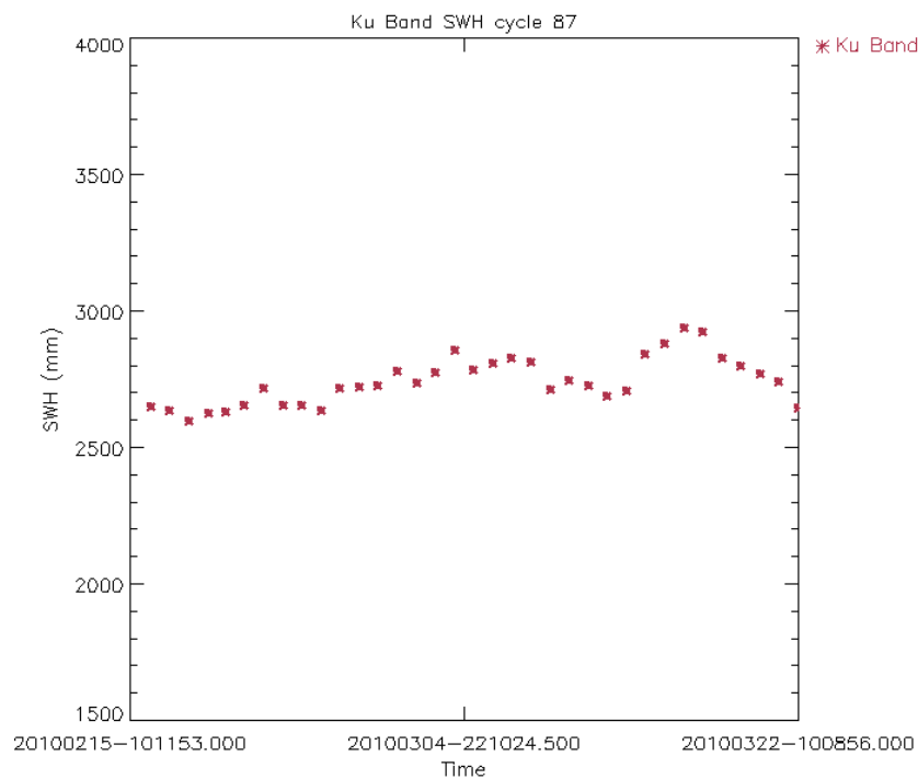
Figure 29: Ku Band SWH daily average for Cycle 87 (mm)
