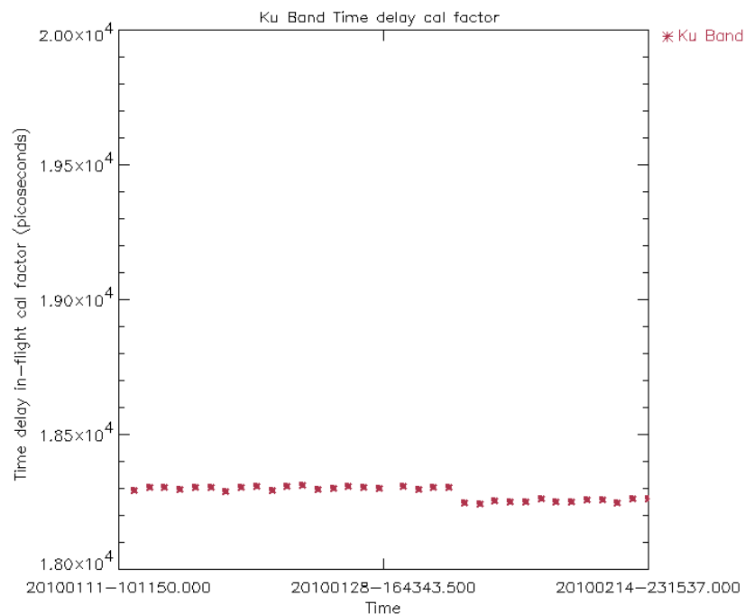
Figure 14: Ku Band in-flight time delay calibration factor for cycle 86 (averaged per day)
