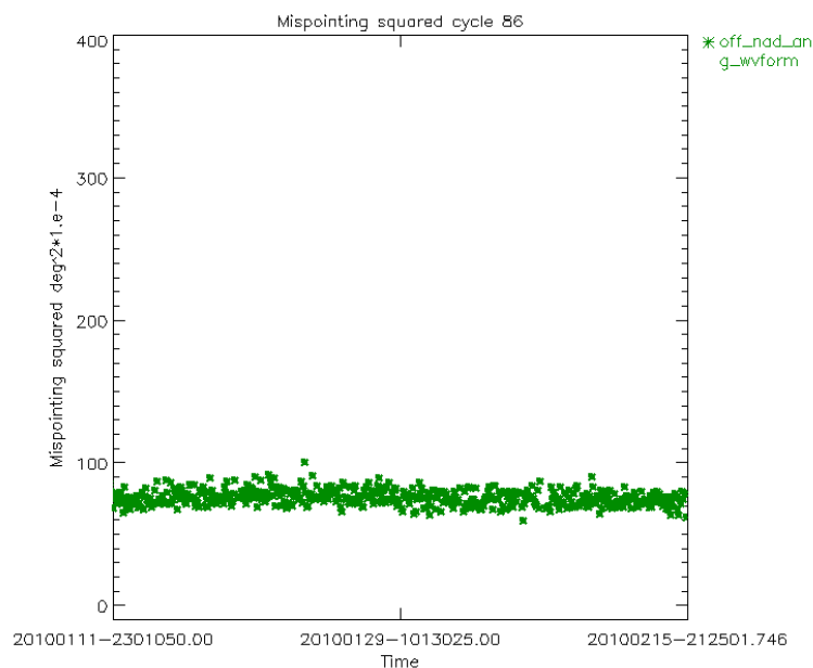
Figure 19: Smoothed mispointing squared trend for cycle 86 ( \text{deg}^2 \cdot 10^{-4} )
