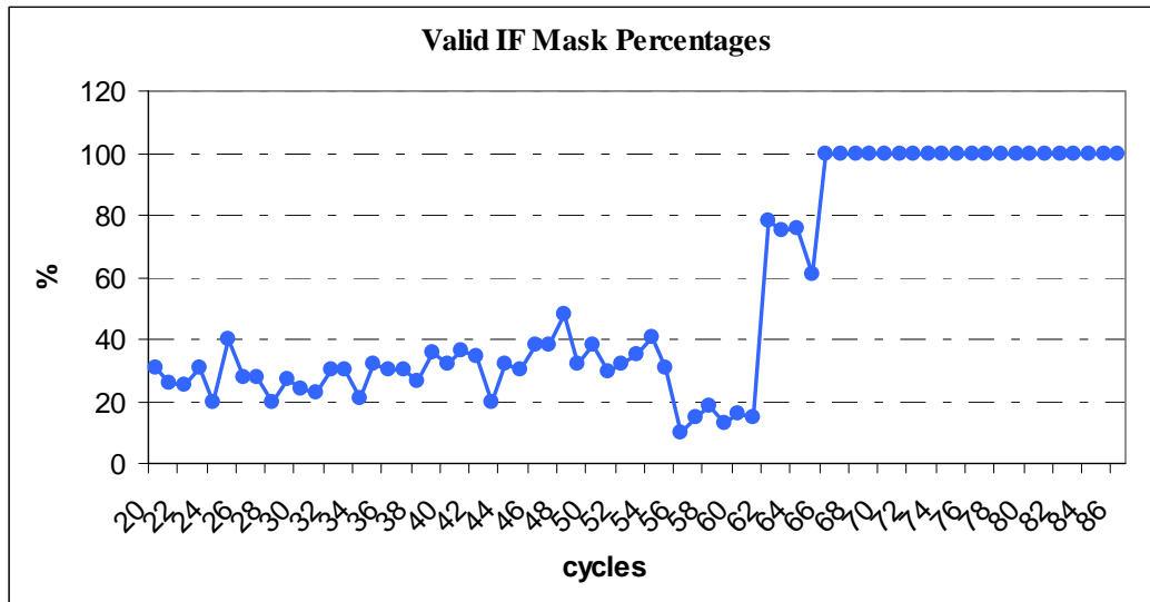
Figure 8: Percentages of valid IF Mask up to cycle 86
