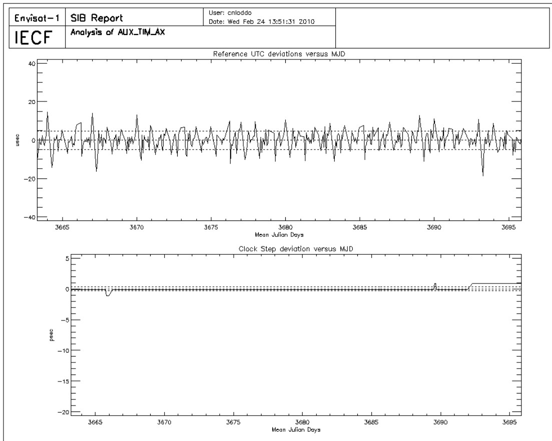
Figure 11: UTC deviations and ICU clock period for cycle 86
