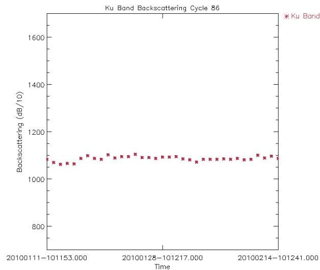
Figure 32: Ku Band Sigma_0 daily average for cycle 86 (dB/100)
