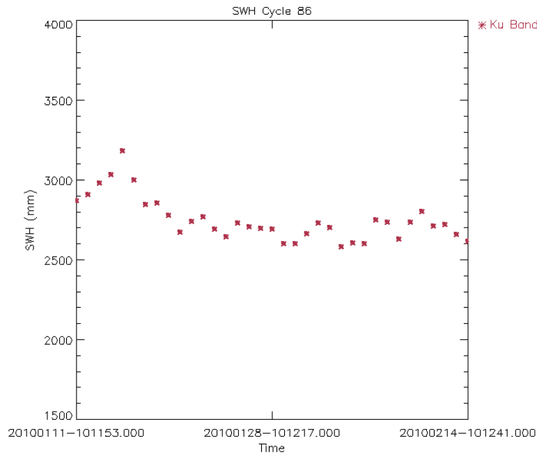
Figure 29: Ku Band SWH daily average for Cycle 86 (mm)
