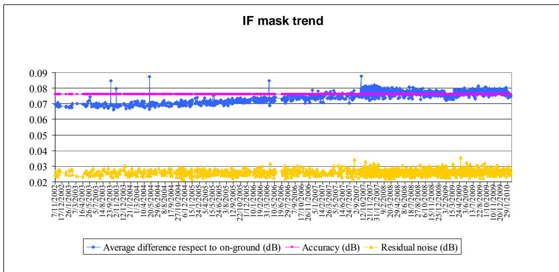
Figure 7: Evolution of the IF mask related parameters for valid IF masks retrieved up to cycle 86
