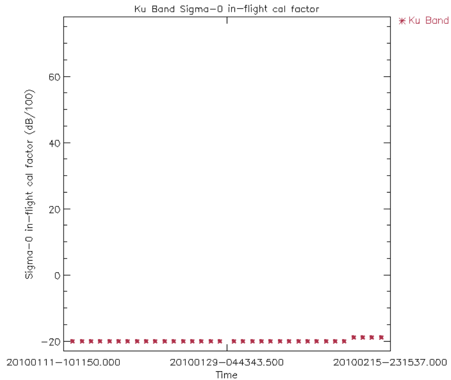
Figure 15: Ku Band in-flight Sigma0 calibration factor for cycle 86 (averaged per day)
