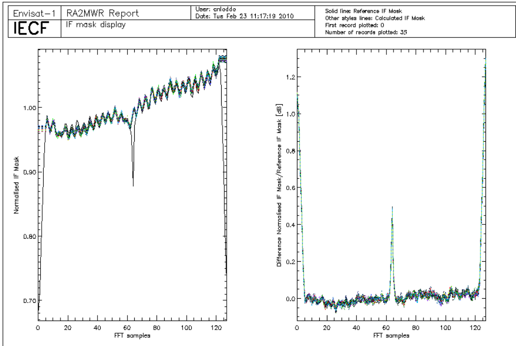
Figure 5: Valid IF masks retrieved during cycle 86 plotted together with the on-ground reference.
