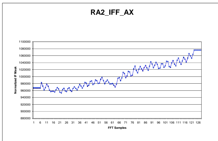
Figure 6: Previous and IF Mask updated on 22 nd December 2009
