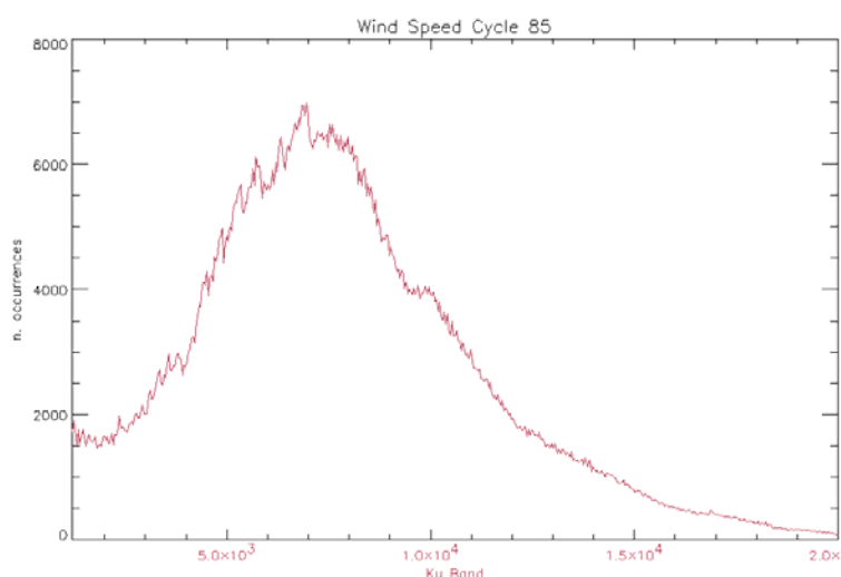
Figure 33: Histogram of Ku Wind Speed for cycle 85 (mm/sec)
