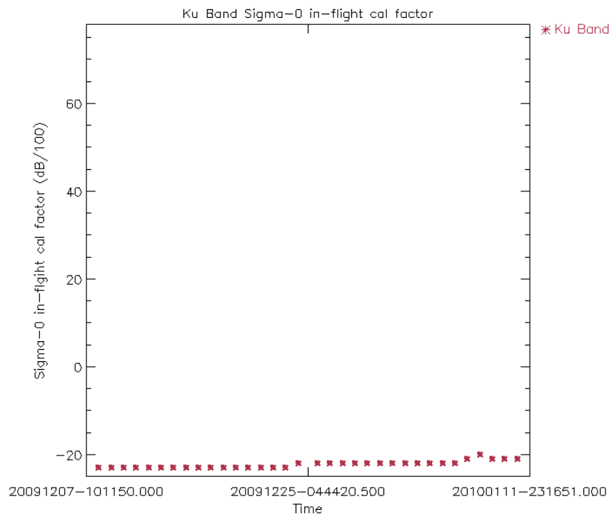
Figure 15: Ku Band in-flight Sigma0 calibration factor for cycle 85 (averaged per day)
