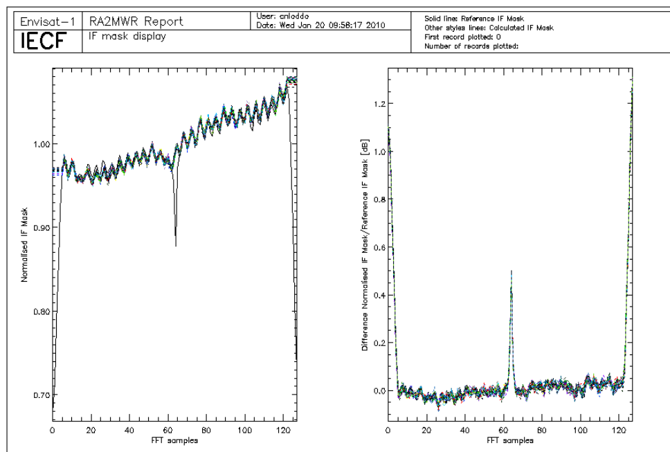
Figure 5: Valid IF masks retrieved during cycle 85 plotted together with the on-ground reference.
