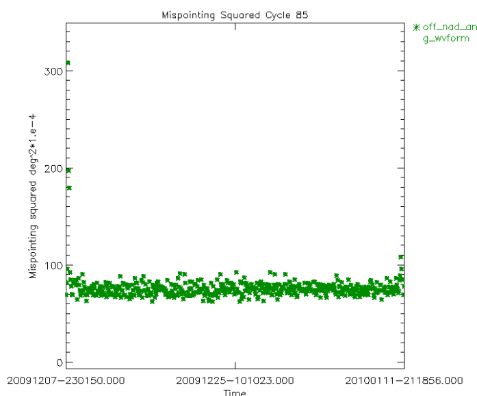
Figure 19: Smoothed mispointing squared trend for cycle 85 ( \text{deg}^2 \cdot 10^{-4} )
