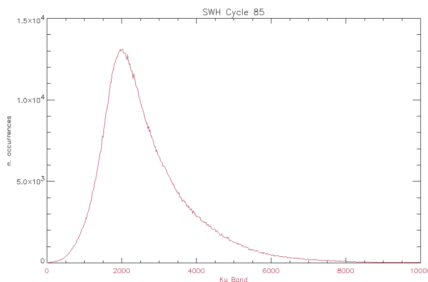
Figure 28: Histogram of Ku Band SWH for cycle 85
