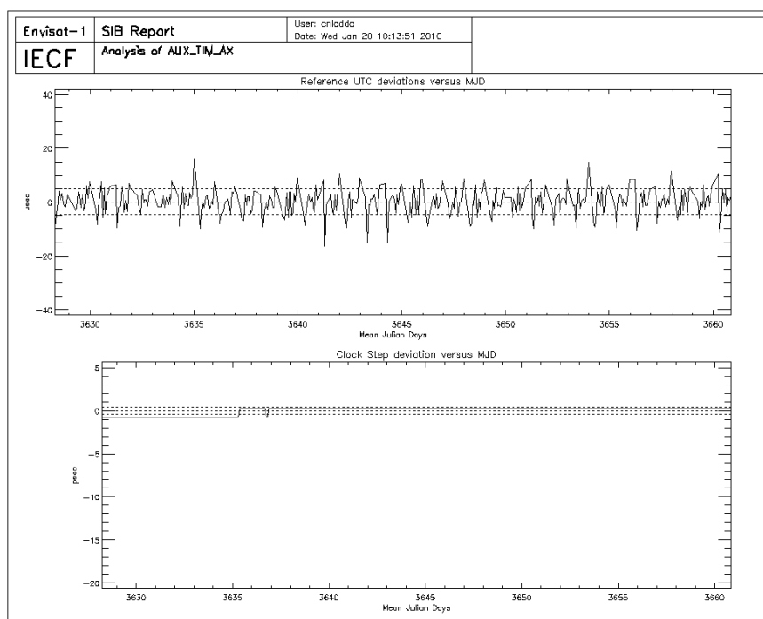
Figure 11: UTC deviations and ICU clock period for cycle 85
