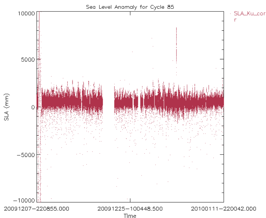
Figure 27A: Sea Level Anomalies Cycle 85 only MDSRs with valid DORIS Flag
