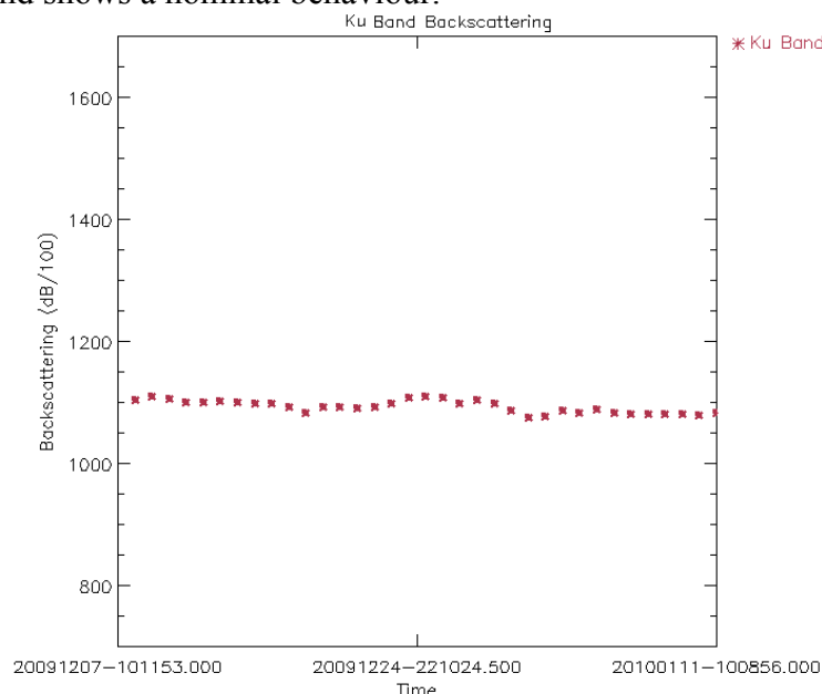
Figure 32: Ku Band Sigma_0 daily average for cycle 85 (dB/100)
