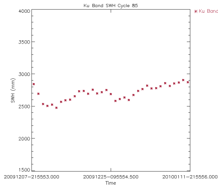
Figure 29: Ku Band SWH daily average for Cycle 85 (mm)
