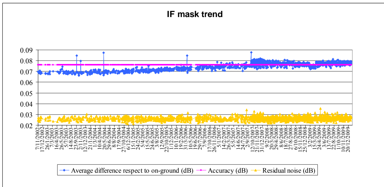
Figure 7: Evolution of the IF mask related parameters for valid IF masks retrieved up to cycle 85
