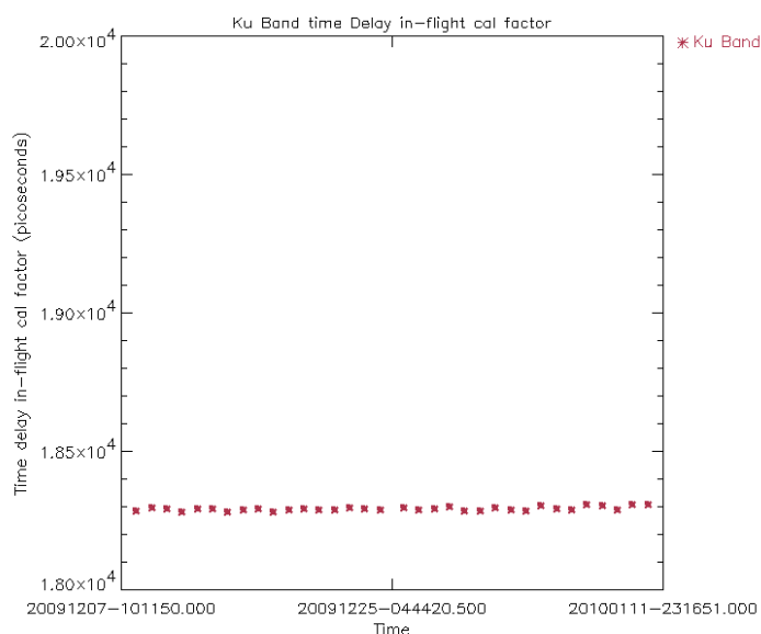
Figure 14: Ku Band in-flight time delay calibration factor for cycle 85 (averaged per day)
