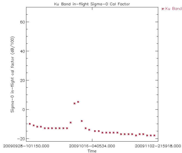
Figure 15: Ku Band in-flight Sigma0 calibration factor for cycle 83 (averaged per day)
