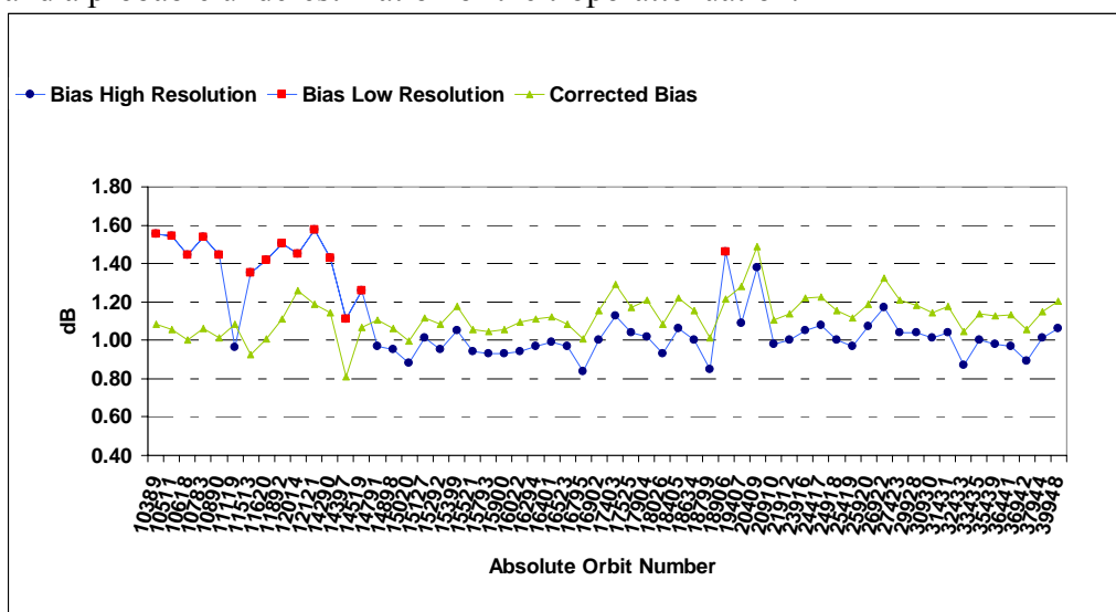
Figure 18: Time behaviour of the transponder bias
