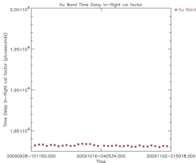
Figure 14: Ku Band in-flight time delay calibration factor for cycle 83 (averaged per day)
