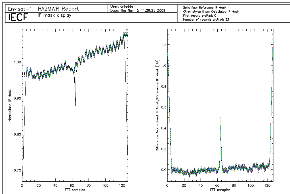
Figure 5: Valid IF masks retrieved during cycle 83 plotted together with the on-ground reference.
