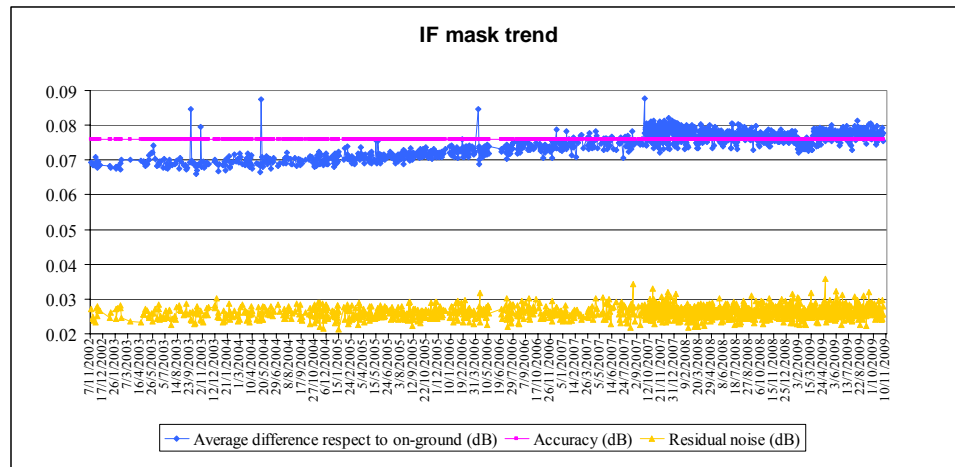
Figure 7: Evolution of the IF mask related parameters for valid IF masks retrieved up to cycle 83
