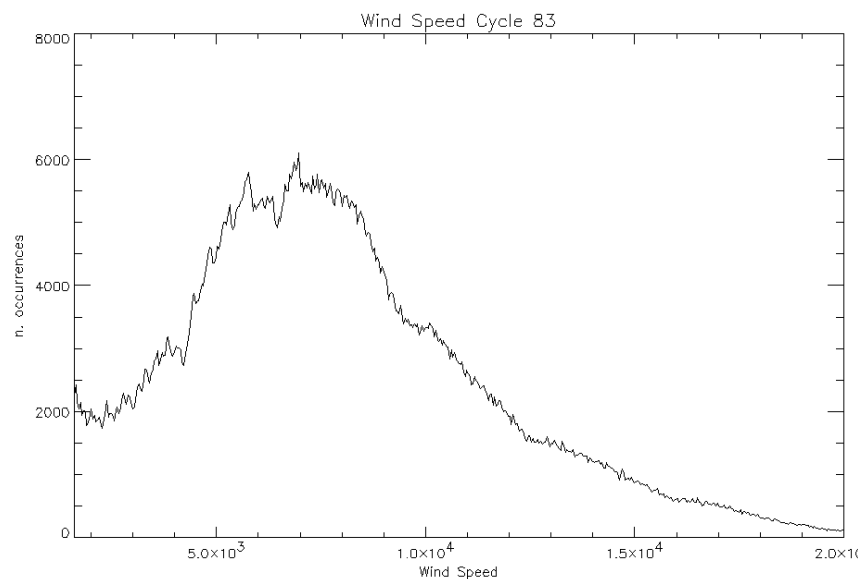
Figure 33: Histogram of Ku Wind Speed for cycle 83 (mm/sec)
