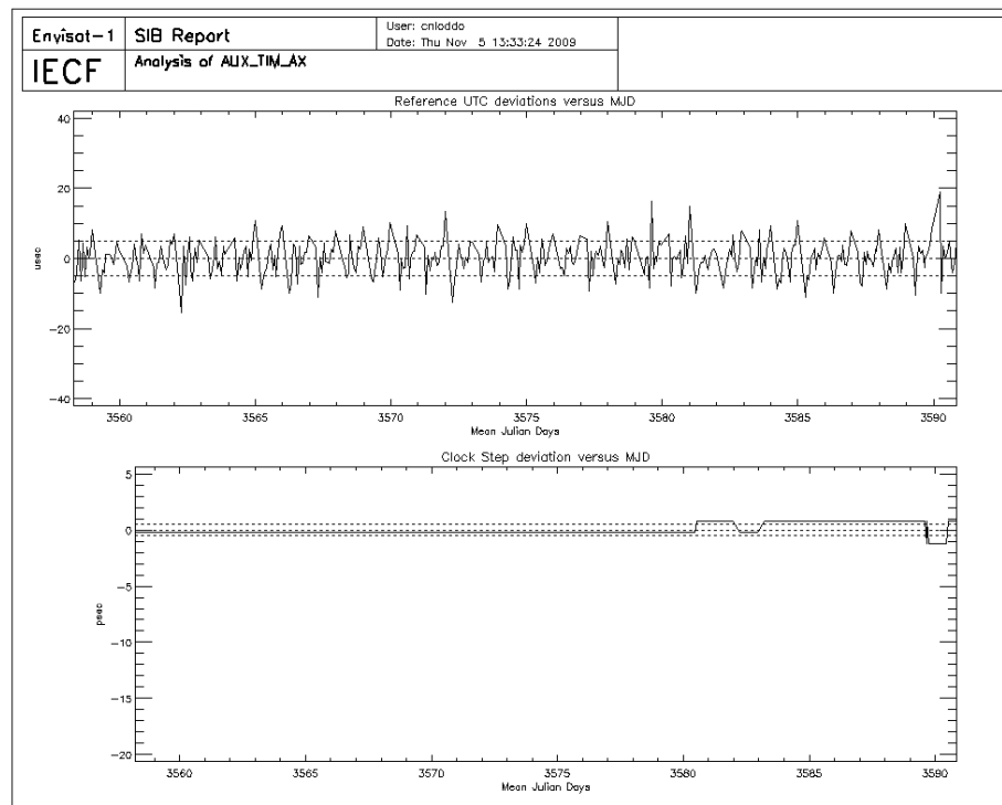
Figure 11: UTC deviations and ICU clock period for cycle 83
