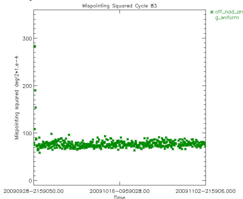
Figure 19: Smoothed mispointing squared trend for cycle 83 ( \text{deg}^2 \cdot 10^{-4} )
