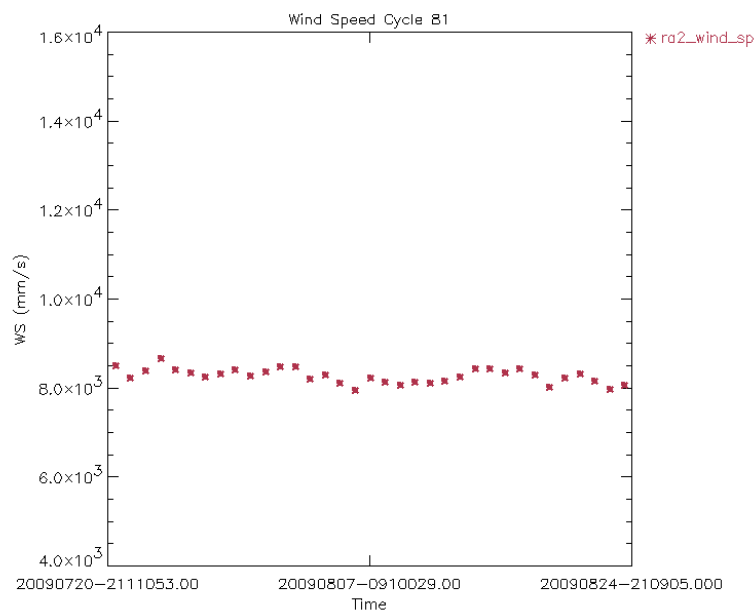
Figure 34: Ku Band Wind Speed daily average for cycle 81 (mm/s)
