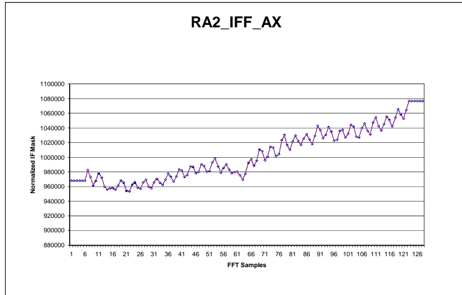
Figure 6: Previous and IF Mask updated on 20 th August 2009
