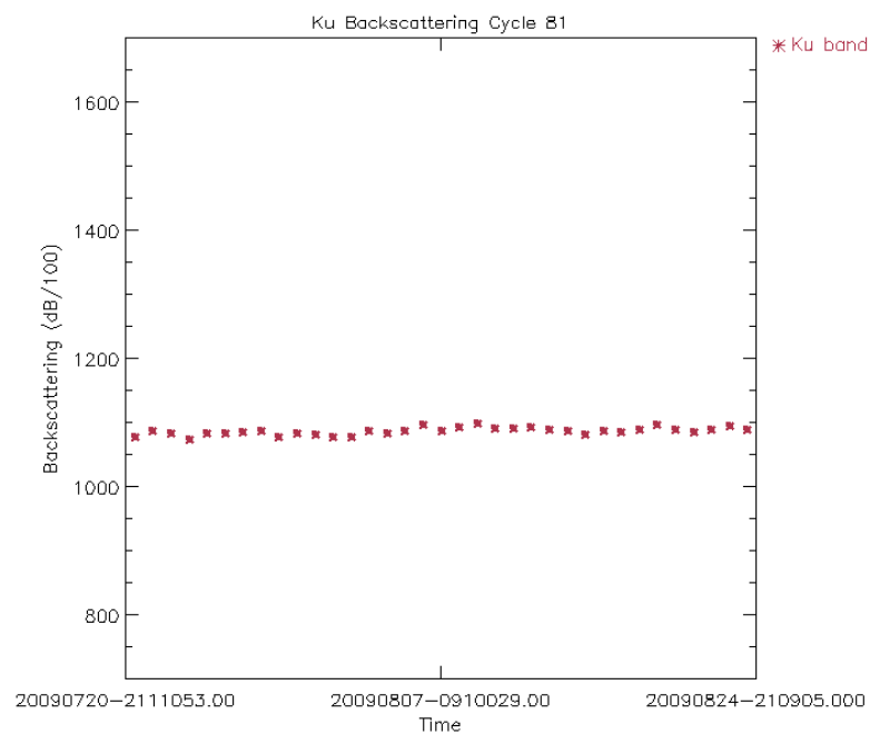
Figure 32: Ku Band Sigma_0 daily average for cycle 81 (dB/100)
