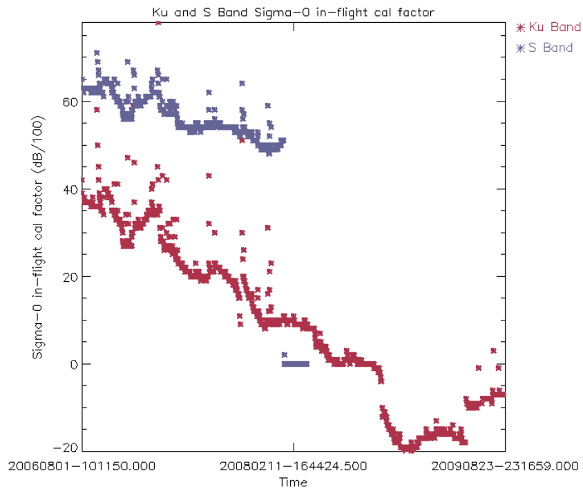
Figure 17A: Ku and S Band in-flight Sigma0 calibration factor from cycle 50 onwards (averaged per day)
