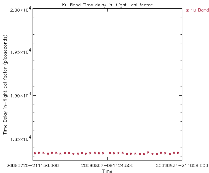
Figure 14: Ku Band in-flight time delay calibration factor for cycle 81 (averaged per day)
