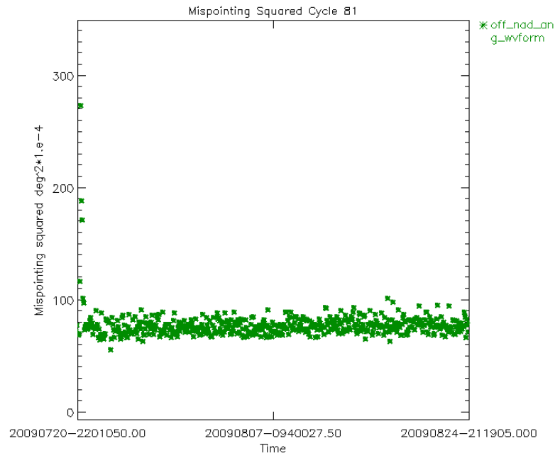
Figure 19: Smoothed mispointing squared trend for cycle 81 ( \text{deg}^2 \cdot 10^{-4} )
