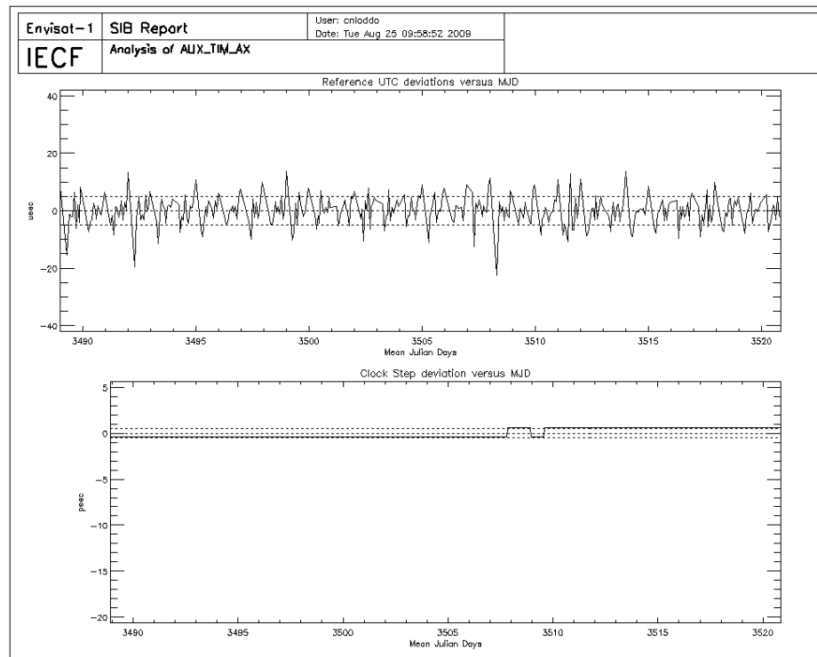
Figure 11: UTC deviations and ICU clock period for cycle 81
