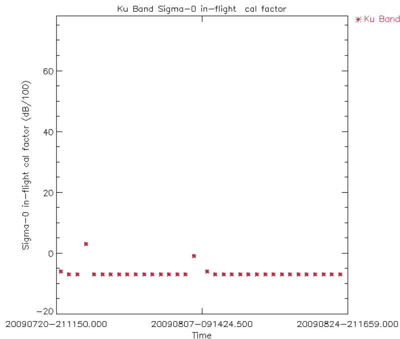
Figure 15: Ku Band in-flight Sigma0 calibration factor for cycle 81 (averaged per day)
