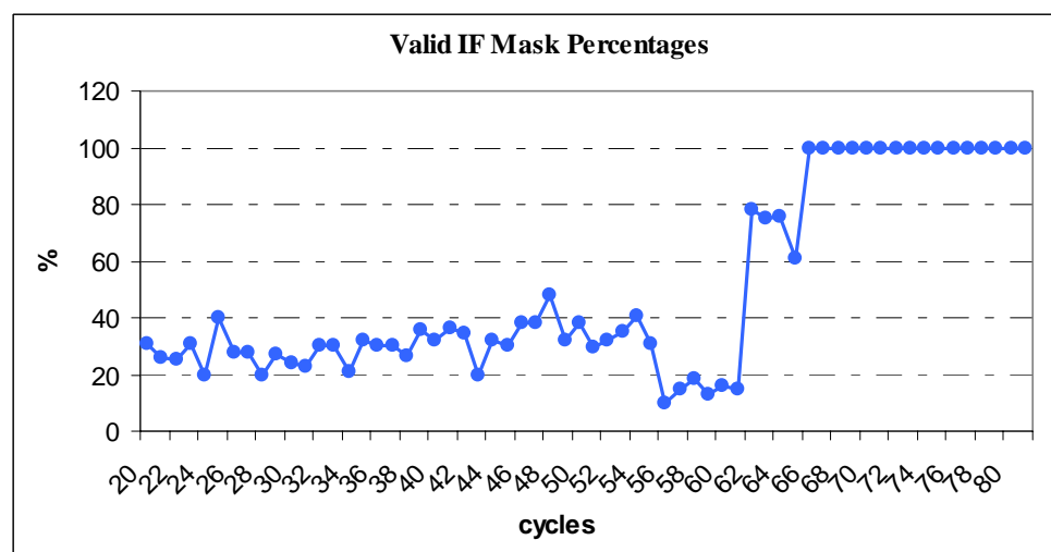
Figure 8: Percentages of valid IF Mask up to cycle 81
