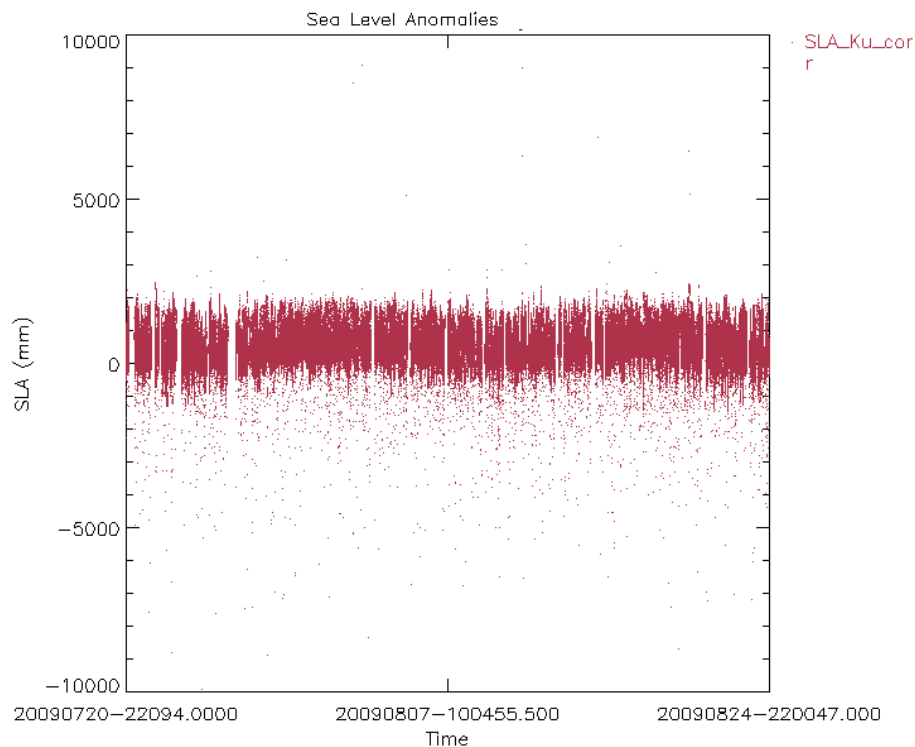
Figure 27A: Sea Level Anomalies Cycle 81 only MDSRs with valid DORIS Flag
