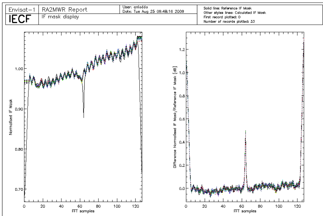
Figure 5: Valid IF masks retrieved during cycle 81 plotted together with the on-ground reference.
