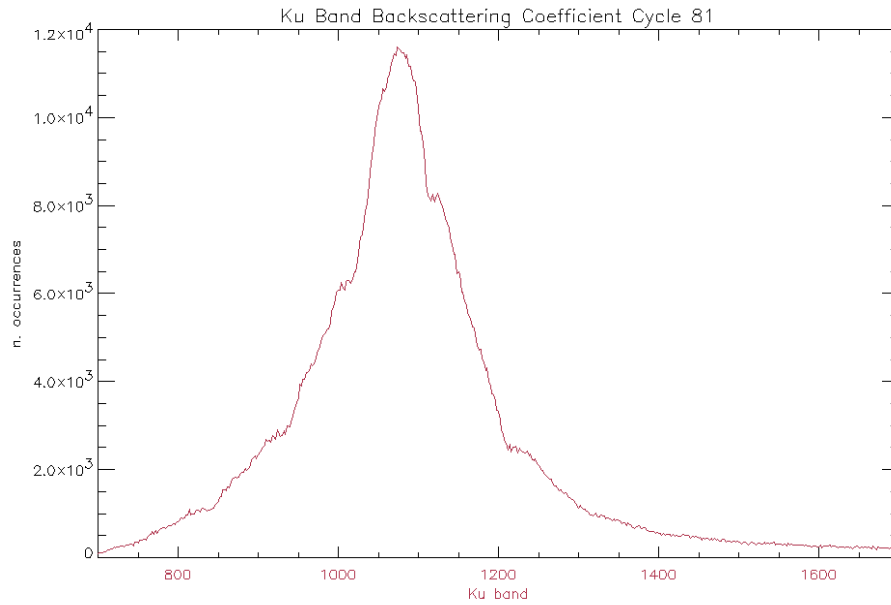
Figure 31: Histogram of Ku Band Backscattering Coefficient for cycle 81
