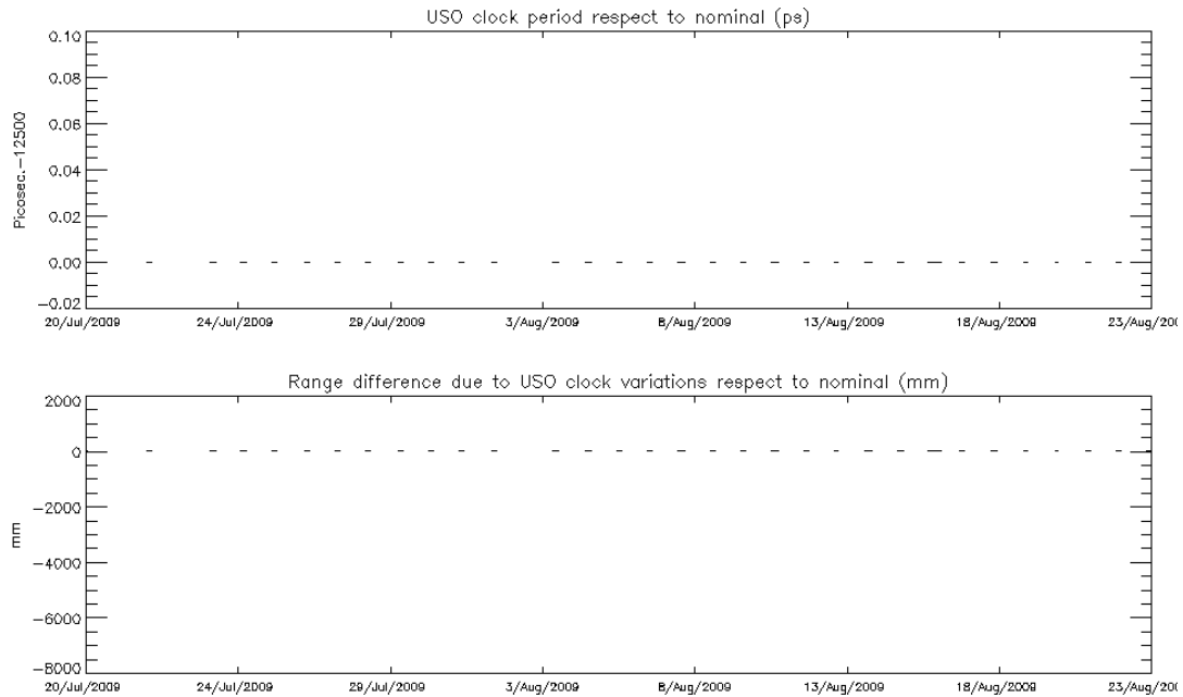
Figure 9: USO clock period (top) and range difference with nominal (bottom) for cycle 81
