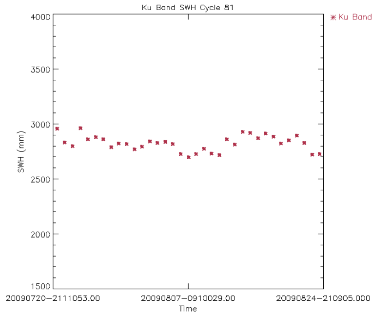
Figure 29: Ku Band SWH daily average for Cycle 81 (mm)
