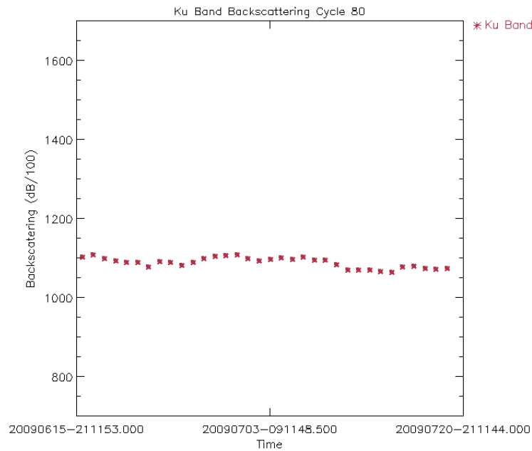
Figure 32: Ku Band Sigma_0 daily average for cycle 80 (dB/100)
