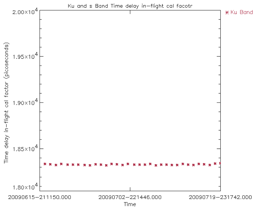
Figure 14: Ku Band in-flight time delay calibration factor for cycle 80 (averaged per day)
