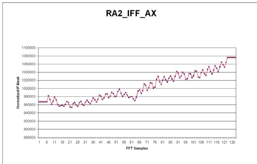
Figure 6: Previous and IF Mask updated on 17 th June 2009
