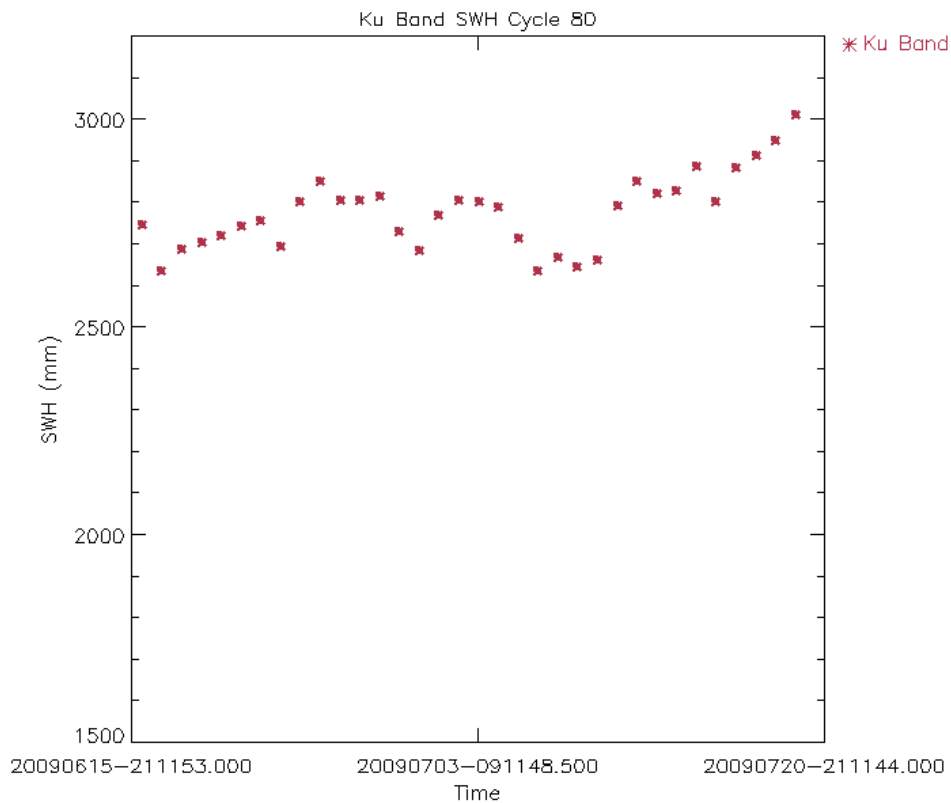
Figure 29: Ku Band SWH daily average for Cycle 80 (mm)
