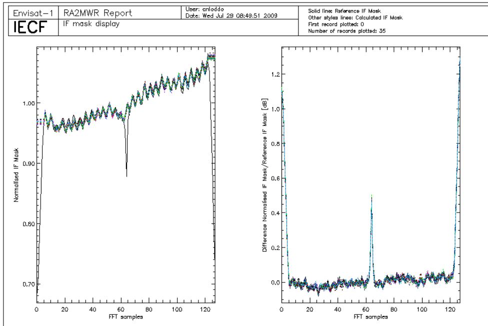
Figure 5: Valid IF masks retrieved during cycle 80 plotted together with the on-ground reference.
