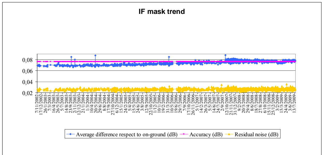
Figure 7: Evolution of the IF mask related parameters for valid IF masks retrieved up to cycle 80
