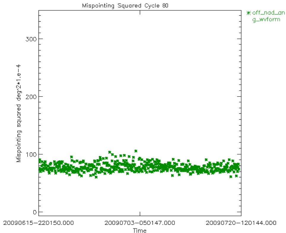
Figure 19: Smoothed mispointing squared trend for cycle 80 ( \text{deg}^2 \cdot 10^{-4} )
