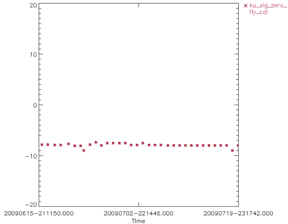
Figure 15: Ku Band in-flight Sigma0 calibration factor for cycle 80 (averaged per day)
