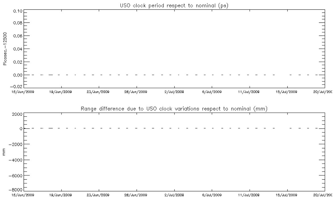
Figure 9: USO clock period (top) and range difference with nominal (bottom) for cycle 80
