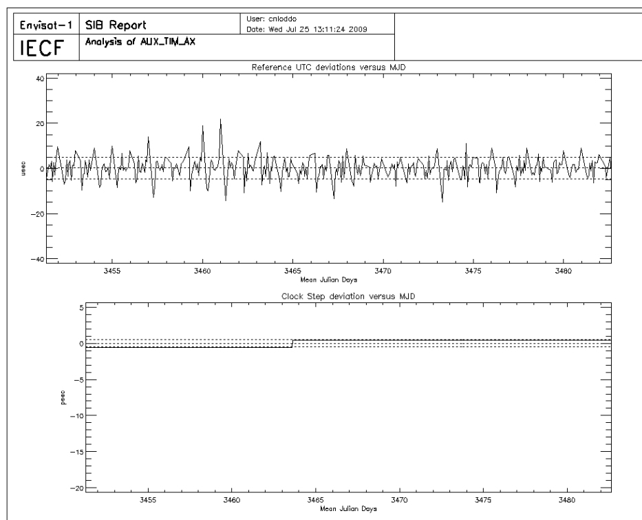
Figure 11: UTC deviations and ICU clock period for cycle 80
