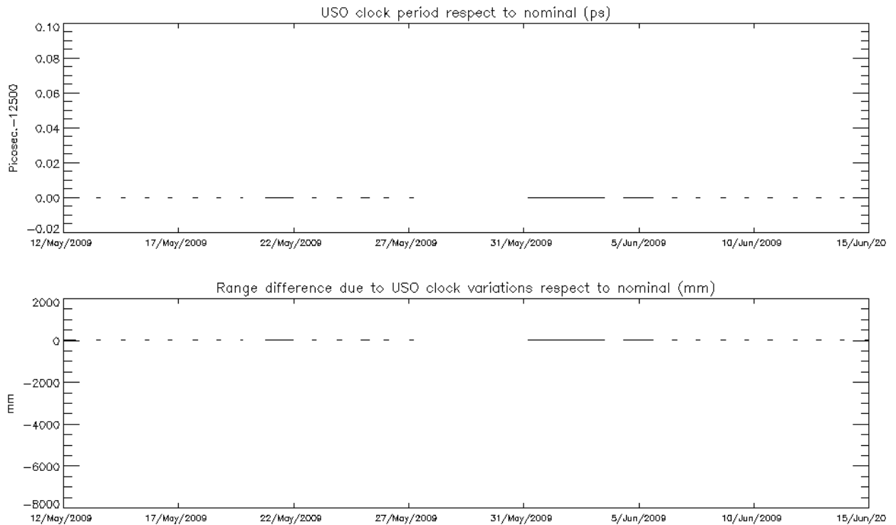
Figure 9: USO clock period (top) and range difference with nominal (bottom) for cycle 79
