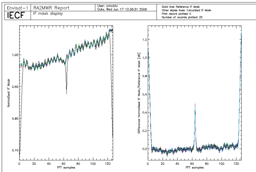
Figure 5: Valid IF masks retrieved during cycle 79 plotted together with the on-ground reference.
