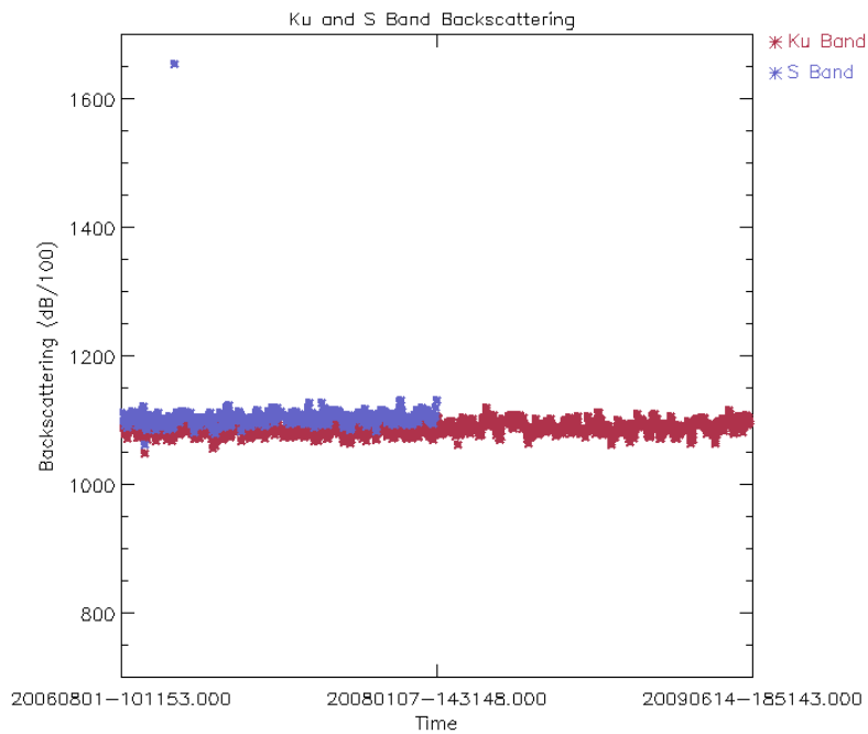
Figure 35A: Ku and S band Backscatter daily averages from cycle 50 onwards (dB/100)
