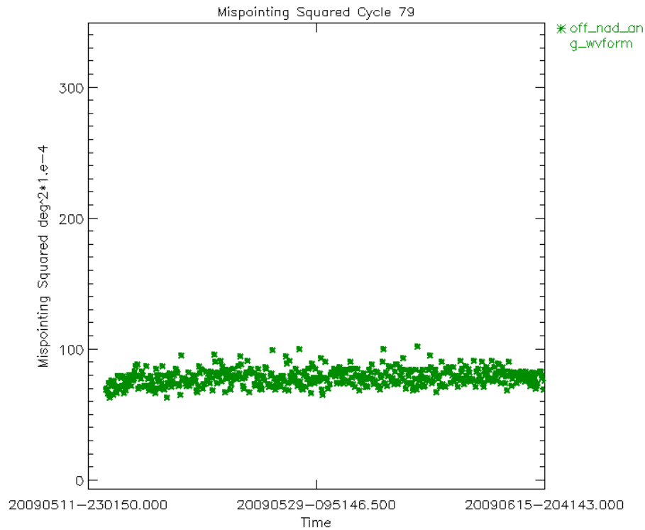
Figure 19: Smoothed mispointing squared trend for cycle 79 ( \text{deg}^2 \cdot 10^{-4} )
