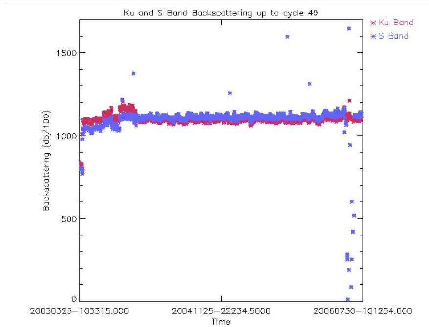
Figure 35: Ku and S band Backscatter daily averages up to cycle 49 (dB/100)
