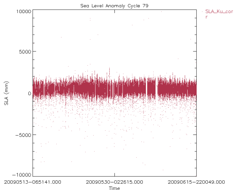
Figure 27A: Sea Level Anomalies Cycle 79 only MDSRs with valid DORIS Flag
