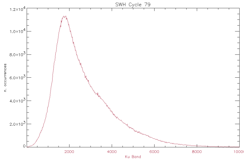
Figure 28: Histogram of Ku Band SWH for cycle 79
