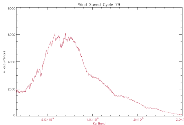
Figure 33: Histogram of Ku Wind Speed for cycle 79 (mm/sec)
