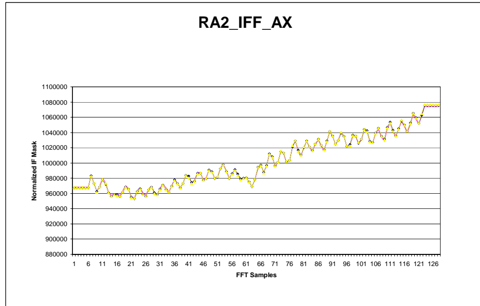
Figure 6: Previous and IF Mask updated on 20 th May 2009
