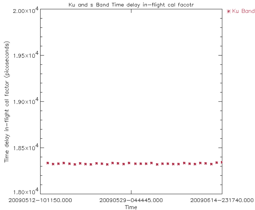
Figure 14: Ku Band in-flight time delay calibration factor for cycle 79 (averaged per day)
