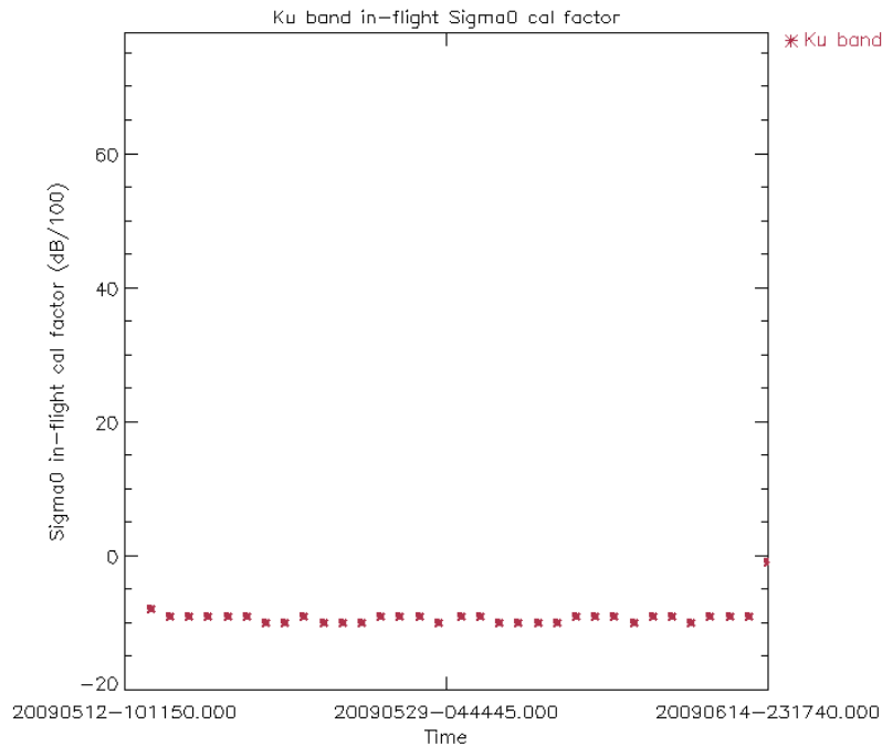
Figure 15: Ku Band in-flight Sigma0 calibration factor for cycle 79 (averaged per day)
