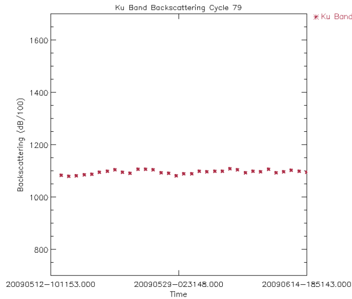
Figure 32: Ku Band Sigma_0 daily average for cycle 79 (dB/100)
