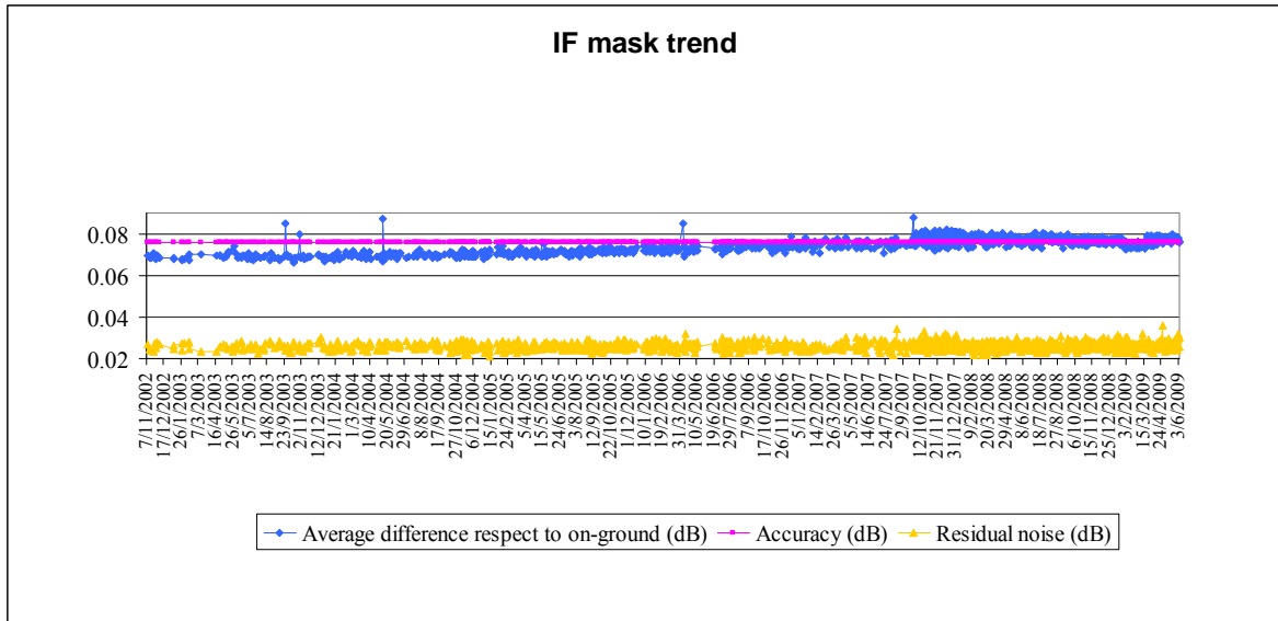
Figure 7: Evolution of the IF mask related parameters for valid IF masks retrieved up to cycle 79
