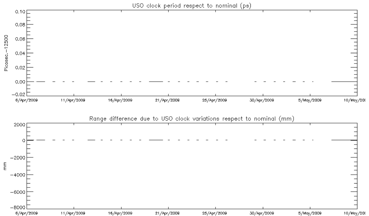
Figure 9: USO clock period (top) and range difference with nominal (bottom) for cycle 78
