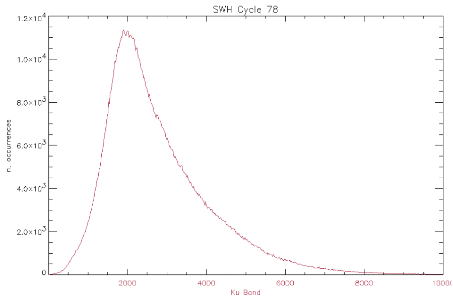
Figure 28: Histogram of Ku Band SWH for cycle 78
