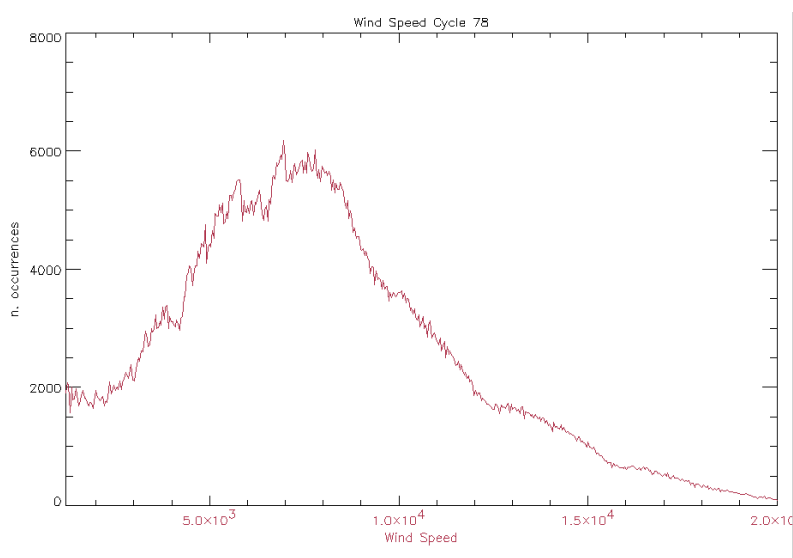
Figure 33: Histogram of Ku Wind Speed for cycle 78 (mm/sec)
