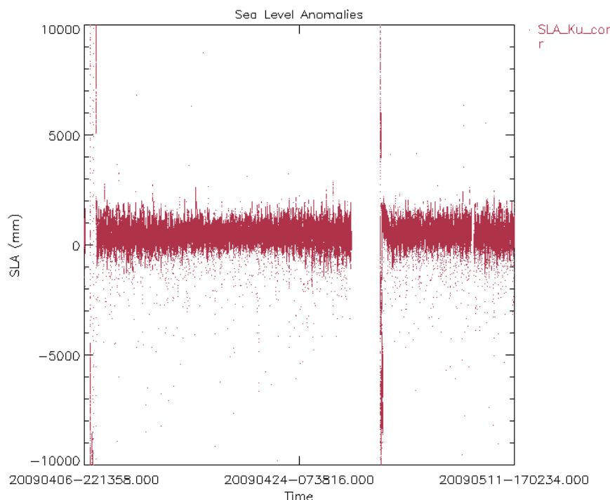
Figure 27A: Sea Level Anomalies Cycle 78 only MDSRs with valid DORIS Flag
