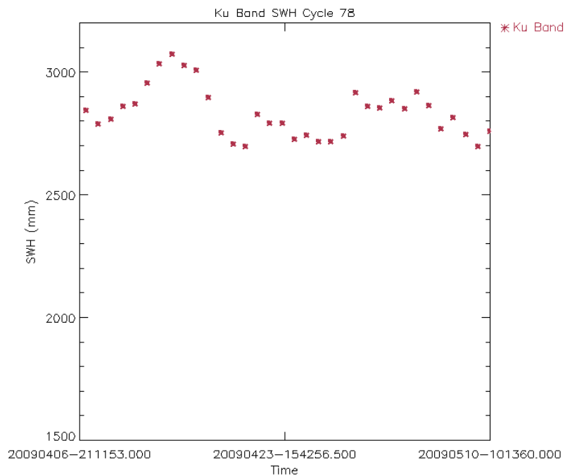
Figure 29: Ku Band SWH daily average for Cycle 78 (mm)
