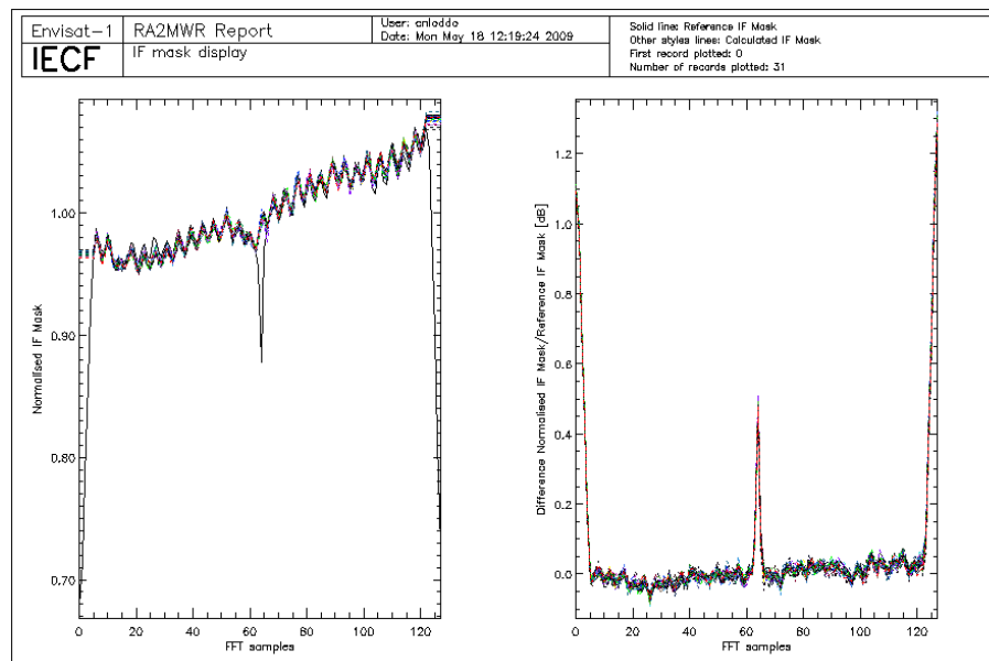
Figure 5: Valid IF masks retrieved during cycle 78 plotted together with the on-ground reference.
