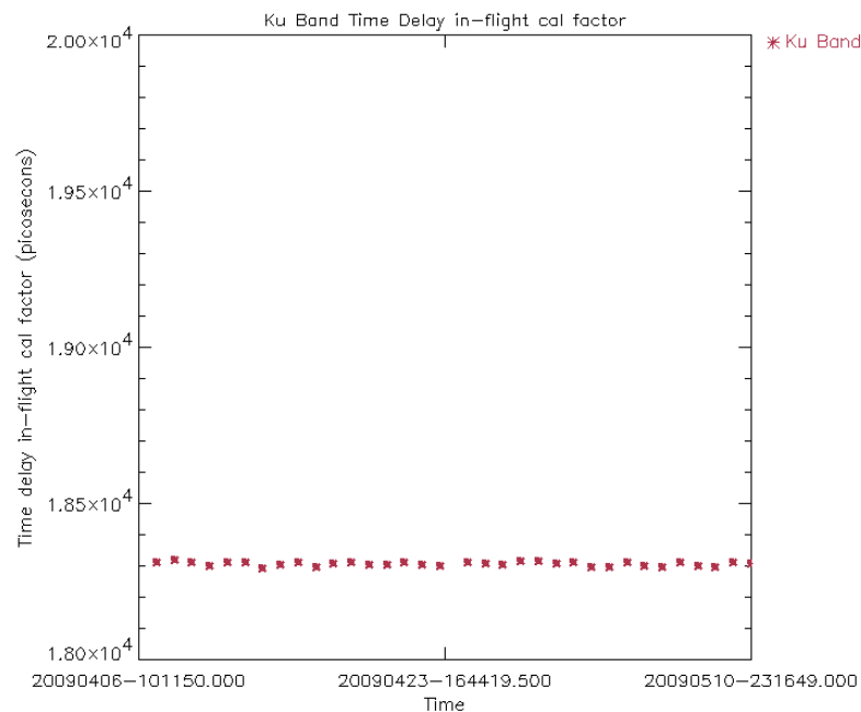
Figure 14: Ku Band in-flight time delay calibration factor for cycle 78 (averaged per day)
