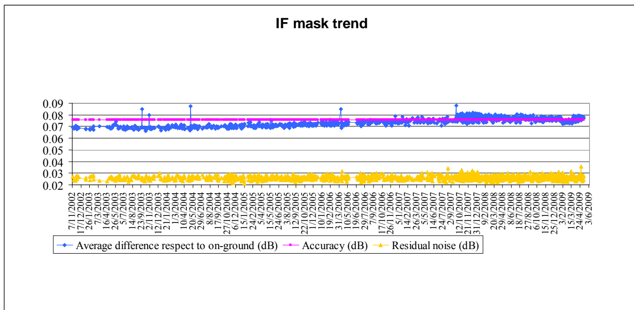
Figure 7: Evolution of the IF mask related parameters for valid IF masks retrieved up to cycle 78
