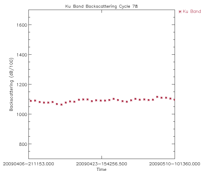
Figure 32: Ku Band Sigma_0 daily average for cycle 78 (dB/100)
