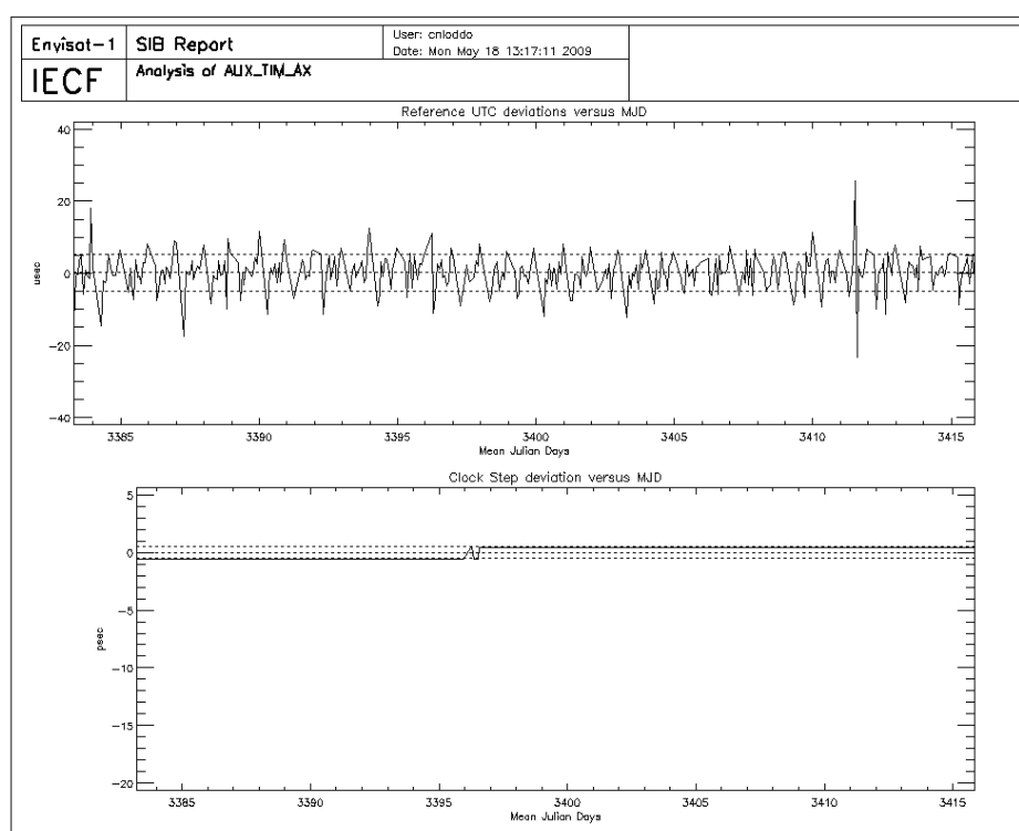
Figure 11: UTC deviations and ICU clock period for cycle 78
