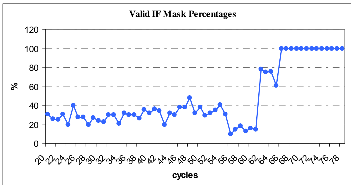
Figure 8: Percentages of valid IF Mask up to cycle 78
