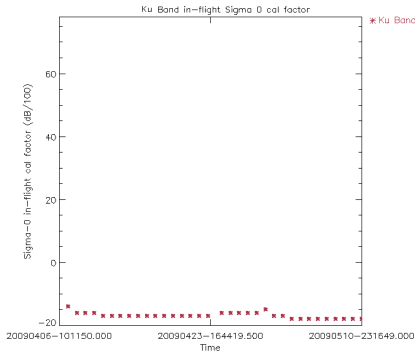
Figure 15: Ku Band in-flight Sigma0 calibration factor for cycle 78 (averaged per day)
