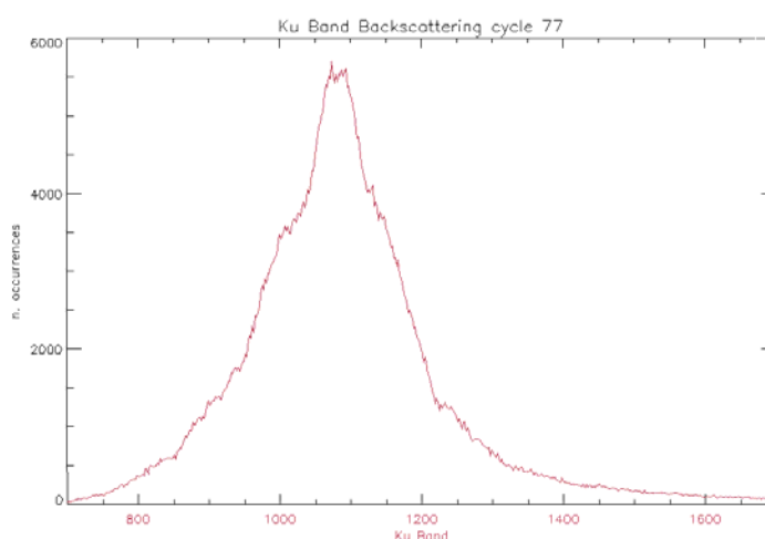
Figure 31: Histogram of Ku Band Backscattering Coefficient for cycle 77
