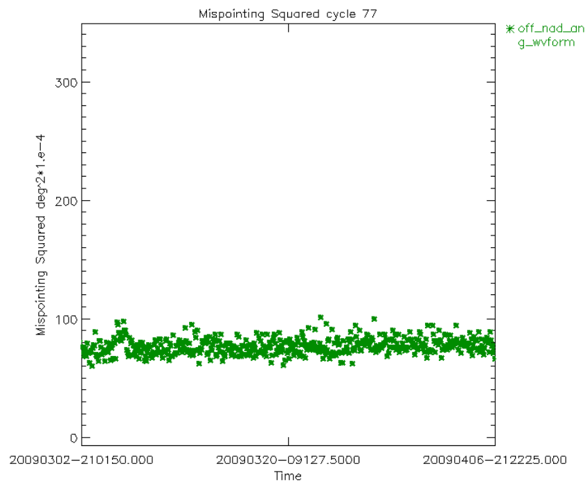
Figure 19: Smoothed mispointing squared trend for cycle 77 ( \text{deg}^2 \cdot 10^{-4} )
