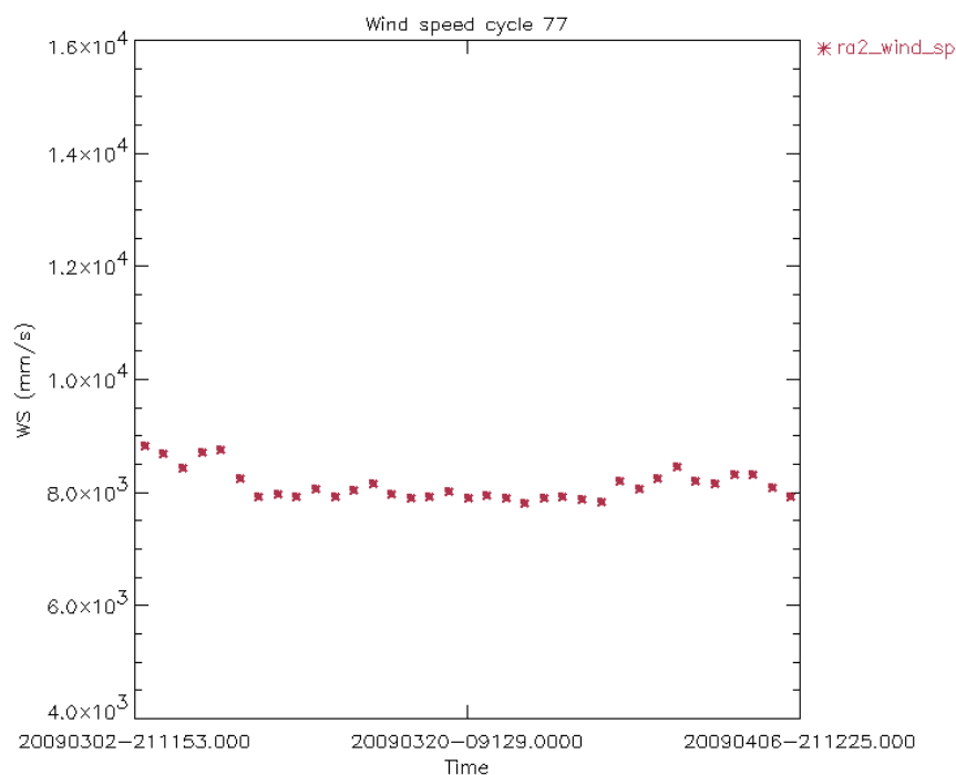
Figure 34: Ku Band Wind Speed daily average for cycle 77 (mm/s)
