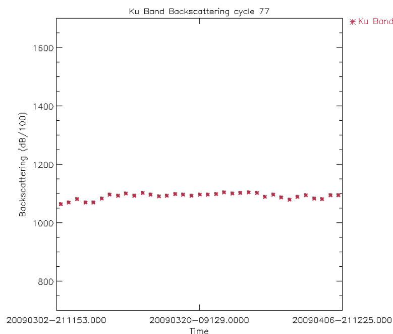
Figure 32: Ku Band Sigma_0 daily average for cycle 77 (dB/100)
