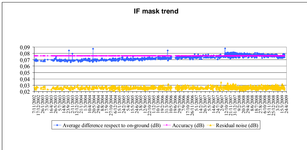
Figure 7: Evolution of the IF mask related parameters for valid IF masks retrieved up to cycle 77
