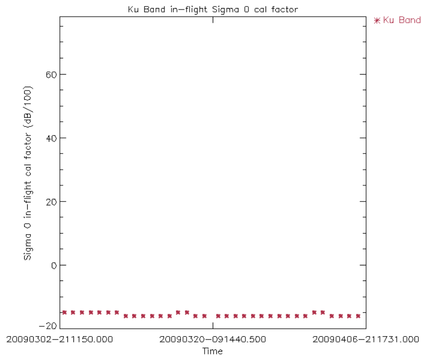
Figure 15: Ku Band in-flight Sigma0 calibration factor for cycle 77 (averaged per day)
