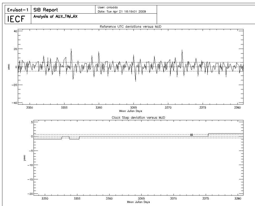
Figure 11: UTC deviations and ICU clock period for cycle 77
