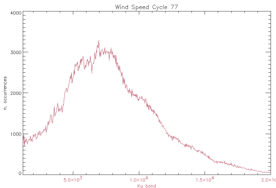
Figure 33: Histogram of Ku Wind Speed for cycle 77 (mm/sec)
