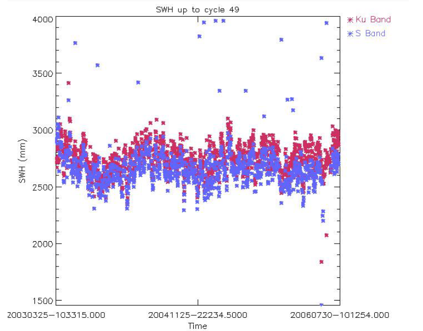
Figure 30: Ku and S SWH daily average up to cycle 49 (mm)
