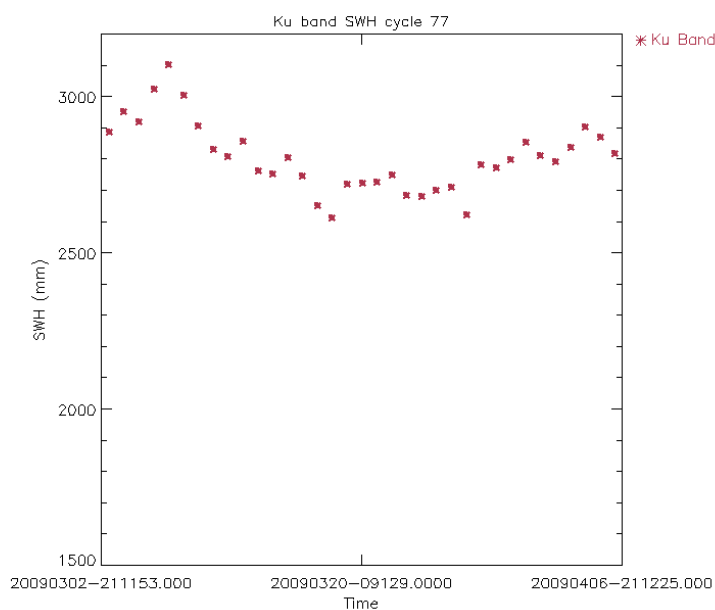
Figure 29: Ku Band SWH daily average for Cycle 77 (mm)
