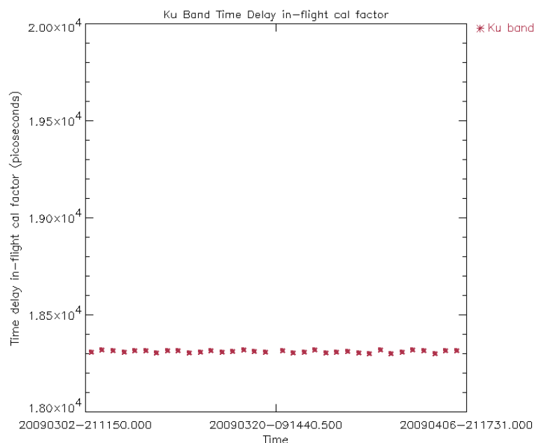
Figure 14: Ku Band in-flight time delay calibration factor for cycle 77 (averaged per day)
