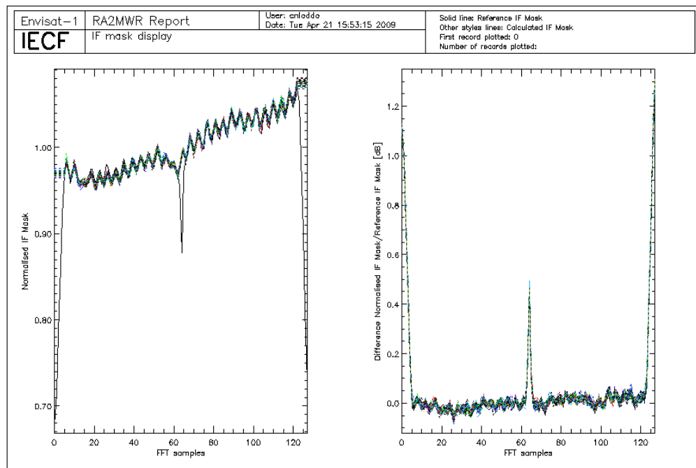
Figure 5: Valid IF masks retrieved during cycle 77 plotted together with the on-ground reference.
