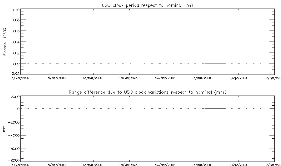
Figure 9: USO clock period (top) and range difference with nominal (bottom) for cycle 77
