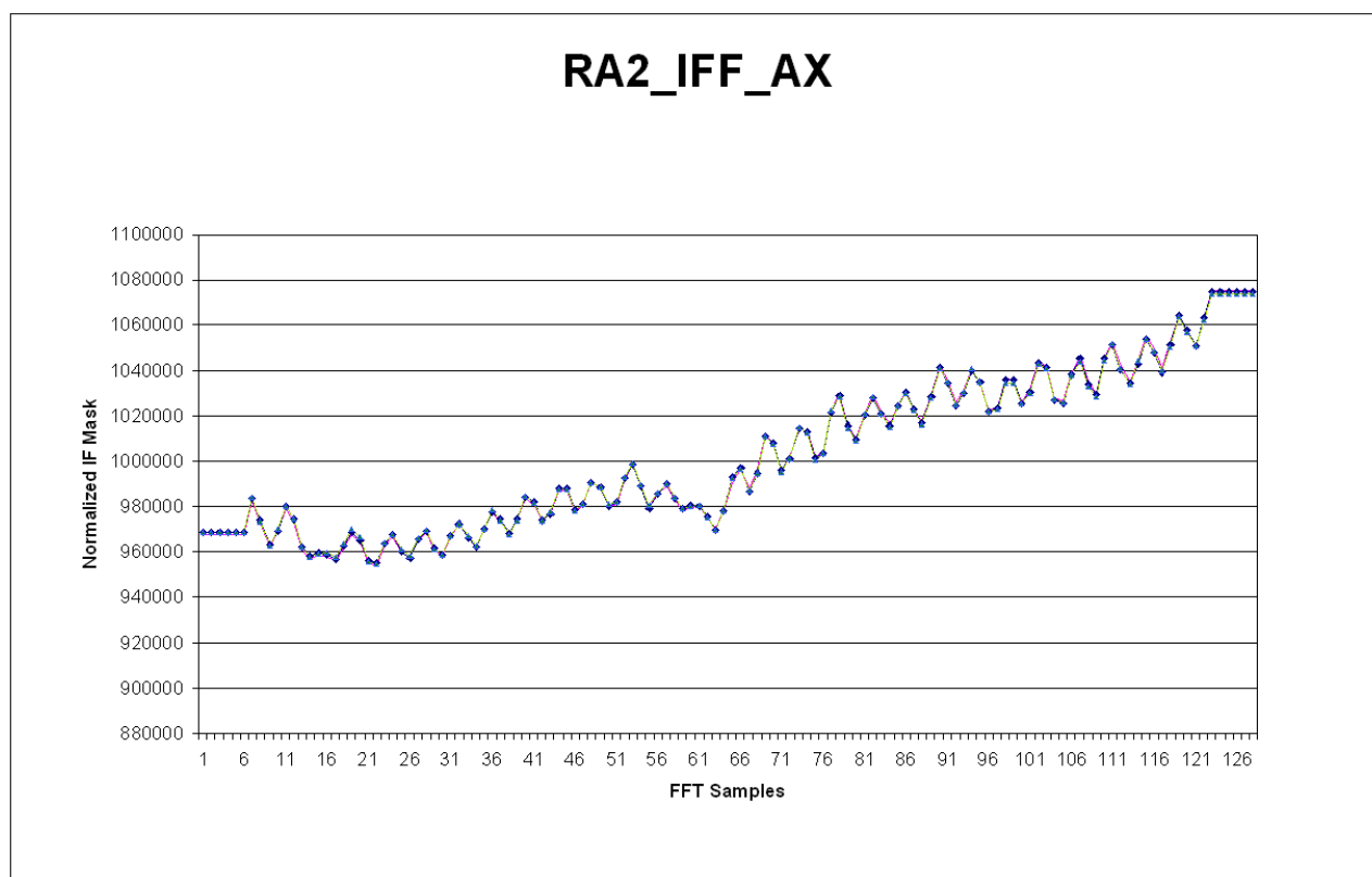
Figure 6: Previous and IF Mask updated on 26 th March 2009
