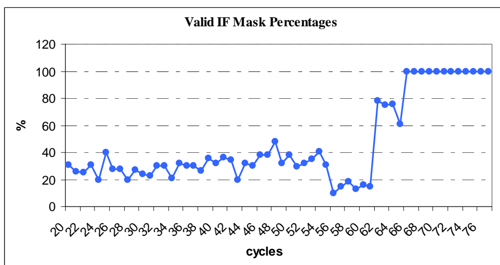
Figure 8: Percentages of valid IF Mask up to cycle 77
