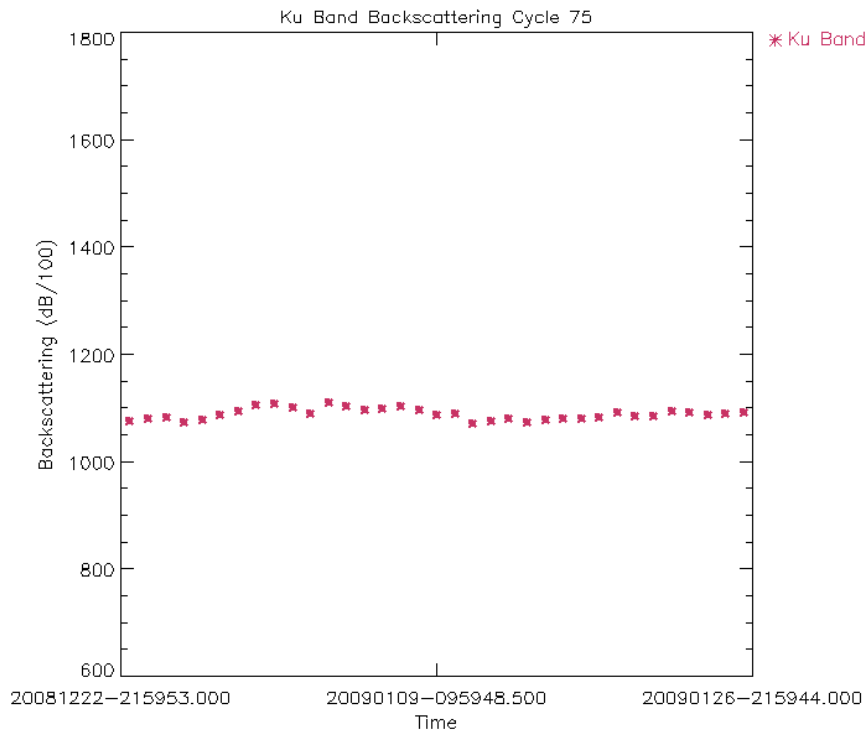
Figure 32: Ku Band Sigma_0 daily average for cycle 75(dB/100)
