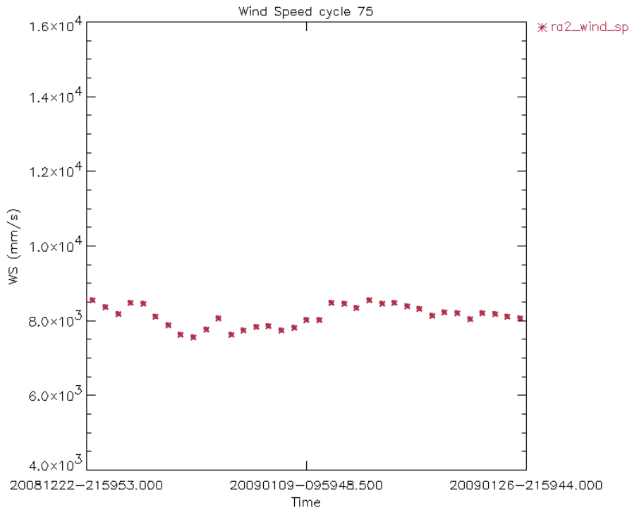
Figure 34: Ku Band Wind Speed daily average for cycle 75(mm/s)
