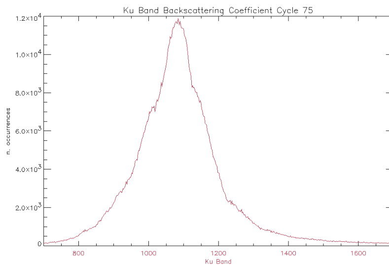
Figure 31: Histogram of Ku Band Backscattering Coefficient for cycle 75
