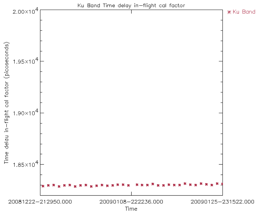
Figure 14: Ku Band in-flight time delay calibration factor for cycle 75 (averaged per day)
