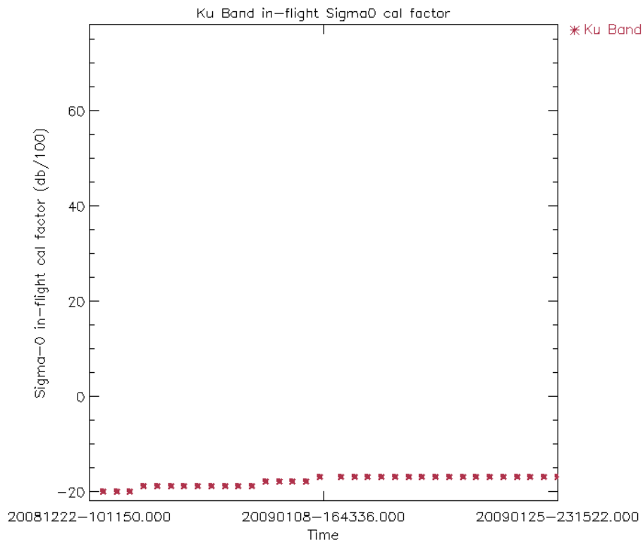
Figure 15: Ku Band in-flight Sigma0 calibration factor for cycle 75 (averaged per day)
