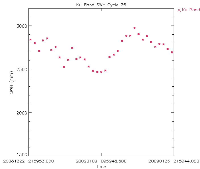
Figure 29: Ku Band SWH daily average for Cycle 75(mm)
