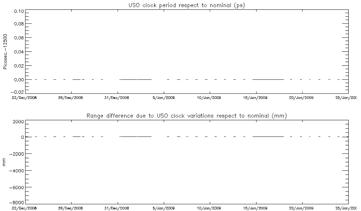
Figure 9: USO clock period (top) and range difference with nominal (bottom) for cycle 75
