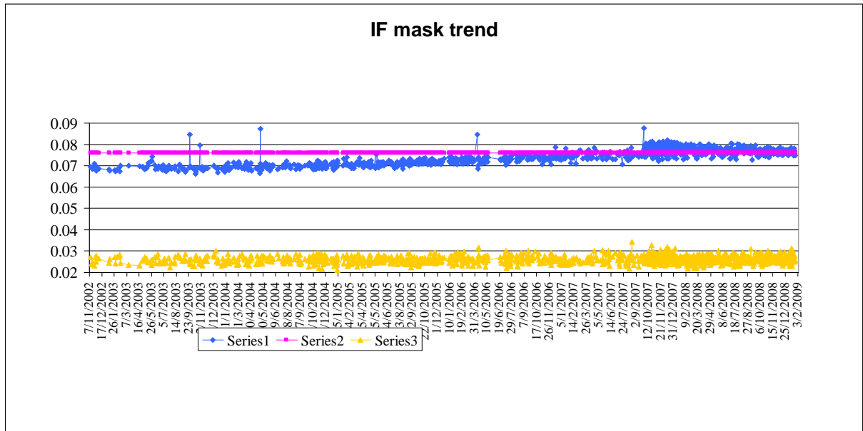
Figure 7: Evolution of the IF mask related parameters for valid IF masks retrieved up to cycle 75
