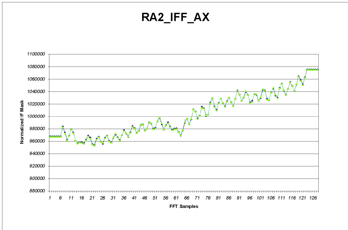
Figure 6: Previous and IF Mask updated on 14 th January 2009
