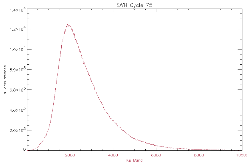
Figure 28: Histogram of Ku Band SWH for cycle 75
