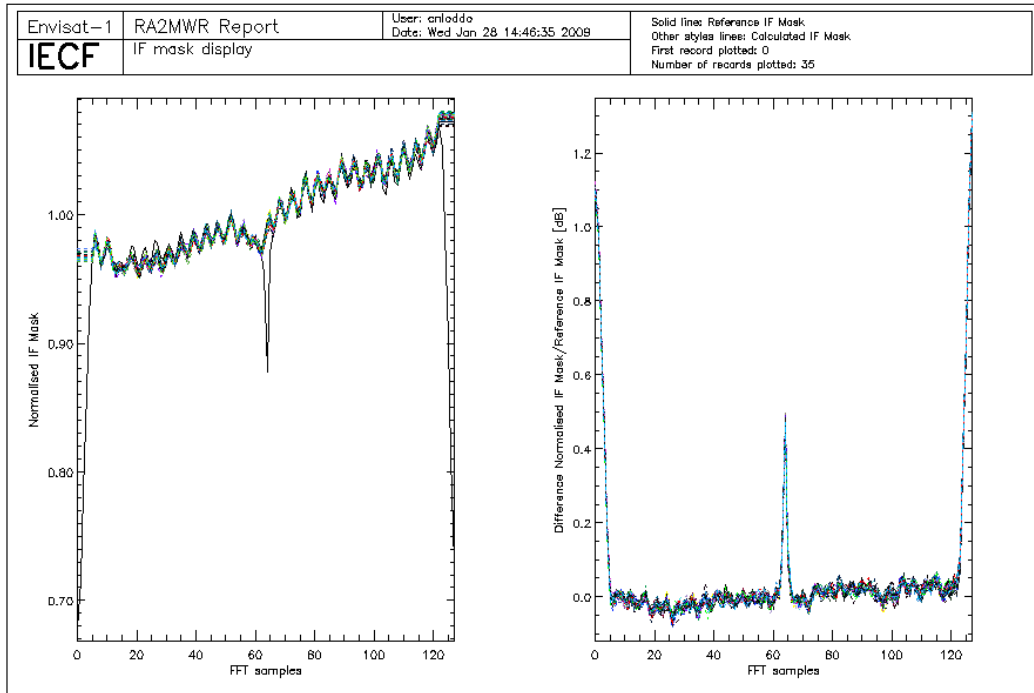
Figure 5: Valid IF masks retrieved during cycle 75 plotted together with the on-ground reference.
