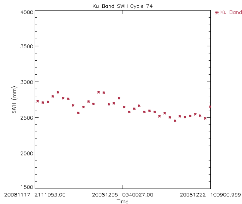
Figure 29: Ku Band SWH daily average for Cycle 74 (mm)
