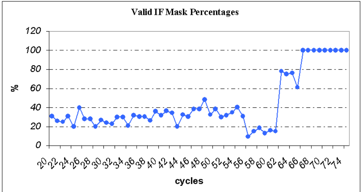
Figure 8: Percentages of valid IF Mask up to cycle 74
