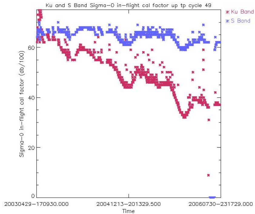
Figure 17: Ku and S Band in-flight Sigma0 calibration factor up to cycle 49 (averaged per day)
