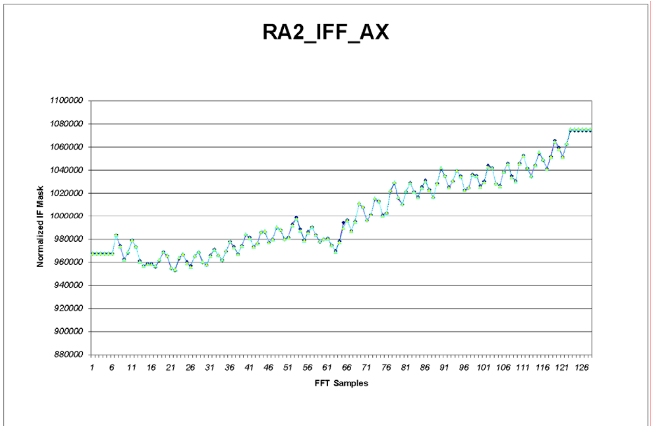
Figure 6: Previous and IF Mask updated on 10 December 2008
