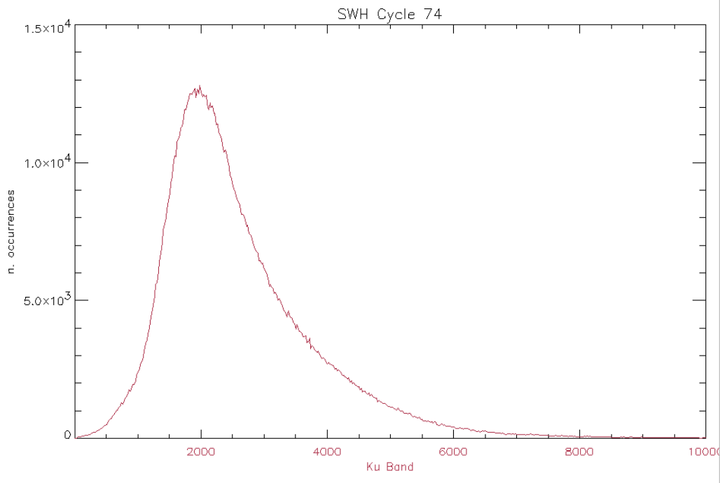
Figure 28: Histogram of Ku Band SWH for cycle 74
