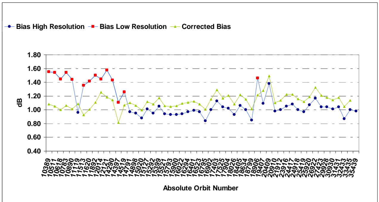
Figure 18: Time behavior of the transponder bias
