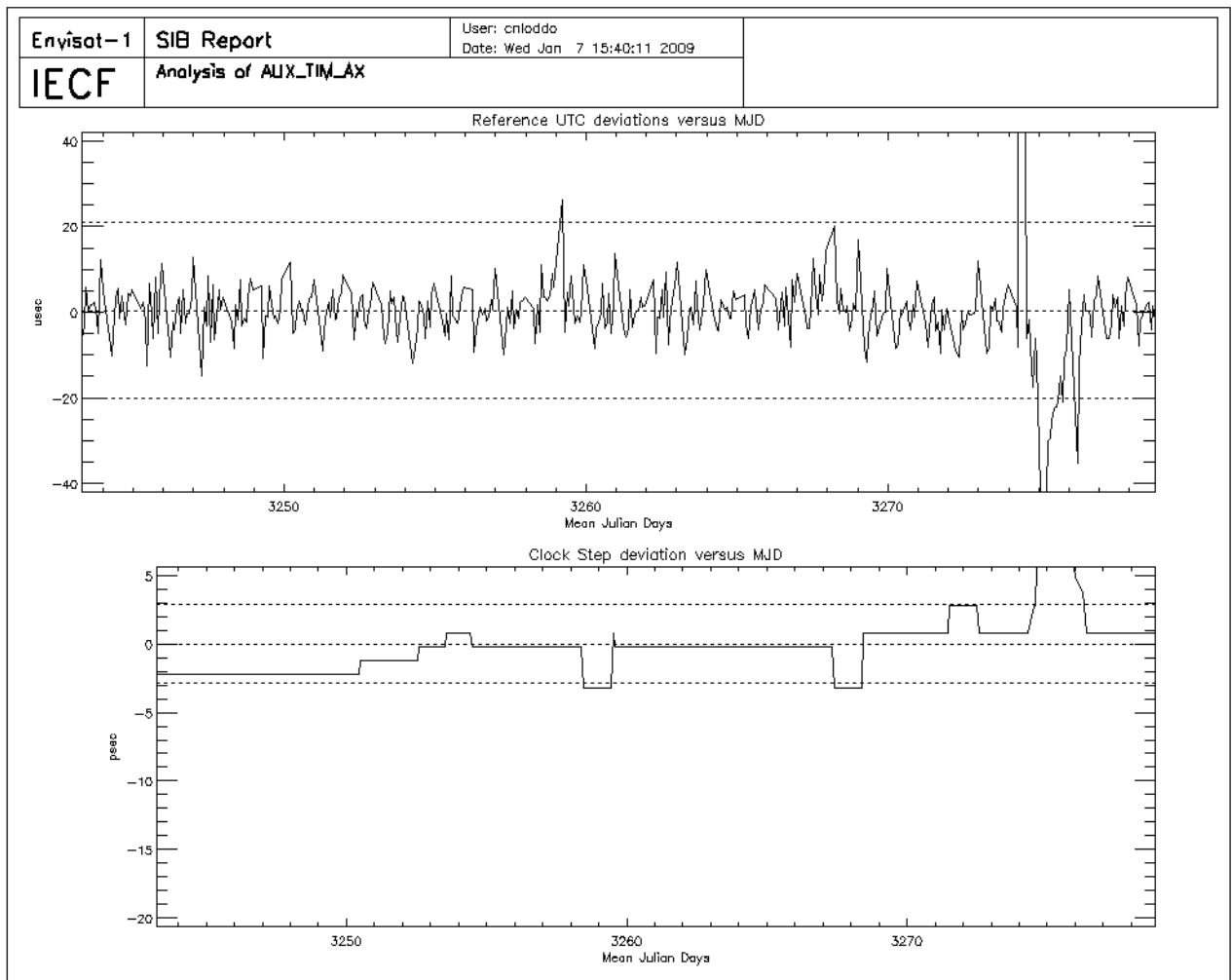
Figure 11: UTC deviations and ICU clock period for cycle 74
