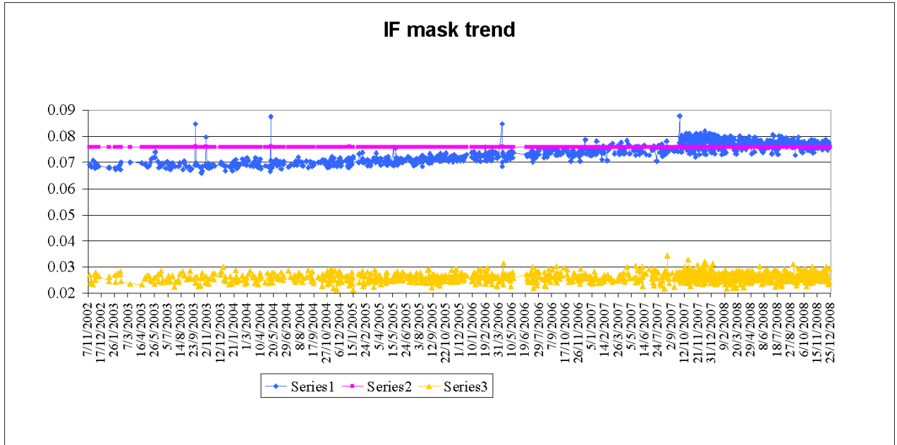
Figure 7: Evolution of the IF mask related parameters for valid IF masks retrieved up to cycle 74
