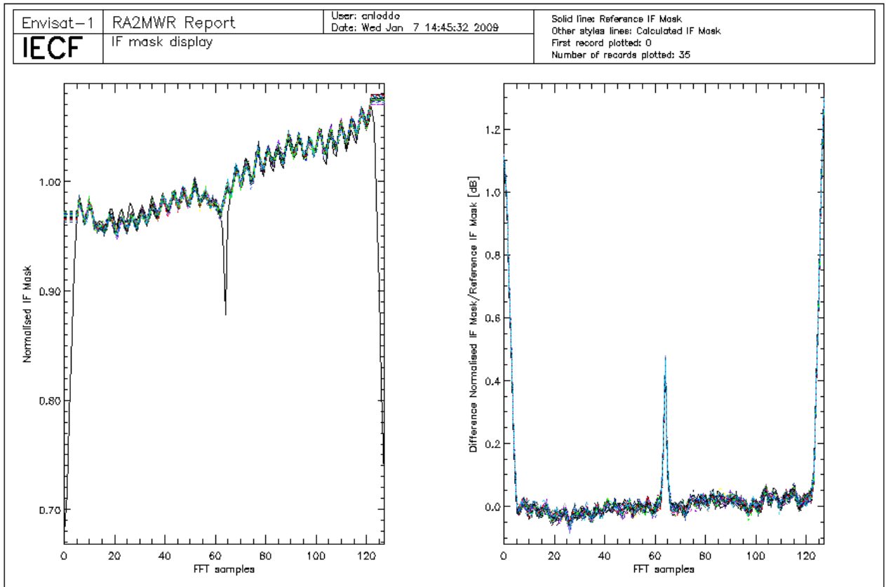
Figure 5: Valid IF masks retrieved during cycle 74 plotted together with the on-ground reference.
