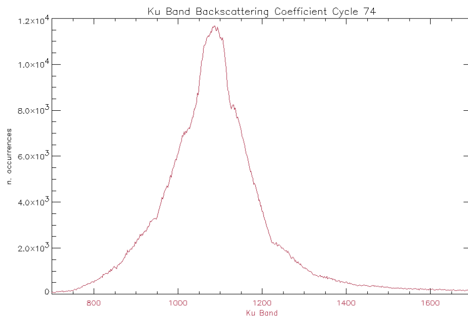
Figure 31: Histogram of Ku Band Backscattering Coefficient for cycle 74
