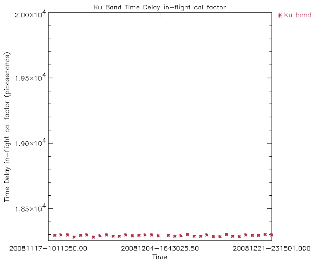
Figure 14: Ku Band in-flight time delay calibration factor for cycle 74 (averaged per day)
