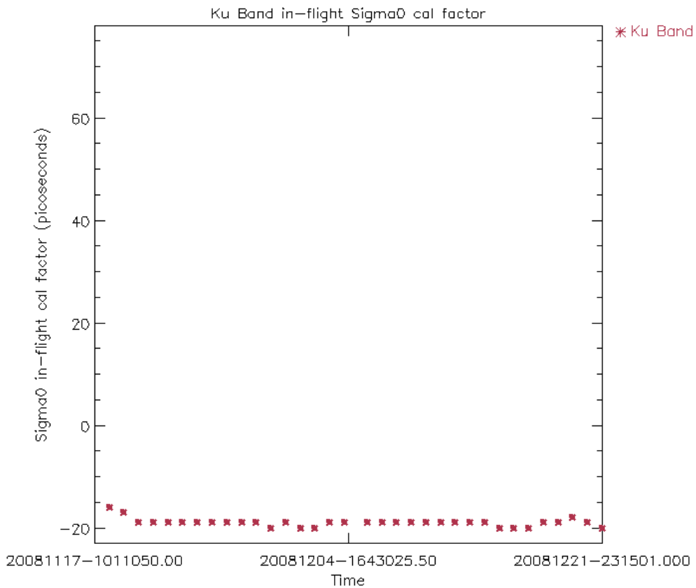
Figure 15: Ku Band in-flight Sigma0 calibration factor for cycle 74 (averaged per day)
