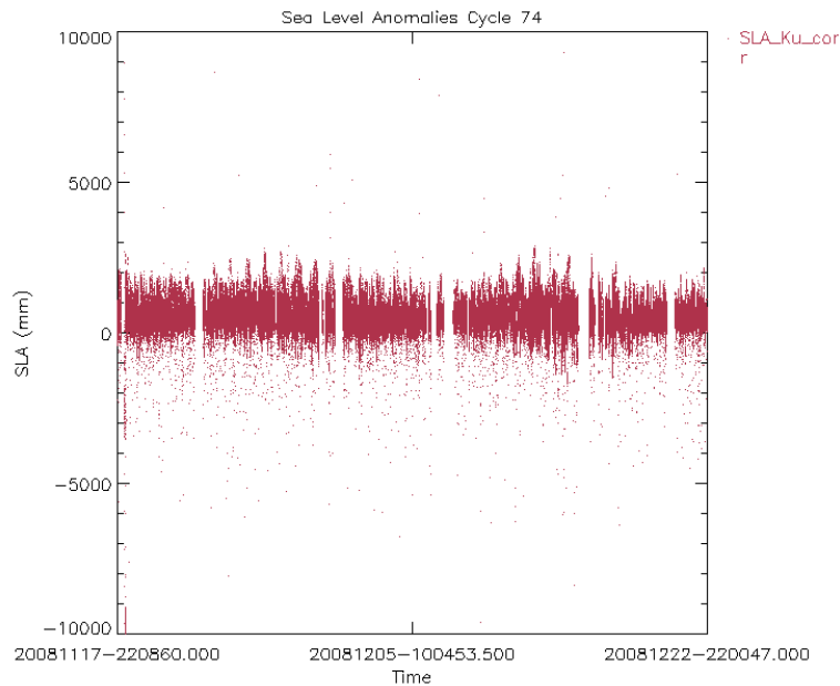
Figure 27A: Sea Level Anomalies Cycle 74, only MDSRs with valid DORIS Flag
