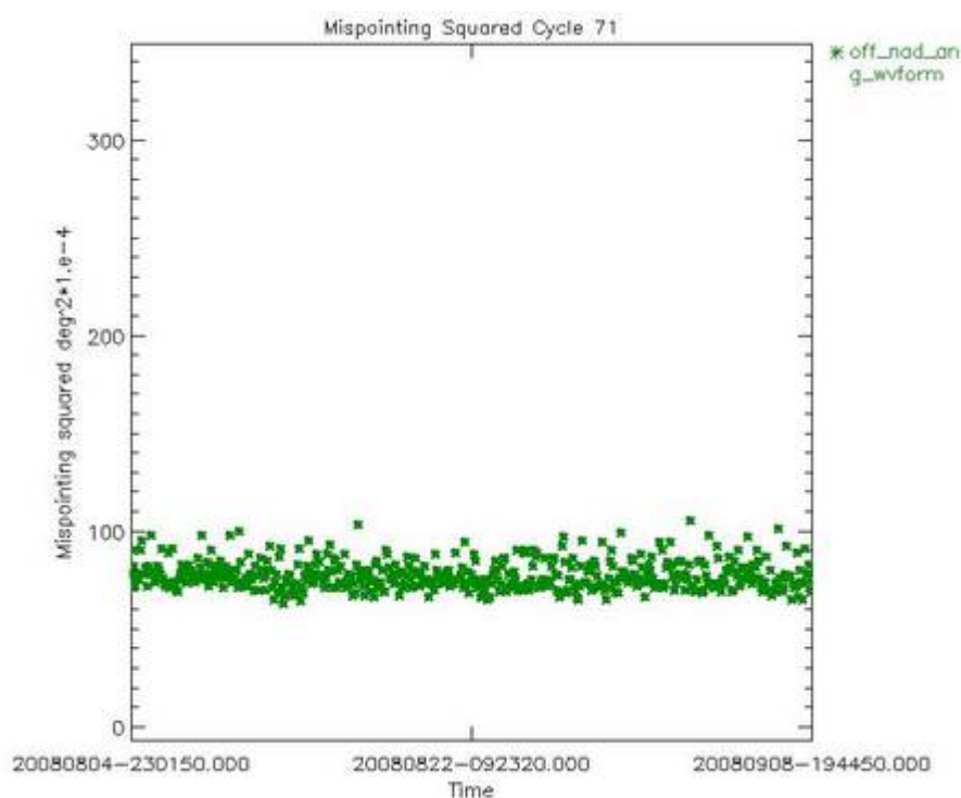
Figure 19: Smoothed mispointing squared trend for cycle 71 ( \text{deg}^2 \cdot 10^{-4} )
