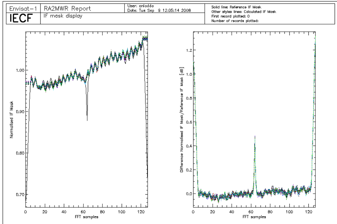
Figure 5: Valid IF masks retrieved during cycle 71 plotted together with the on-ground reference.
