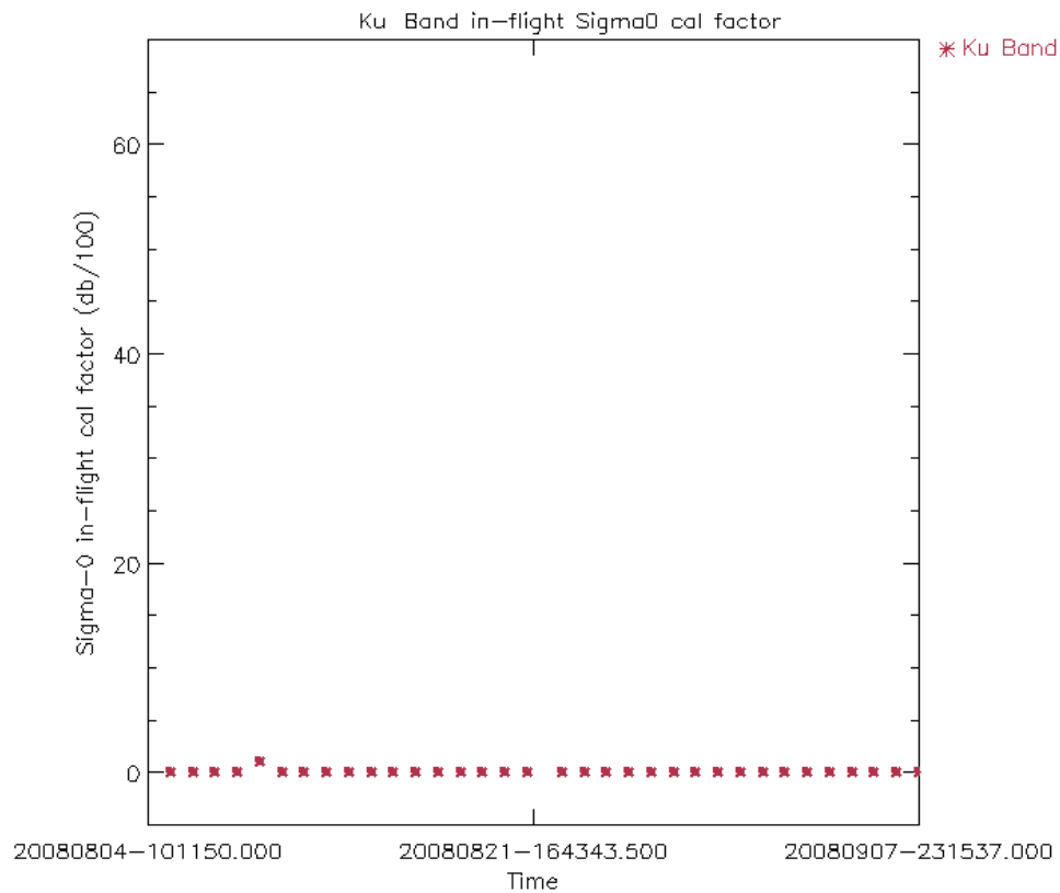
Figure 15: Ku Band in-flight Sigma0 calibration factor for cycle 71 (averaged per day)
