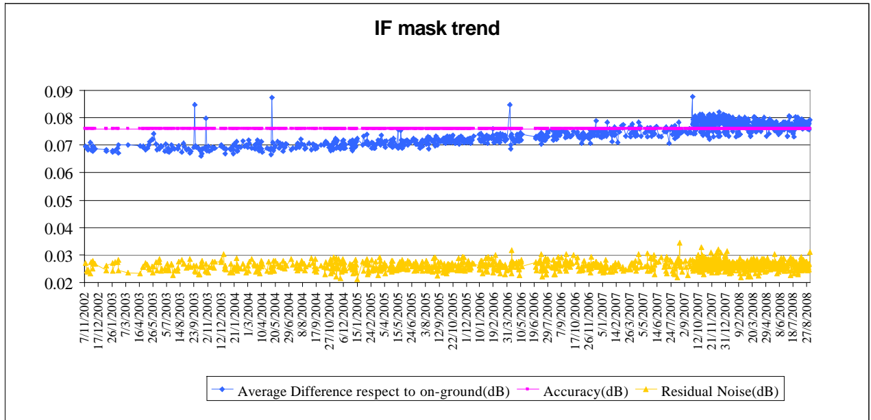
Figure 7: Evolution of the IF mask related parameters for valid IF masks retrieved up to cycle 71
