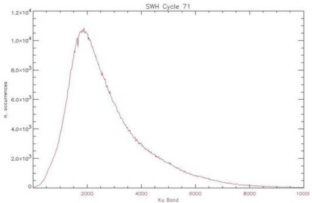
Figure 28: Histogram of Ku Band SWH for cycle 71
