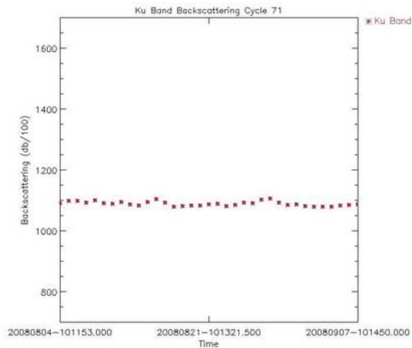
Figure 32: Ku Band Sigma_0 daily average for cycle 71 (dB/100)
