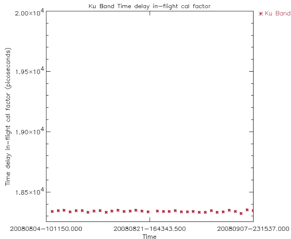
Figure 14: Ku Band in-flight time delay calibration factor for cycle 71 (averaged per day)
