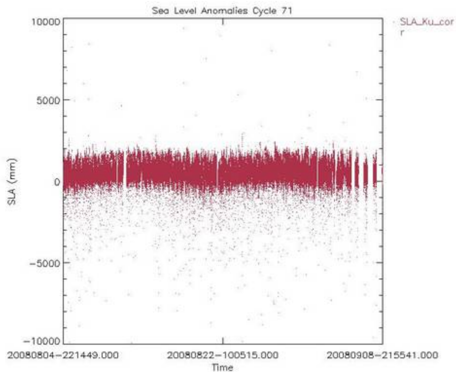
Figure 27B: Sea Level Anomalies Cycle 71, only MDSRs with valid DORIS Flag
