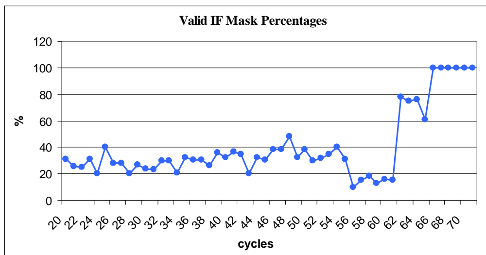
Figure 8: Percentages of valid IF Mask up to cycle 71
