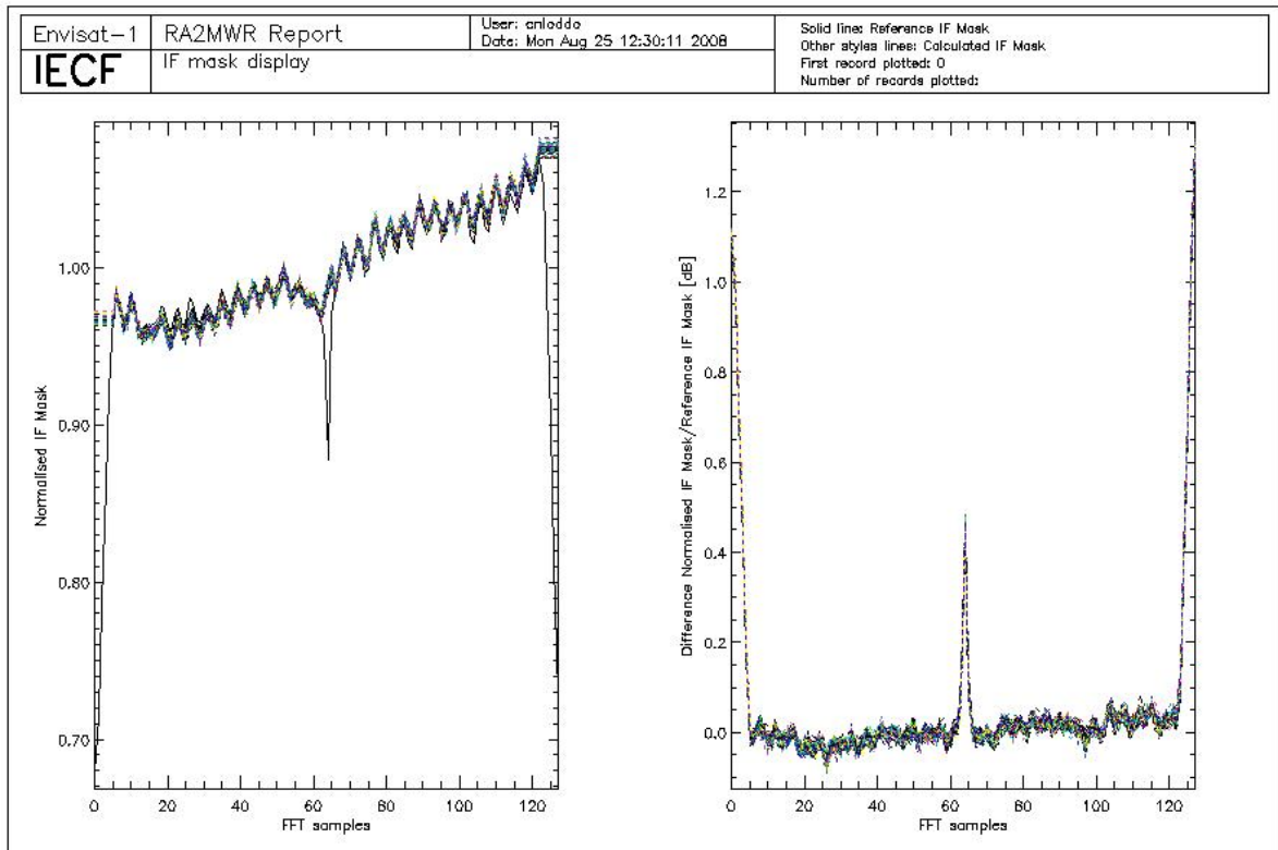
Figure 5: Valid IF masks retrieved during cycle 70 plotted together with the on-ground reference.
