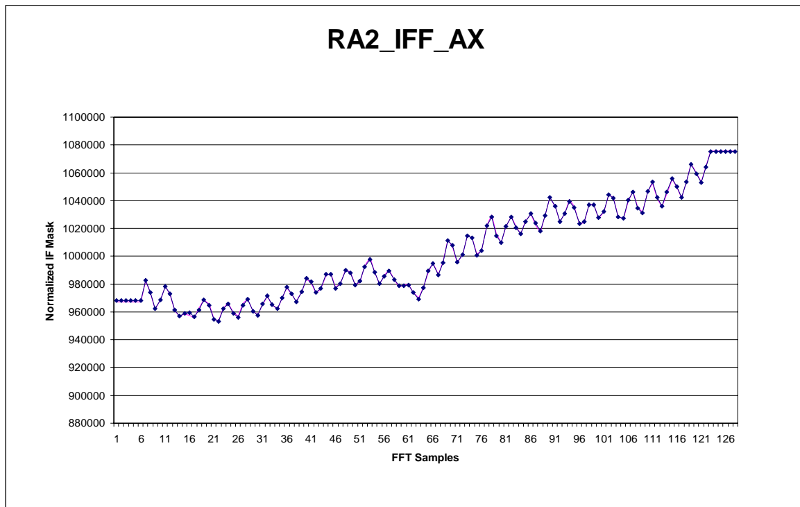
Figure 6: Previous and IF Mask updated on 12 August 2008
