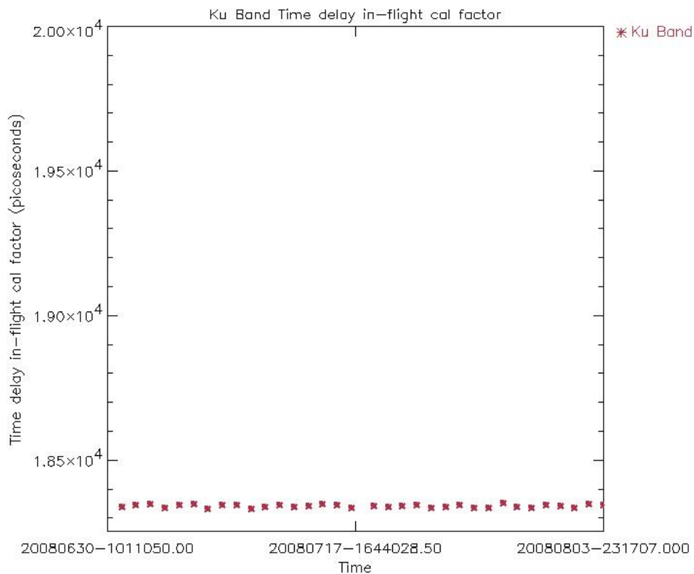
Figure 14: Ku Band in-flight time delay calibration factor for cycle 70 (averaged per day)
