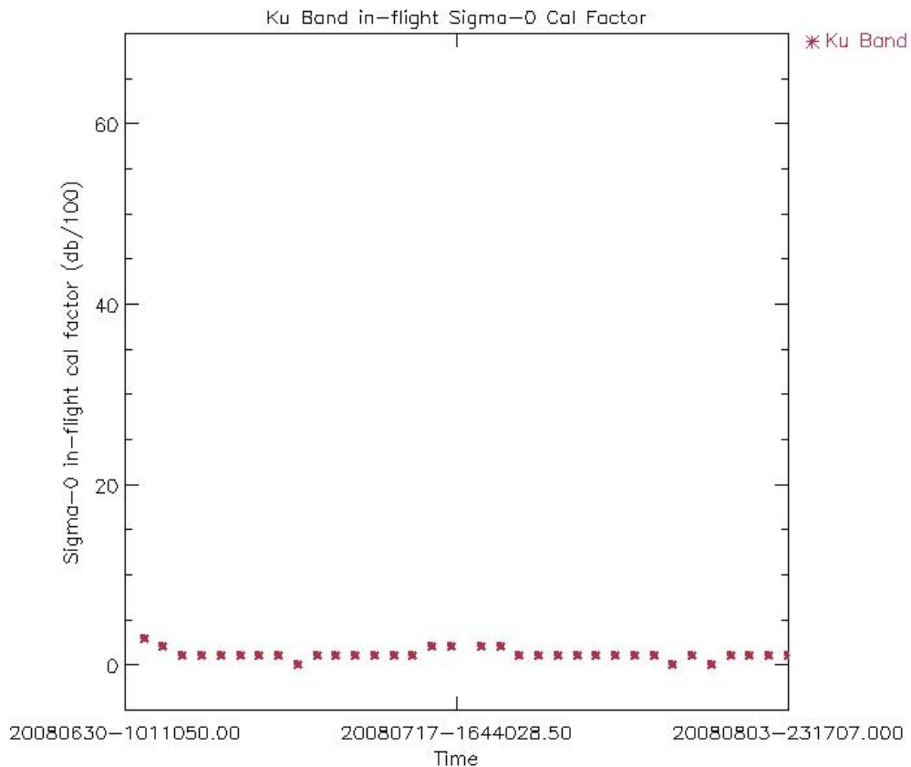
Figure 15: Ku Band in-flight Sigma0 calibration factor for cycle 70 (averaged per day)
