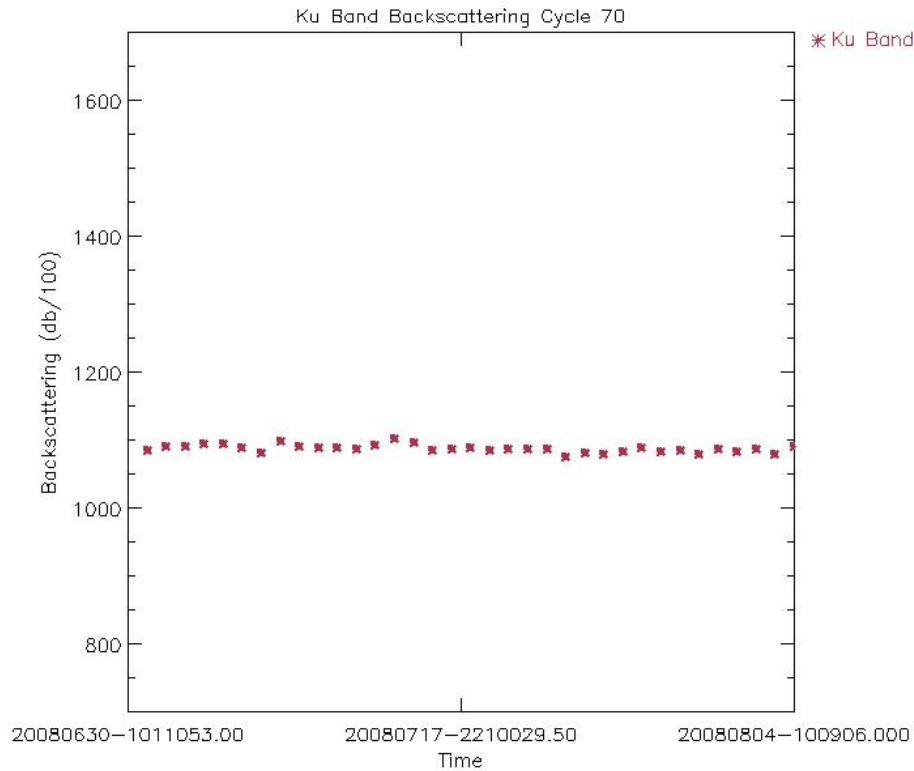
Figure 32: Ku Band Sigma_0 daily average for cycle 70 (dB/100)
