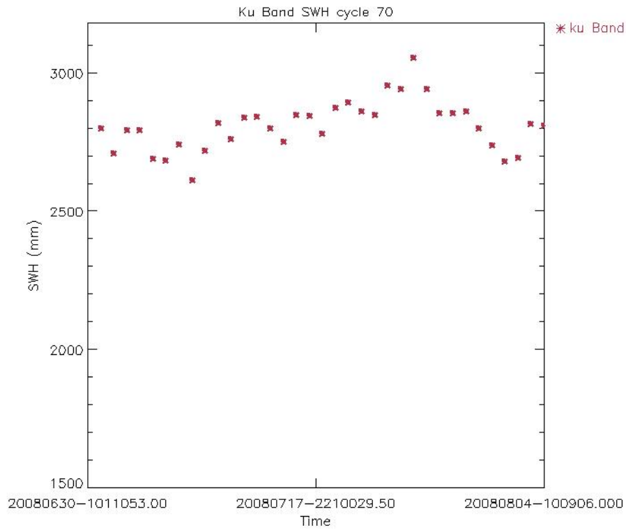
Figure 29: Ku Band SWH daily average for Cycle 70 (mm)
