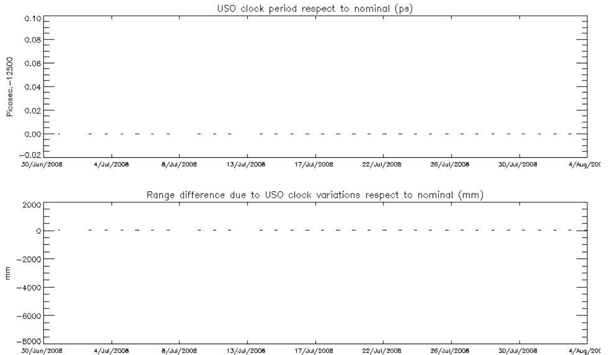
Figure 9: USO clock period (top) and range difference with nominal (bottom) for cycle 70
