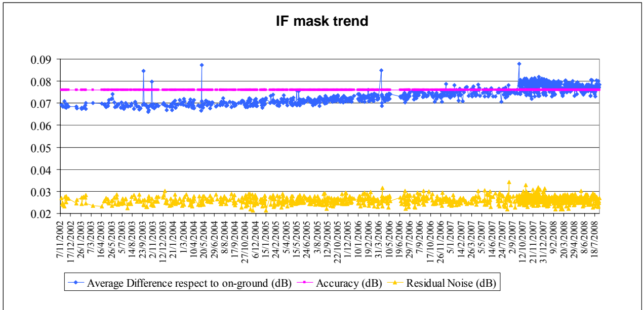
Figure 7: Evolution of the IF mask related parameters for valid IF masks retrieved up to cycle 70
