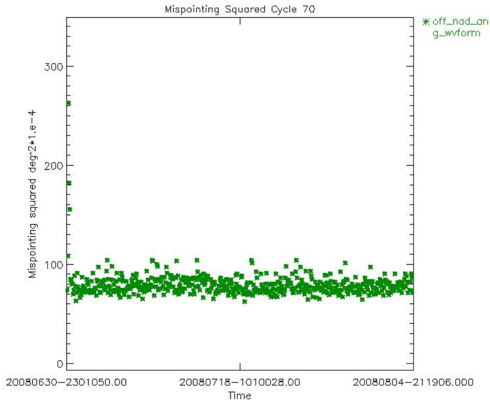
Figure 19: Smoothed mispointing squared trend for cycle 70 (deg 2 *10 -4 )
