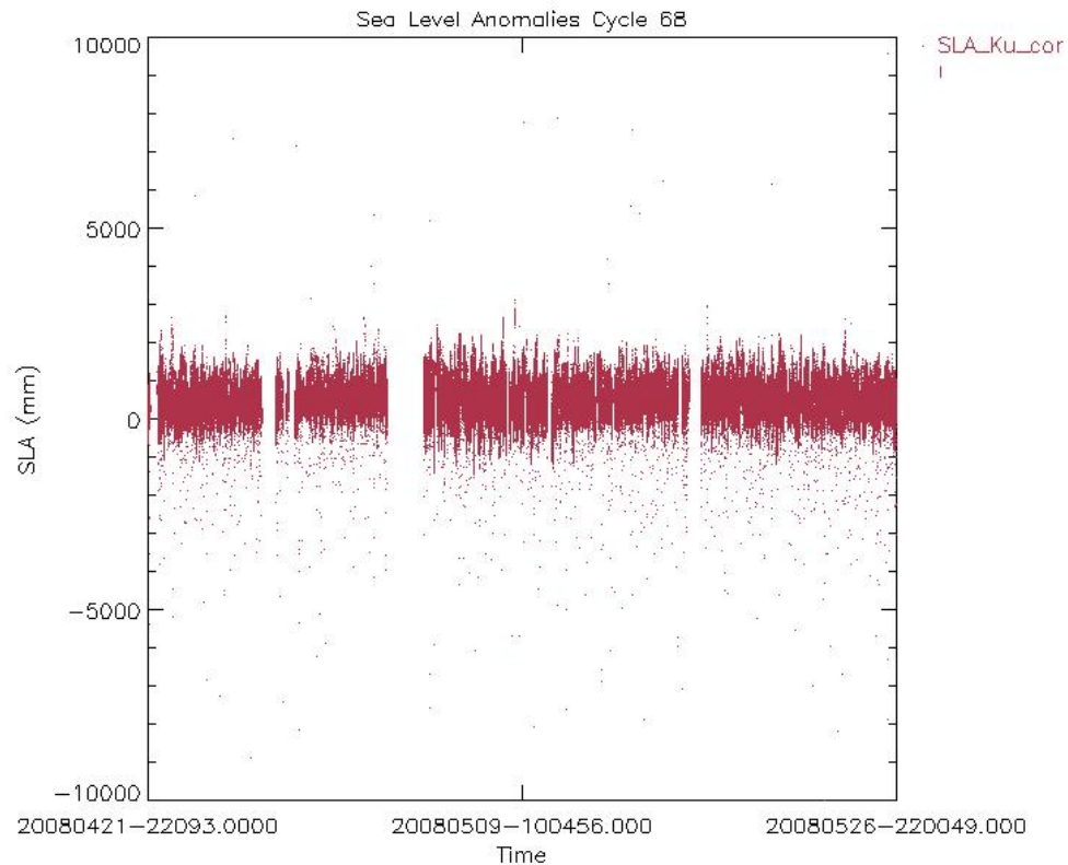
Figure 27B: Sea Level Anomalies Cycle 68, only MDSRs with valid DORIS Flag
