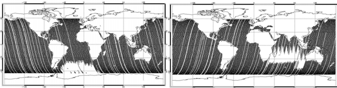
Figure 27: Ascending and Descending passes processed with DORIS on cycle 68
