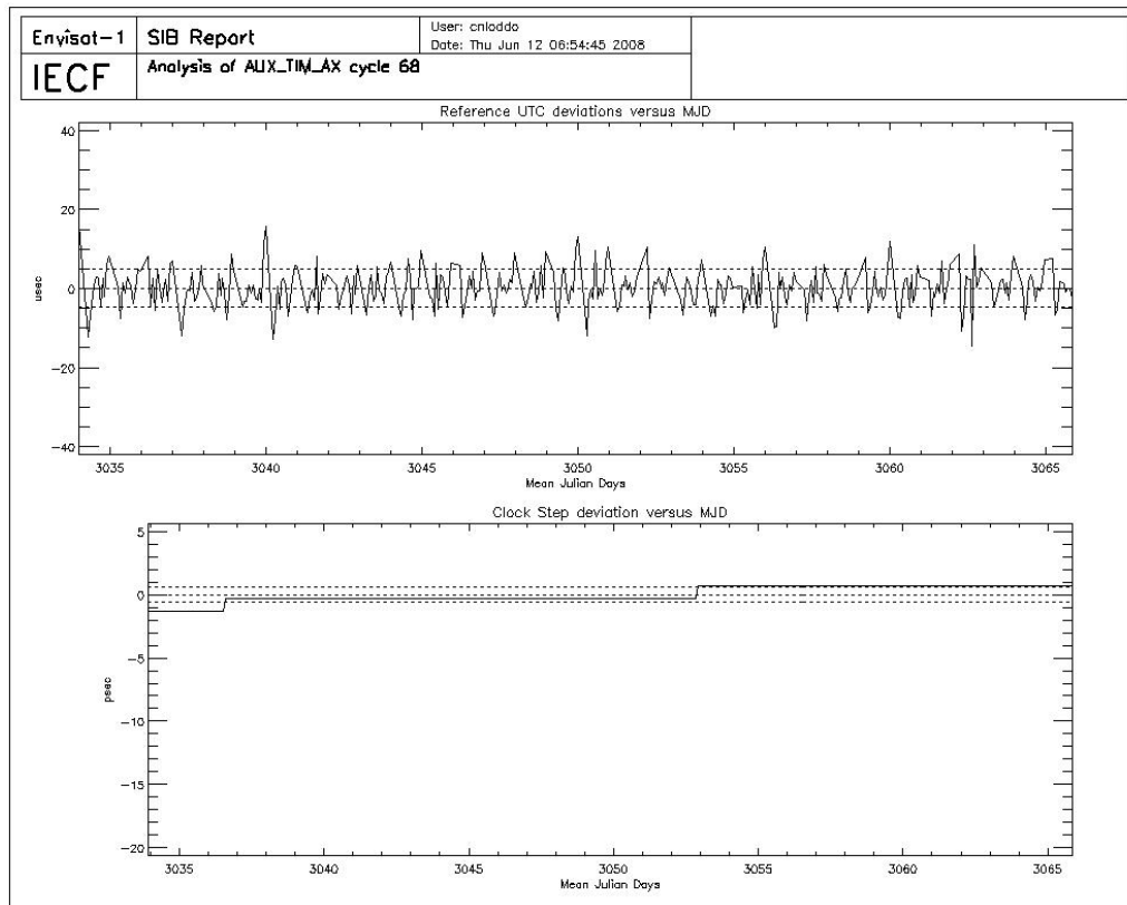
Figure 11: UTC deviations and ICU clock period for cycle 68
