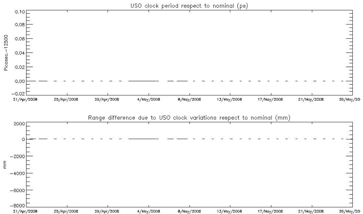
Figure 9: USO clock period (top) and range difference with nominal (bottom) for cycle 68
