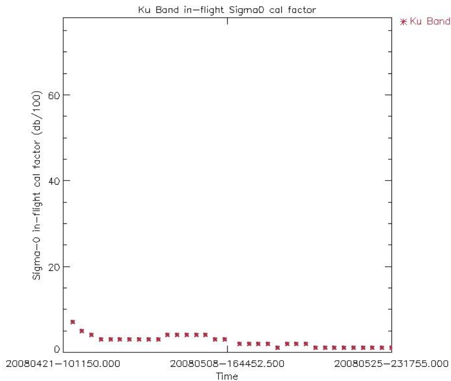
Figure 15: Ku and S Band in-flight Sigma0 calibration factor for cycle 68 (averaged per day)
