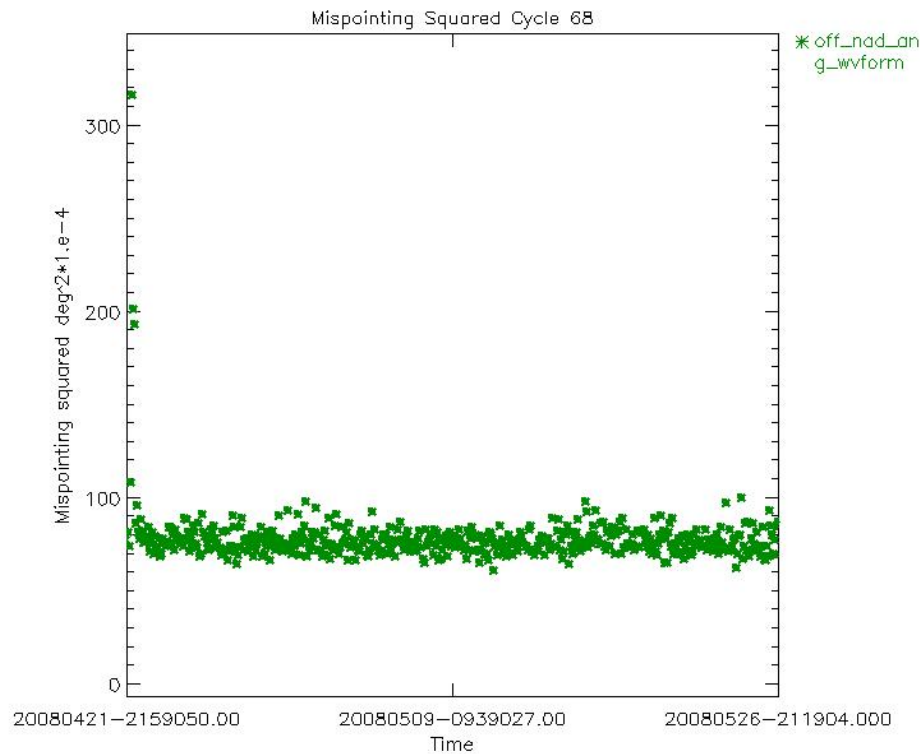
Figure 19: Smoothed mispointing squared trend for cycle 68 (deg 2 *10 -4 )
