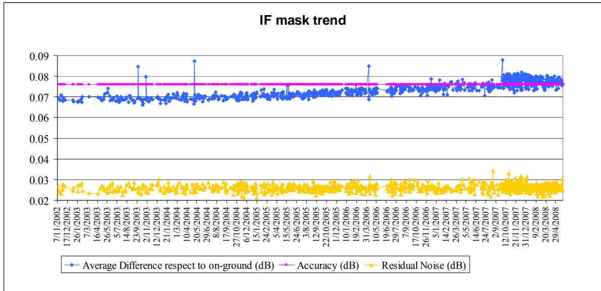
Figure 7: Evolution of the IF mask related parameters for valid IF masks retrieved up to cycle 68
