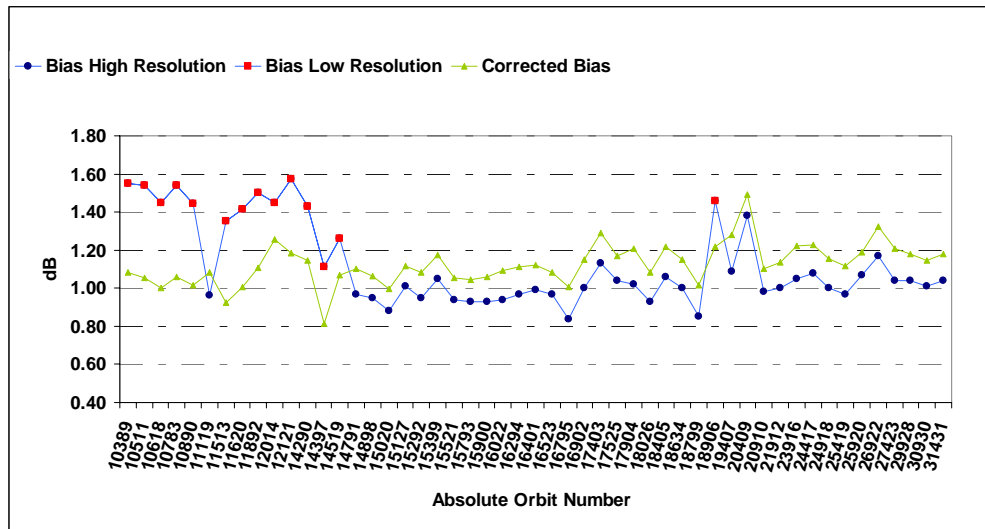
Figure 18: Time behavior of the transponder bias
