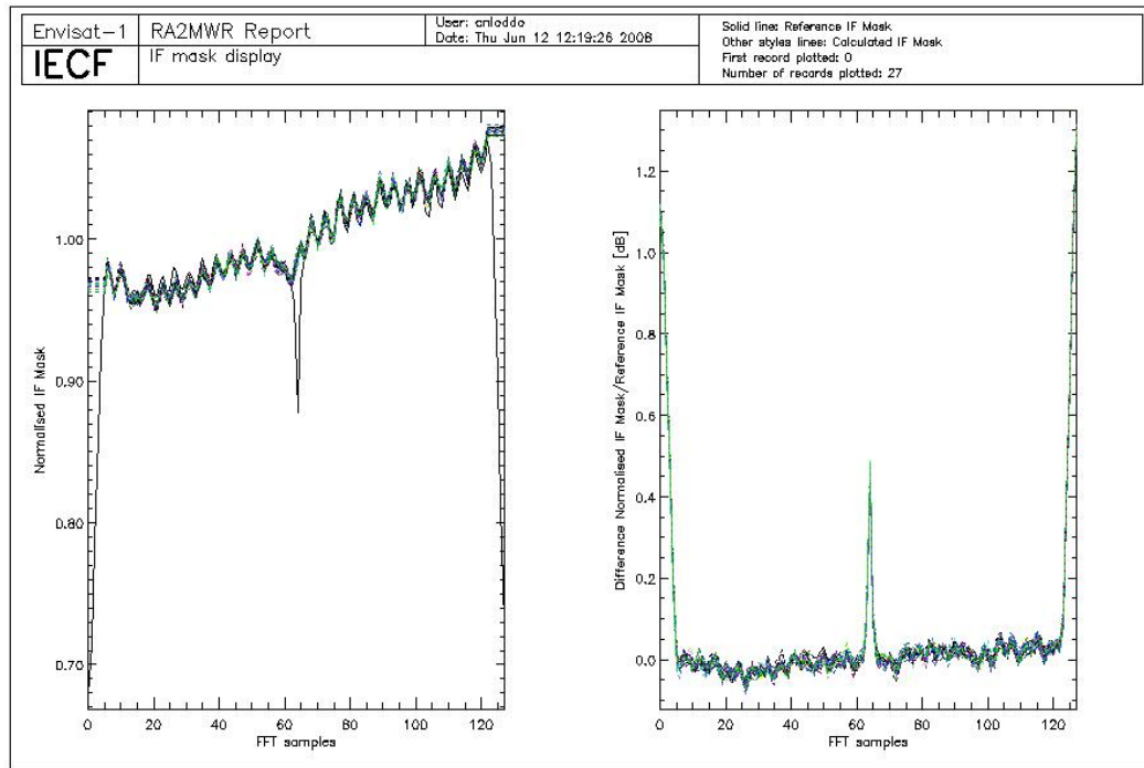
Figure 5: Valid IF masks retrieved during cycle 68 plotted together with the on-ground reference.
