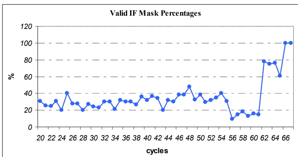
Figure 8: Percentages of valid IF Mask up to cycle 67
