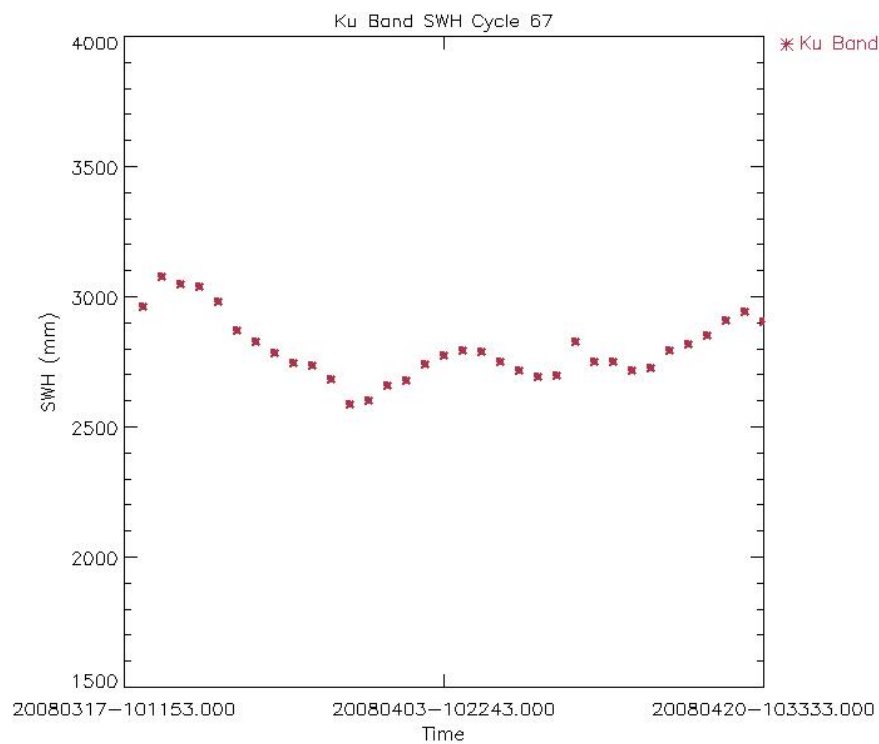
Figure 29: Ku Band SWH daily average for Cycle 67 (mm)
