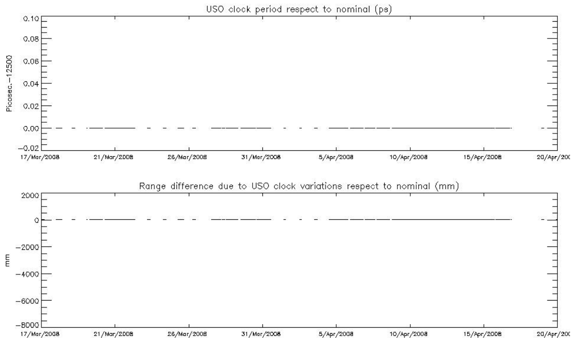
Figure 9: USO clock period (top) and range difference with nominal (bottom) for cycle 67
