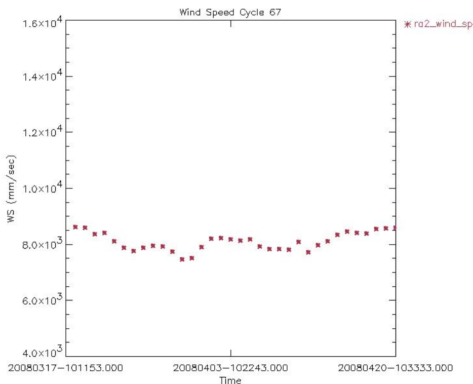
Figure 34: Ku Band Wind Speed daily average for cycle 67 (mm/s)
