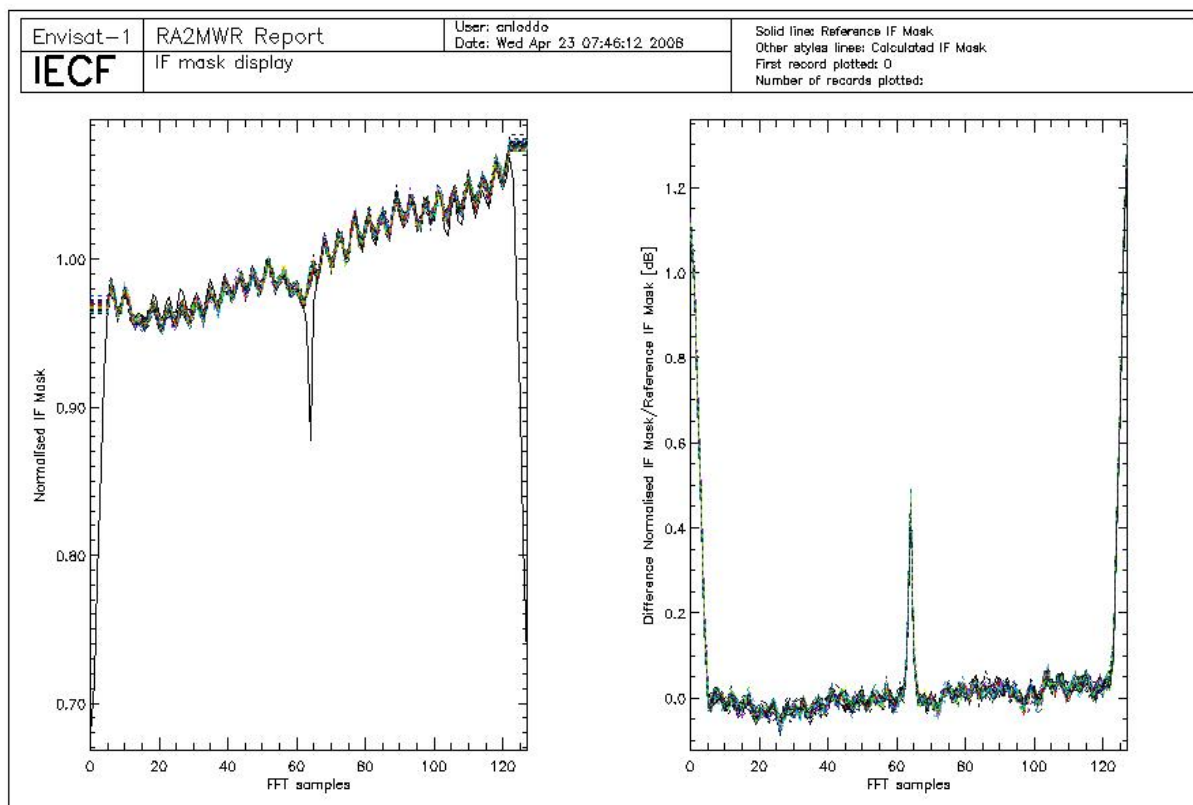
Figure 5: Valid IF masks retrieved during cycle 67 plotted together with the on-ground reference.
