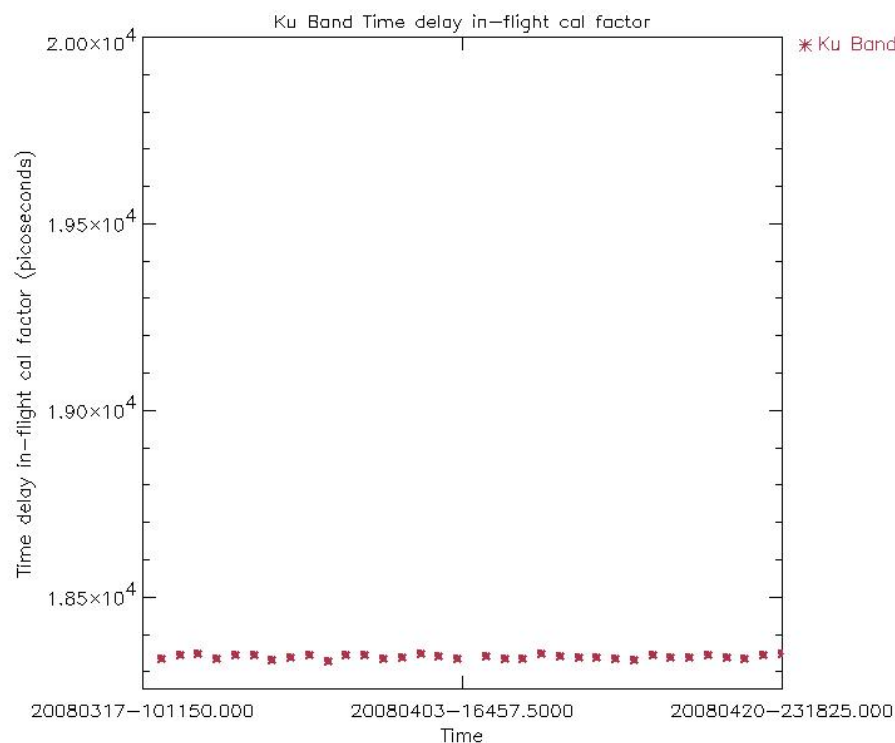
Figure 14: Ku and S Band in-flight time delay calibration factor for cycle 67 (averaged per day)
