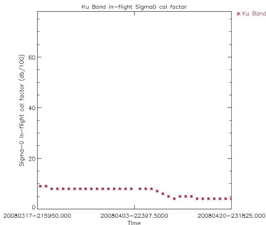
Figure 15: Ku and S Band in-flight Sigma0 calibration factor for cycle 67 (averaged per day)
