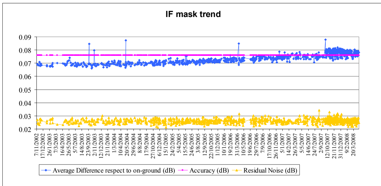
Figure 7: Evolution of the IF mask related parameters for valid IF masks retrieved up to cycle 67
