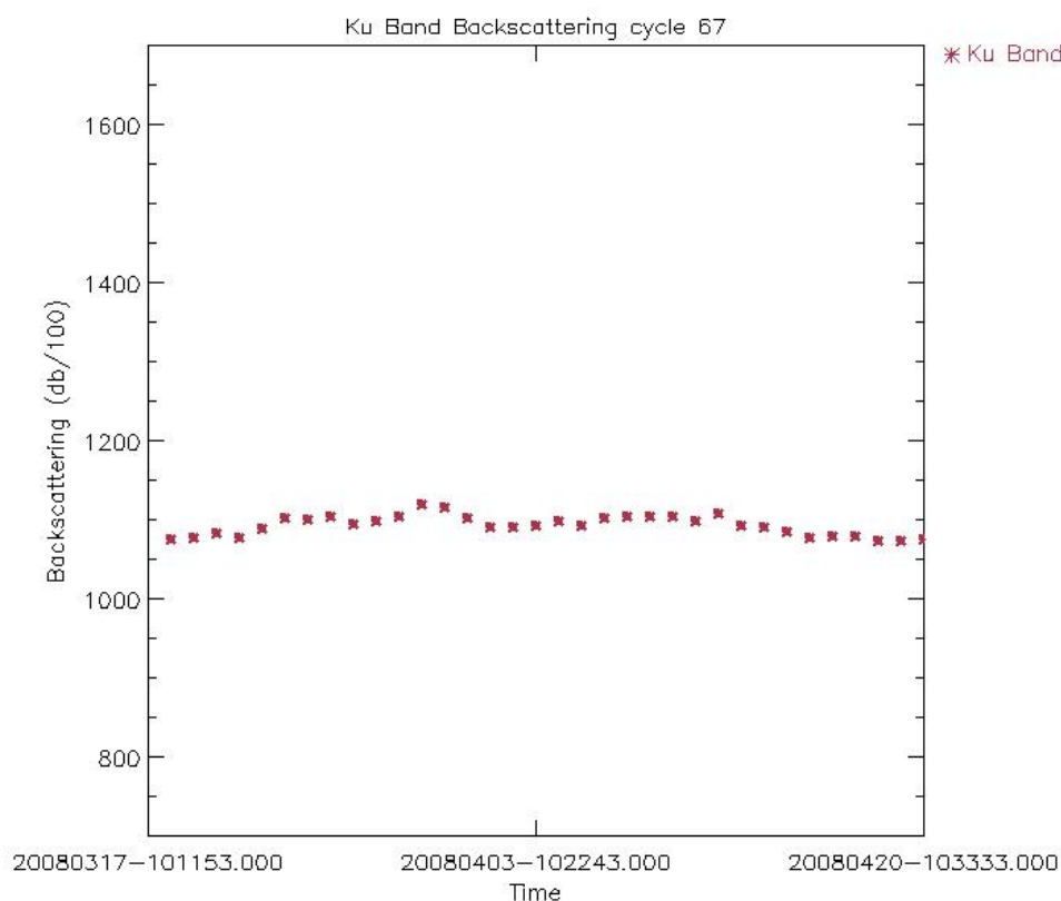
Figure 32: Ku Band Sigma_0 daily average for cycle 67 (dB/100)
