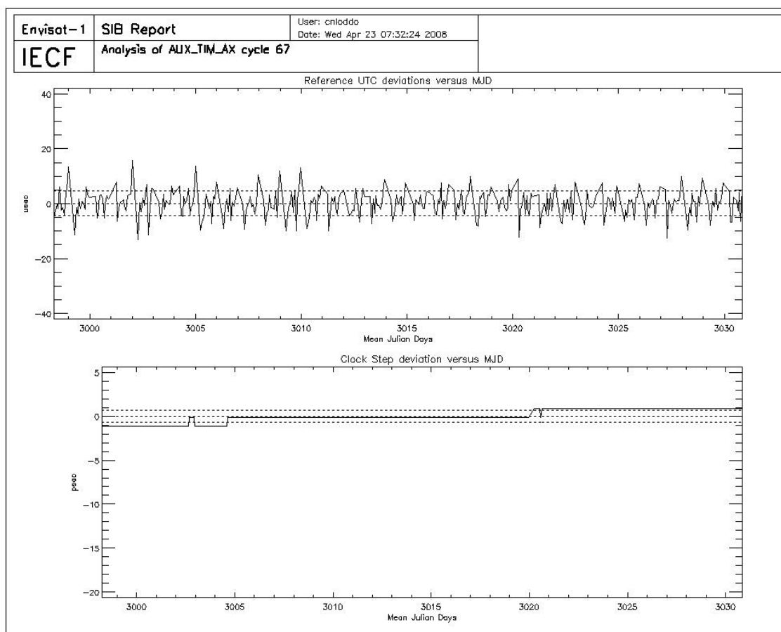
Figure 11: UTC deviations and ICU clock period for cycle 67
