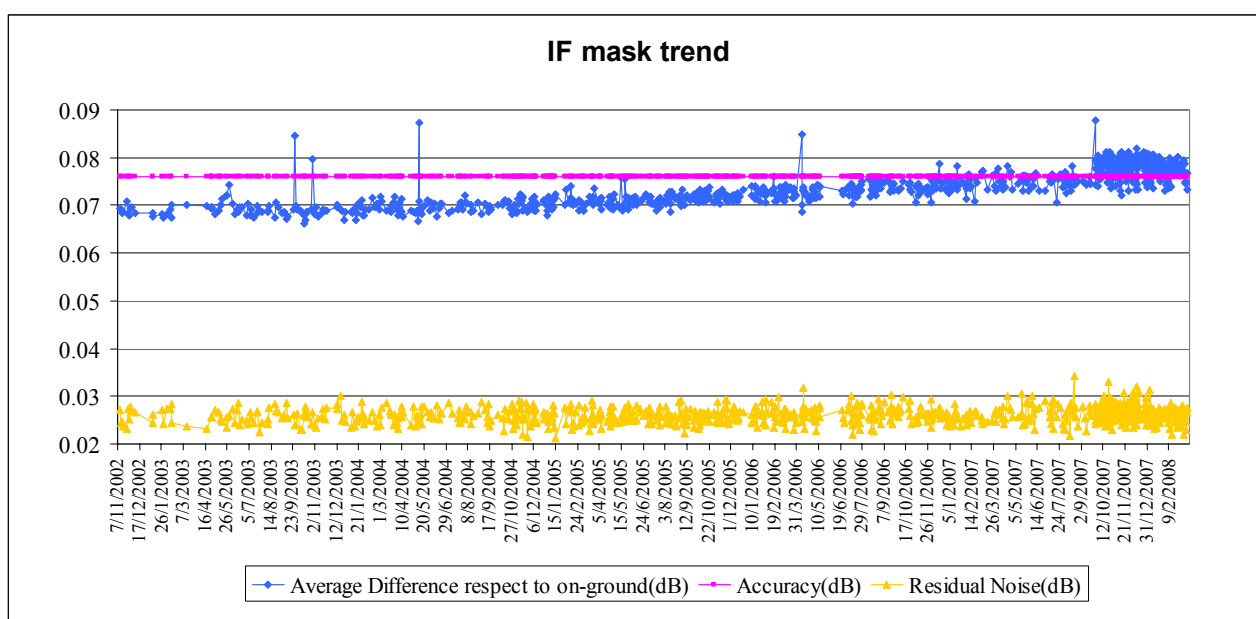
Figure 7: Evolution of the IF mask related parameters for valid IF masks retrieved up to cycle 66
