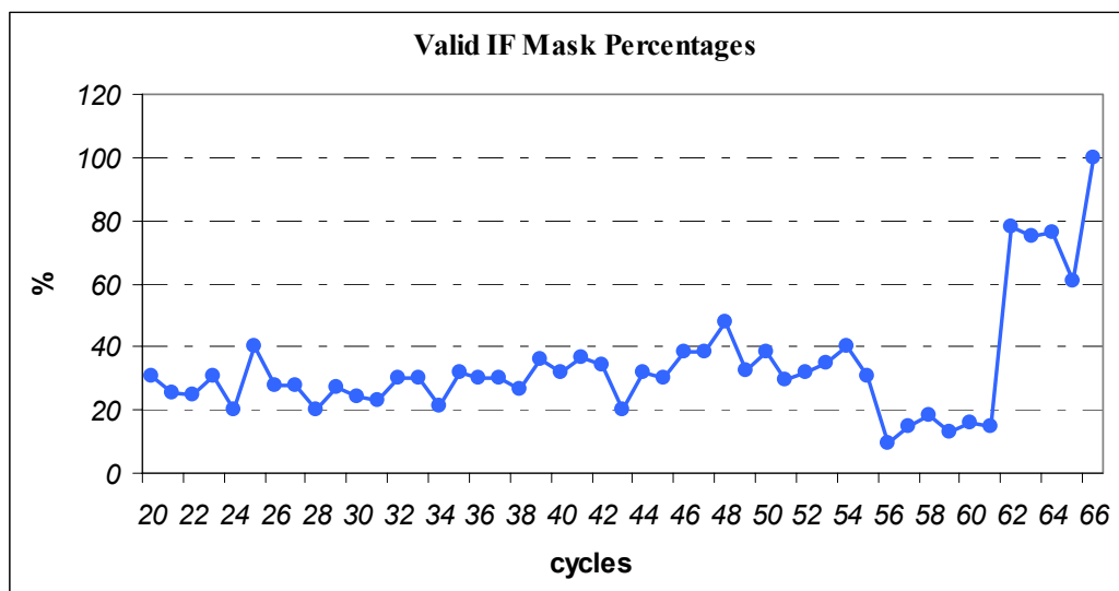
Figure 8: Percentages of valid IF Mask up to cycle 66
