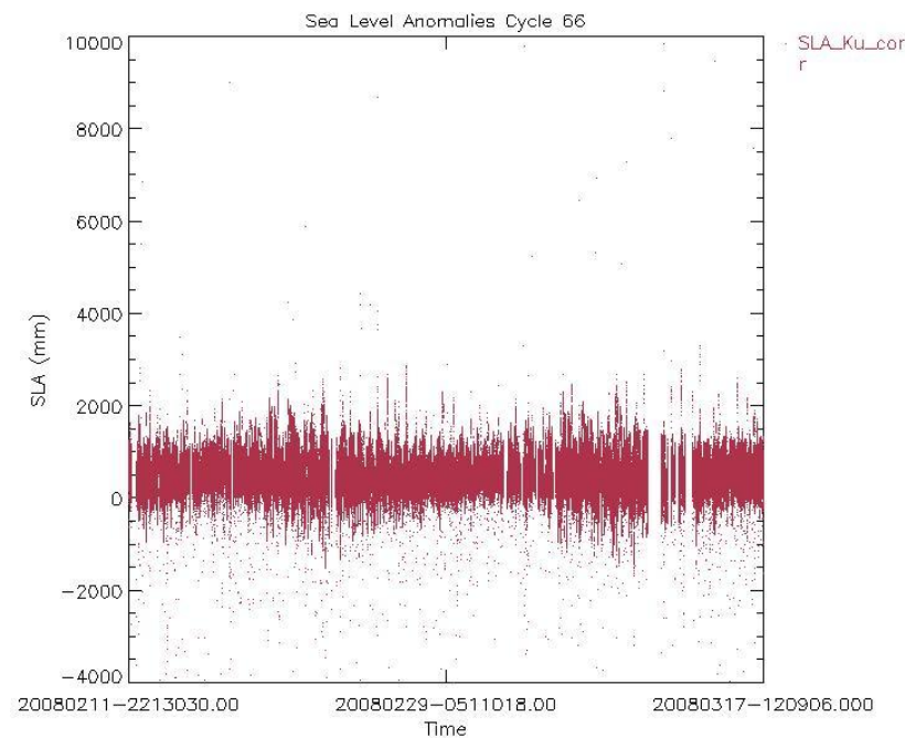
Figure 27B: Sea Level Anomalies Cycle 66, only MDSRs with valid DORIS Flag
