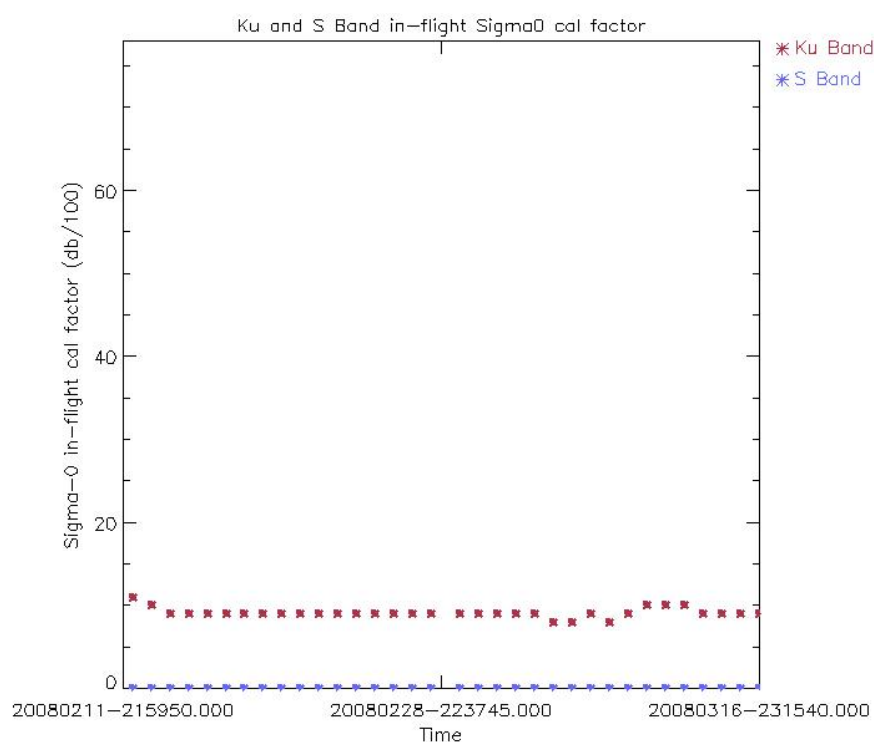
Figure 15: Ku and S Band in-flight Sigma0 calibration factor for cycle 66 (averaged per day)
