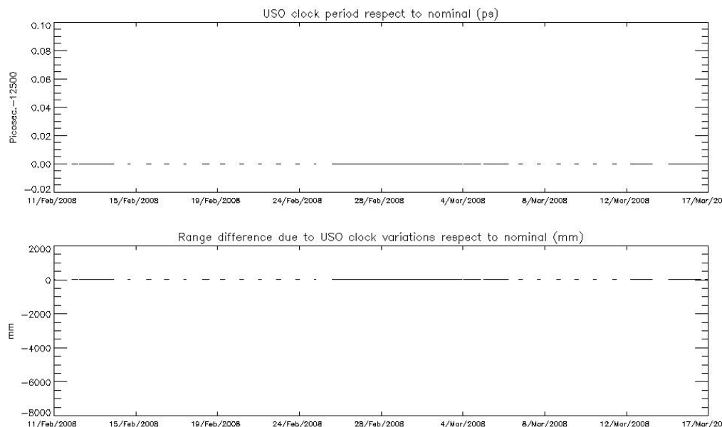
Figure 9: USO clock period (top) and range difference with nominal (bottom) for cycle 66
