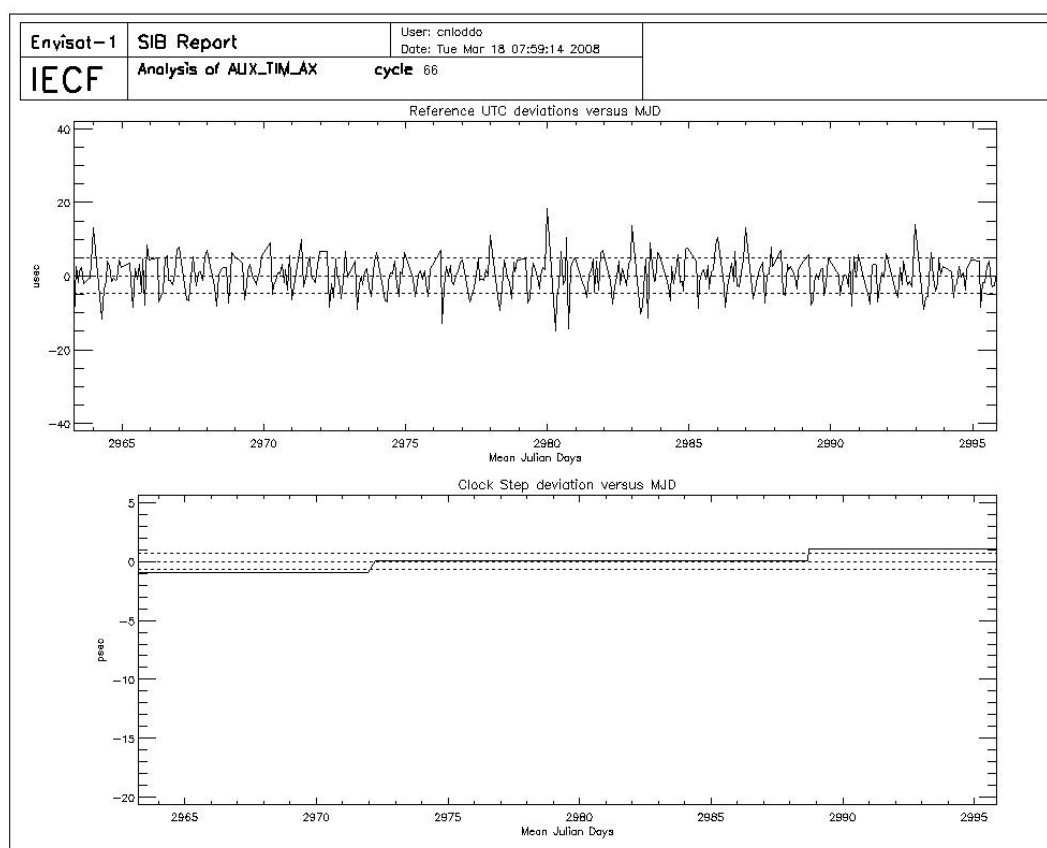
Figure 11: UTC deviations and ICU clock period for cycle 66
