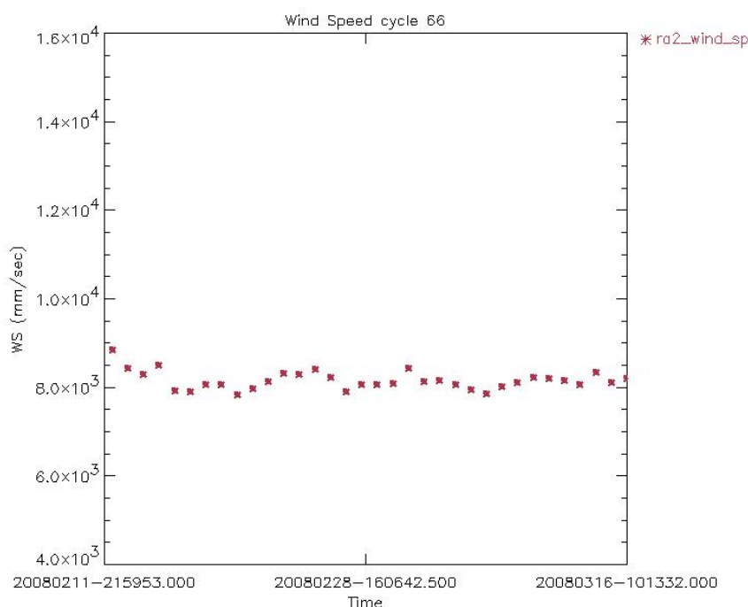
Figure 34: Ku Band Wind Speed daily average for cycle 66 (mm/s)
