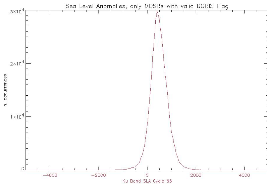
Figure 27C: Histogram of Sea Level Anomalies on Ku Band computed on MDSRs with valid DORIS Flag
