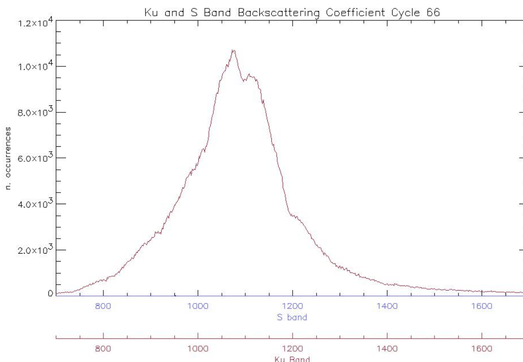
Figure 31: Histogram of Ku and S Band Backscattering Coefficient for cycle 66
