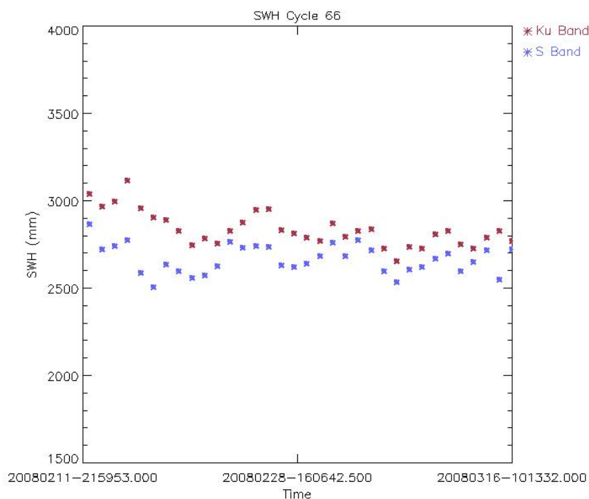
Figure 29: Ku and S SWH daily average for Cycle 66 (mm)
