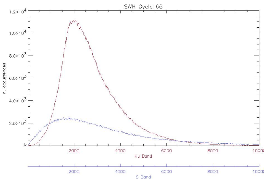
Figure 28: Histogram of Ku and S Band SWH for cycle 66
