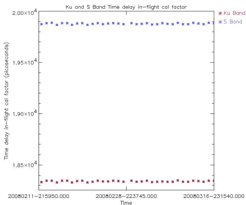
Figure 14: Ku and S Band in-flight time delay calibration factor for cycle 66 (averaged per day)
