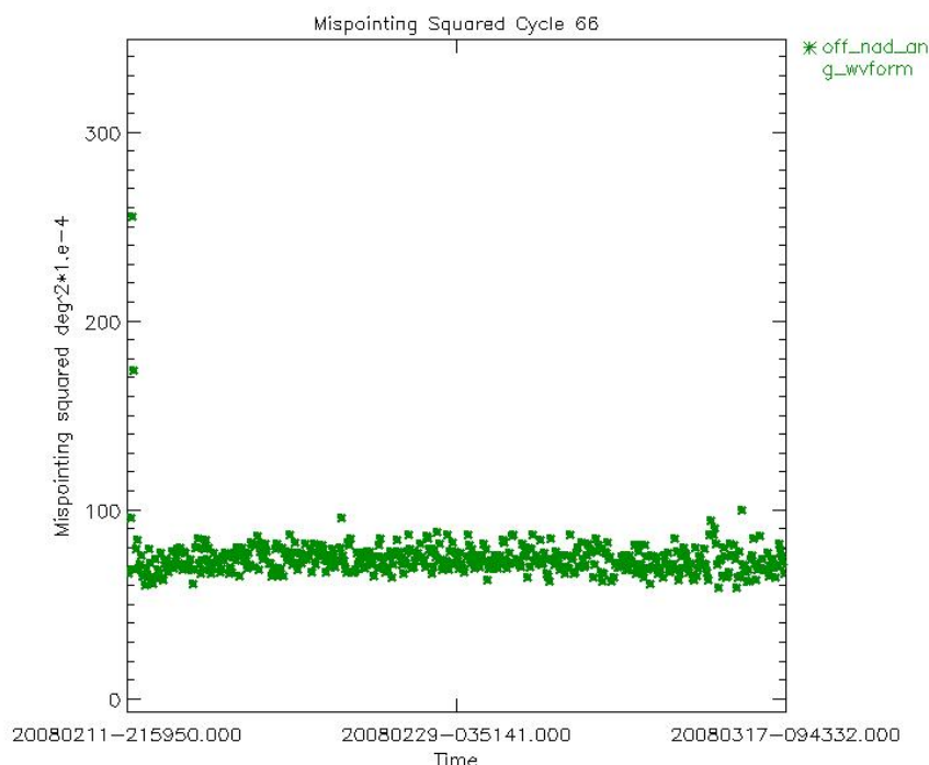
Figure 19: Smoothed mispointing squared trend for cycle 66 ( \text{deg}^2 \cdot 10^{-4} )
