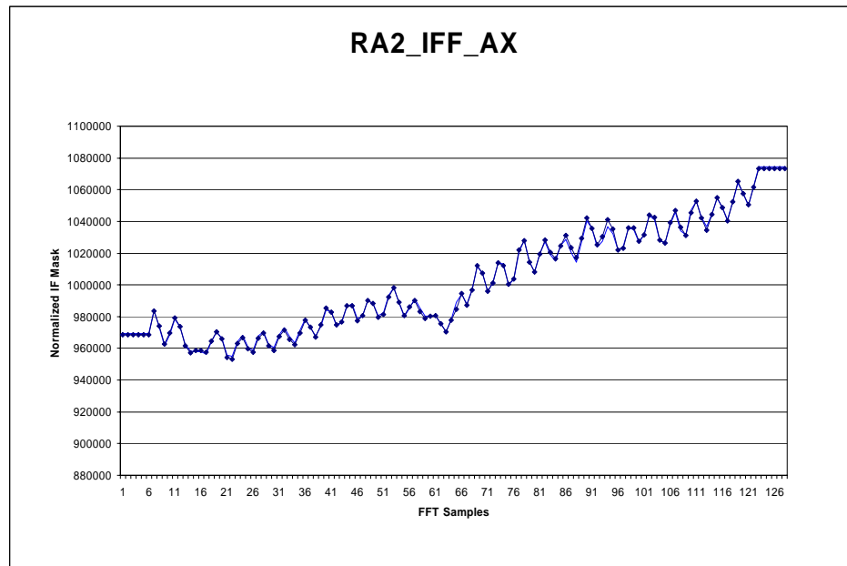
Figure 6: Previous and IF Mask updated on 15th of October 2007
