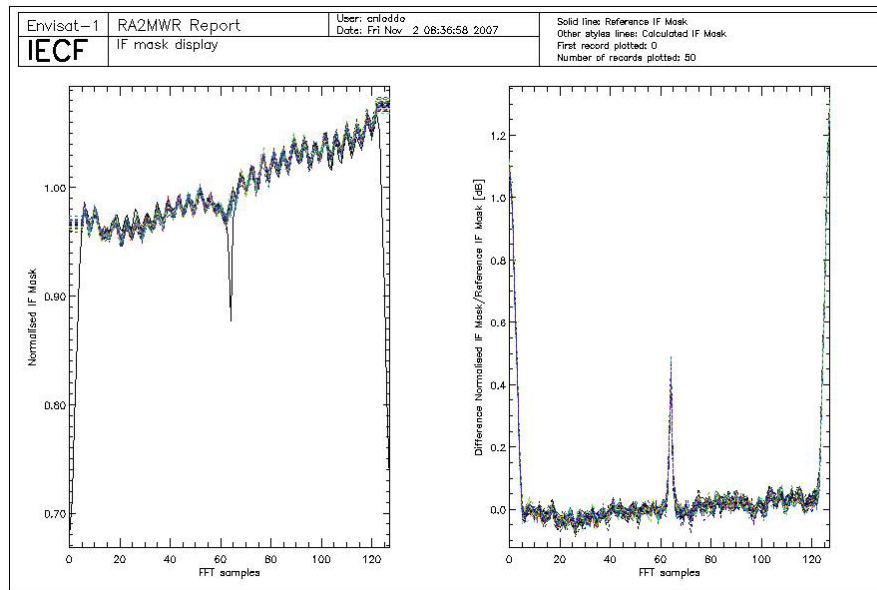
Figure 5: Valid IF masks retrieved during cycle 62 plotted together with the on-ground reference.
