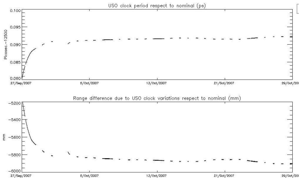
Figure 9: USO clock period for cycle 62
