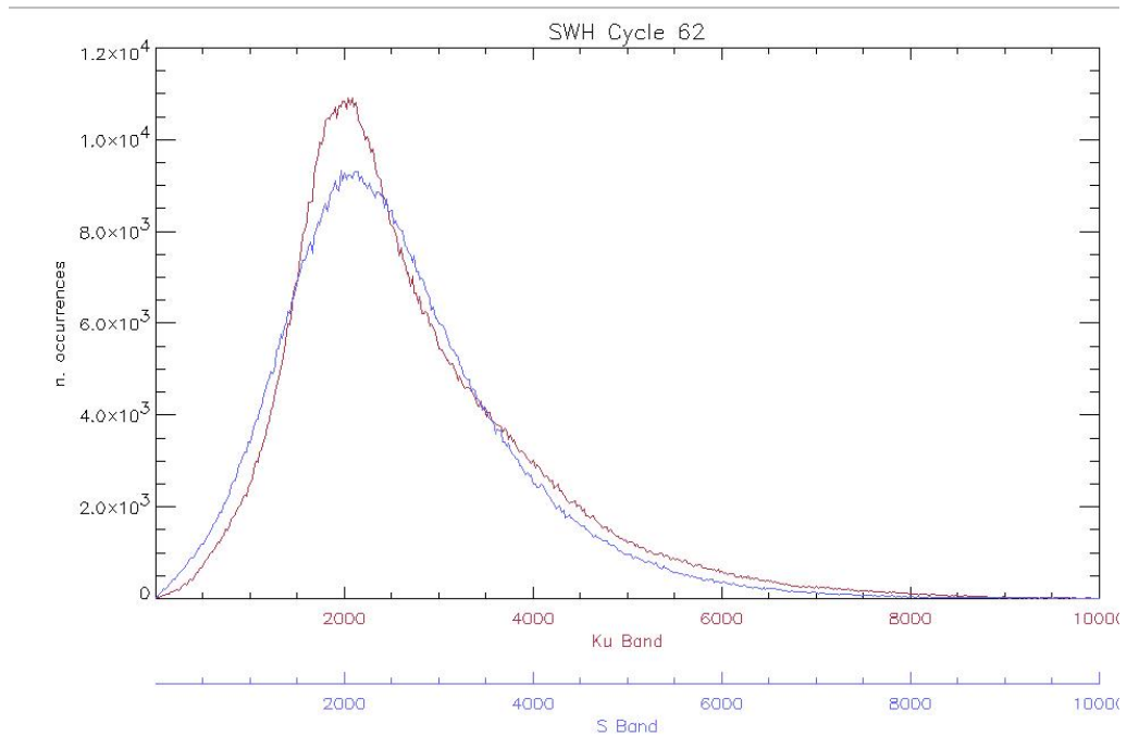
Figure 28: Histogram of Ku and S Band SWH for cycle 62
