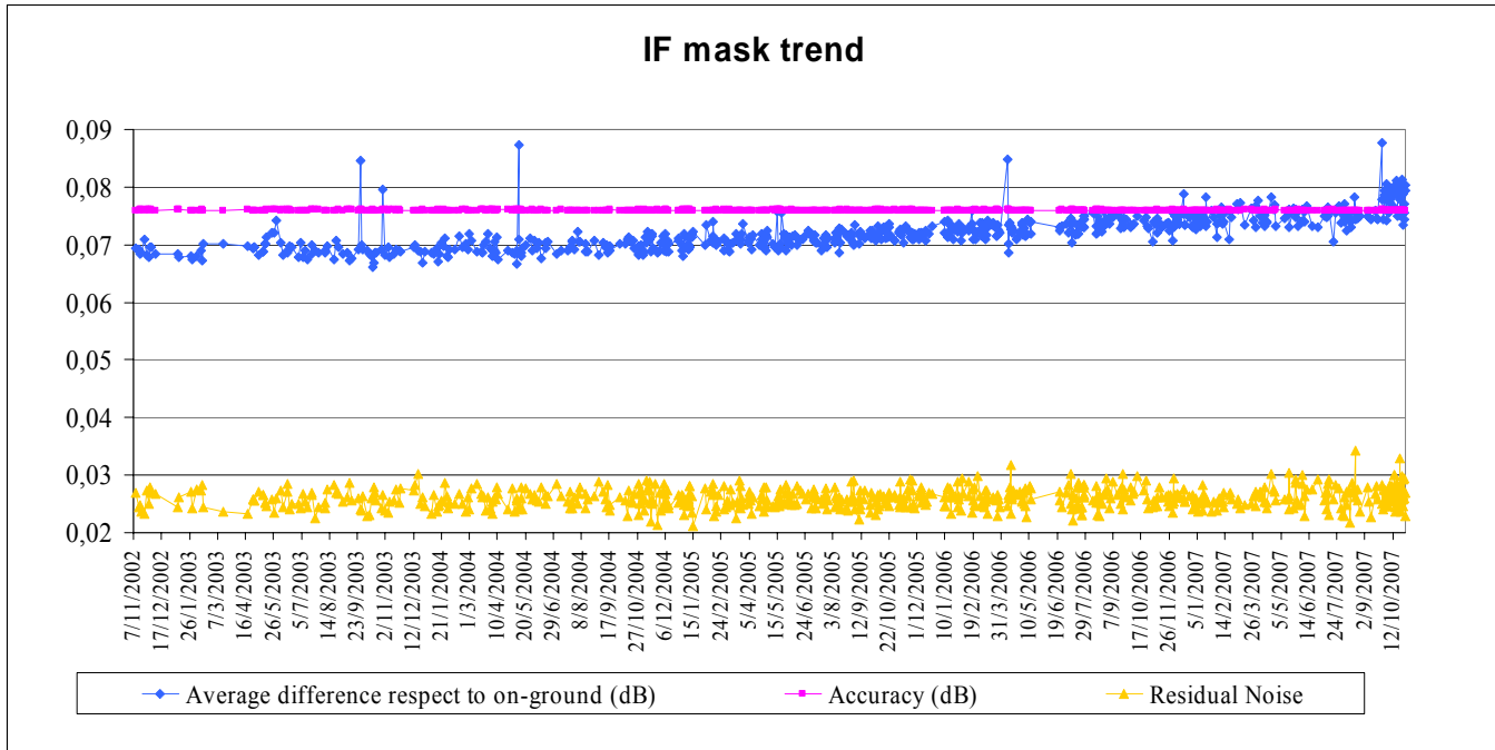
Figure 7: Evolution of the IF mask related parameters for valid IF masks retrieved up to cycle 62
