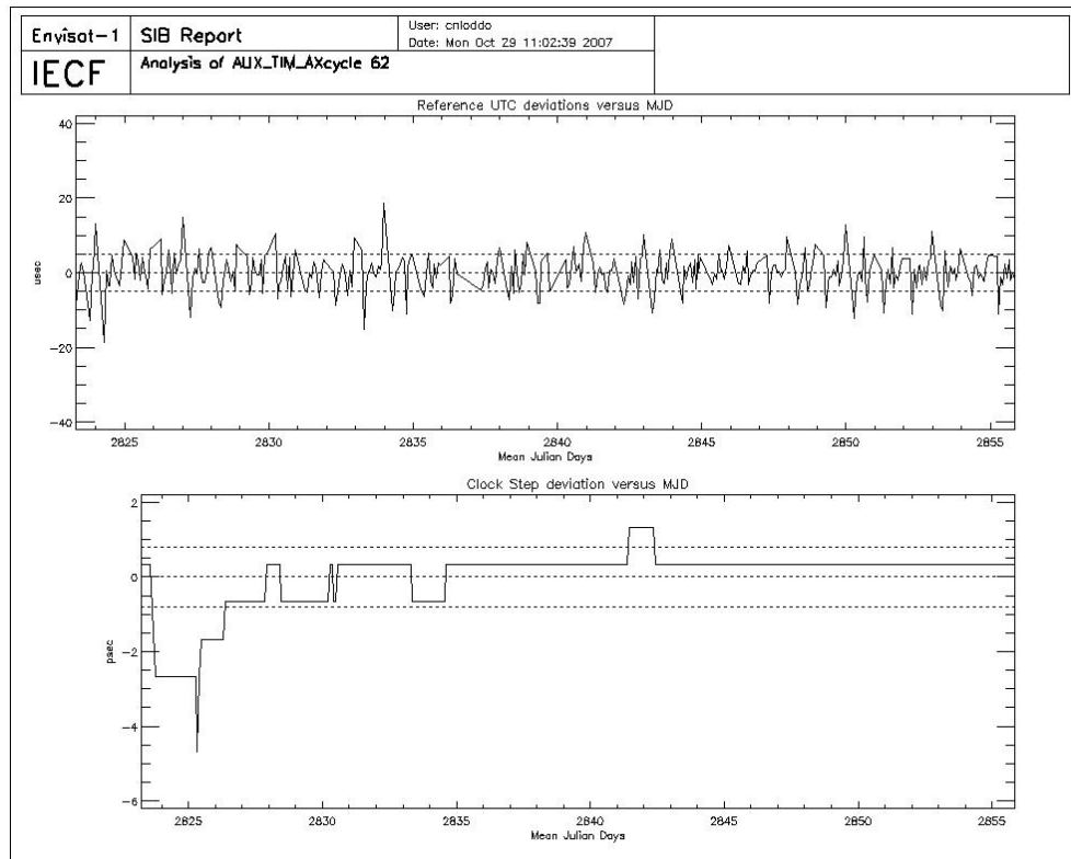
Figure 11: UTC deviations and ICU clock period for cycle 62
