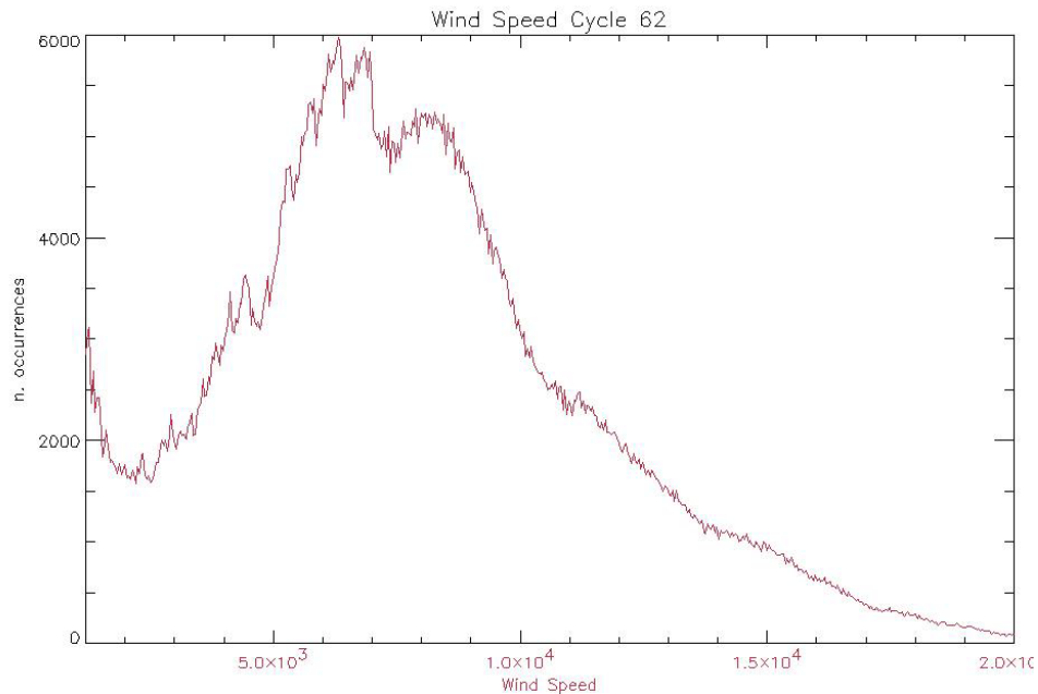
Figure 33: Histogram of Ku Wind Speed for cycle 62 (mm/sec)
