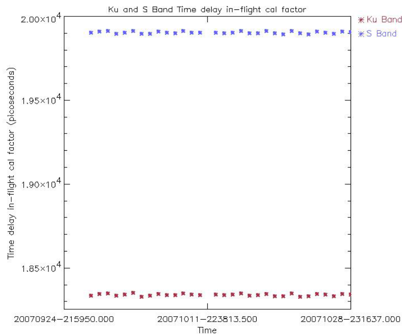
Figure 14: Ku and S Band in-flight time delay calibration factor for cycle 62 (averaged per day)
