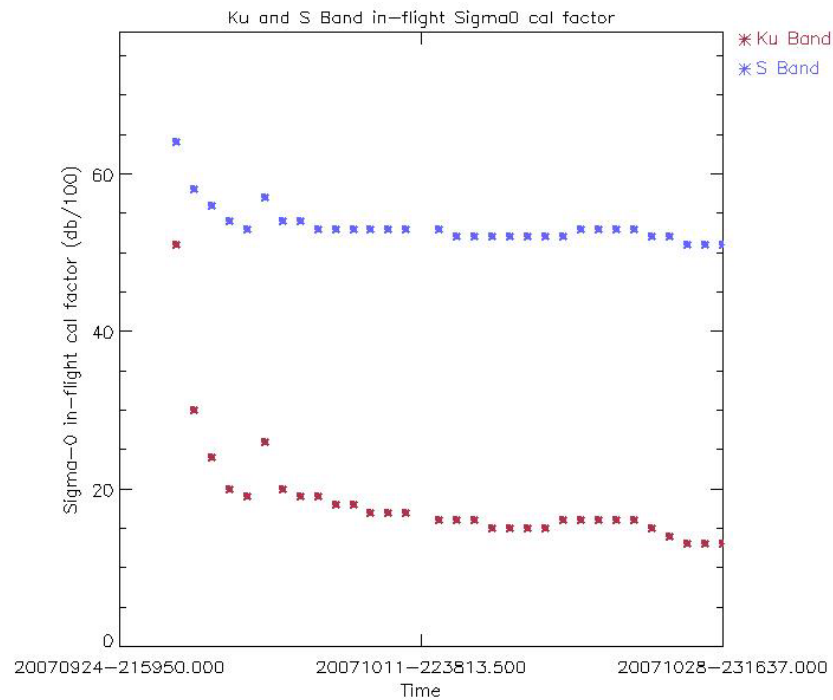
Figure 15: Ku and S Band in-flight Sigma0 calibration factor for cycle 62 (averaged per day)
