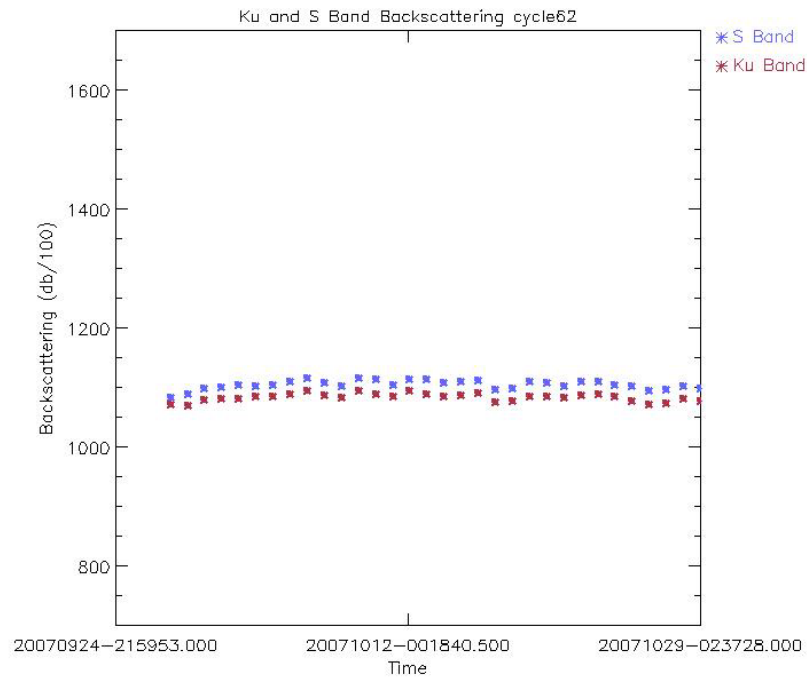
Figure 32: Ku and S Sigma 0 daily average for cycle 62 (dB/100)
