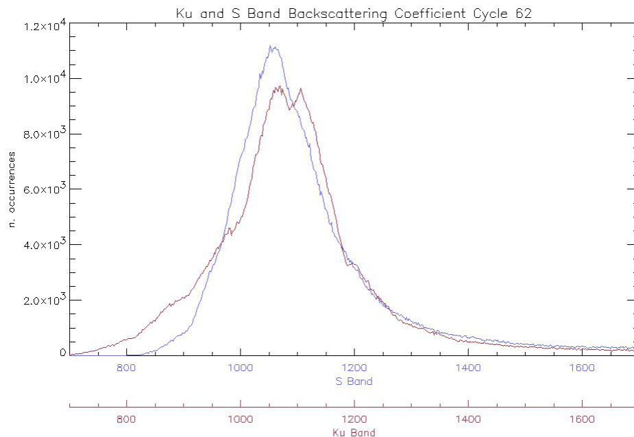
Figure 31: Histogram of Ku and S Band Backscattering Coefficient for cycle 62
