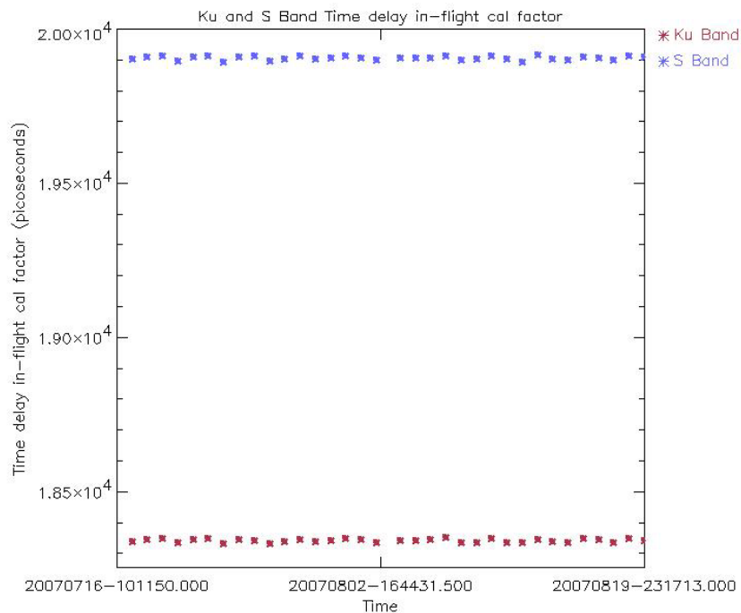
Figure 14: Ku and S Band in-flight time delay calibration factor for cycle 60 (averaged per day)
