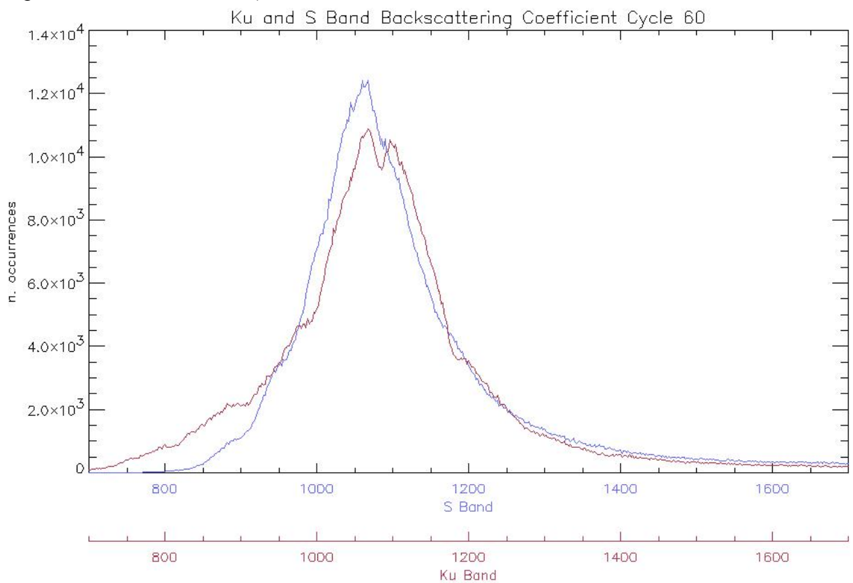
Figure 31: Histogram of Ku and S Band Backscattering Coefficient for cycle 60
