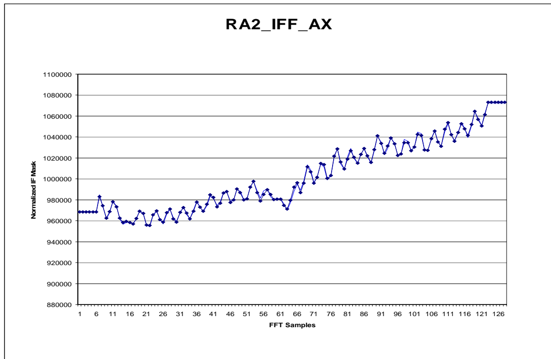
Figure 6: Previous and IF Mask updated on 2nd of August 2007
