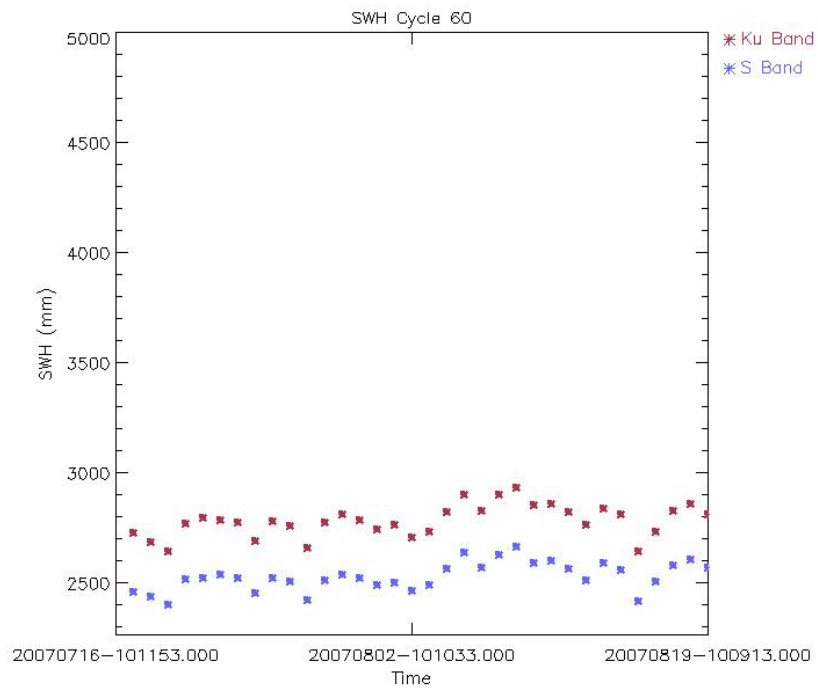
Figure 29: Ku and S SWH daily average for Cycle 60 (mm)
