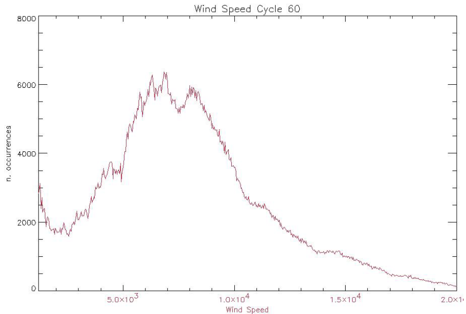
Figure 33: Histogram of Ku Wind Speed for cycle 60 (mm/sec)
