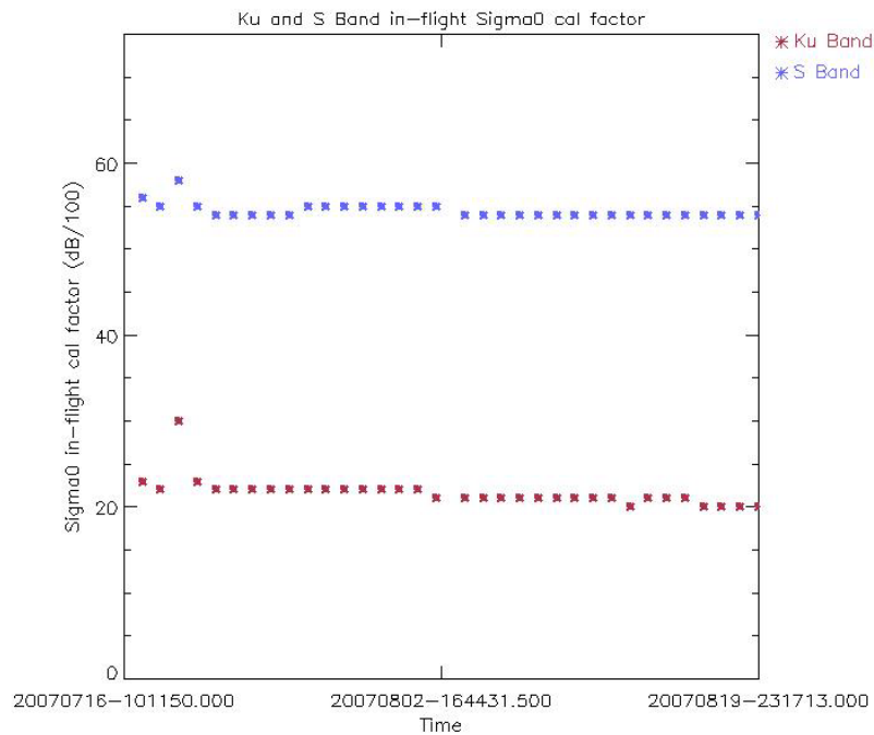
Figure 15: Ku and S Band in-flight Sigma0 calibration factor for cycle 60 (averaged per day)
