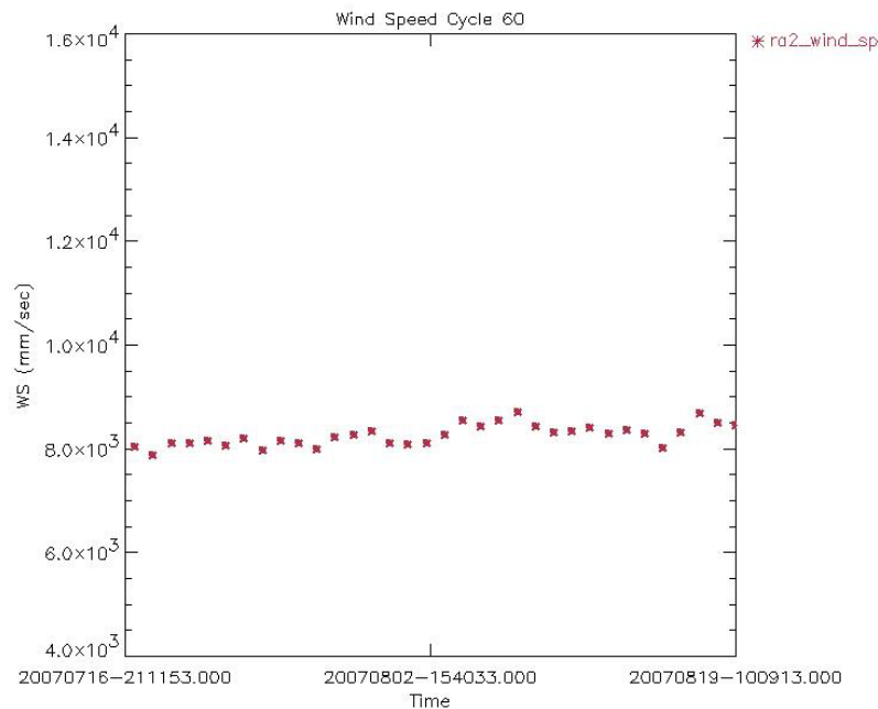
Figure 34: Ku Band Wind Speed daily average for cycle 60 (mm/s)
