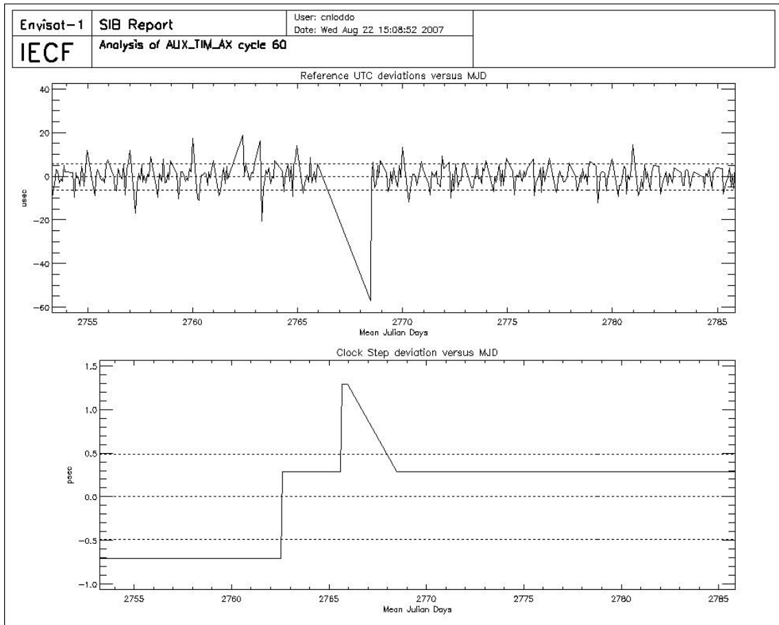
Figure 11: UTC deviations and ICU clock period for cycle 60
