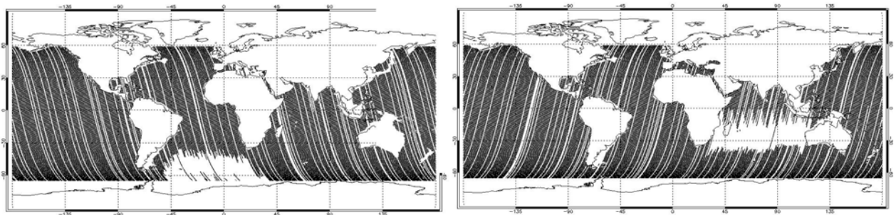
Figure 27: Ascending and Descending passes processed with DORIS on cycle 60
