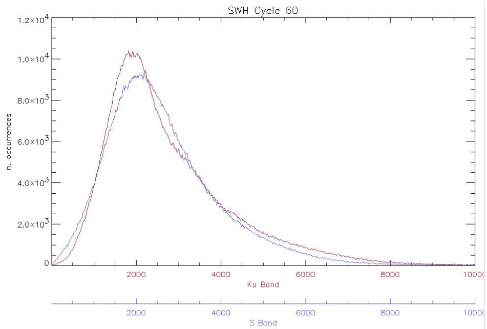
Figure 28: Histogram of Ku and S Band SWH for cycle 60
