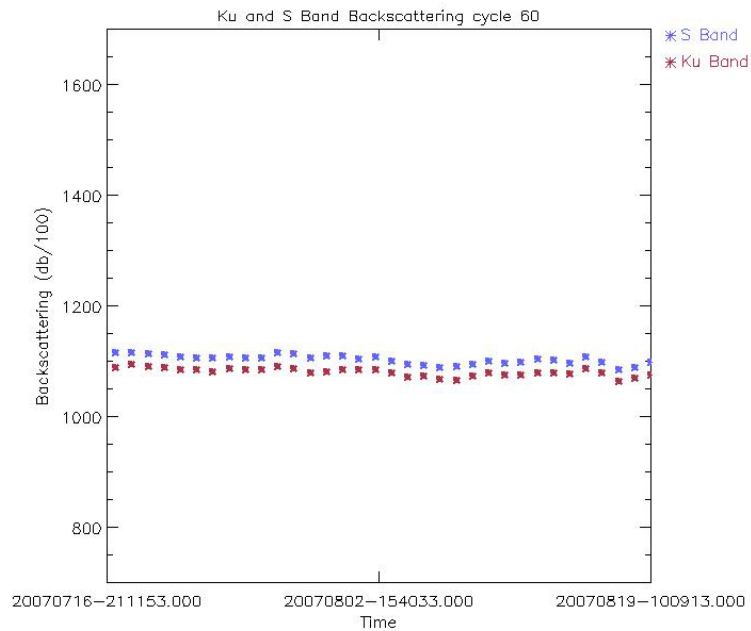
Figure 32: Ku and S Sigma_0 daily average for cycle 60 (dB/100)
