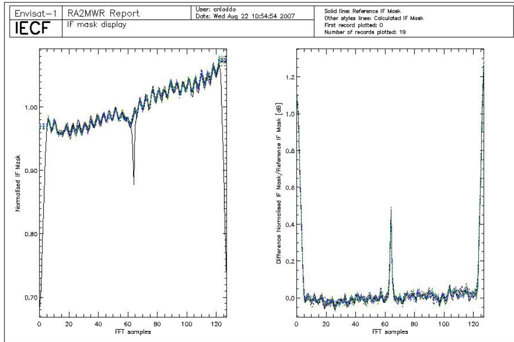
Figure 5: Valid IF masks retrieved during cycle 60 plotted together with the on-ground reference.
