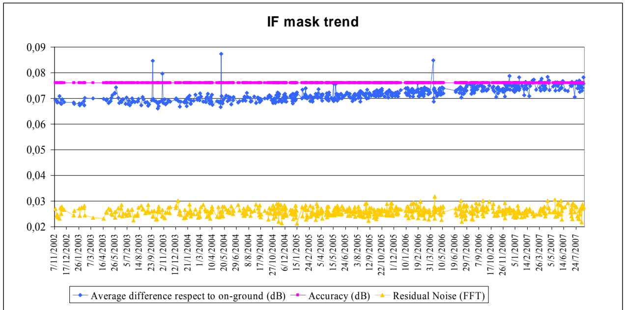
Figure 7: Evolution of the IF mask related parameters for valid IF masks retrieved up to cycle 60
