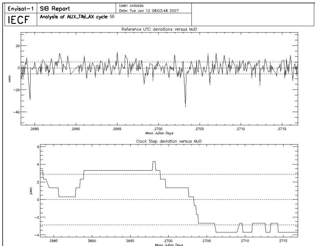
Figure 11: UTC deviations and ICU clock period for cycle 58
