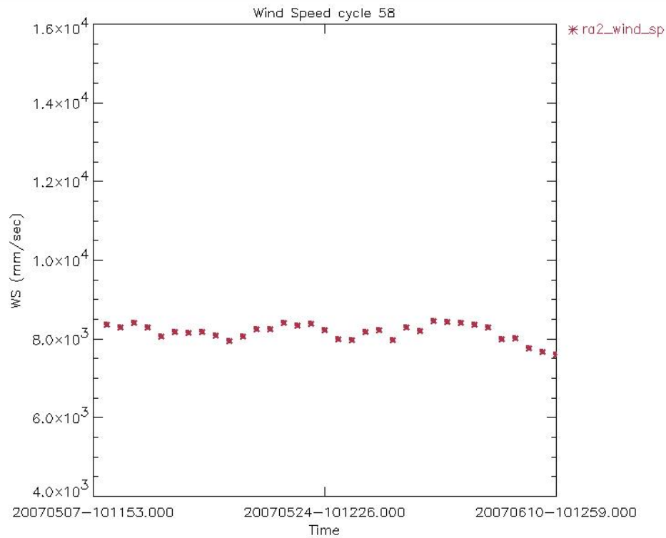
Figure 34: Ku Band Wind Speed daily average for cycle 58 (mm/s)
