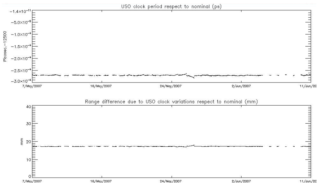
Figure 9: USO clock period for cycle 58
