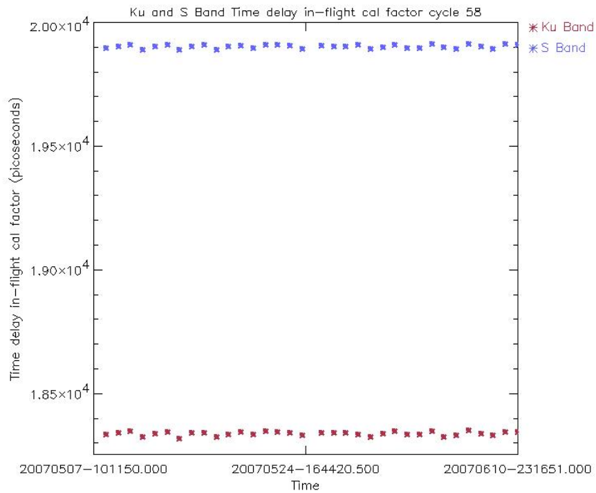
Figure 14: Ku and S Band in-flight time delay calibration factor for cycle 58 (averaged per day)
