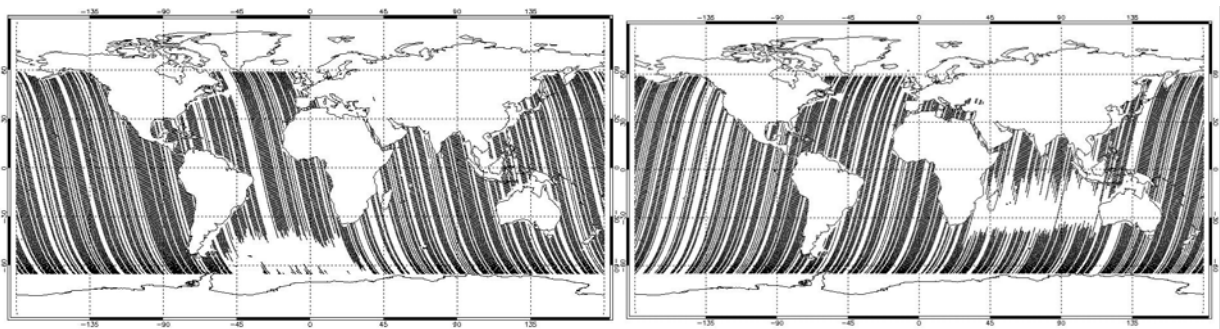
Figure 27: Ascending and Descending passes processed with DORIS on cycle 58
