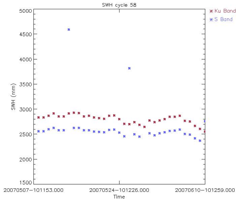
Figure 29: Ku and S SWH daily average for Cycle 58 (mm)
