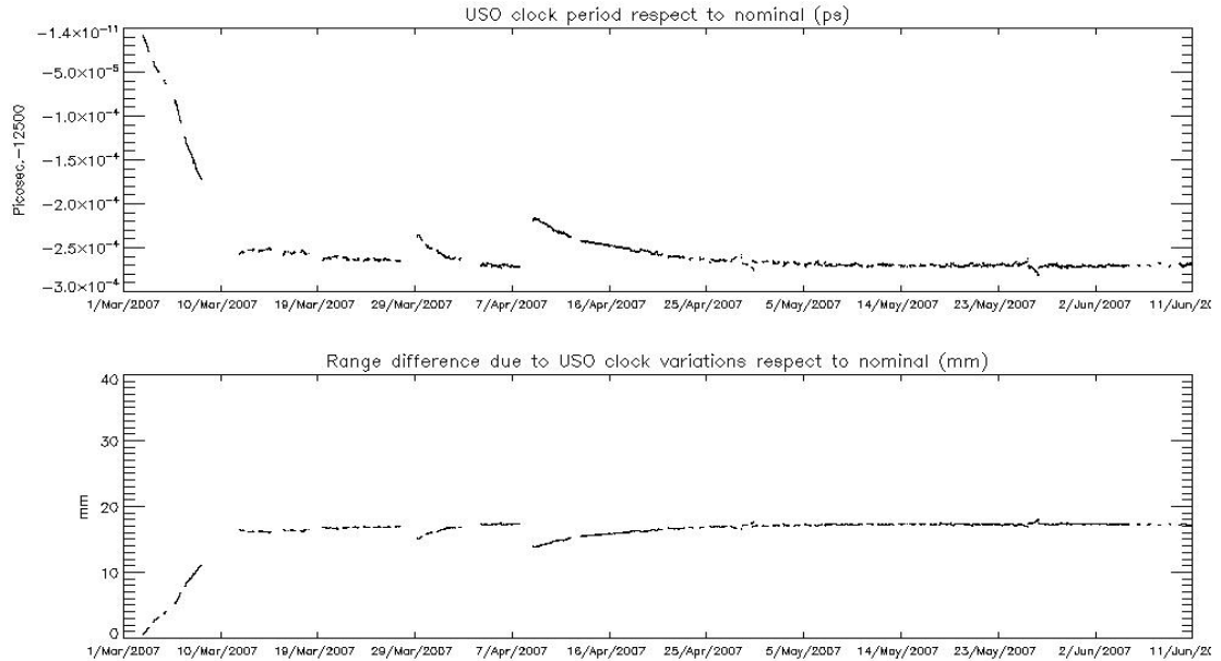
Figure 10B: USO clock period from 1 st of March onwards
