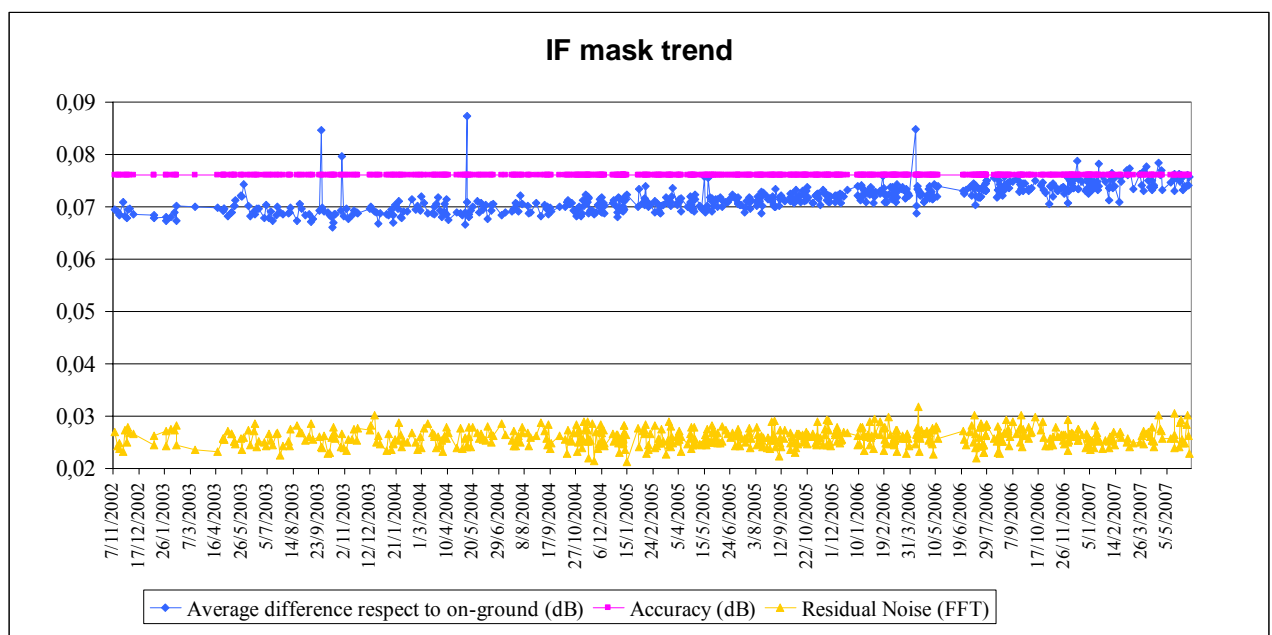
Figure 7: Evolution of the IF mask related parameters for valid IF masks retrieved up to cycle 58
