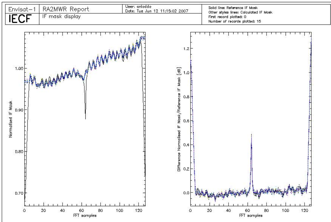
Figure 5: Valid IF masks retrieved during cycle 58 plotted together with the on-ground reference.
