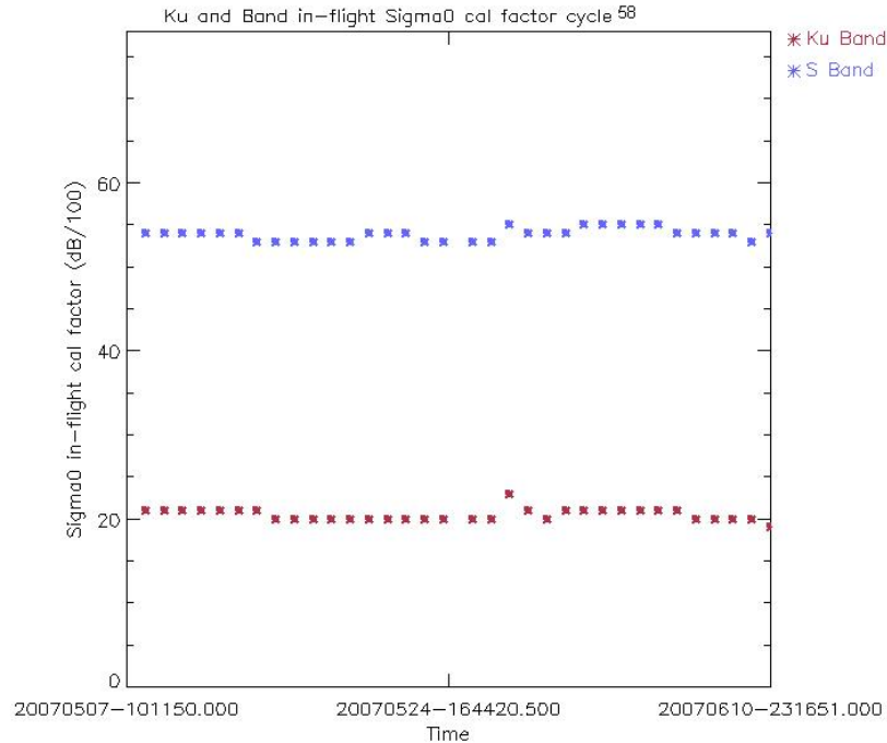
Figure 15: Ku and S Band in-flight Sigma0 calibration factor for cycle 58 (averaged per day)
