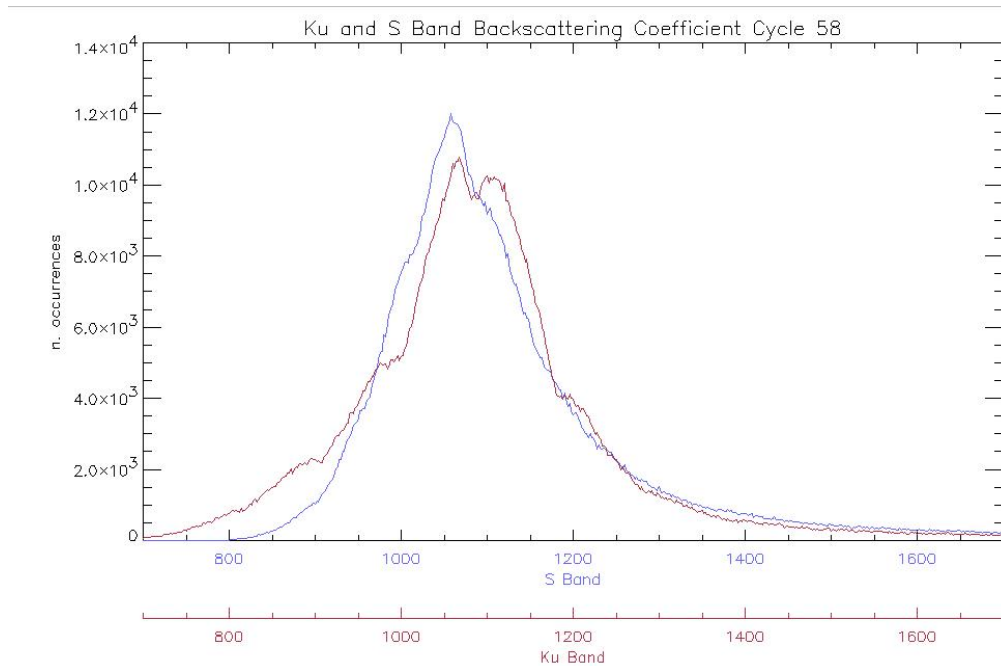
Figure 31: Histogram of Ku and S Band Backscattering Coefficient for cycle 58
