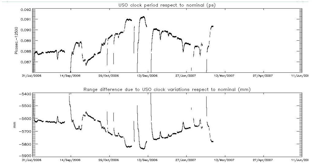
Figure 10A: USO clock period from cycle 50 onwards
