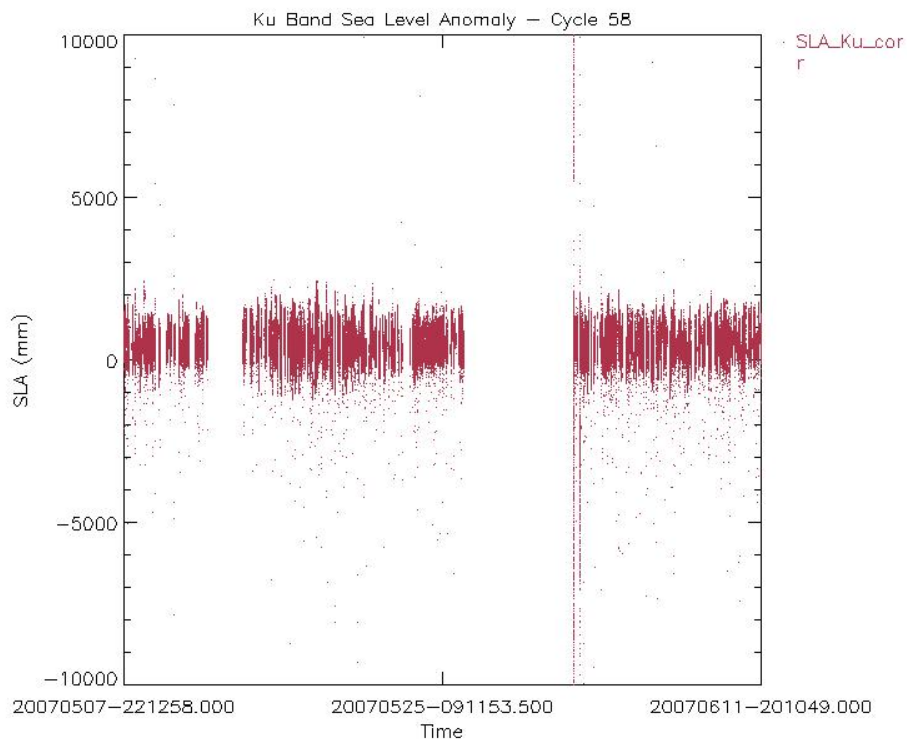
Figure 27A: Sea Level Anomalies Cycle 58, only MDSRs with valid DORIS Flag
