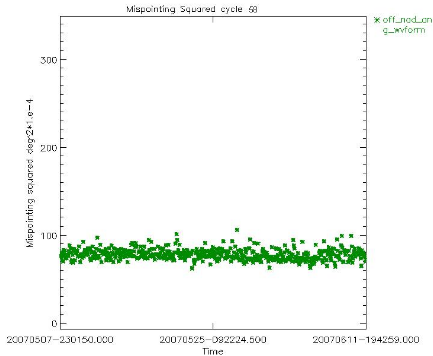
Figure 19: Smoothed mispointing squared trend for cycle 58 (deg 2 *10 -4 )
