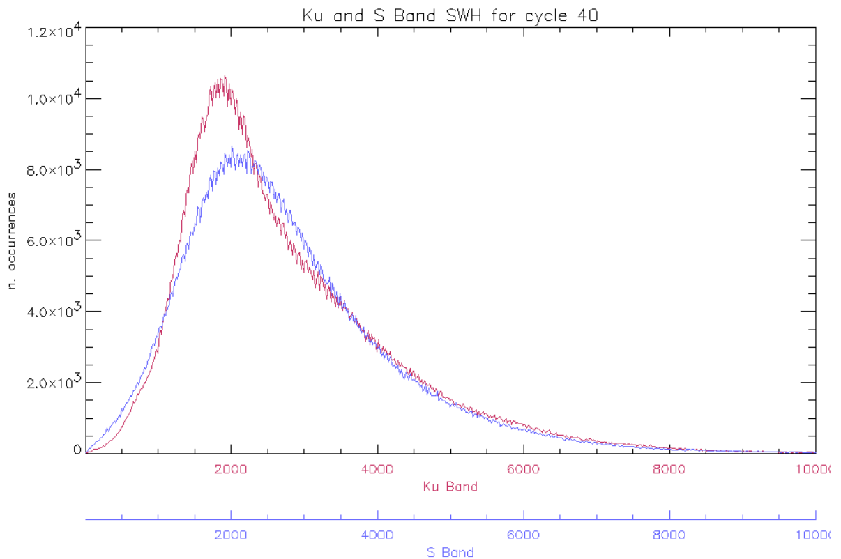
Figure 13: Histogram of Ku and S Band SWH for cycle 40 (mm)
