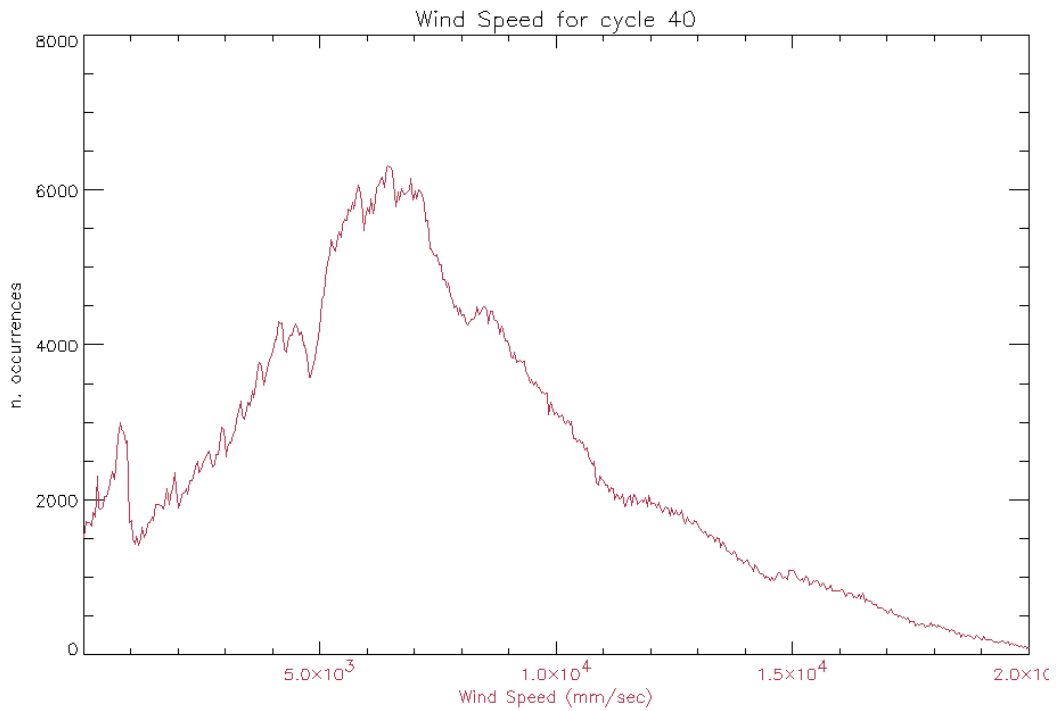
Figure 17: Histogram of Ku Wind Speed for cycle 40 (mm/s)
