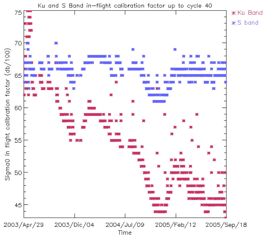
Figure 30: Ku and S Band in-flight Sigma0 calibration factor up to cycle 40
