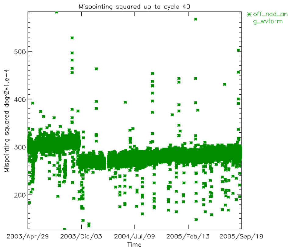
Figure 26: Smoothed mispointing squared trend until end of cycle 40 (deg 2 *10e-4)
