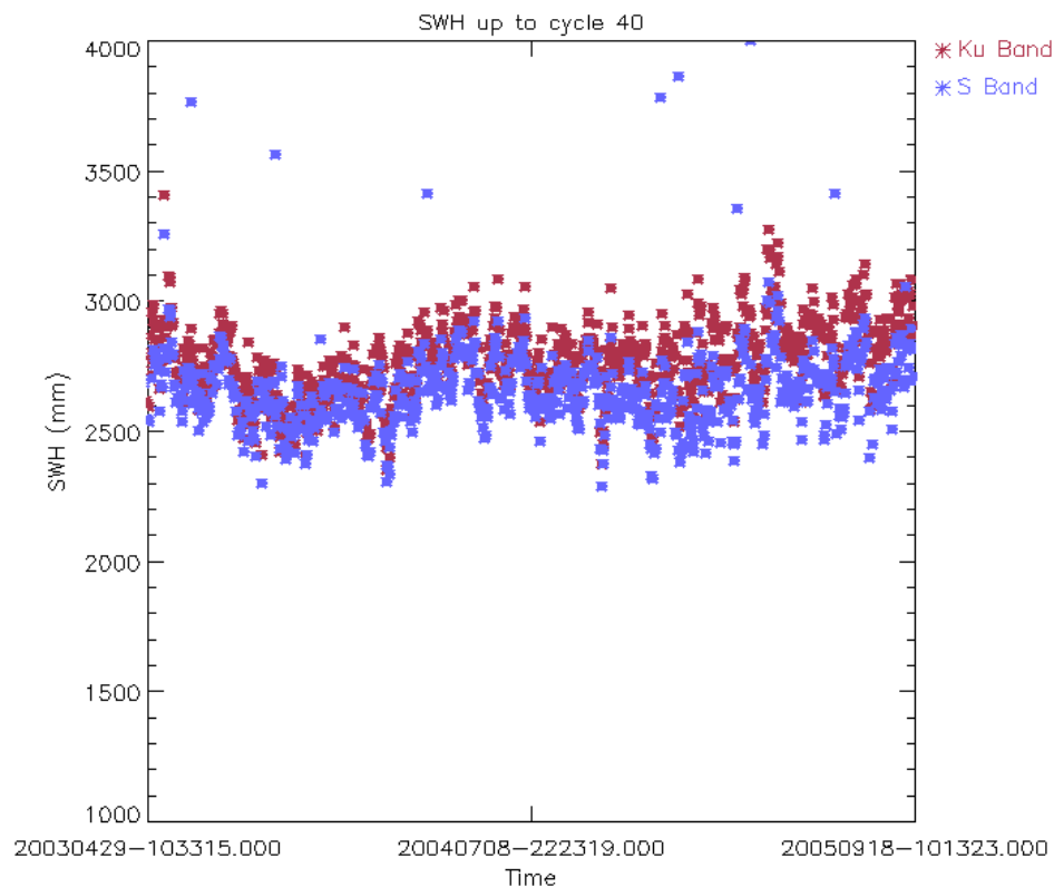
Figure 32: Ku and S SWH daily average up to cycle 40 (mm)
