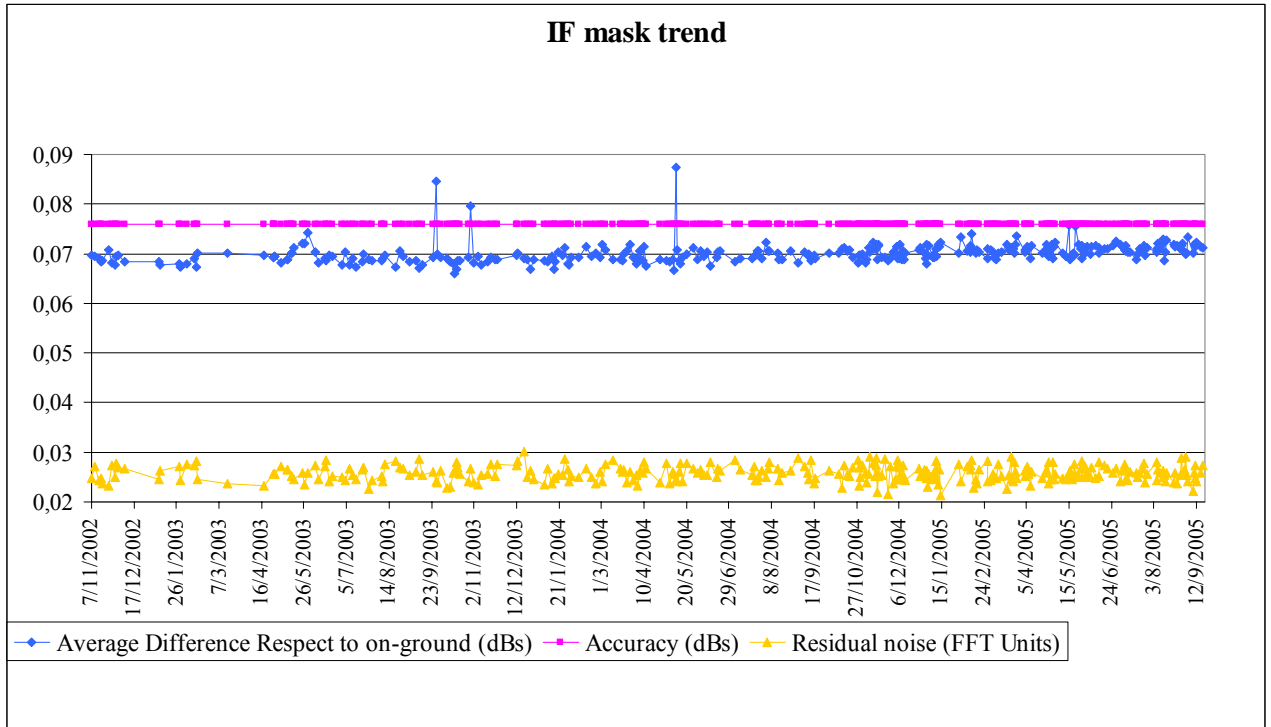
Figure 19: Evolution of the IF mask related parameters for valid IF masks retrieved up to cycle 40
