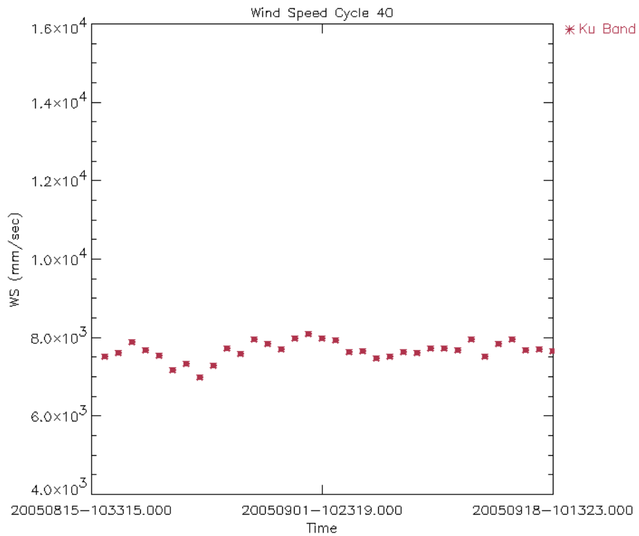
Figure 18: Ku Band Wind Speed daily average for cycle 40 (mm/s)
