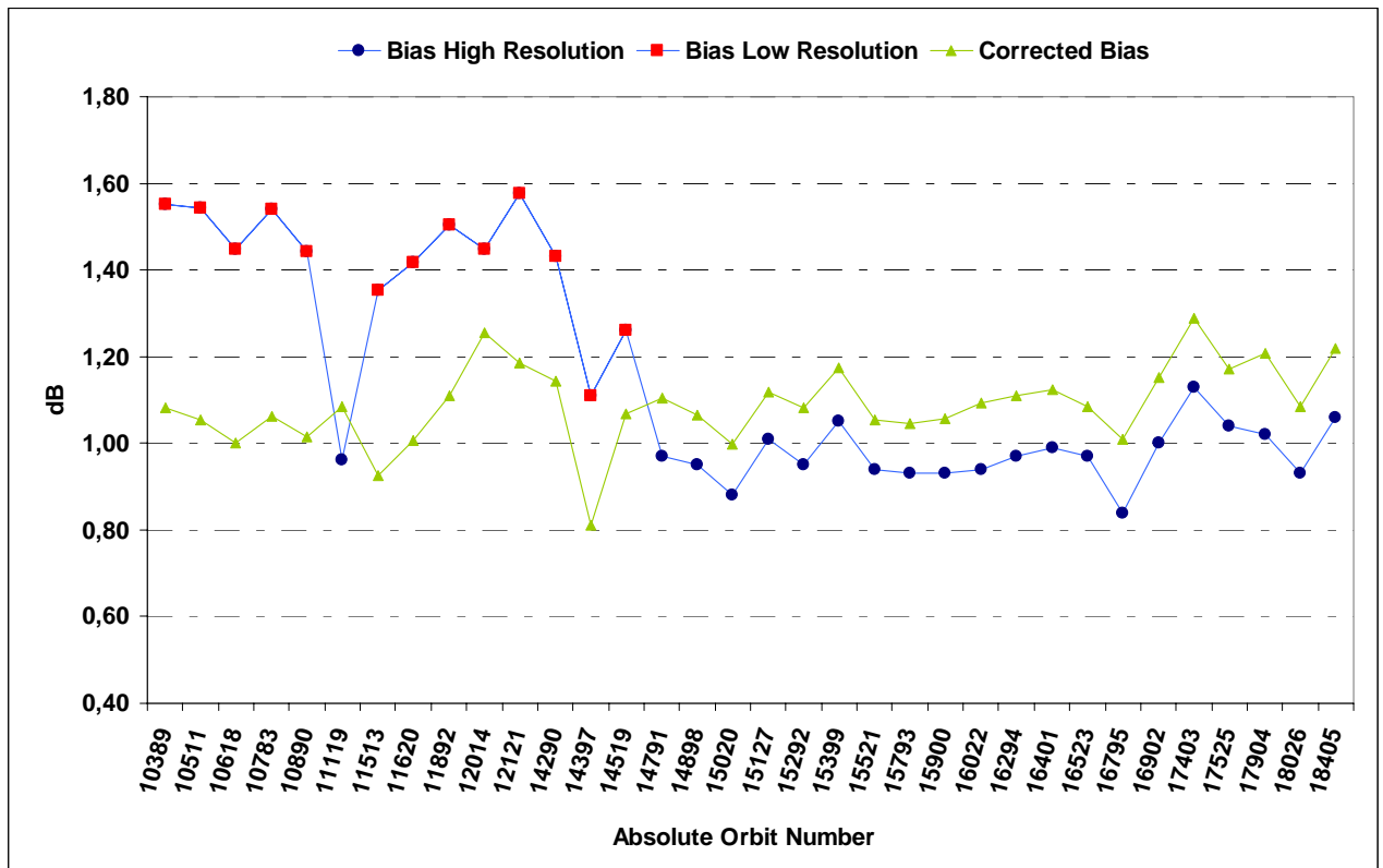
Figure 24: Time behavior of the transponder bias
