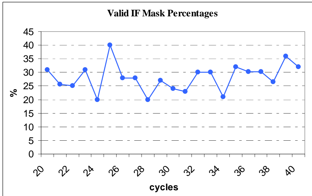
Figure 19A: Percentages of valid IF Mask up to cycle 40
