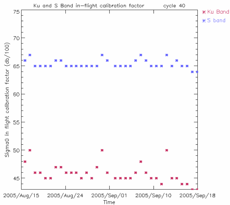
Figure 9: Ku and S Band in-flight Sigma0 calibration factor for cycle 40
