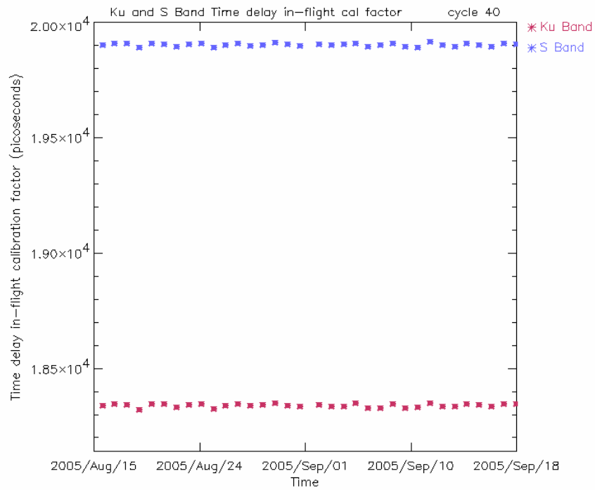
Figure 8: Ku and S Band in-flight time delay calibration factor for cycle 40
