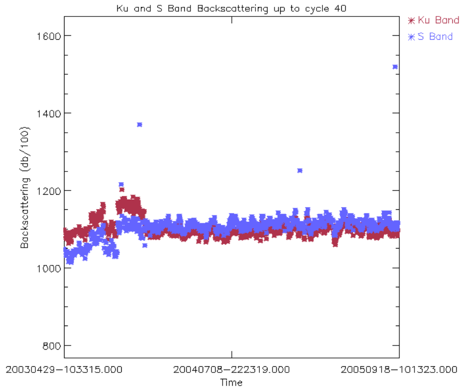
Figure 33: Ku and S band Backscattering daily averages up to cycle 40 (dB/100)
