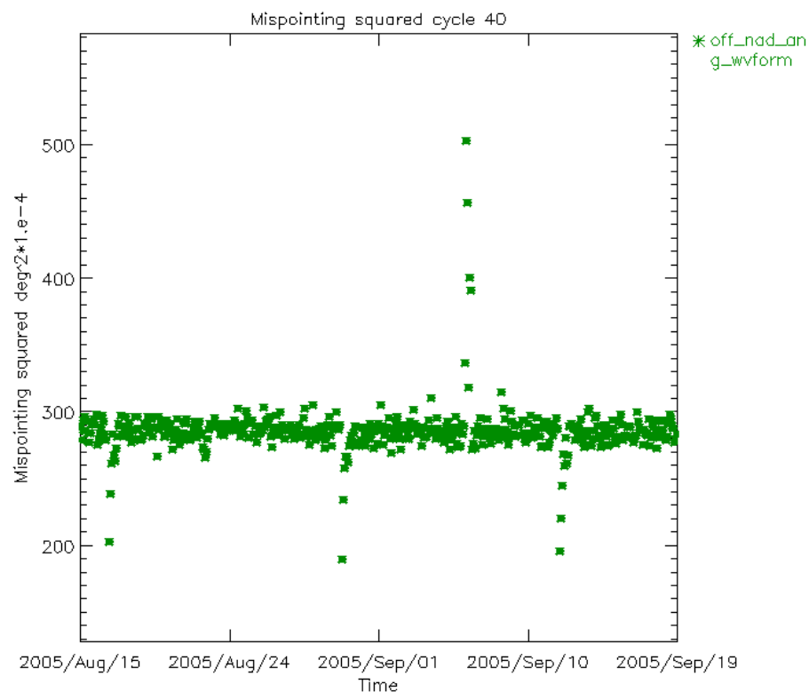
Figure 7: Smoothed mispointing squared trend for cycle 40 ( \text{deg}^2 \cdot 10^4 )
