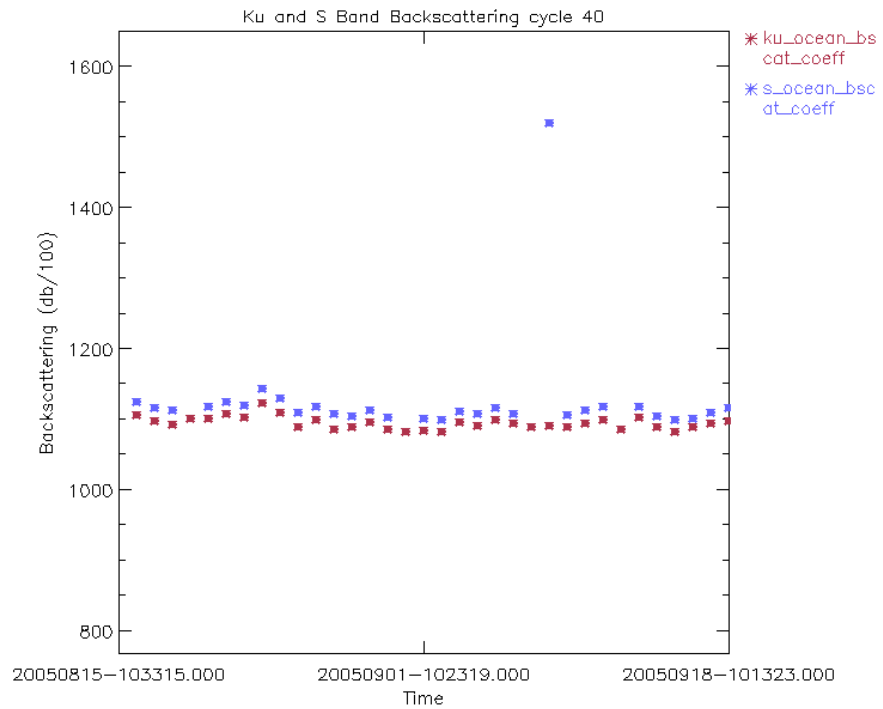
Figure 16: Ku and S Sigma_0 daily average for cycle 40 (dB/100)
