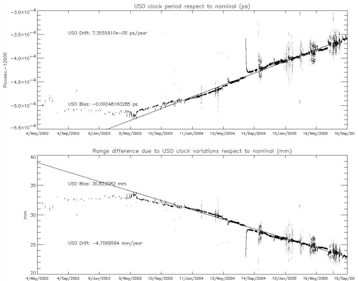
Figure 20: USO clock period until end of cycle 40
