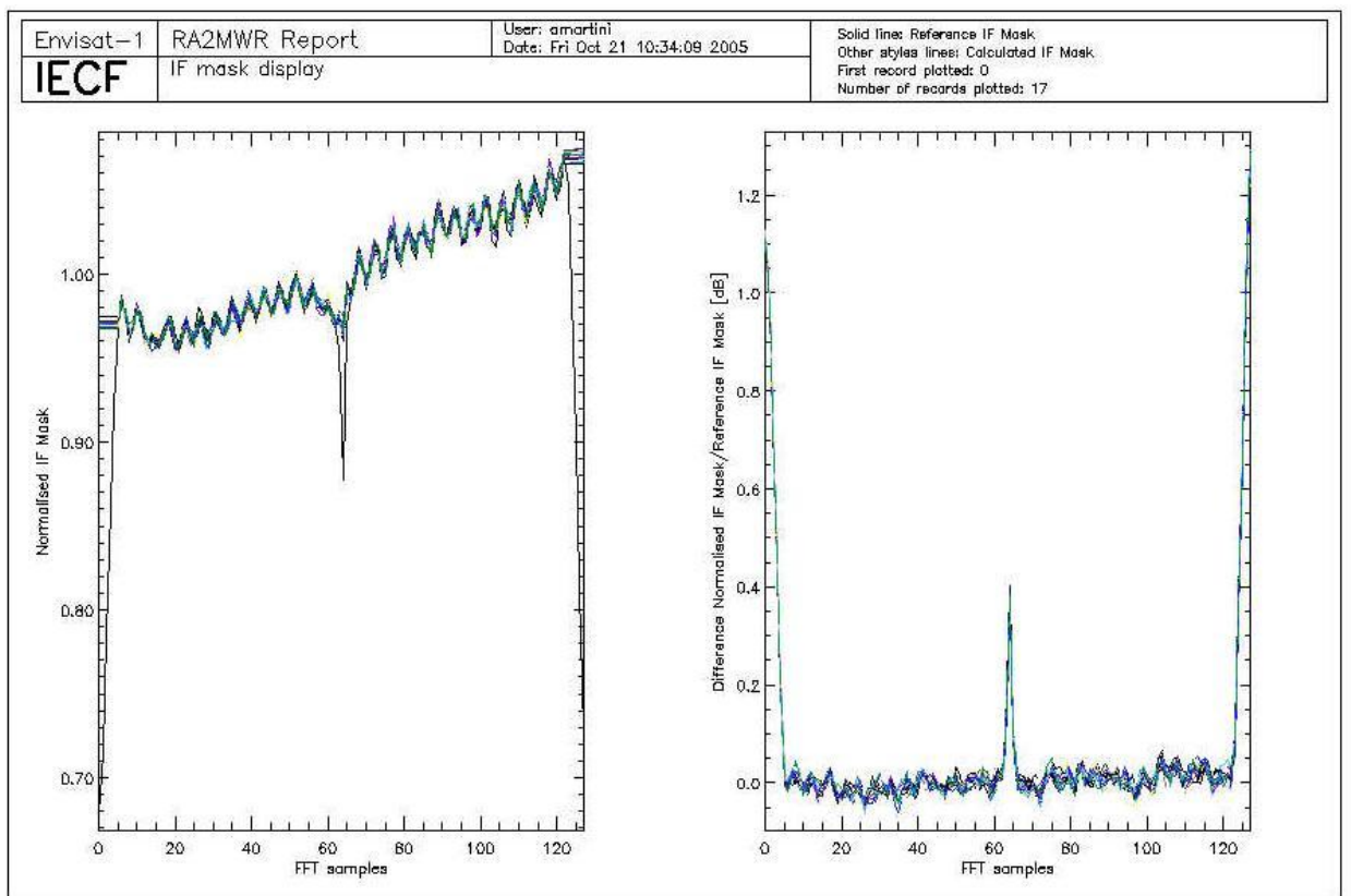
Figure 2: Valid IF masks retrieved daily during cycle 40 plotted together with the on-ground reference.
