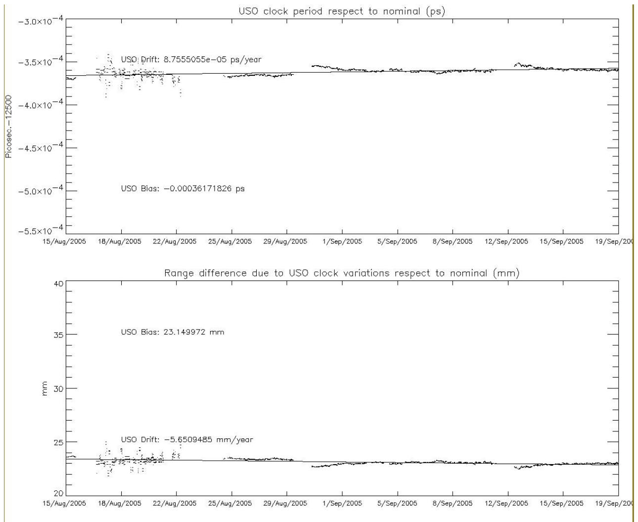
Figure 3: USO clock period for cycle 40
