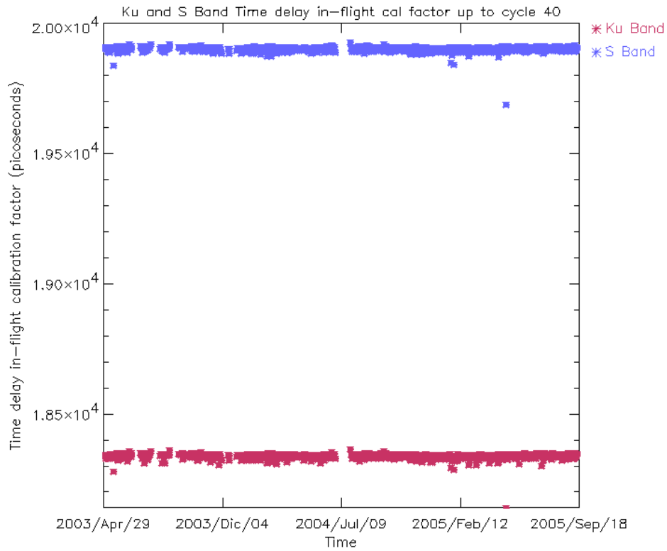
Figure 29: Ku and S Band in-flight time delay calibration factor up to cycle 40
