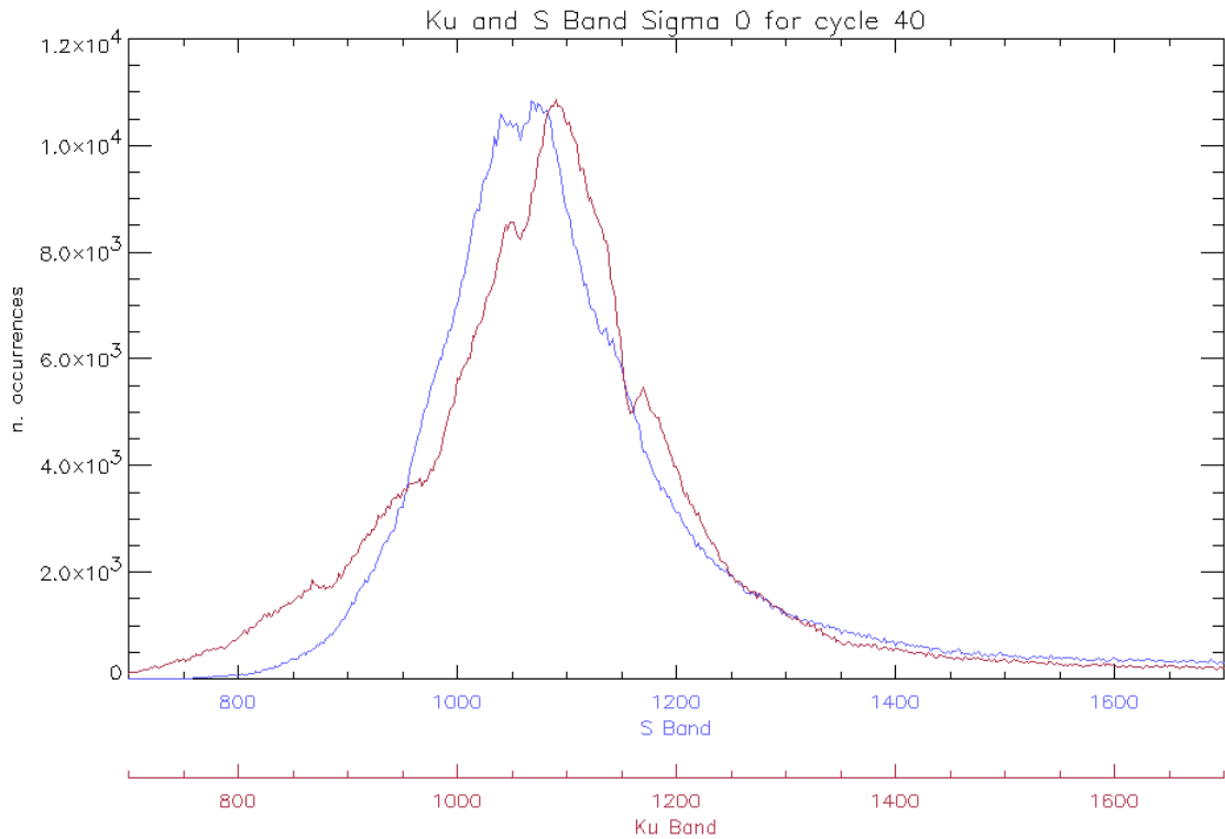
Figure 15: Histogram of Ku and S Band Backscattering Coefficient for cycle 40 (dB/100)
