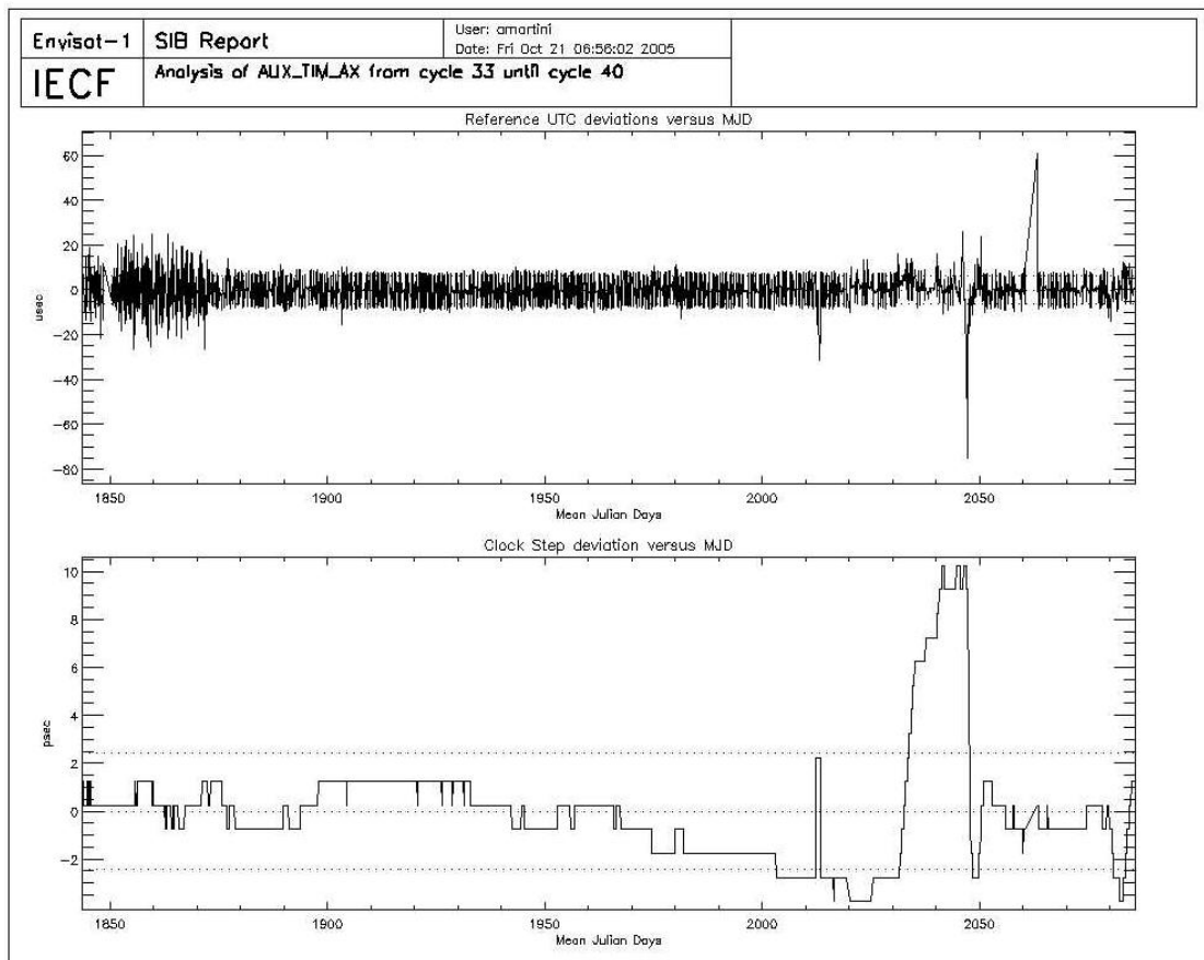
Figure 25A: UTC deviations and ICU clock period from cycle 33 up to cycle 40
