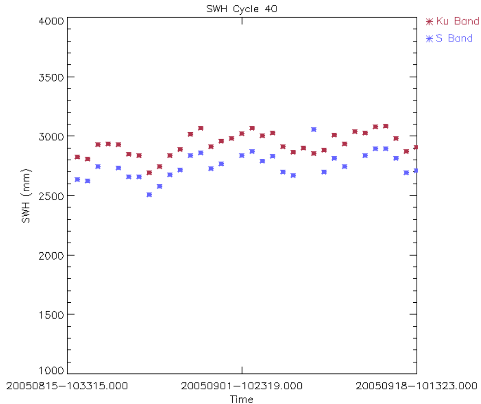
Figure 14: Ku and S SWH daily average for cycle 40 (mm)
