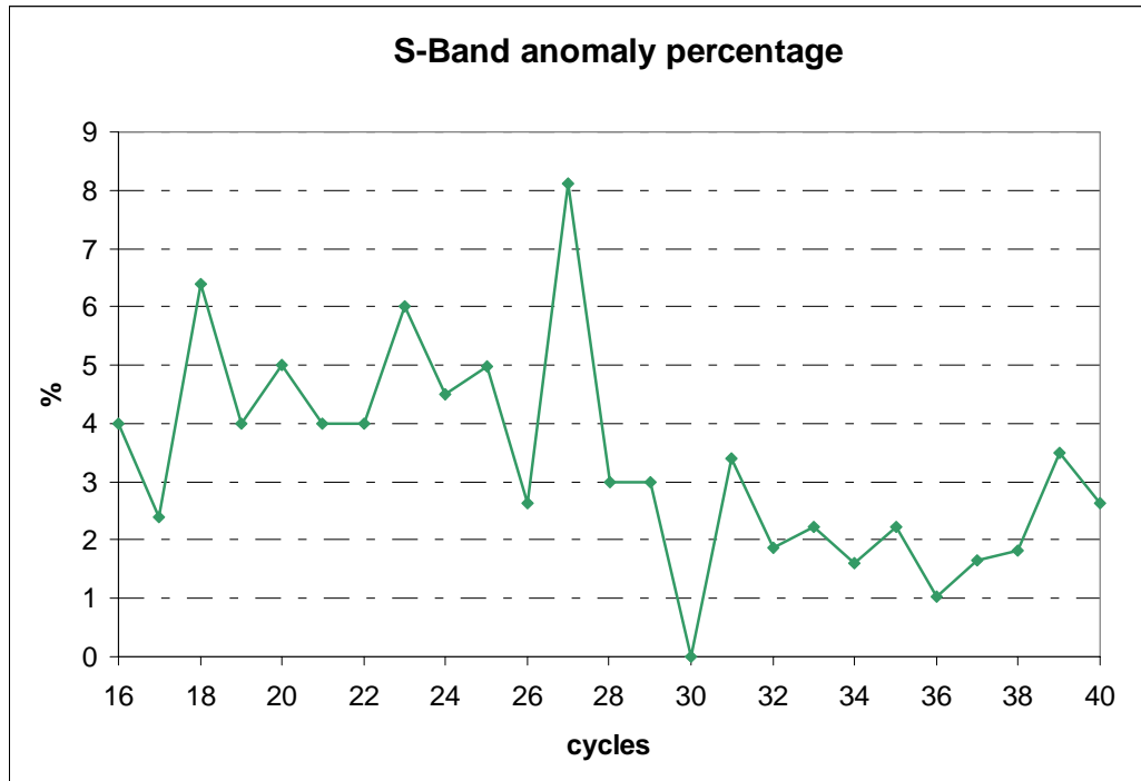
Figure 28: Percentage of data affected by the “S-Band Anomaly” for cycles 16-40
