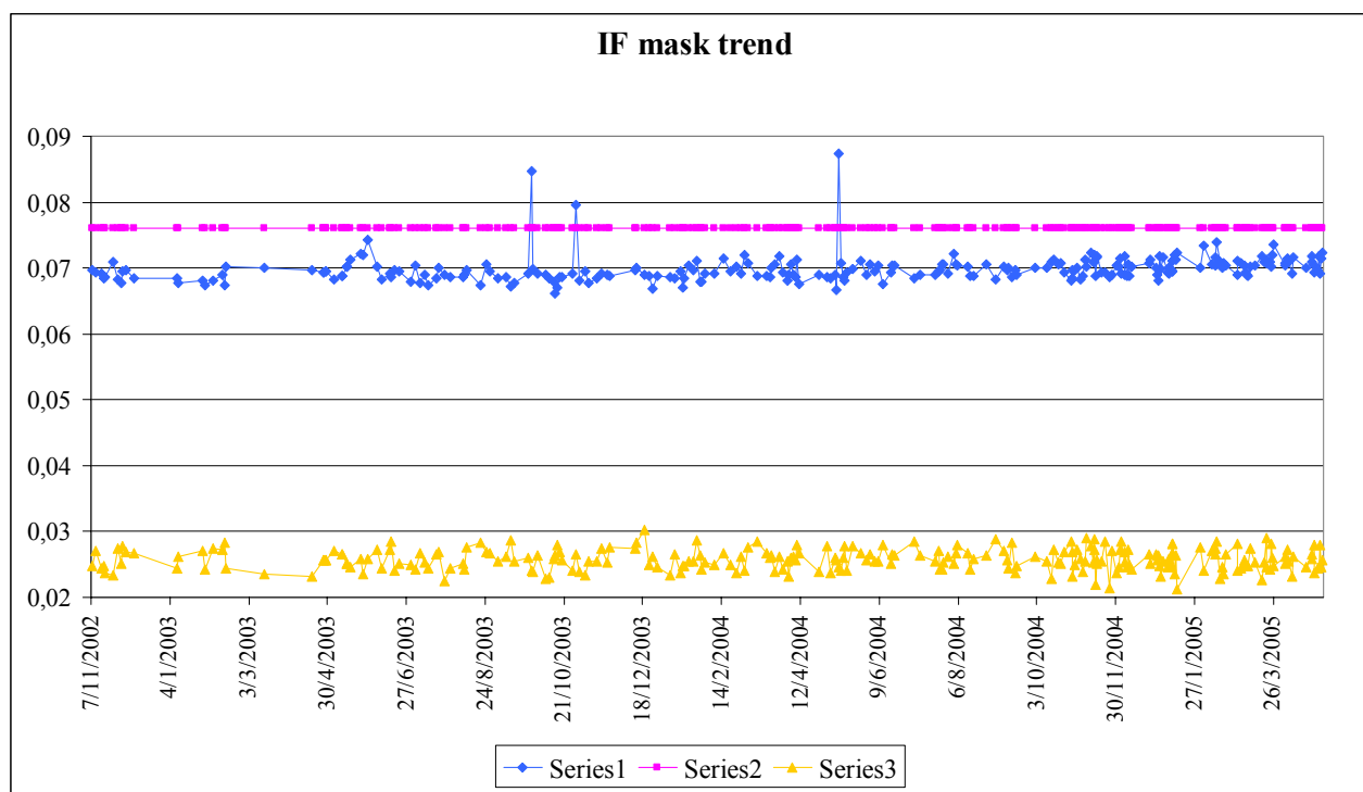
Figure 19: Evolution of the IF mask related parameters for valid IF masks retrieved up to cycle 36
