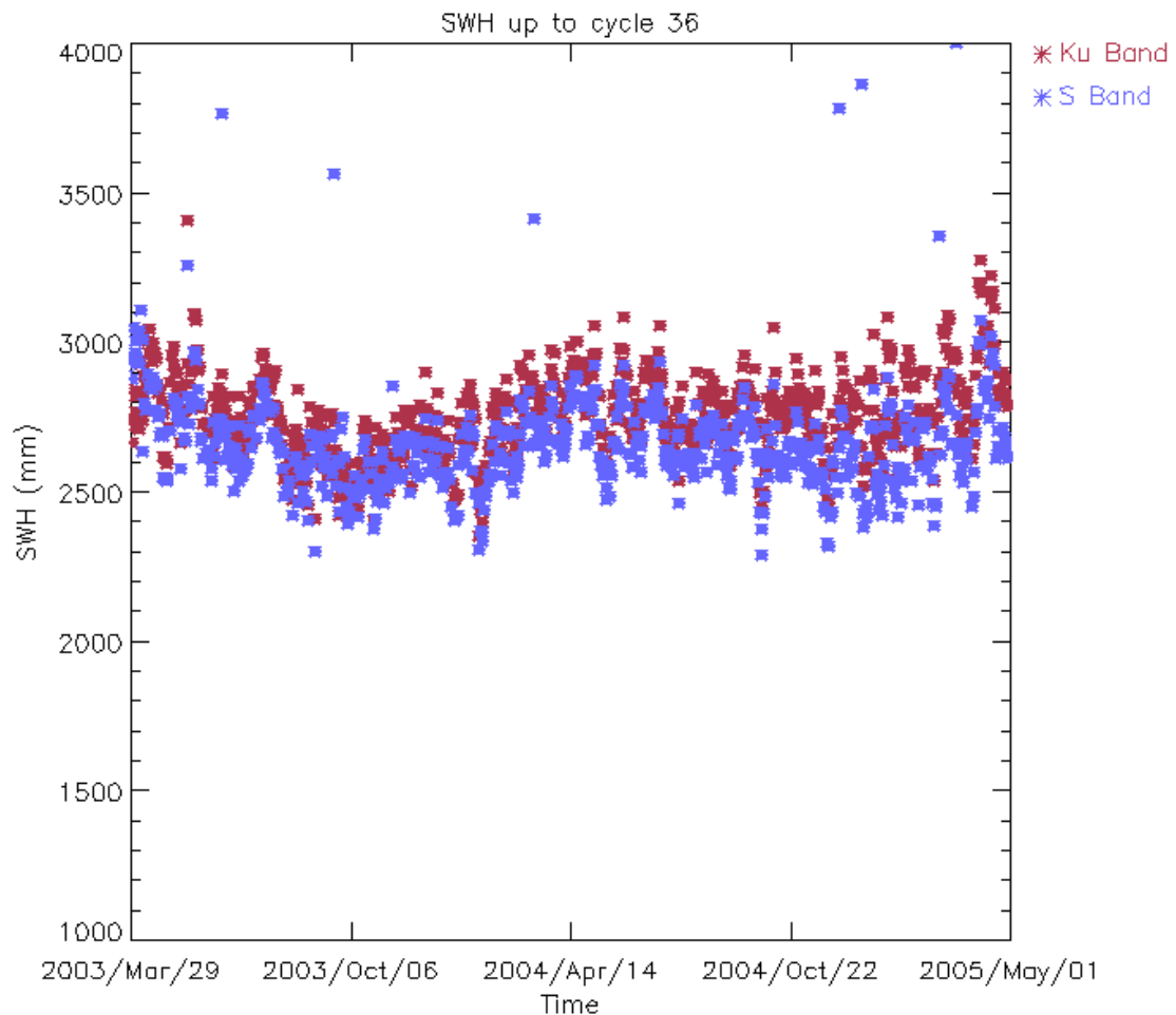
Figure 32: Ku and S SWH daily average up to cycle 36 (mm)
