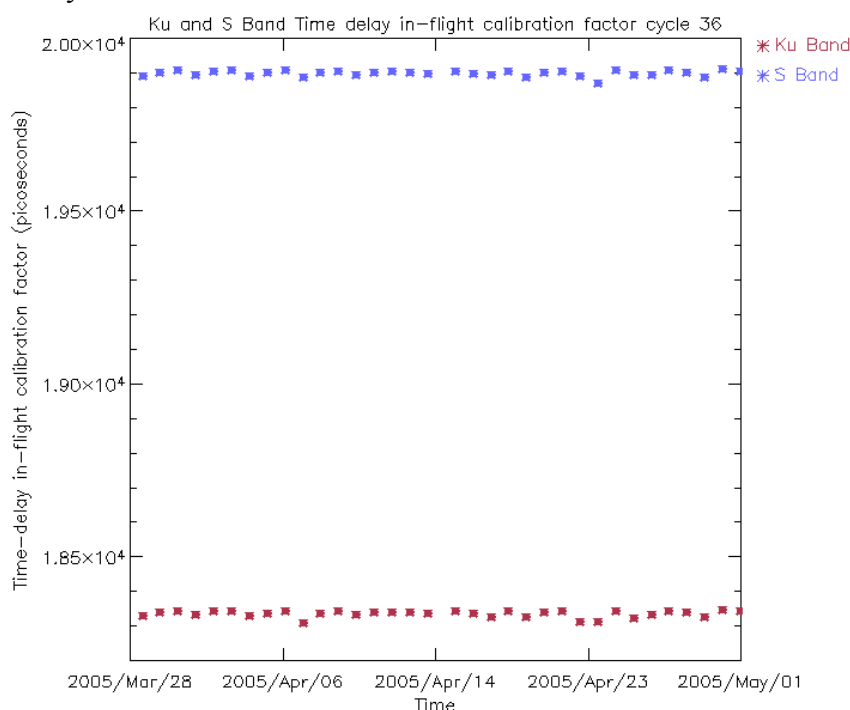
Figure 8: Ku and S Band in-flight time delay calibration factor for cycle 36
