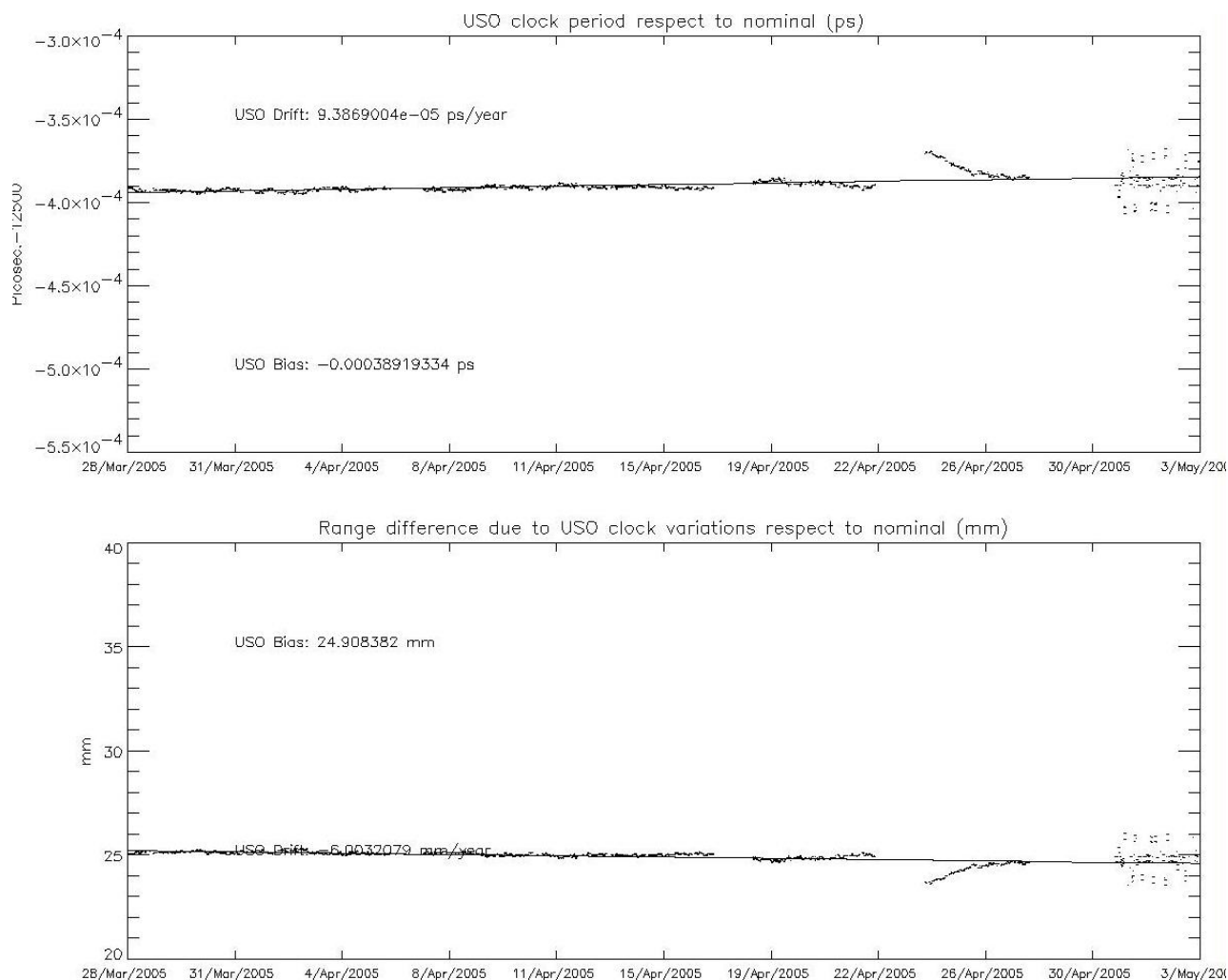
Figure 3: USO clock period for cycle 36
