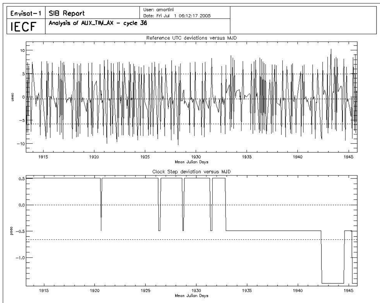
Figure 6: UTC deviations and ICU clock period for cycle 36
