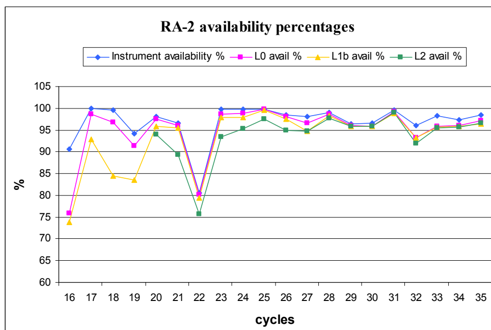
Figure 31: Percentage of Products unavailability up to cycle 36
