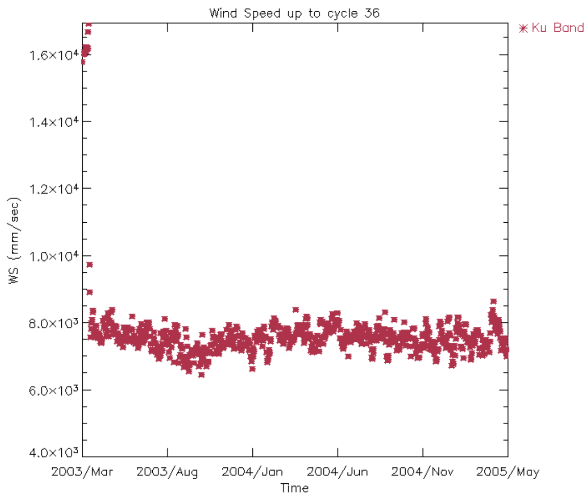
Figure 34: Wind Speed daily averages up to cycle 36 (mm/s)
