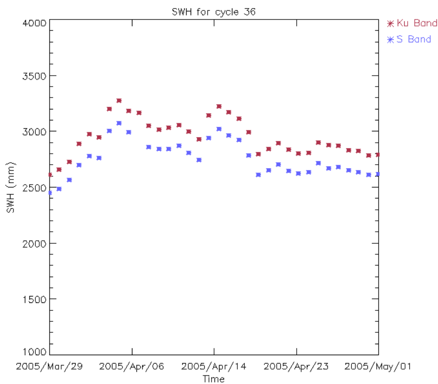
Figure 14: Ku and S SWH daily average for cycle 36 (mm)
