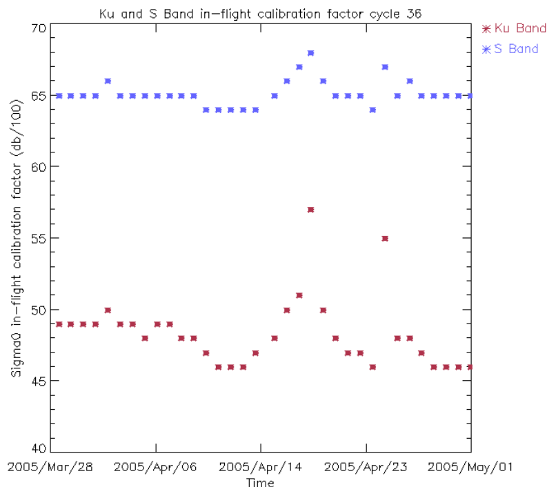
Figure 9: Ku and S Band in-flight Sigma0 calibration factor for cycle 36
