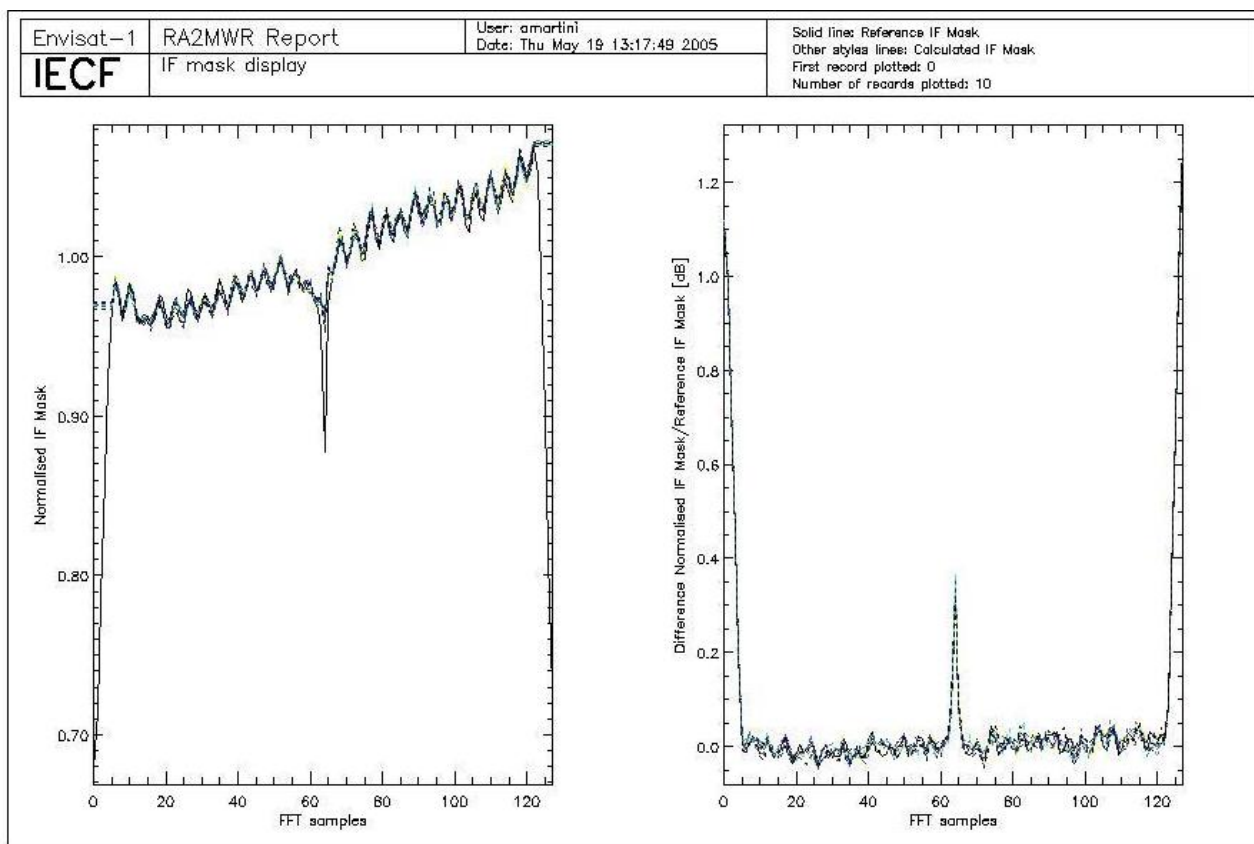
Figure 2: Valid IF masks retrieved daily during cycle 36 plotted together with the on-ground reference.
