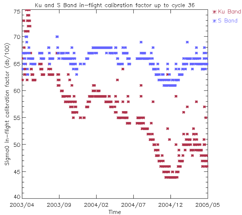
Figure 30: Ku and S Band in-flight Sigma0 calibration factor up to cycle 36
