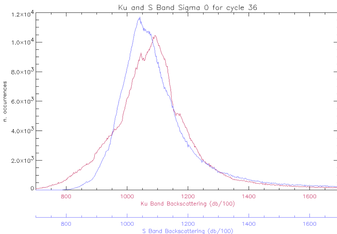
Figure 15: Histogram of Ku and S Band Backscattering Coefficient for cycle 36 (dB/100)
