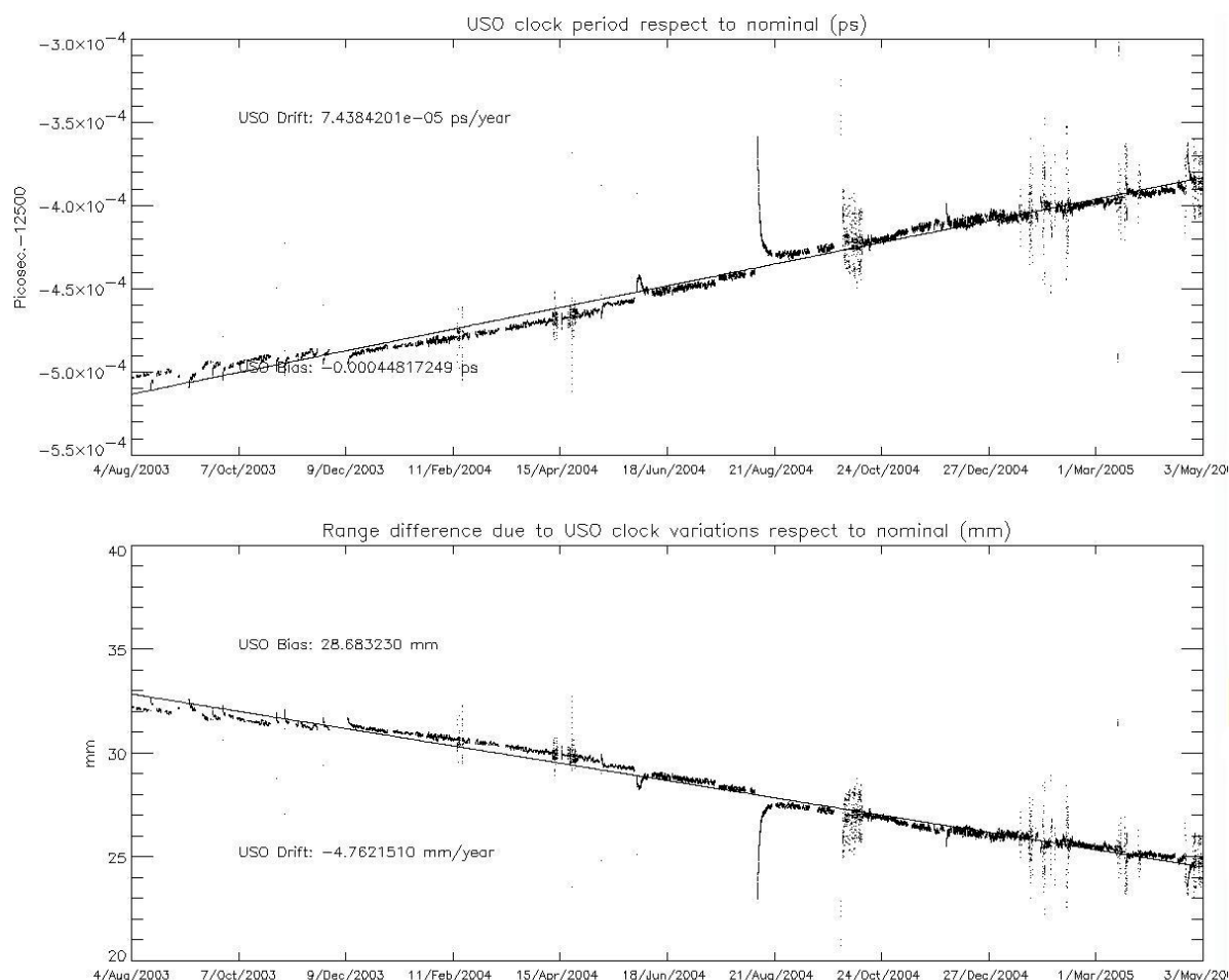
Figure 20: USO clock period until end of cycle 36
