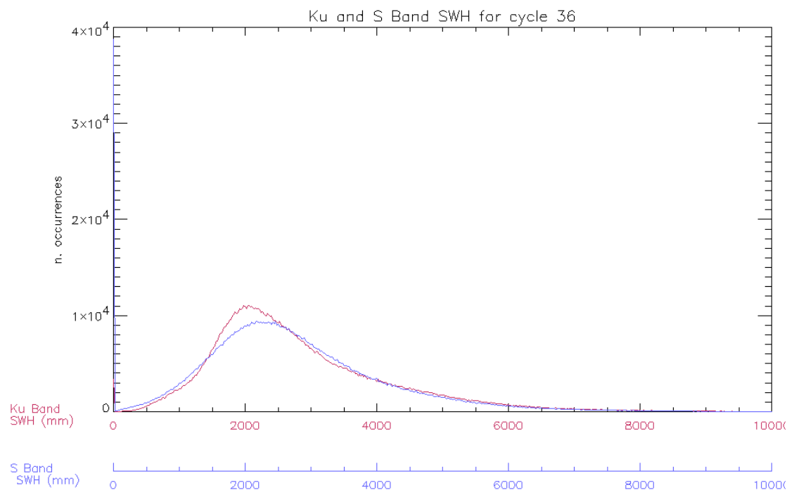
Figure 13: Histogram of Ku and S Band SWH for cycle 36 (mm)
