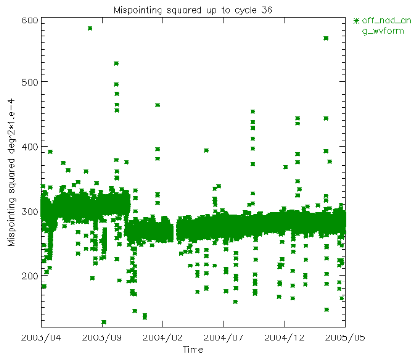
Figure 26: Smoothed mispointing squared trend until end of cycle 36 ( \text{deg}^2 \cdot 10^{-4} )
