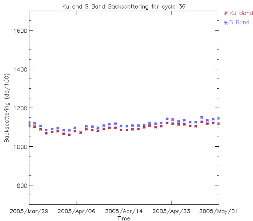
Figure 16: Ku and S Sigma_0 daily average for cycle 36 (dB/100)
