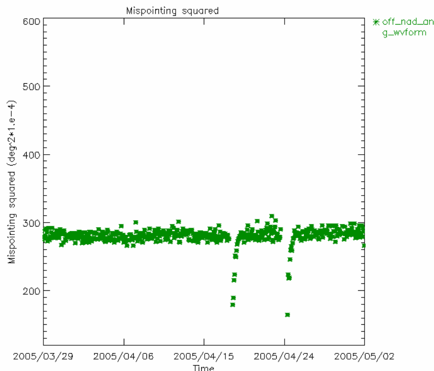
Figure 7: Smoothed mispointing squared trend for cycle 36 ( \text{deg}^2 \cdot 10^4 )
