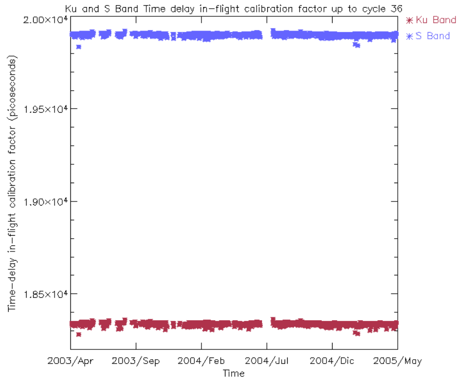
Figure 29: Ku and S Band in-flight time delay calibration factor up to cycle 36
