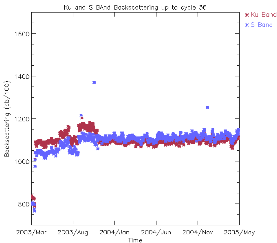
Figure 33: Ku and S band Backscattering daily averages up to cycle 36 (dB/100)
