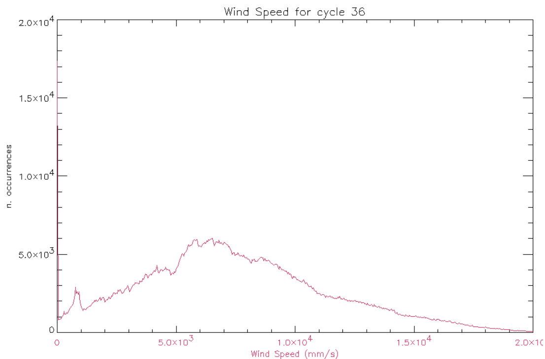
Figure 17: Histogram of Ku Wind Speed for cycle 36 (mm/s)
