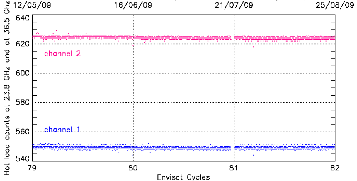
Figure 2: Time evolution of the sky horn (top) and hot load (bottom) counts (zoom on the last 3 cycles).
