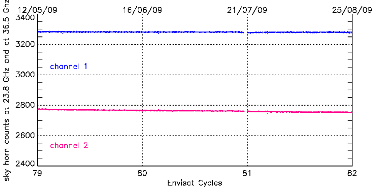
ENVISAT MWR sky horn counts (zoom on last 3 cycles)
