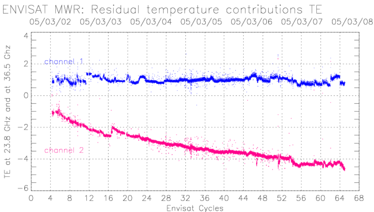
Figure 7: Time evolution of the residual temperature TE since Envisat launch.
