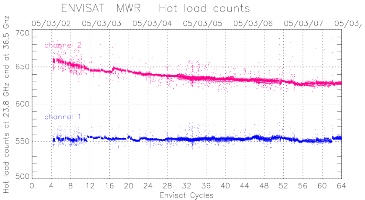
Figure 6: Time evolution of the sky horn (top) and hot load (bottom) counts since Envisat launch.
