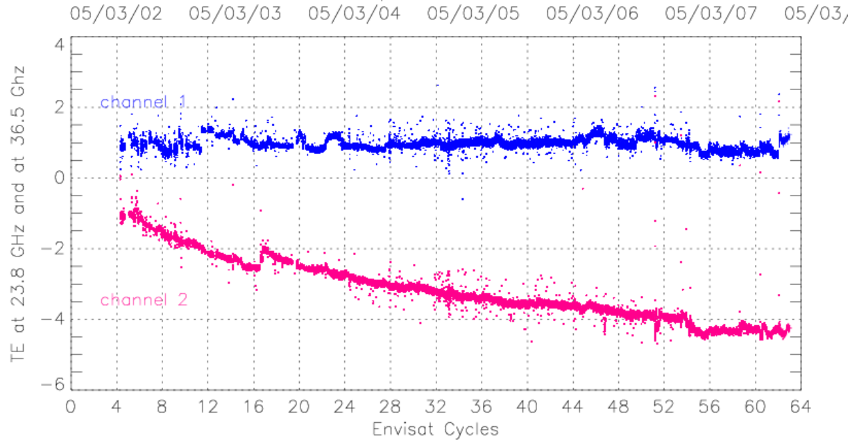
Figure 7: Time evolution of the residual temperature TE since Envisat launch.
