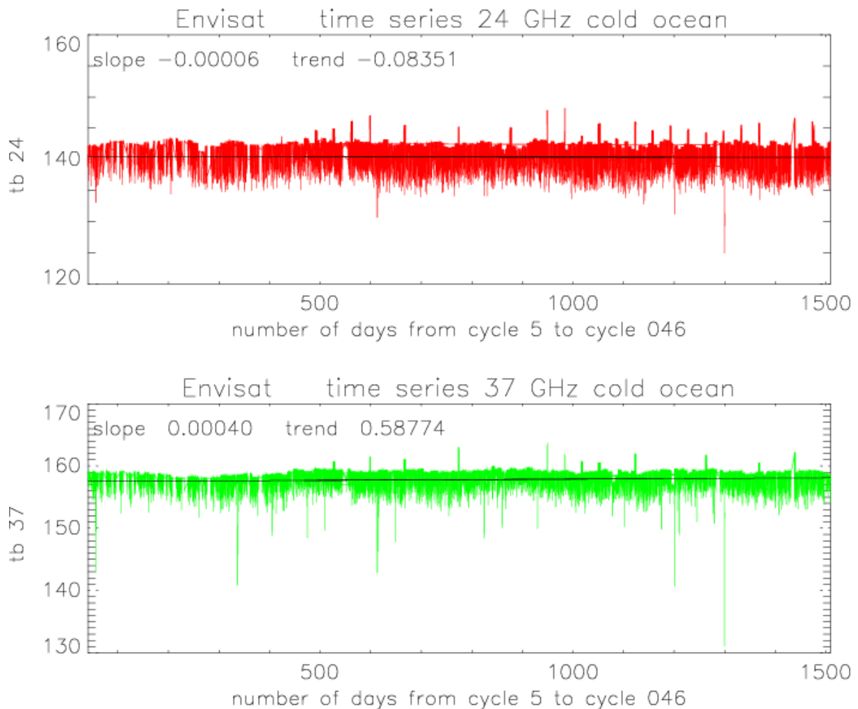
Figure 6: time series of the coldest brightness temperatures over ocean. The x-axis represents the number of days since Envisat launch. The data available before cycle 5 (corresponding to about 30 days) are not used for this monitoring
