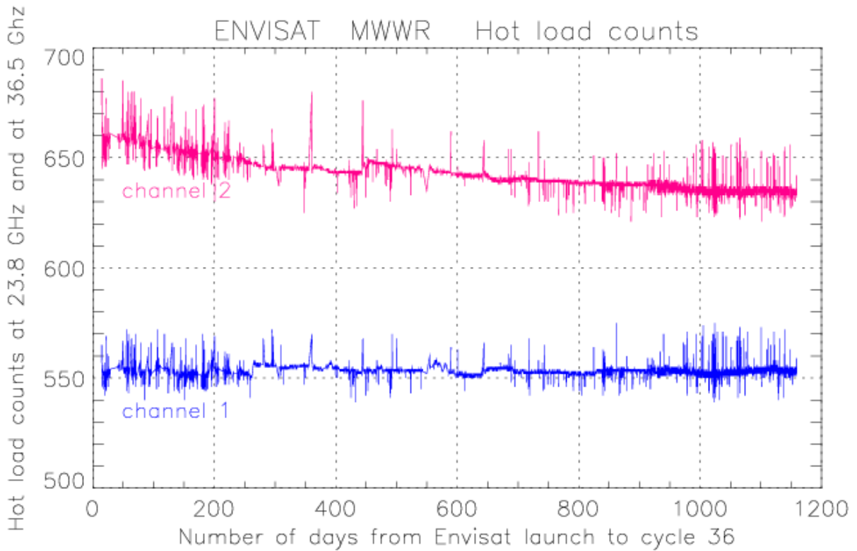
Figure 4: Time evolution of the sky horn count and the hot load count since Envisat launch.
