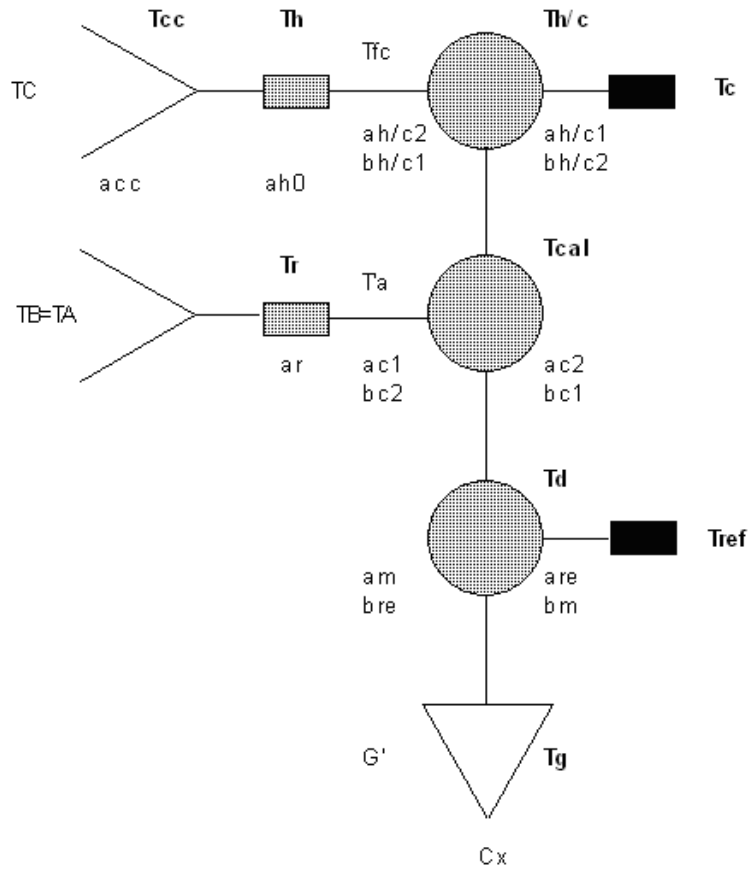
Figure 2: scheme of one channel of the MWR, showing the main antenna, whose measurement is T_A , the two calibration loads, consisting of an internal hot load and a sky horn, the reference load (Dicke load - temperature T_{ref} ) and internal switches to get every measurement. Each component is characterized by transmission and loss factors which are taken into account in the radiometer model, as well as their temperature.
