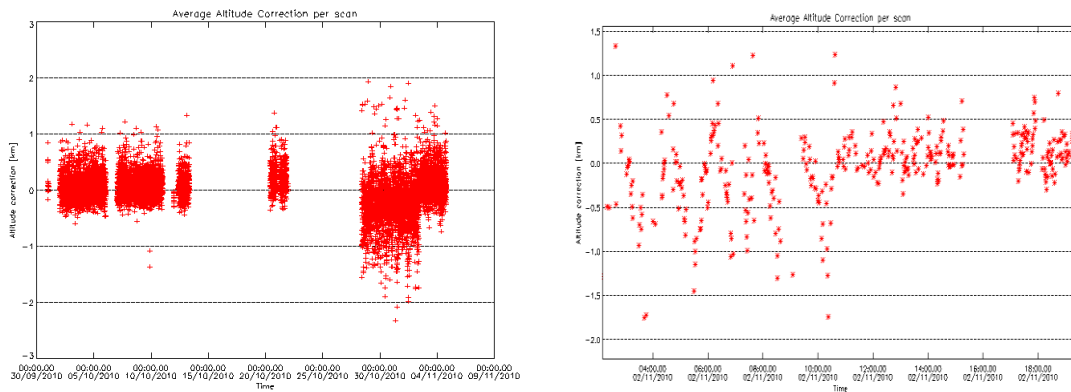
Figure 23 – MIPAS altitude correction in the Level 2 processing averaged over a scan during October 2010 (left) and zoom at the time when the ENVISA SYSM was resumed after the orbit lowering (right).
