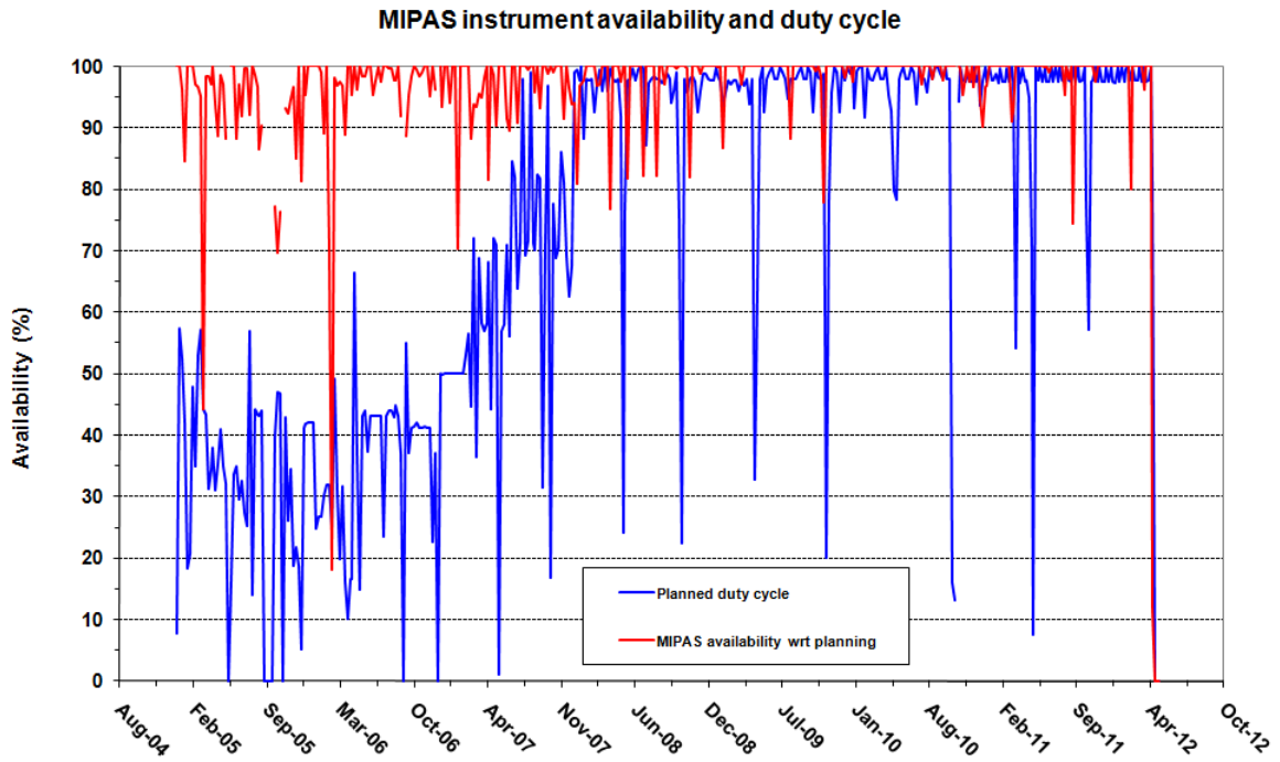
Figure 7 – MIPAS instrument availability w.r.t. planning and planned duty cycle since January 2005
