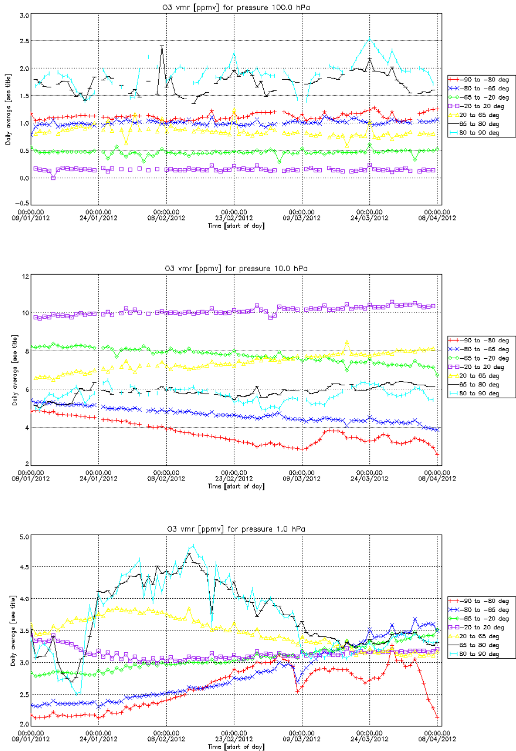
Figure 21 – MIPAS O3 VMR zonal mean at three pressure levels
