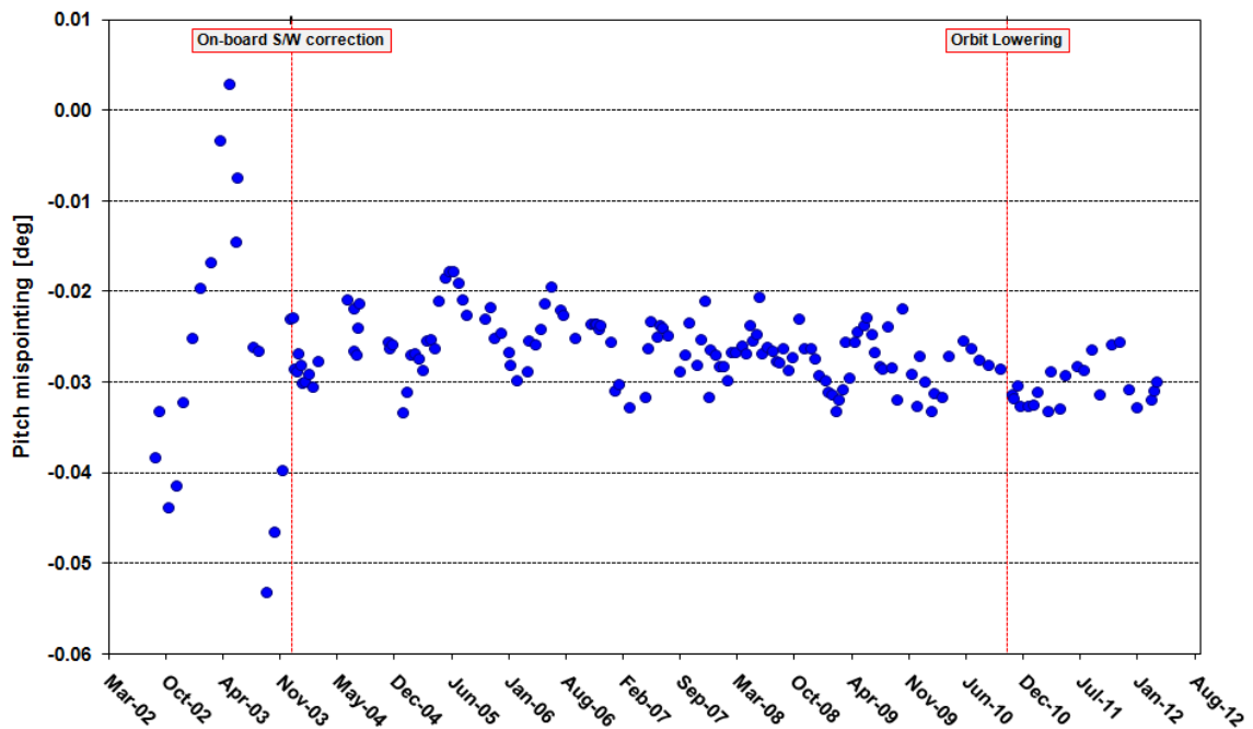
Figure 12 – MIPAS long-term pointing error as a function of time since September 2002
