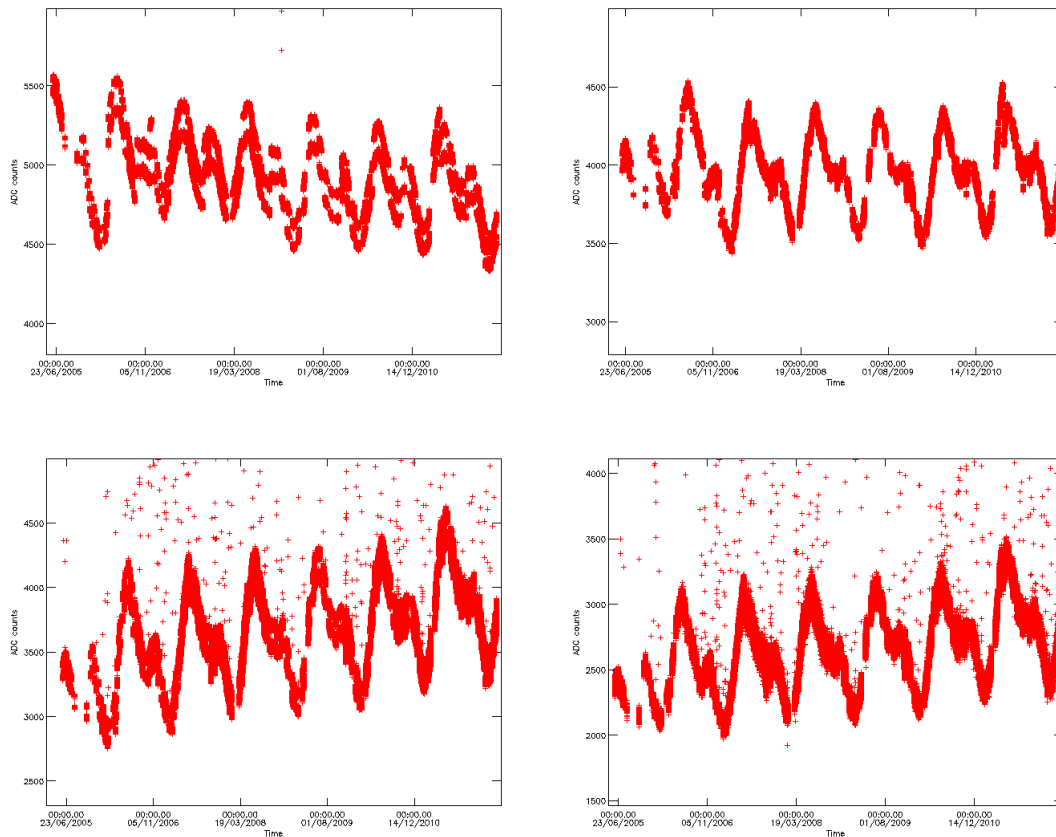
Figure 14 – ADC max counts in channel A1, B1, C1 and D1 during DS measurements since June 2005
