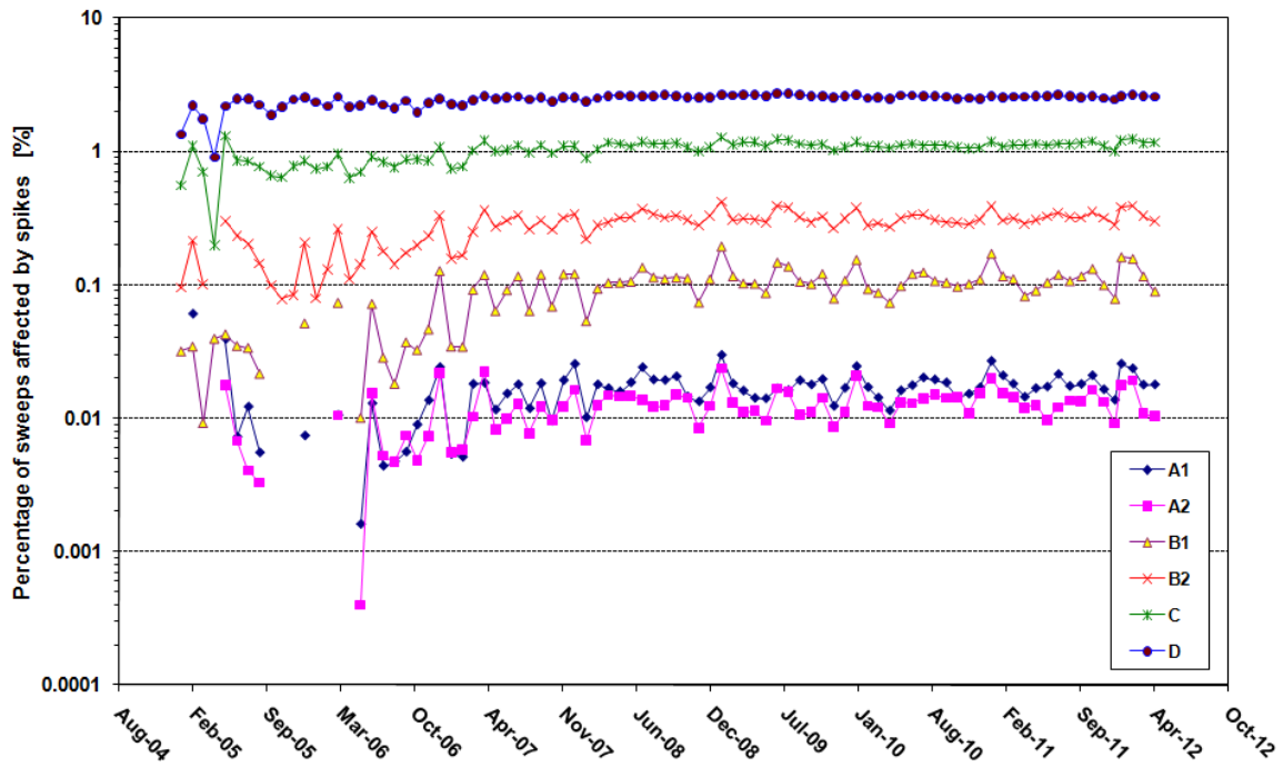
Figure 16 – MIPAS long-term monitoring of spikes: percentage of spike-affected sweeps since Jan 2005
