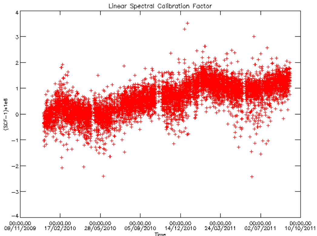
Figure 13 – MIPAS Spectral Calibration Factor (SCF) from January 2010 to September 2011
