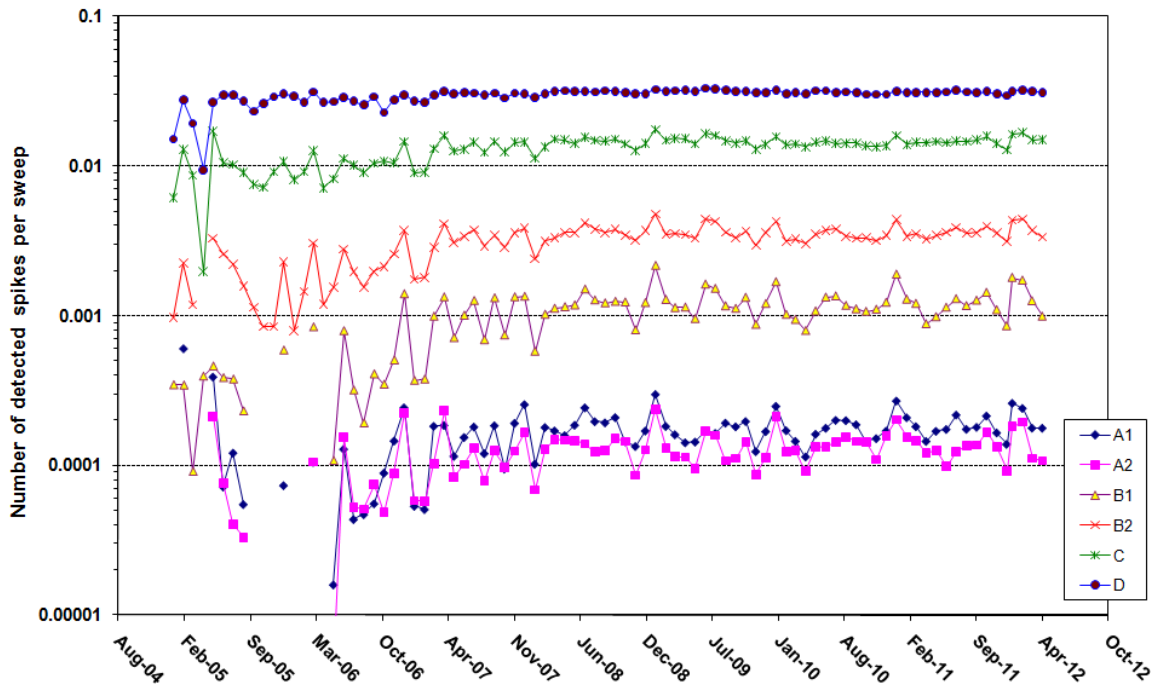
Figure 17 – MIPAS long-term monitoring of spikes: number of detected spikes per sweep since Jan 2005
