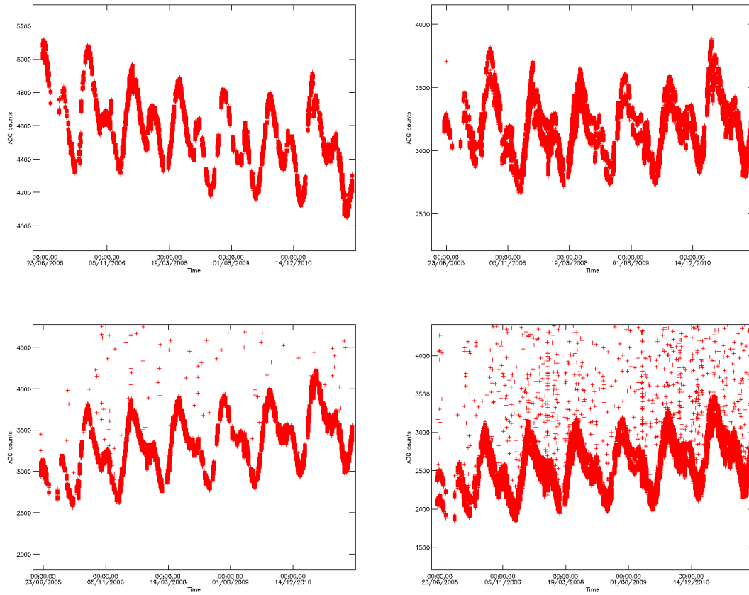
Figure 15 – ADC max counts in channel A2, B2, C2 and D2 during DS measurements since June 2005
