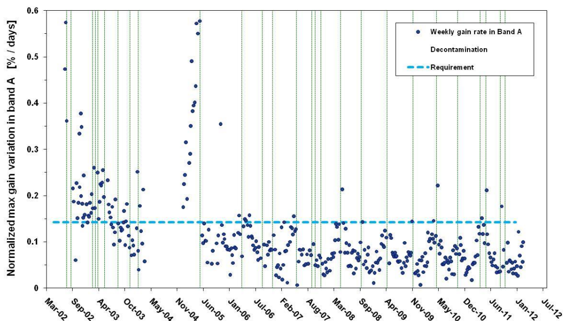
Figure 13 – Gain maximum increase normalized to the time difference between consecutive disseminated gains. The blue line represents the expected gain increase (1%/week).
