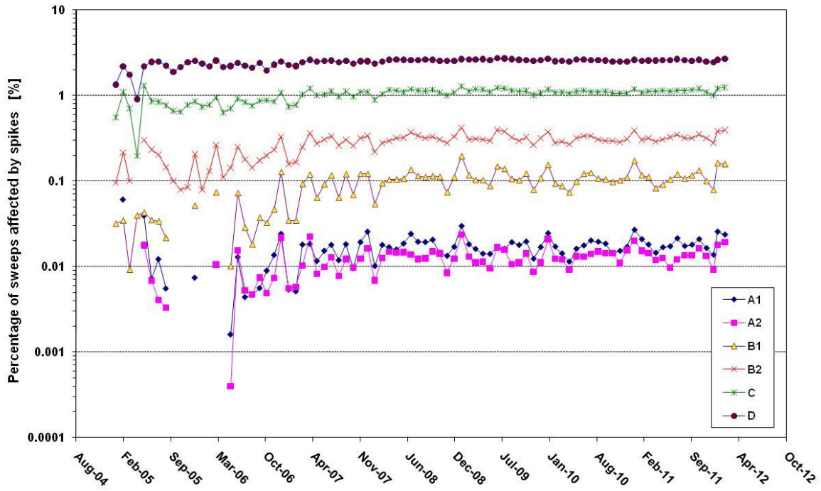
Figure 19 – MIPAS long-term monitoring of spikes: percentage of spike-affected sweeps since Jan 2005
