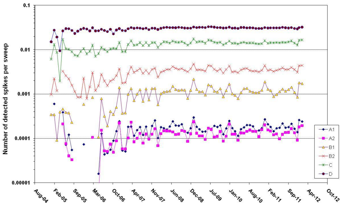
Figure 20 – MIPAS long-term monitoring of spikes: number of detected spikes per sweep since Jan 2005
