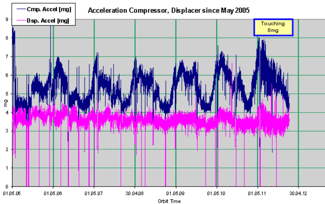
Figure 5 – Cooler Displacer and Compressor vibration level, historical trend since 2005 (courtesy of Astrium)
