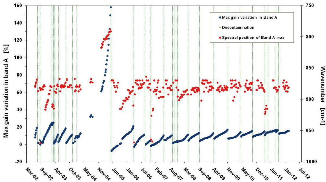
Figure 14 – Gain accumulation increase
