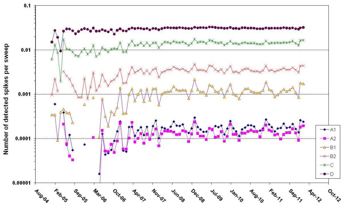
Figure 20 for the Reduced Resolution mission (starting from January 2005) in terms of percentage of sweeps affected by spikes and number of spikes/sweep.
