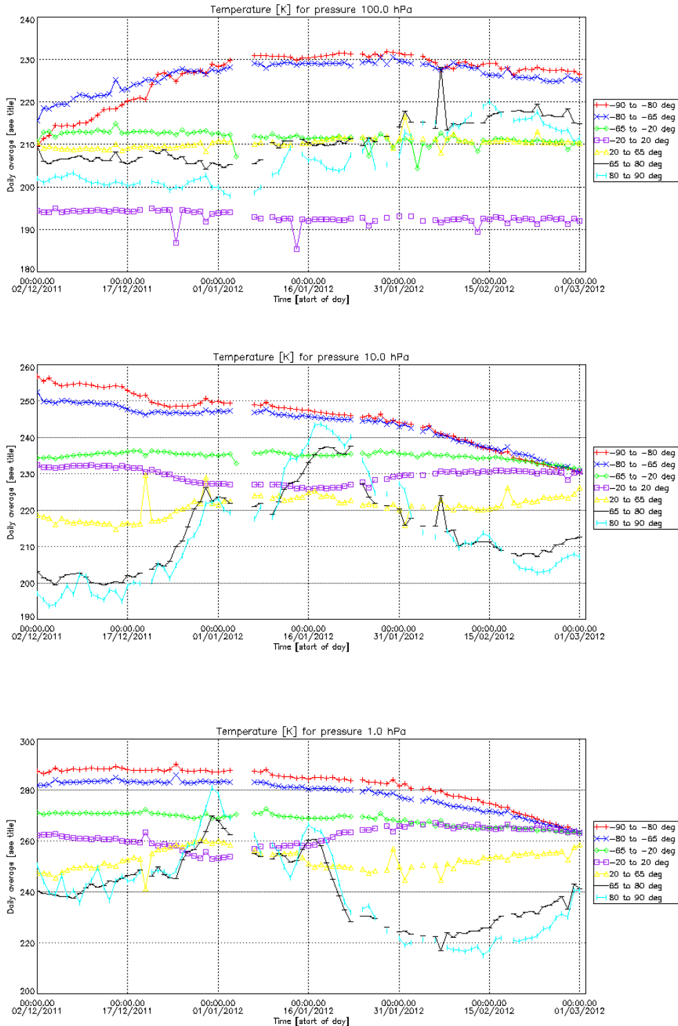
Figure 22 – MIPAS Temperature zonal mean at three pressure levels
