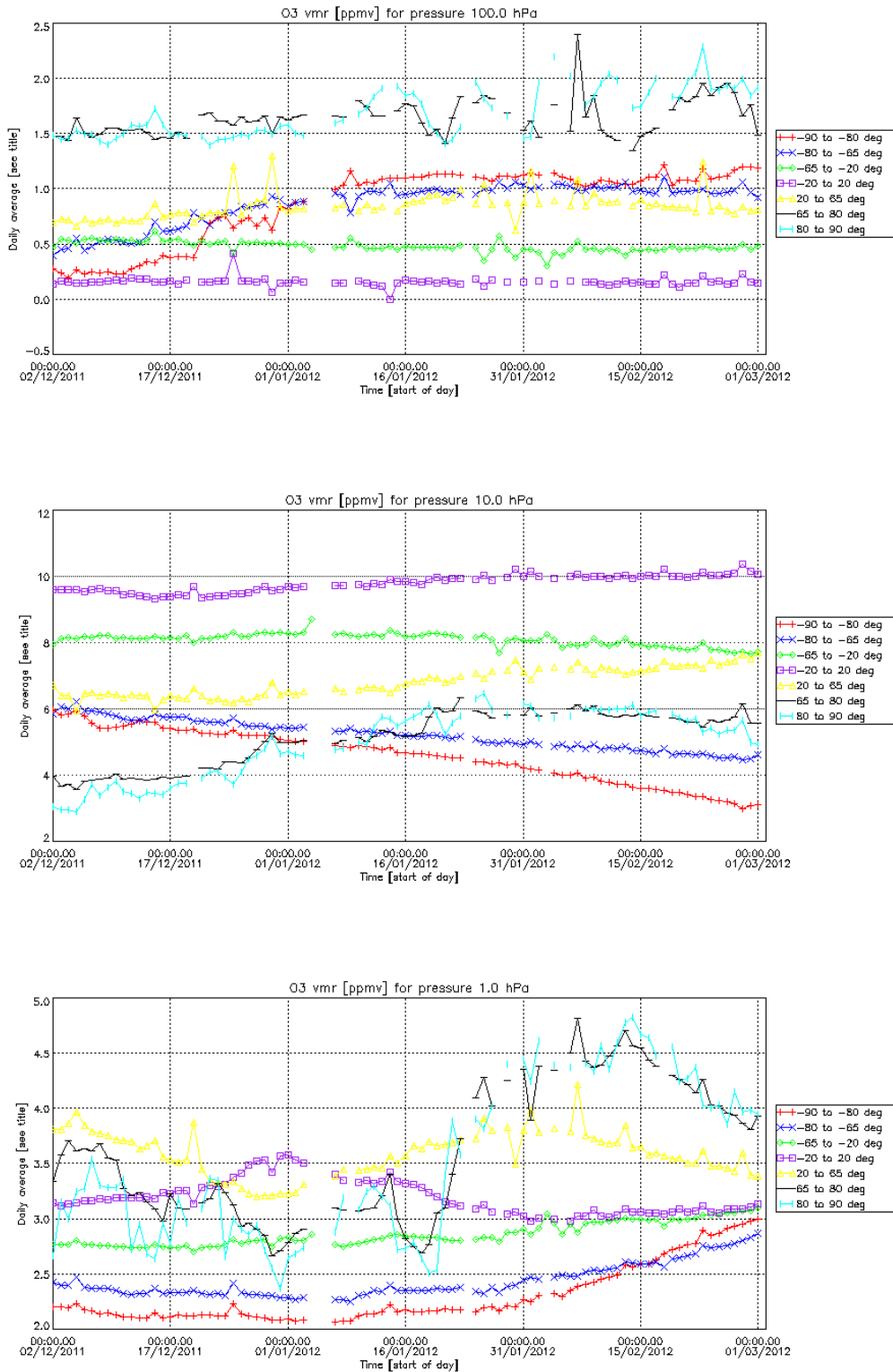
Figure 24 – MIPAS O3 VMR zonal mean at three pressure levels
