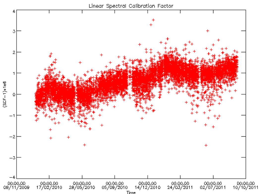
Figure 16 – MIPAS Spectral Calibration Factor (SCF) since January 2010
