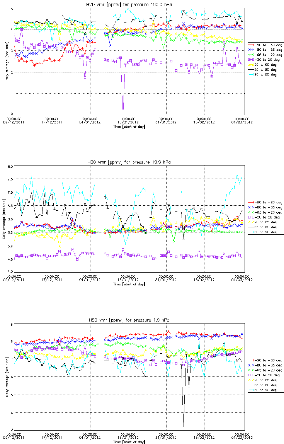
Figure 23 – MIPAS H 2 O VMR zonal mean at three pressure levels
