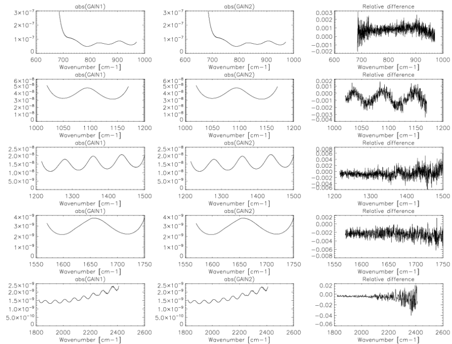
Figure 6 – Relative variations of radiometric gain for consecutive disseminated gains in band A for forward and reverse directions
