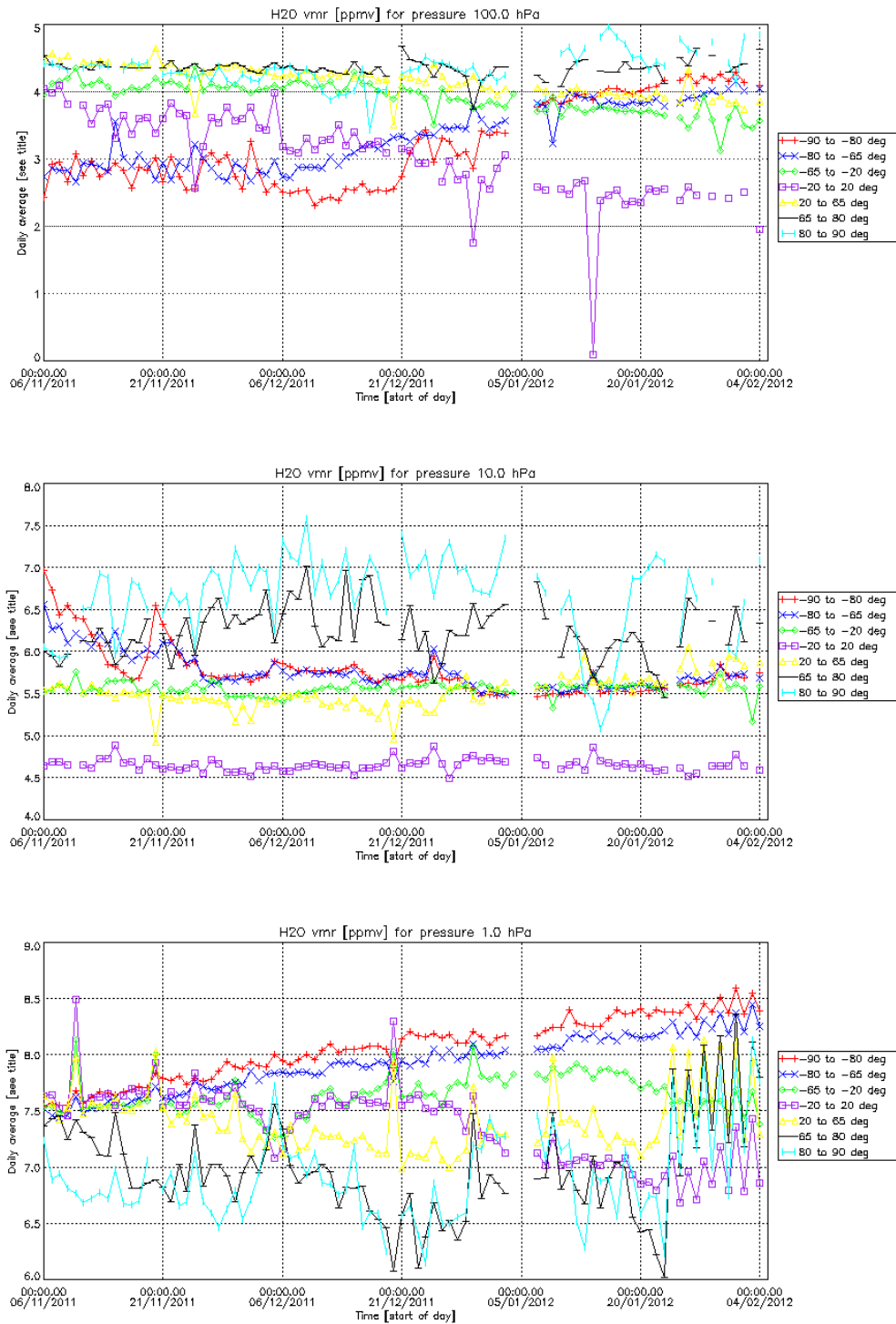
Figure 24 – MIPAS H 2 O VMR zonal mean at three pressure levels
