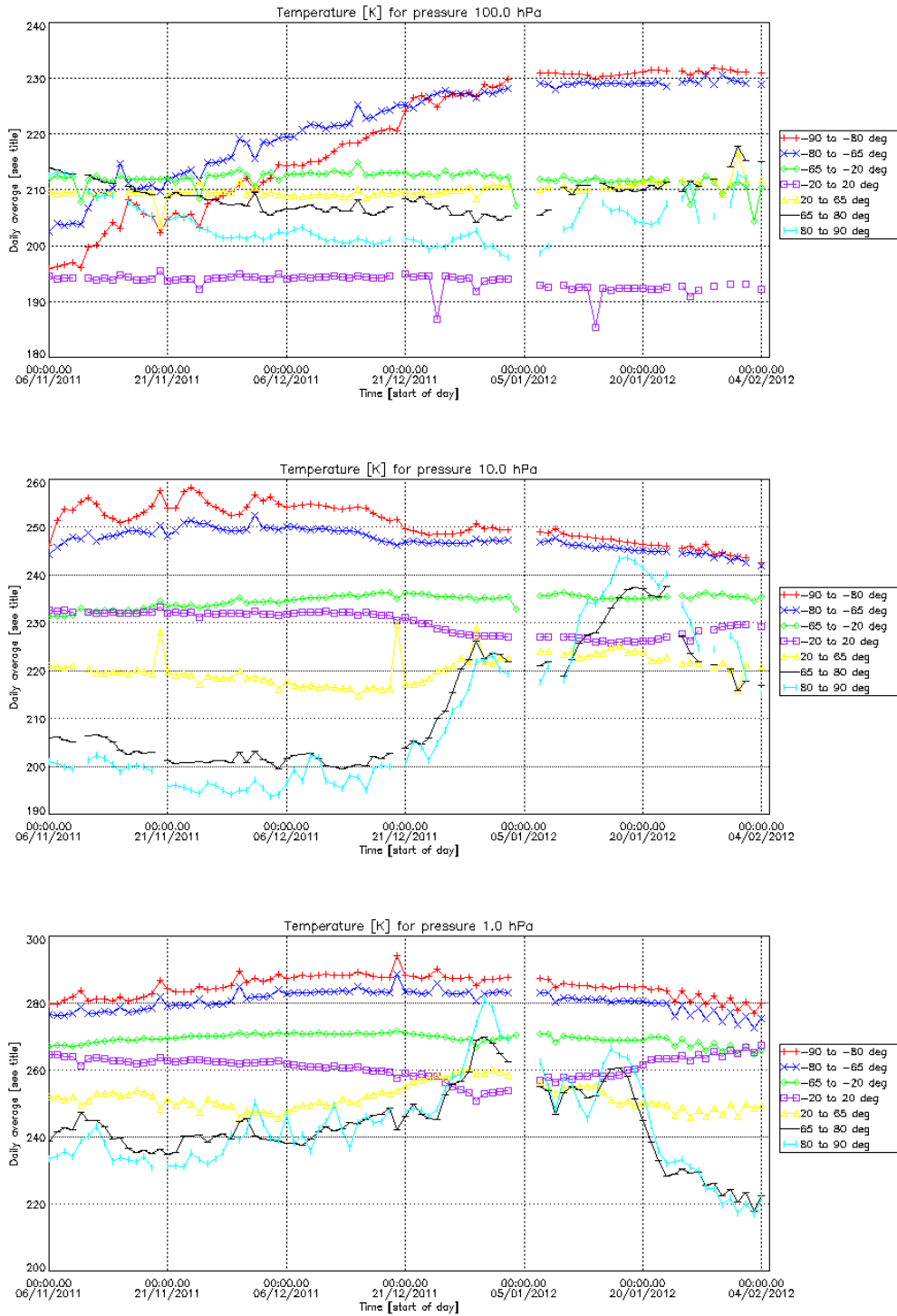
Figure 23 – MIPAS Temperature zonal mean at three pressure levels
