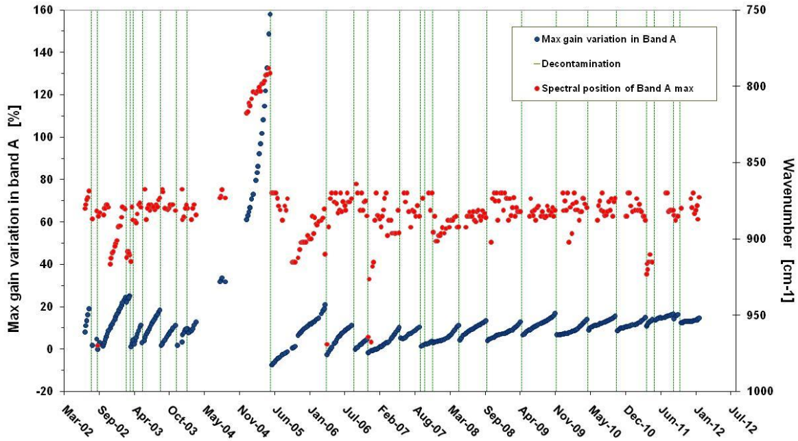
Figure 15 – Gain accumulation increase
