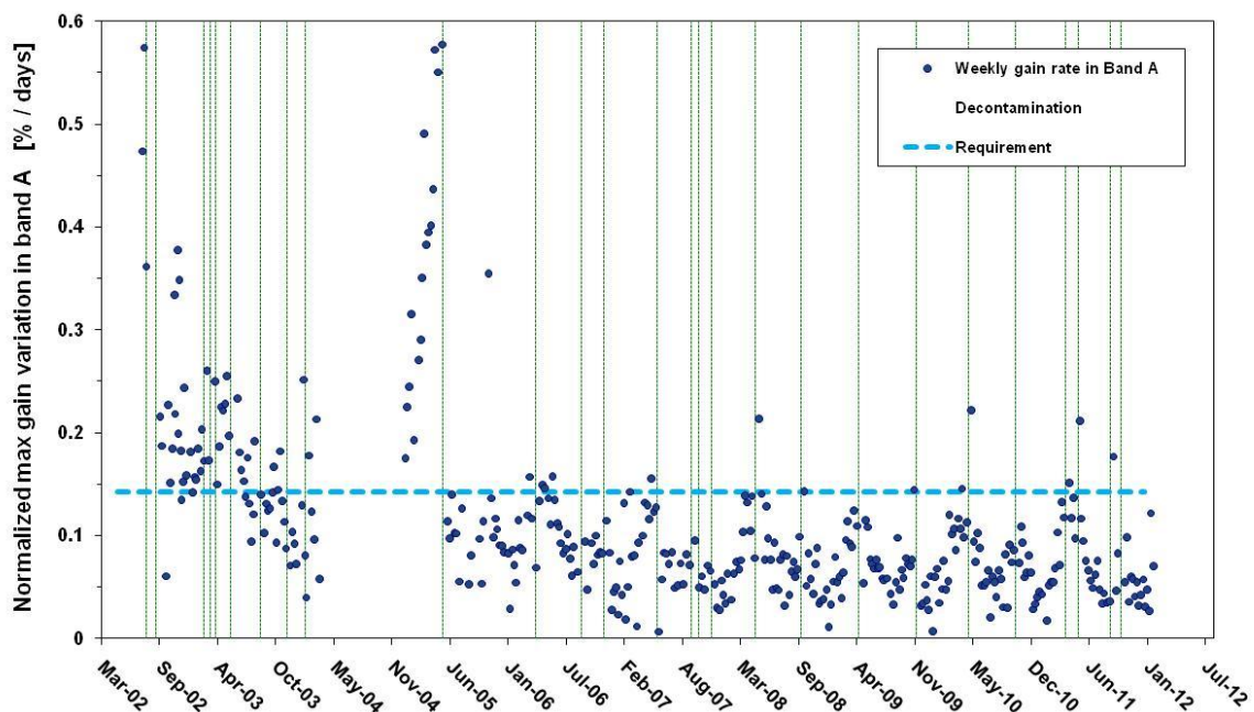
Figure 14 – Gain maximum increase normalized to the time difference between consecutive disseminated gains. The blue line represents the expected gain increase (1%/week).
