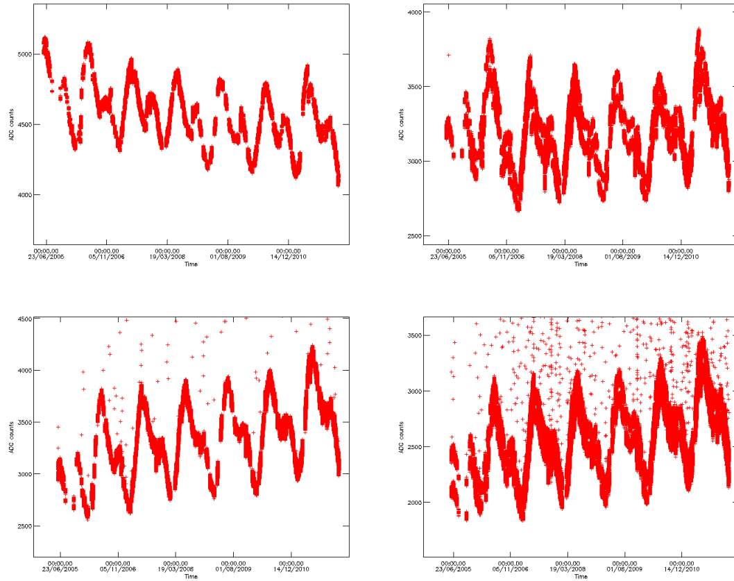
Figure 19 – ADC max counts in channel A2, B2, C2 and D2 during DS measurements since June 2005
