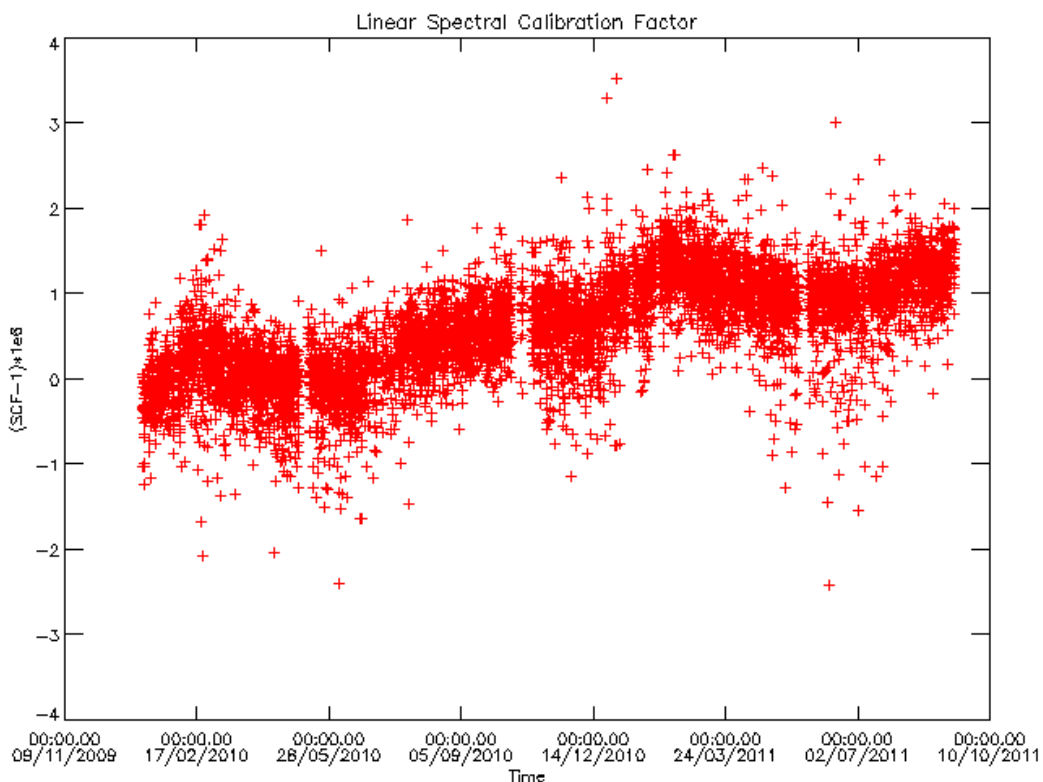
Figure 17 – MIPAS Spectral Calibration Factor (SCF) since January 2010
