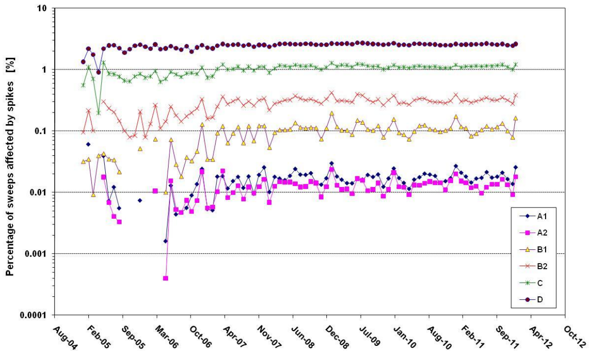
Figure 20 – MIPAS long-term monitoring of spikes: percentage of spike-affected sweeps since Jan 2005
