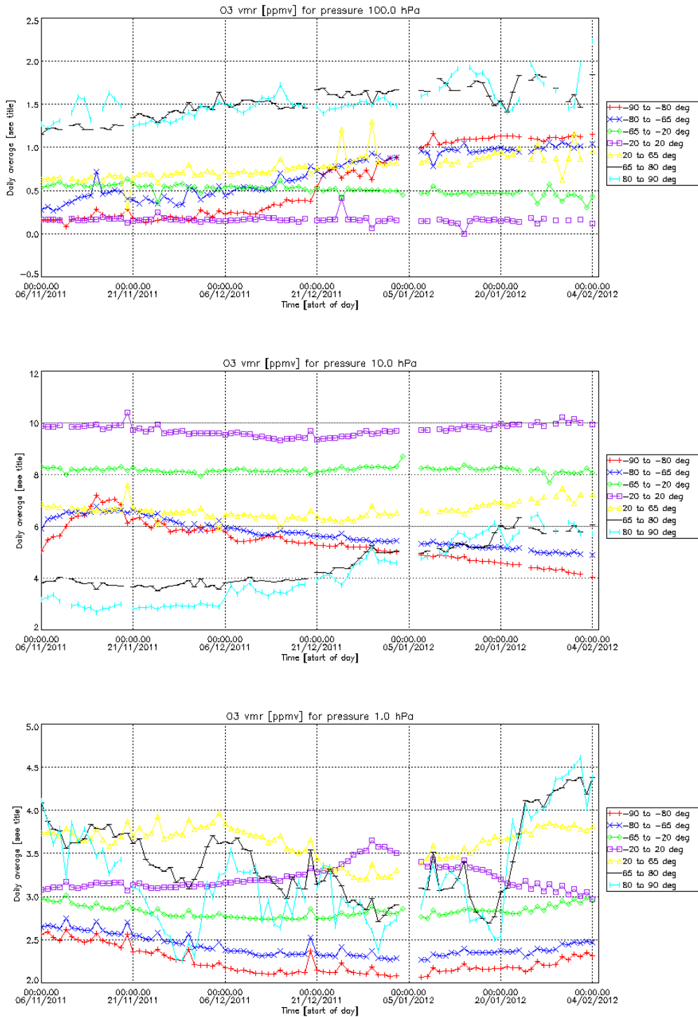
Figure 25 – MIPAS O3 VMR zonal mean at three pressure levels
