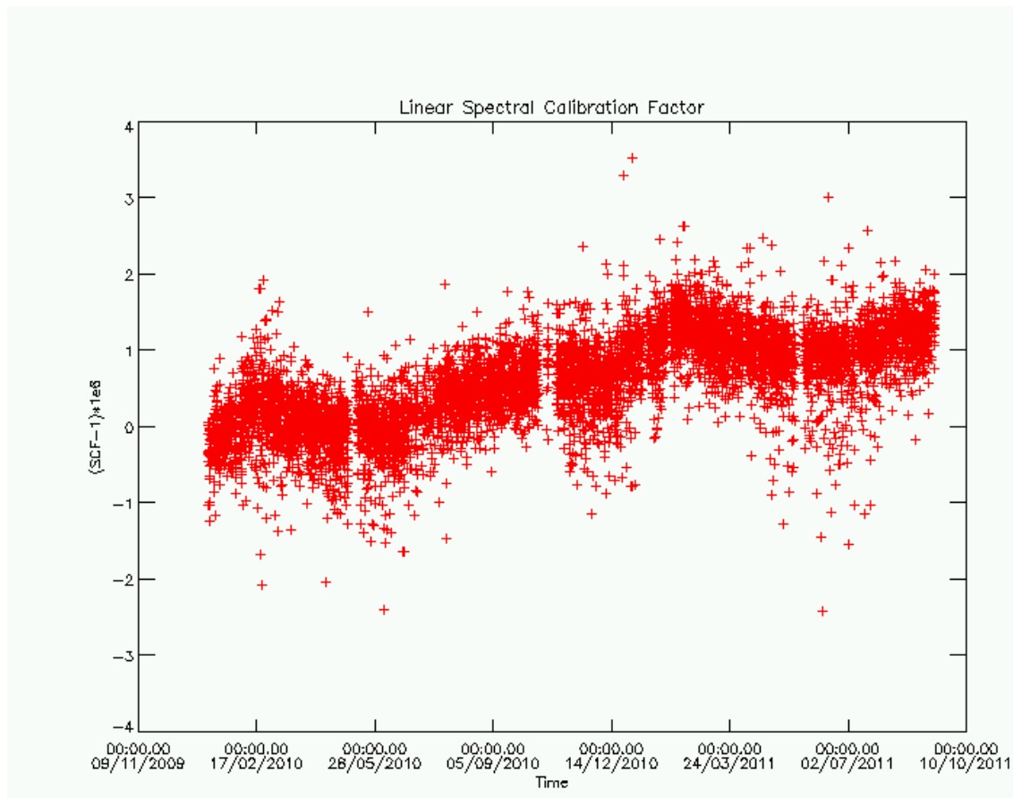
Figure 17 MIPAS Spectral Calibration Factor (SCF) since Jan 2010.
