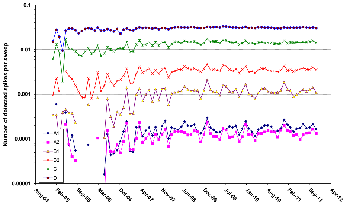
Figure 21 MIPAS long-term monitoring of spikes: number of detected spikes per sweep.
