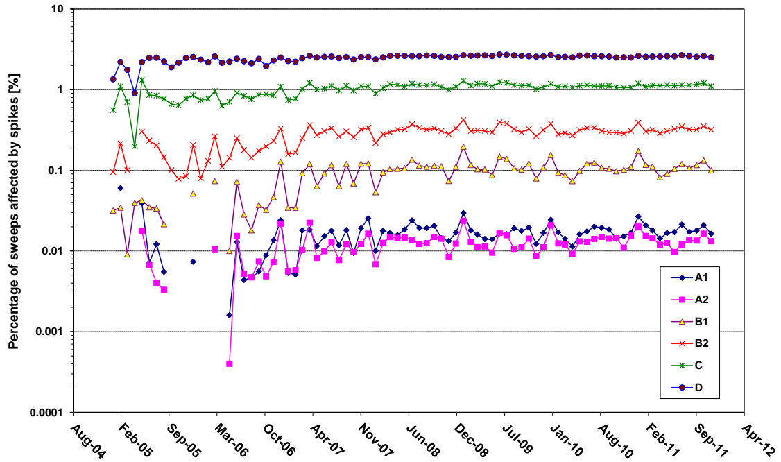
Figure 20 MIPAS long-term monitoring of spikes: percentage of spike-affected sweeps.
