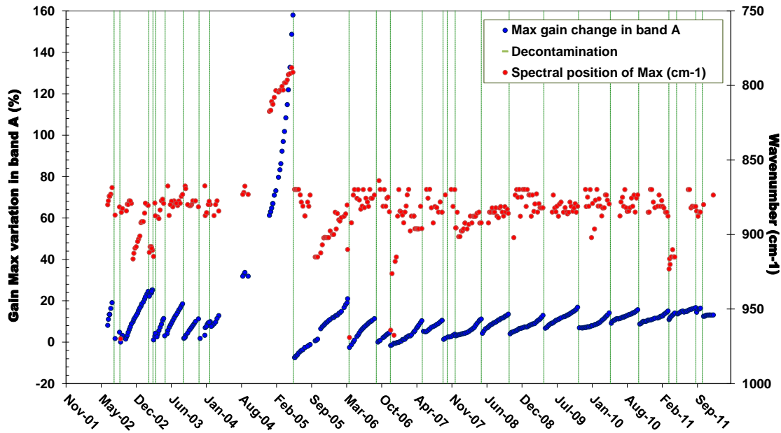
Figure 15 Gain accumulation increase since January 2005.
