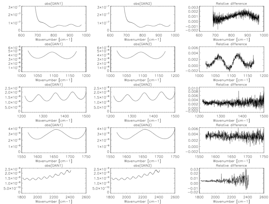
Figure 10 The same as Figure 6 but for a subsequent gain measurement.
