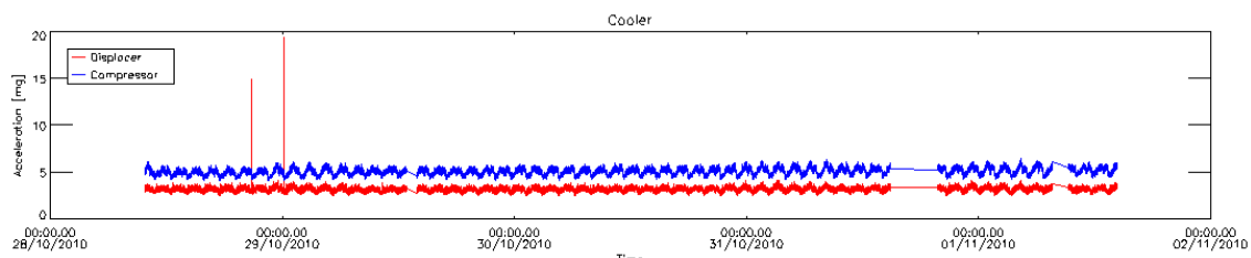
Figure 24 – MIPAS cooler acceleration level after the ENVISAT orbit lowering.
