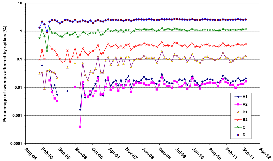
Figure 18 MIPAS long-term monitoring of spikes: percentage of spike-affected sweeps.
