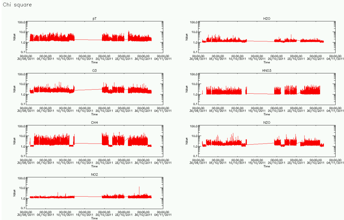
Figure 20 MIPAS last chi square values for NRT retrieval parameters.
