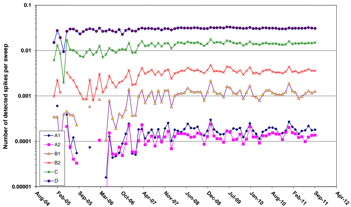
Figure 20 MIPAS long-term monitoring of spikes: number of detected spikes per sweep.
