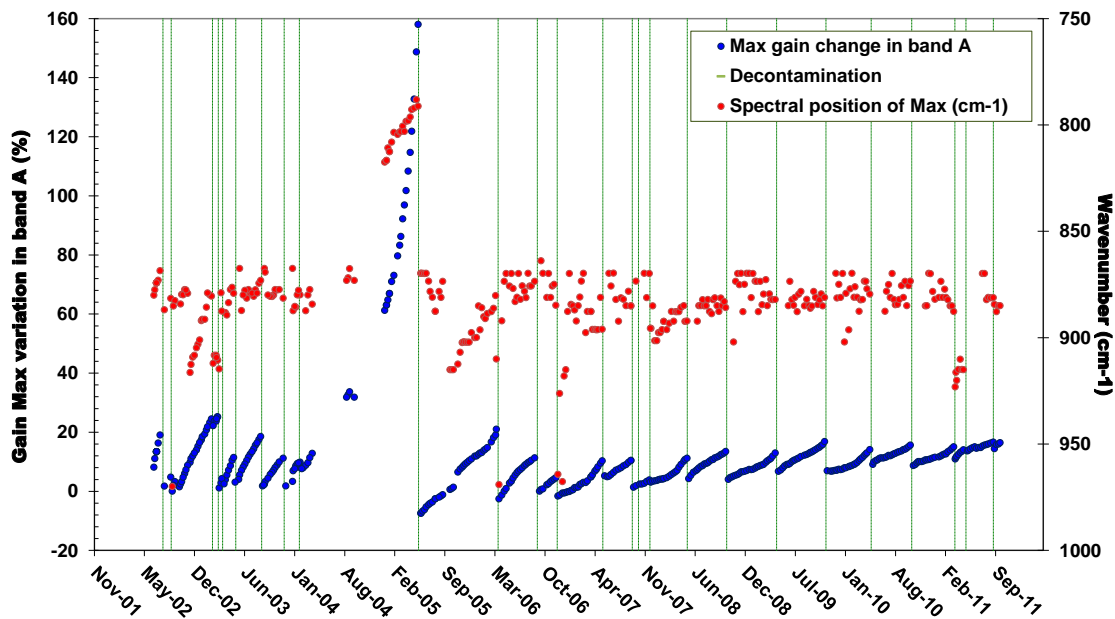
Figure 14 Gain accumulation increase since January 2005.
