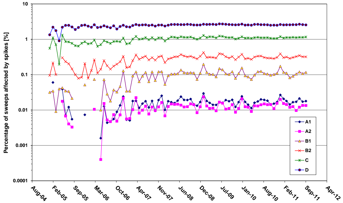
Figure 19 MIPAS long-term monitoring of spikes: percentage of spike-affected sweeps.
