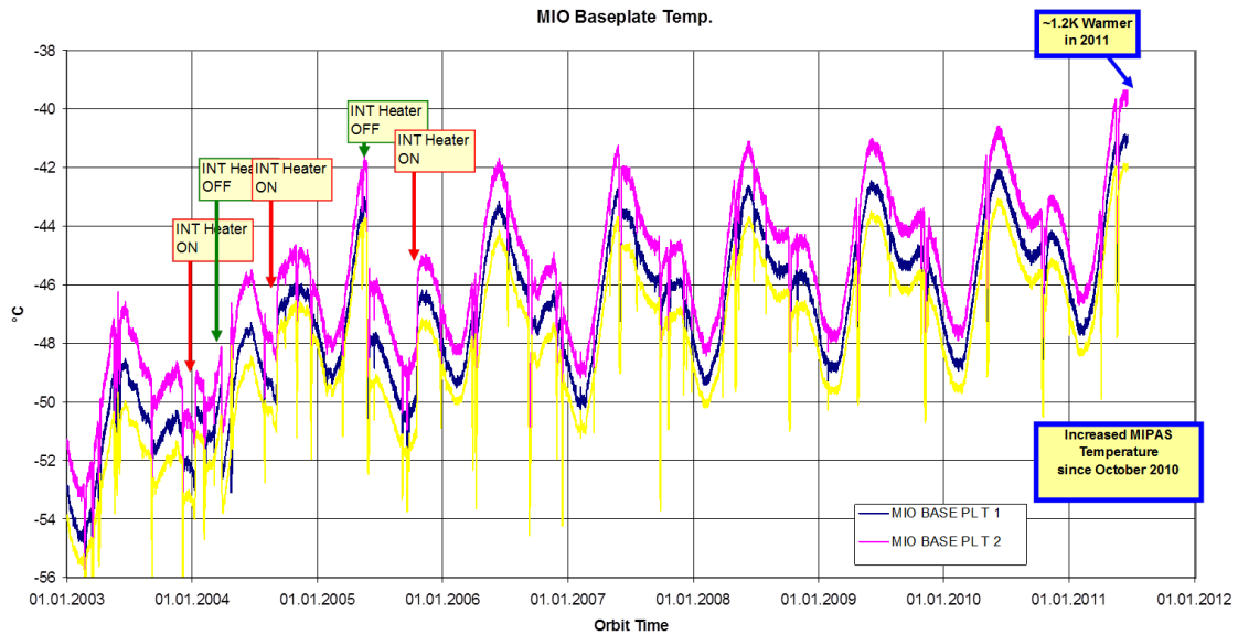
Figure 2 - MIO base plate temperatures since November 2002 (courtesy of Astrium).
