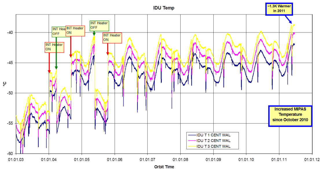
Figure 1 - IDU temperatures since November 2002 (courtesy of Astrium).
