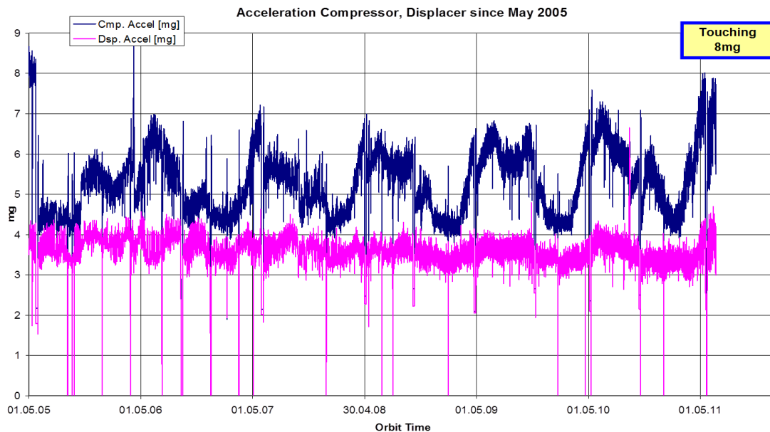
Figure 5 Cooler Displacer and Compressor vibration level, historical trend since 2005 (courtesy of Astrium).
